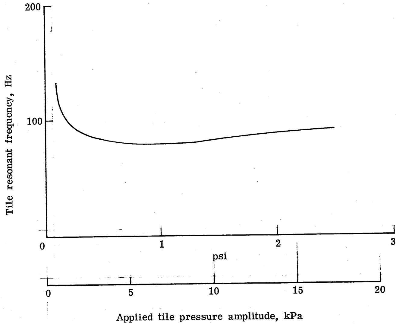
Figure 12.- Variation of resonant tile frequency with applied sinusoidal tile pressure amplitude, ( q = 2 , \zeta = .15 ).
