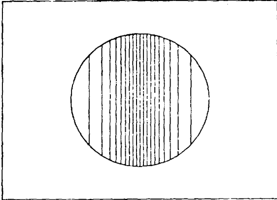
Level lines for z = \tanh px in unit circle.
