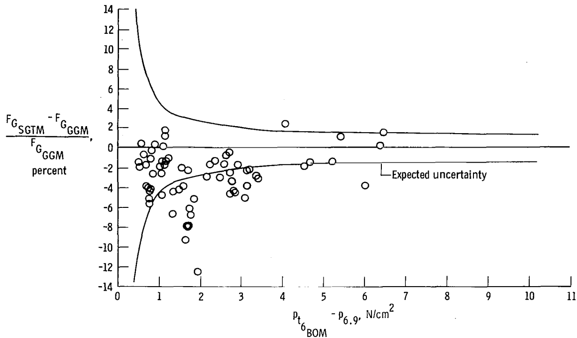
Figure 13. Difference between SGTM using p_{t6_{BOM}} and GGM gross thrust.
