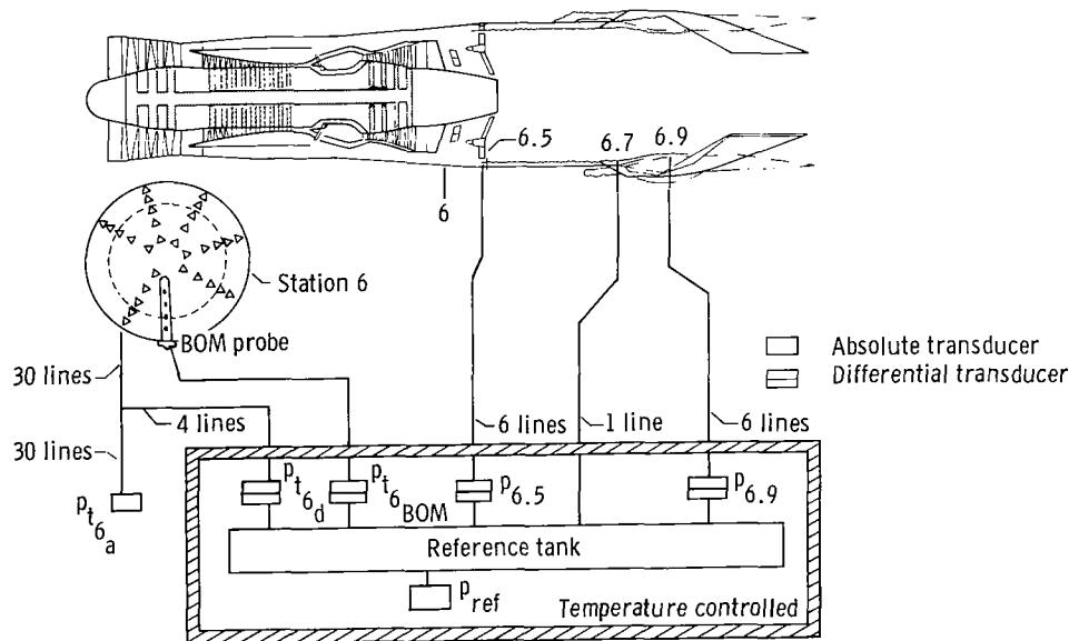
Figure 4. Schematic of pressure measurement system for stations 6, 6.5, and 6.9.
