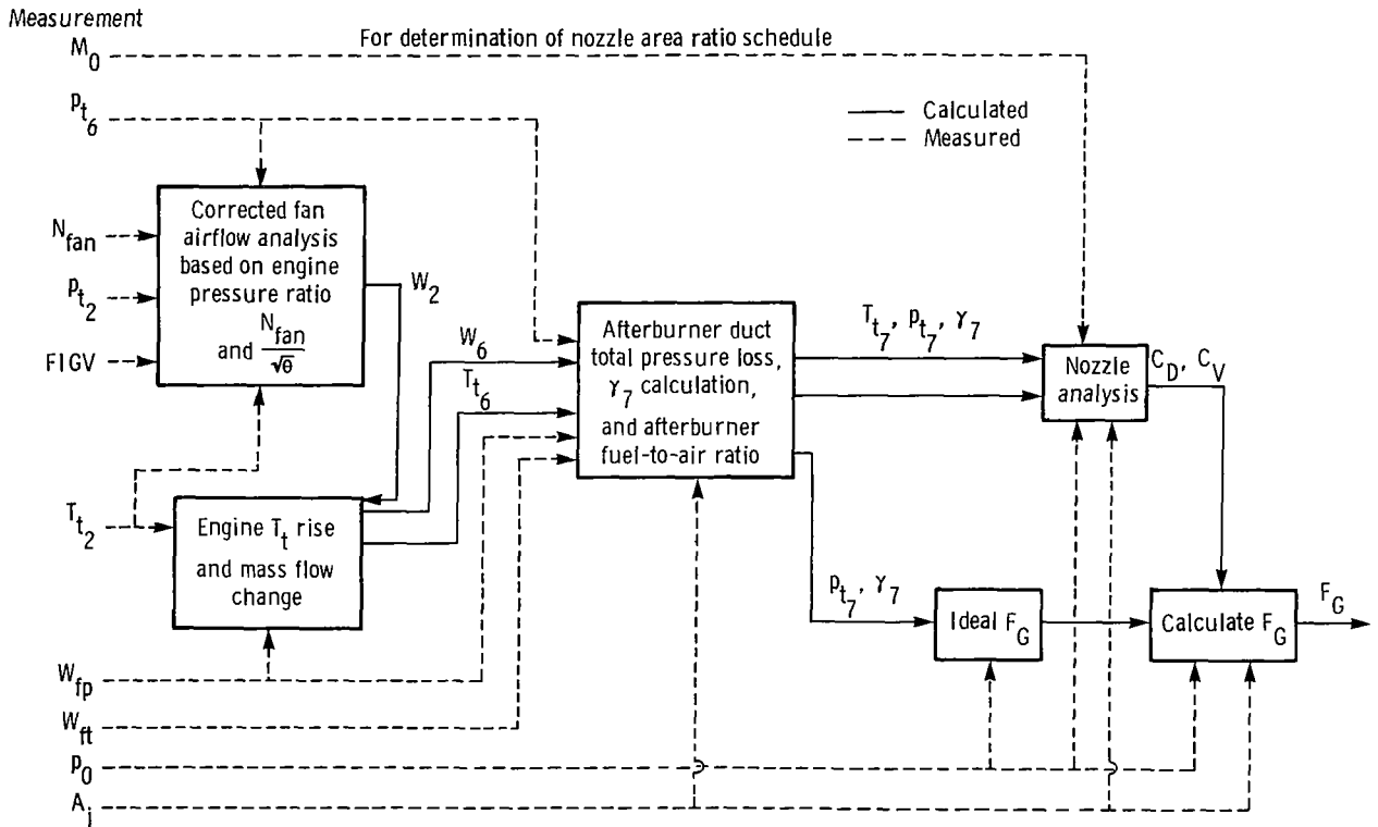
Figure 6. Engine gas generator performance model.
