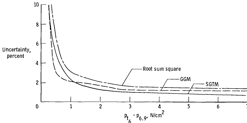
Figure 11. Expected uncertainty of the combined GGM and SGTM.
