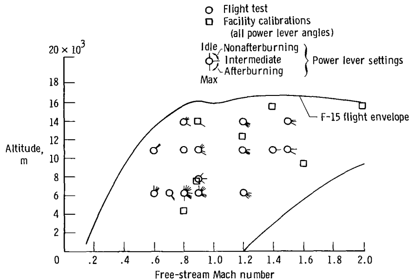
Figure 5. Flight test and facility calibration conditions.
