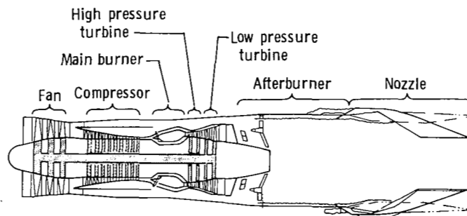
Figure 2. Schematic representation of F100-PW-100 engine.
