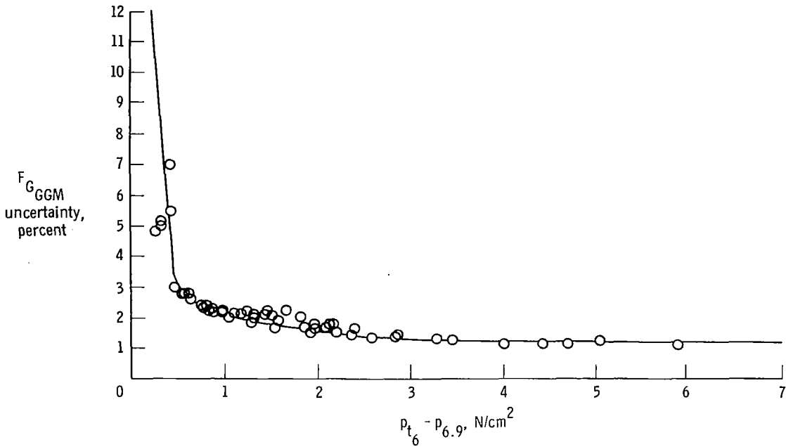
Figure 10. Uncertainty in gas generator model.
