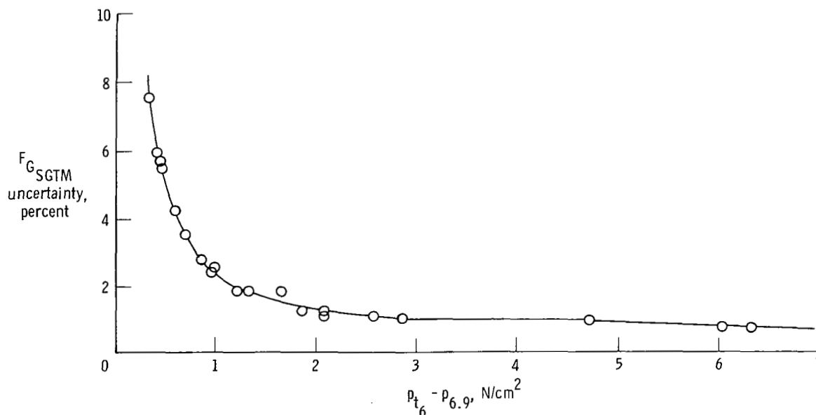
Figure 9. Uncertainty in SGTM.
