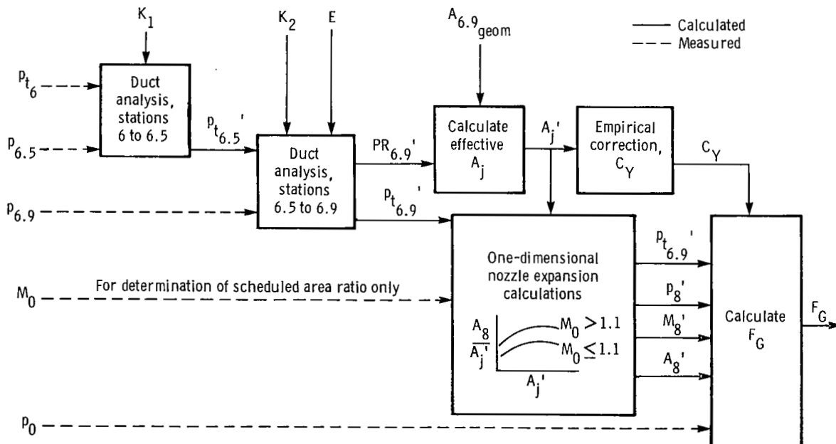
Figure 7. Simplified gross thrust model. Choked flow case, \gamma = 1.3 .
