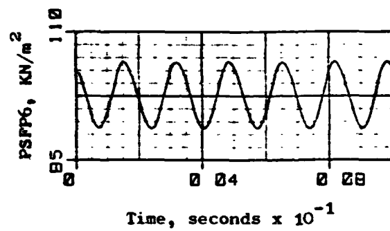
Figure 26. J85-13/P 3 G Simulation Results, f_{P^3G} = 600\text{Hz} .
