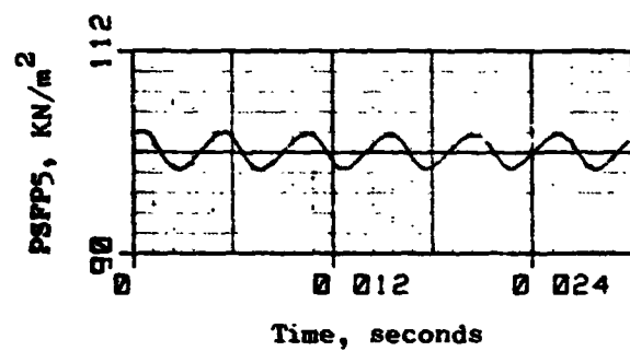
Figure C-3. J85-13/P 3 G Simulation Results, f_{p3G} = 200\text{Hz} .
