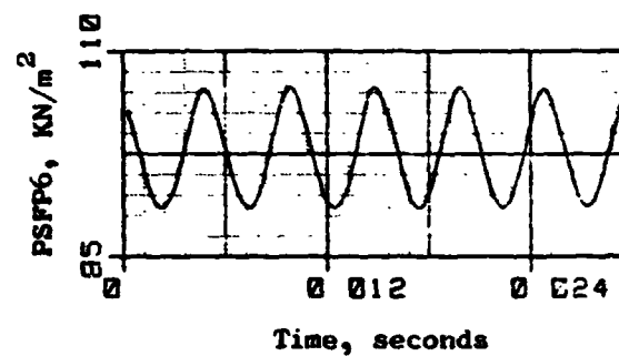
Figure C-3. J85-13/P 3 G Simulation Results, f_{p3G} = 200\text{Hz} .
