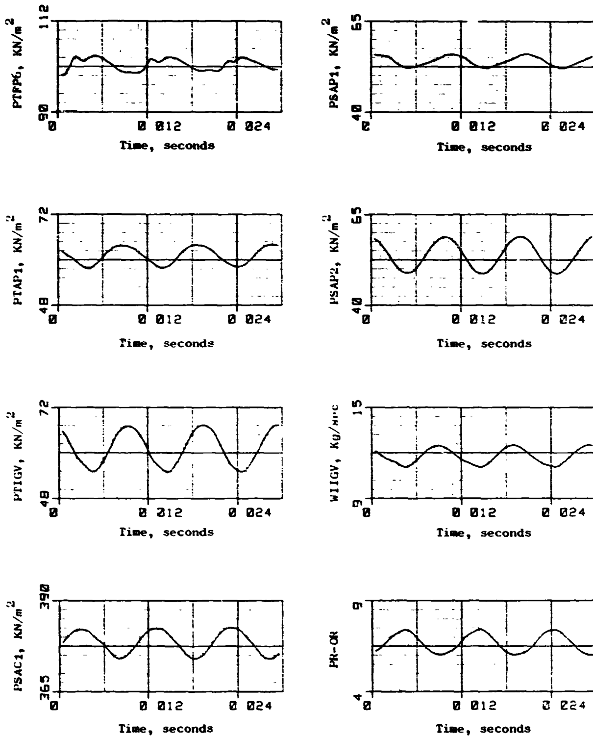
Figure 23. J85-13/P 3 G Simulation Results, f_{pG} = 100\text{Hz} (Concluded). 63
