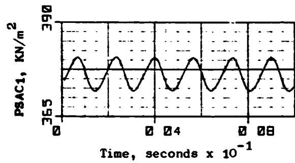
Figure 27. J85-13/P 3 G Simulation Results, f_{P^3G} = 600\text{Hz} (Concluded). 67
