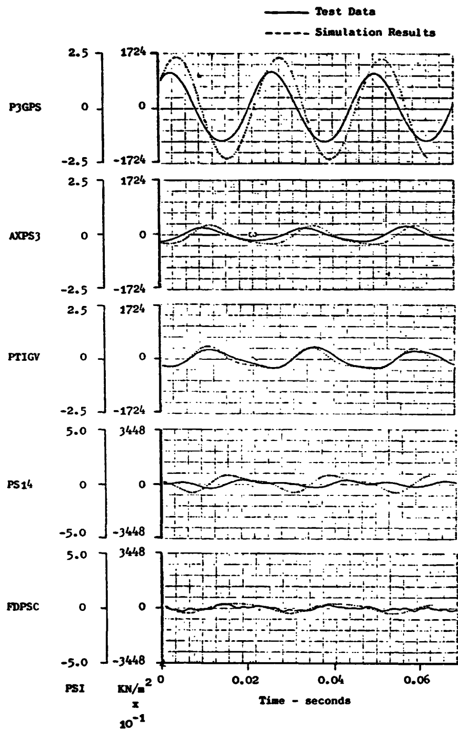
Figure 16. F101 Fan/P 3 G Simulation, 100% N/√θ, 42Hz.
