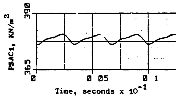
Figure C-6. J85-13/P 3 G Simulation Results, f_{P^3G} = 300\text{Hz} (Concluded).
