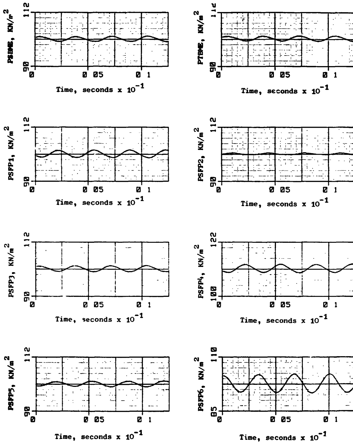
Figure C-5. J85-13/P 3 G Simulation Results, f_{P^3G} = 300\text{Hz} .
