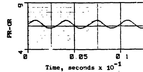
Figure C-6. J85-13/P 3 G Simulation Results, f_{P^3G} = 300\text{Hz} (Concluded).
