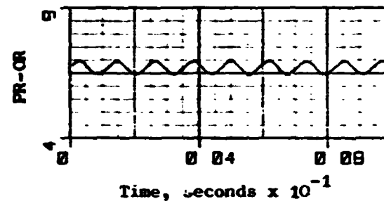
Figure C-10. J85-13/P 3 G Simulation Results, f_{pG} = 850\text{Hz} (Concluded).
