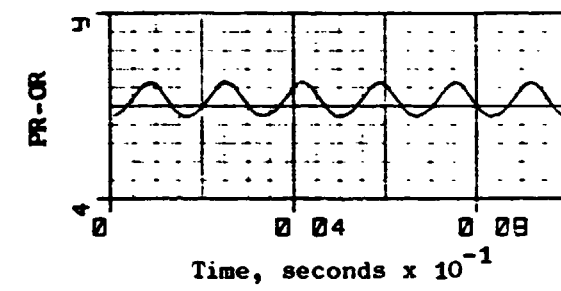
Figure 27. J85-13/P 3 G Simulation Results, f_{P^3G} = 600\text{Hz} (Concluded). 67
