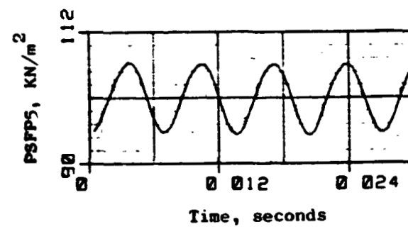
Figure C-1. J85-13/P 3 G Simulation Results, f_{p^3G} = 150\text{Hz} .
