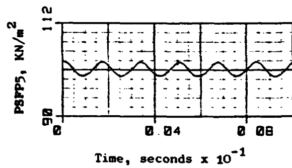
Figure 26. J85-13/P 3 G Simulation Results, f_{P^3G} = 600\text{Hz} .
