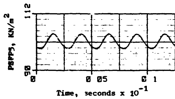
Figure C-7. J85-13/P 3 G Simulation Results, f_{P^3G} = 400\text{Hz} .
