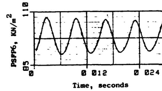
Figure C-1. J85-13/P 3 G Simulation Results, f_{p^3G} = 150\text{Hz} .
