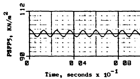
Figure C-9. J85-13/P 3 G Simulation Results, f_p^3 G = 850\text{Hz} .
