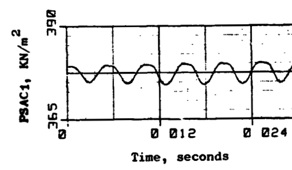
Figure C-4. J85-13/P 3 G Simulation Results, f_{pG} = 200\text{Hz} (Concluded).
