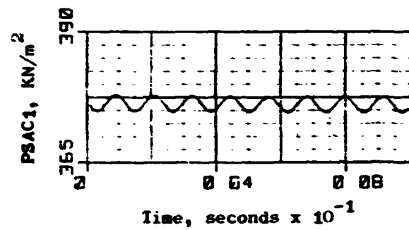
Figure C-10. J85-13/P 3 G Simulation Results, f_{pG} = 850\text{Hz} (Concluded).
