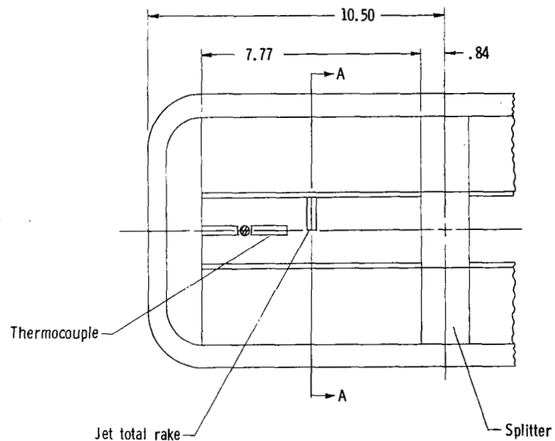
Figure 5.- Sketches of dry power convergent-divergent nozzle flap arrangement showing important dimensions. All dimensions are in centimeters unless otherwise noted.
