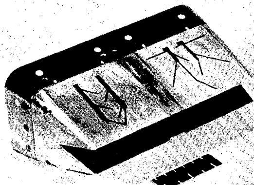
(p) Center line vented sidewall, center line vented splitter.
