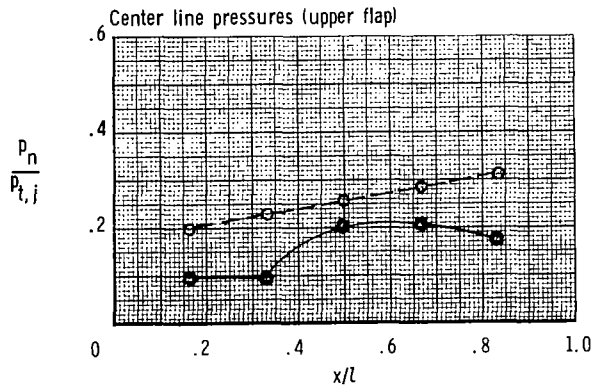
Figure 32.- Variation of nozzle internal static-pressure distribution with jet total pressure ratio at test Mach numbers for afterburning power nozzle with 50 percent sidewall, 100 percent splitter.
