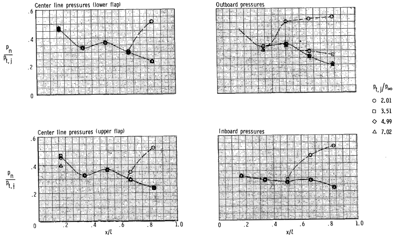
Figure 30.- Variation of nozzle internal static-pressure distribution with jet total pressure ratio at test Mach numbers for dry power nozzle with center line vented sidewall, divergent splitter.
