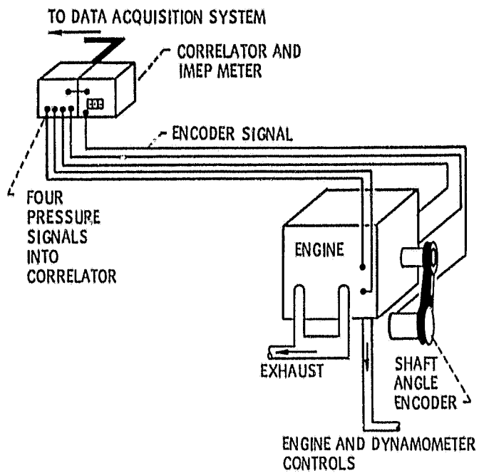
Figure 2. - Test configuration.
