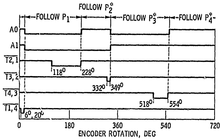
Figure A3. - Timing diagram.
