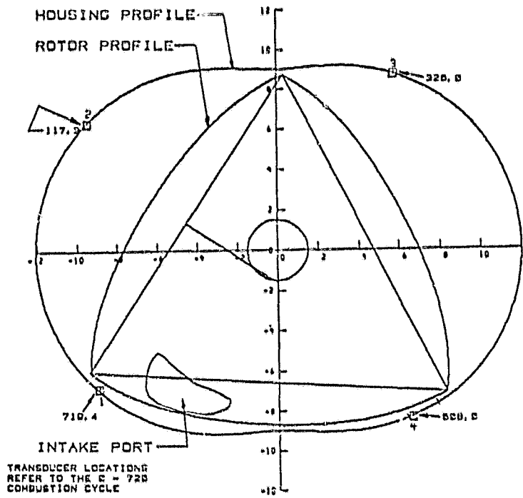
Figure 4. - Transducer locations.
