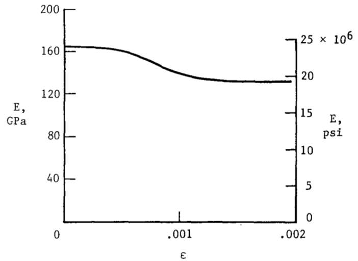
(l) [0_2/\pm 45]_S laminate at 505 K (450°F).
