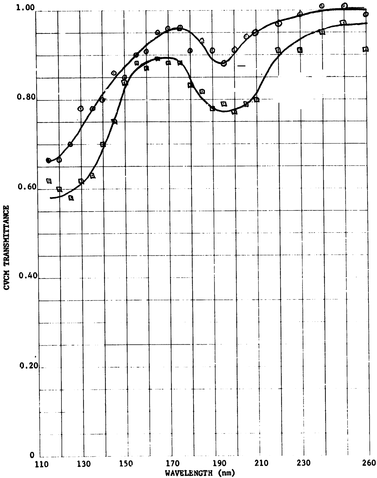
Figure 29. CVC M Transmittance Versus Wavelength, Source Material Z-306/9922, JPL#131-VOD-2, CVC M Thickness In Angstroms \odot 68, \square 104.
