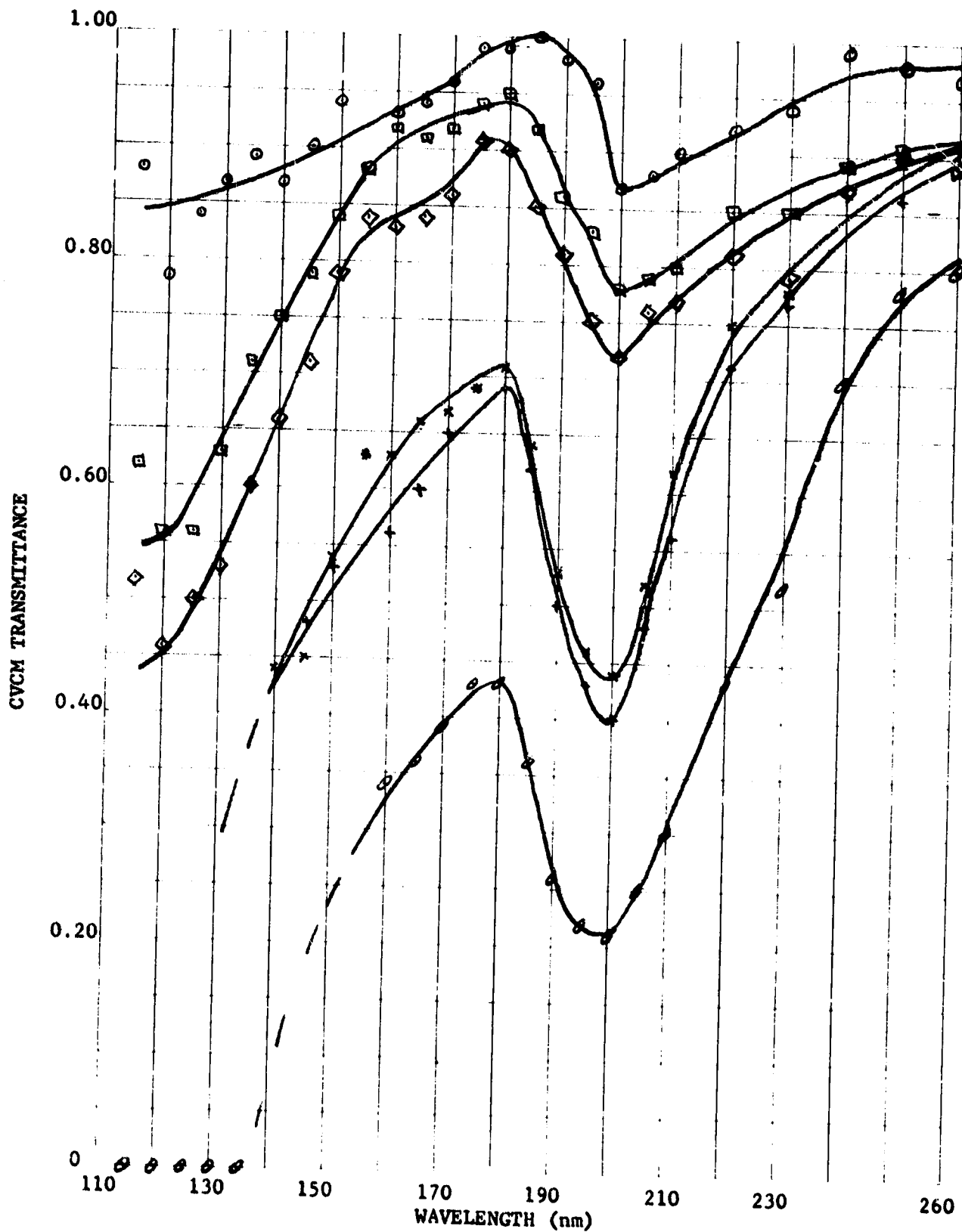
Figure 49. CVCM Transmittance Versus Wavelength, Source Material 3M Nextel 401-C10/901-P1, JPL#144-VOD-1, CVCM Thickness In Angstroms \circ 44, \square 116, \diamond 159, \times 404, + 492, \circ 1013.
