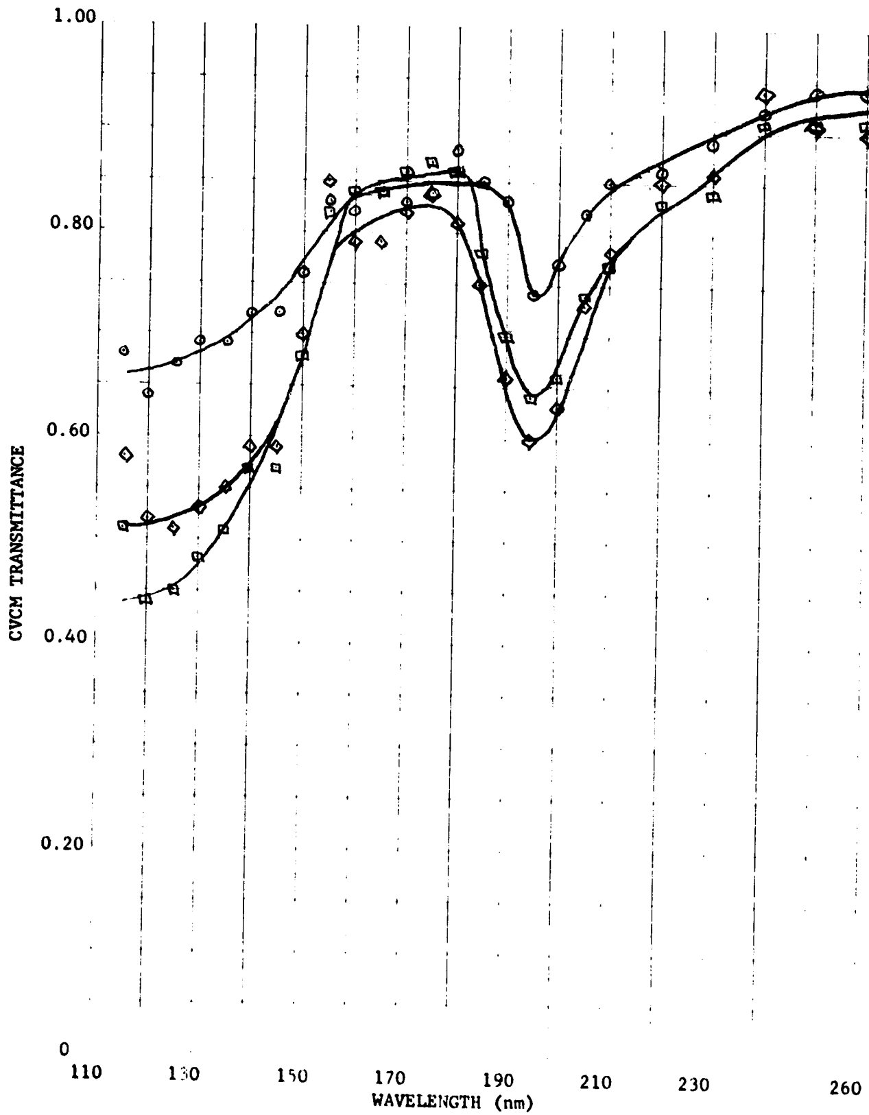
Figure 19. CVCm Transmittance Versus Wavelength, Source Material Scotch-Weld 2216, Cured 9 Hr Ambient/5 Hr 125°F, CVCm Thickness ○ 57, □ 160, ◇ 193.
