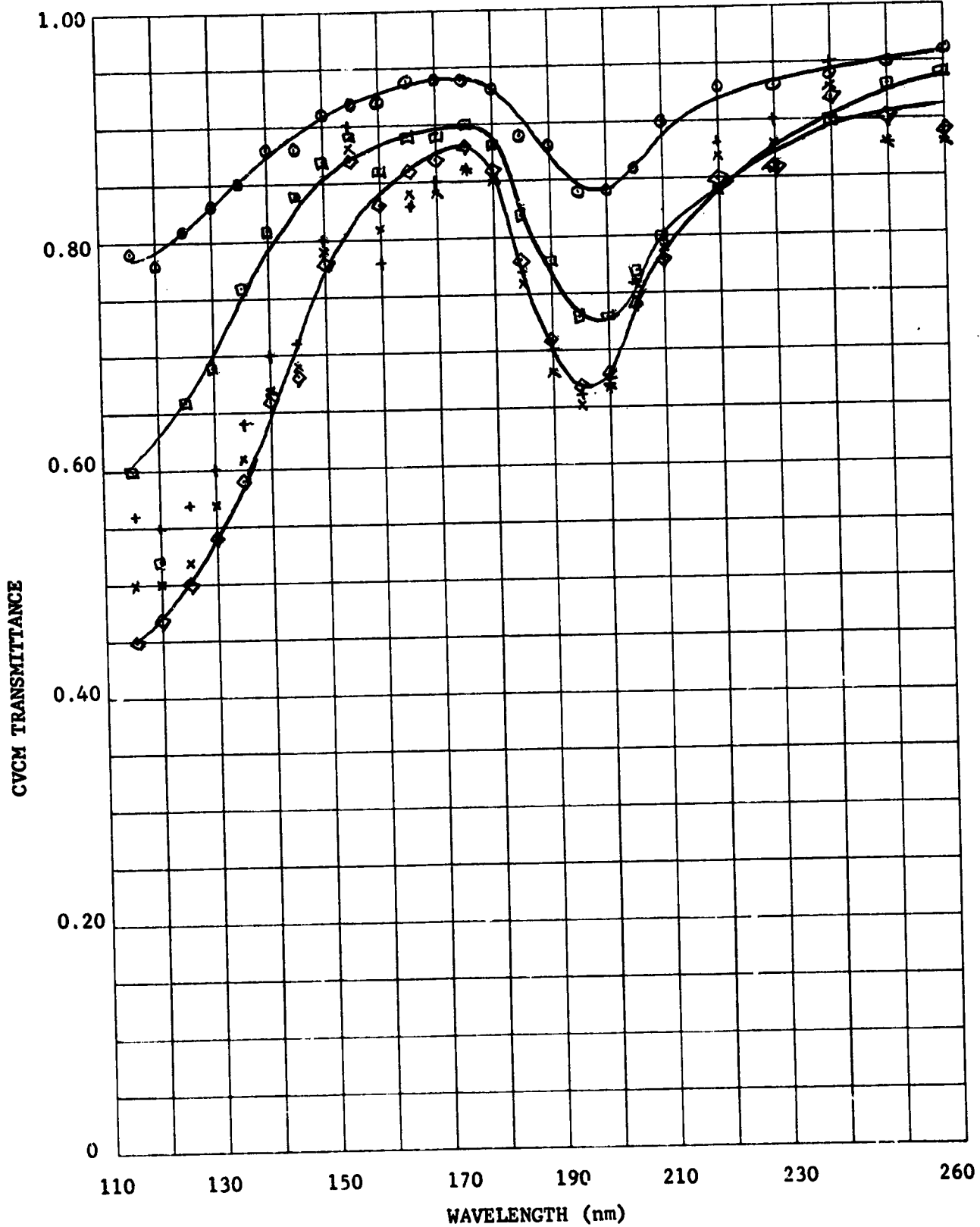
Figure 27. CVCN Transmittance Versus Wavelength, Source Material Chemglaze Z-306/9922, JPL#131-VOD-1, CVCN Thickness In Angstroms \circ 60, \square 118, \diamond 193, \times 203, + 212.
