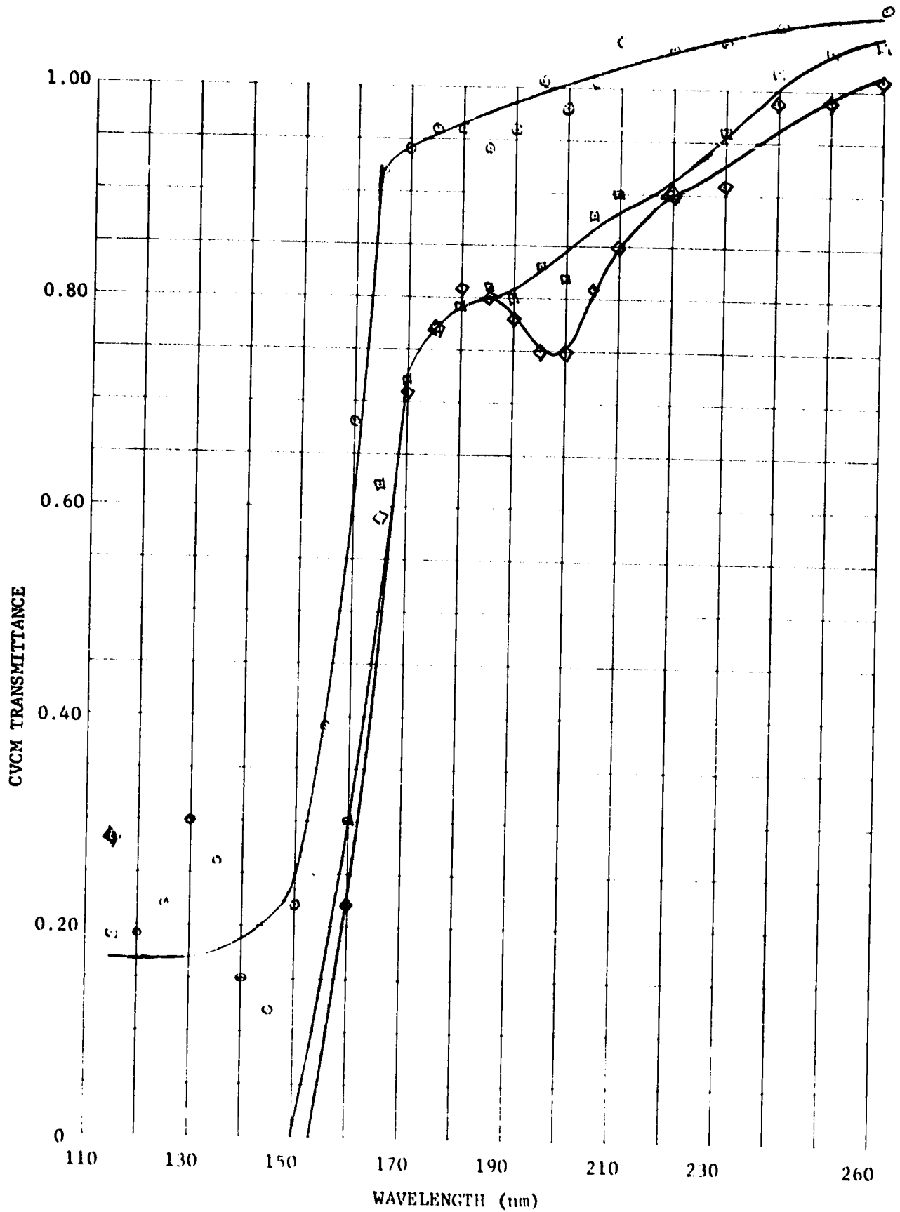
Figure 9. CVCm Transmittance Versus Wavelength, Source Material Trabond BB-2116, CVCm Thickness In Angstroms \circ 72, \square 151, \diamond 208.
