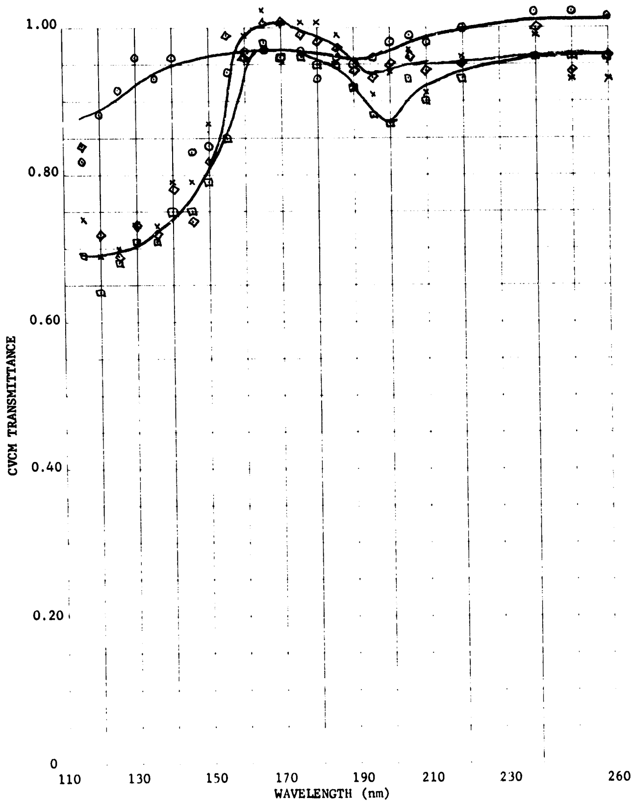
Figure 15. CVCM Transmittance Versus Wavelength, Source Material EA-9309, JPL#140-VOD-3, CVCM Thickness In Angstroms \circ 25, \square 51, \diamond 71, \times 70.
