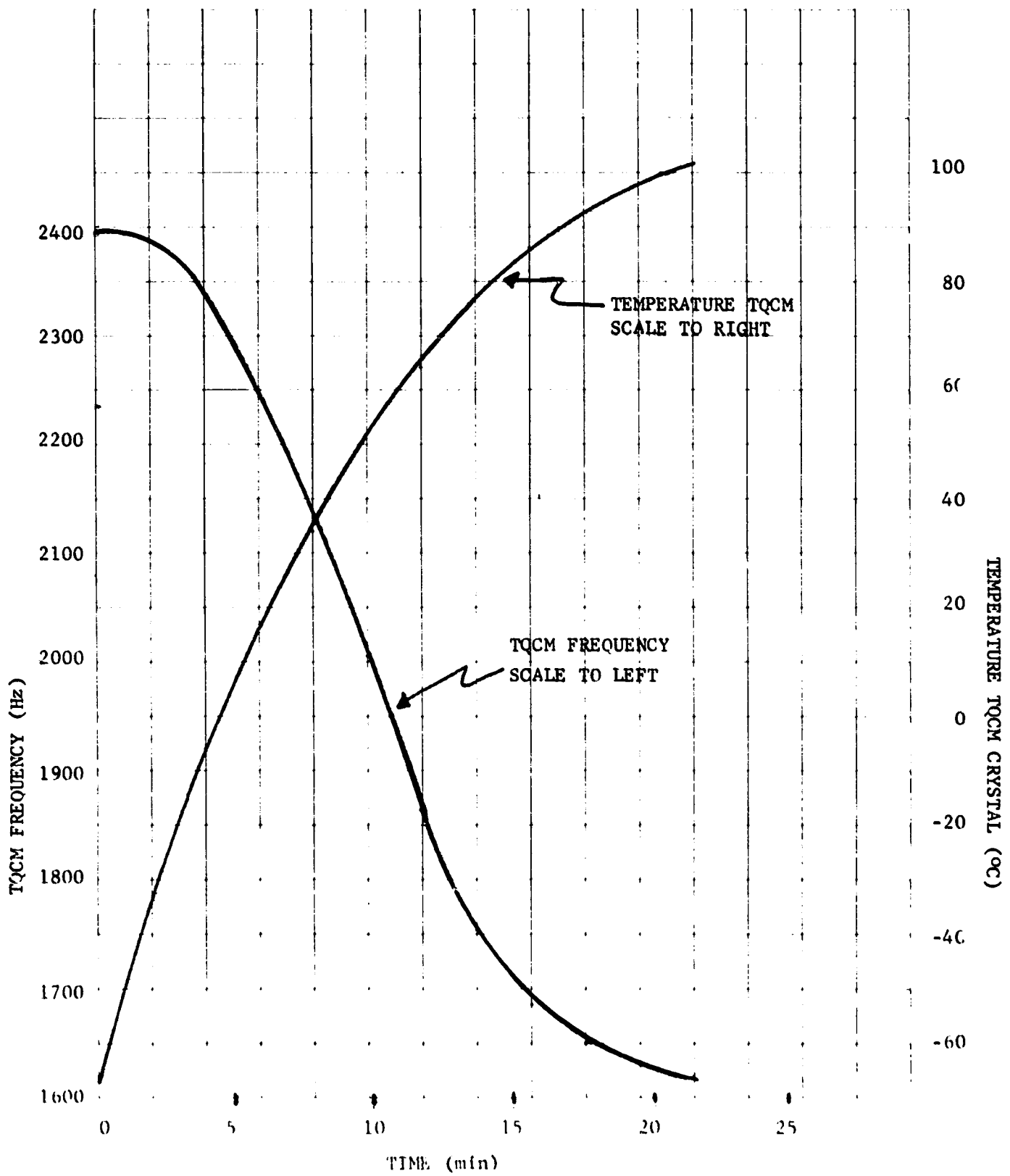
Figure 05. Reemission of CVM From Ablebond 36-2 Versus Time. Temperature Of TQCM Crystal Versus Time.
