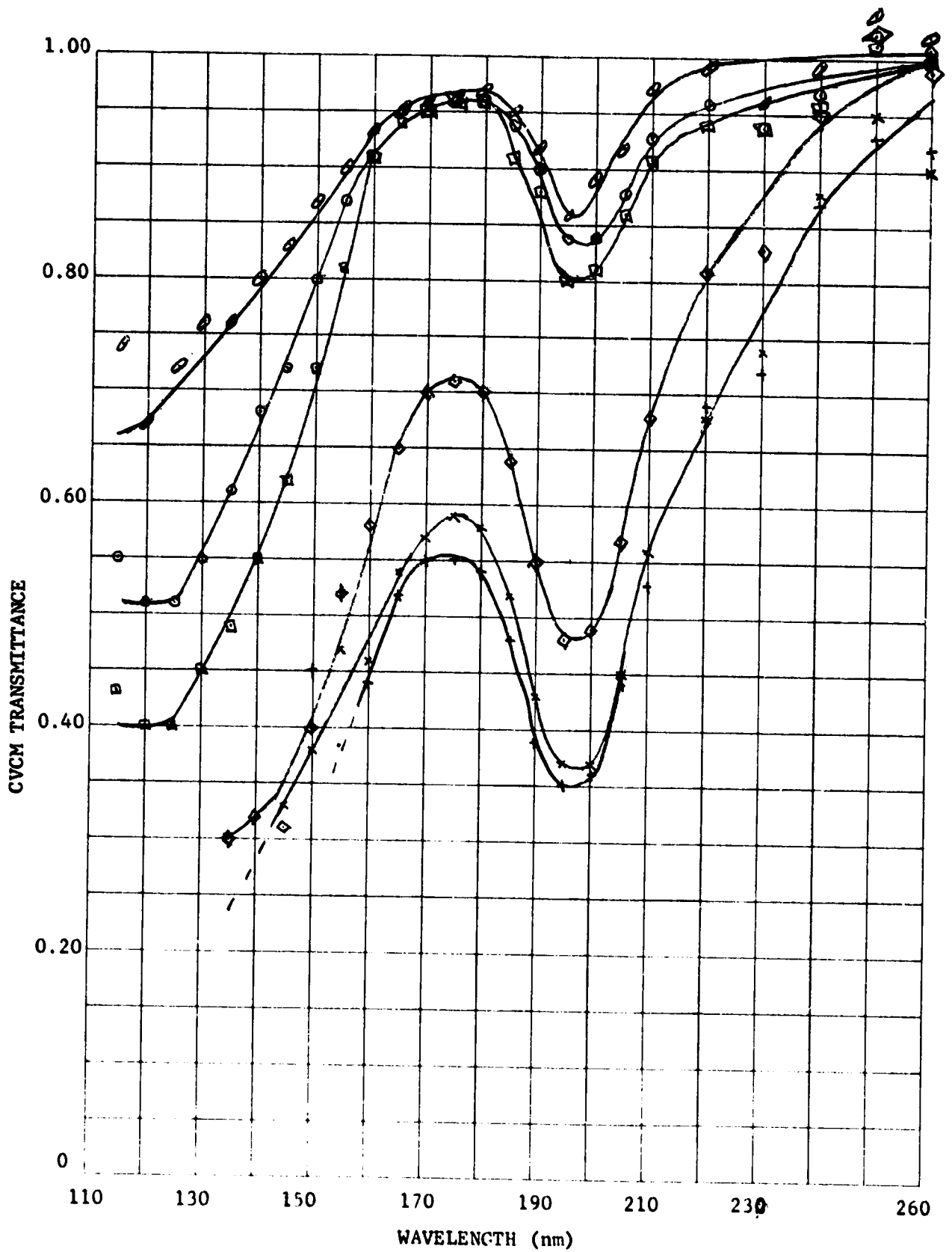
Figure 55. CVCM Transmittance Versus Wavelength, Source Material Solithane 113/C113-300, JPL#12A-VOD-2, CVCM Thickness In Angstroms ○ 69, □ 132, ◇ 191, × 607, + 936, + 1131.
