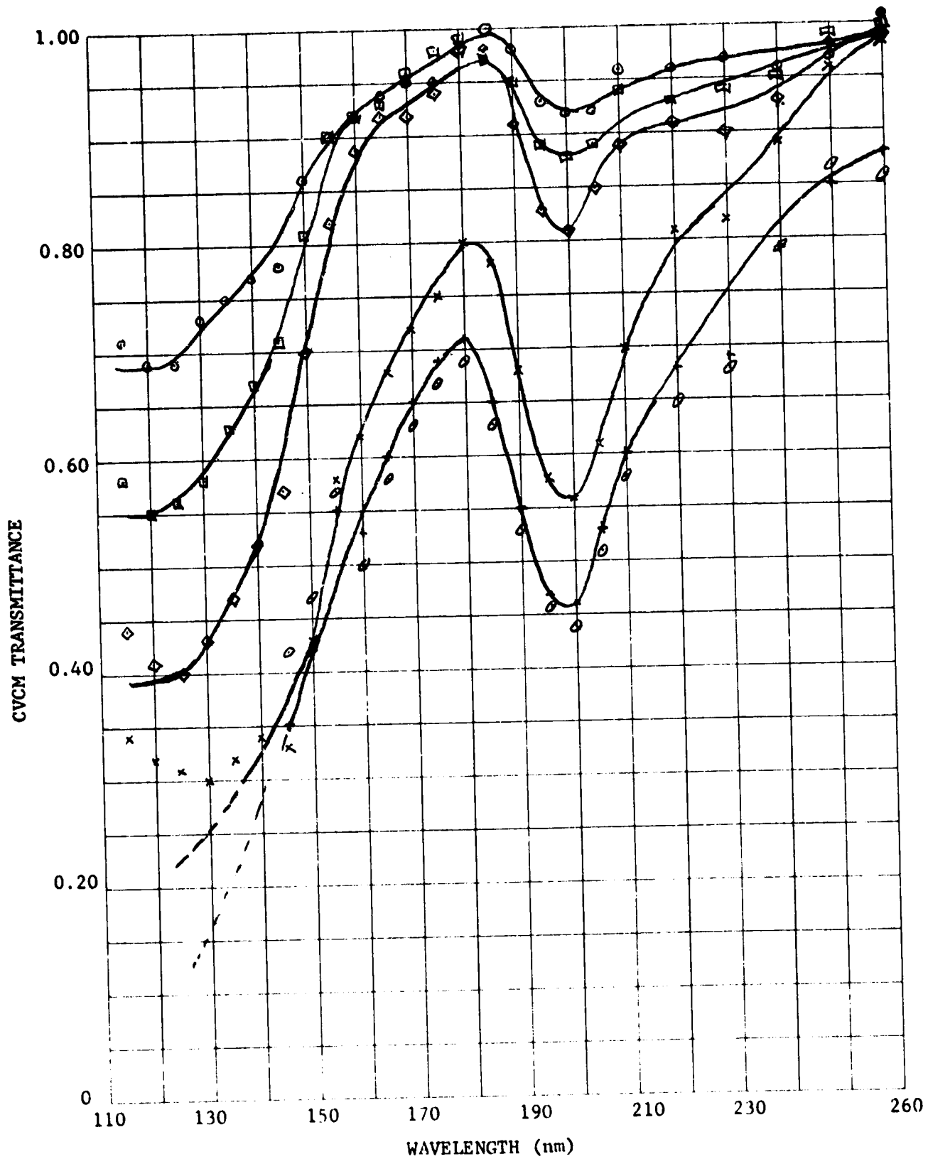
Figure 63. CVCM Transmittance Versus Wavelength, Source Material RT/Duroid, JPL# 91-VOD-I, CVCM Thickness In Angstroms \circ 40, \square 59, \diamond 87, \times 212, + 325, \bullet 382.
