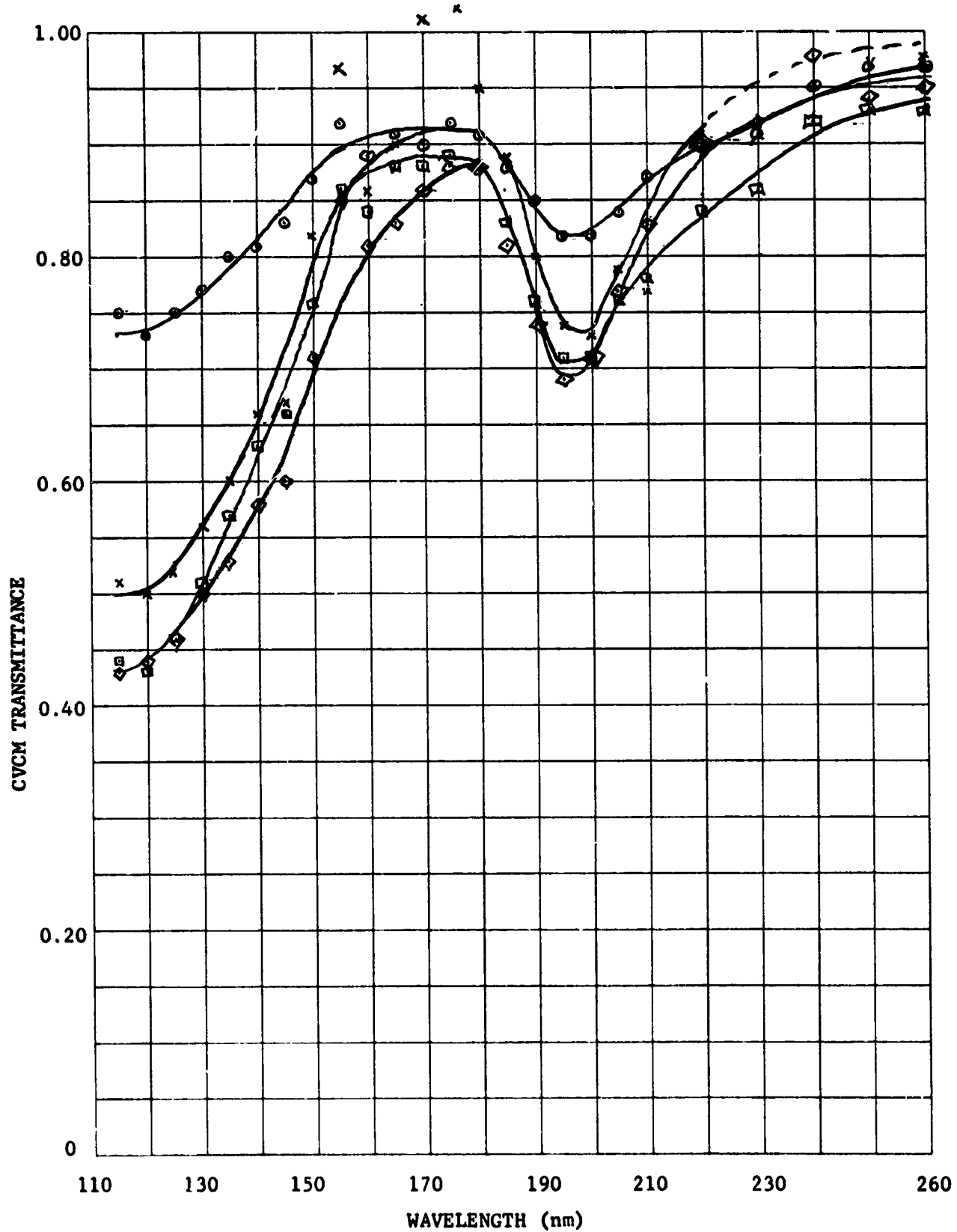
Figure 25. CVCN Transmittance Versus Wavelength, Source Material Chemglaze Z-306, JPL#129B-VOD-1, CVCN Thickness In Angstroms \odot 67, \square 158, \diamond 181, \times 190.
