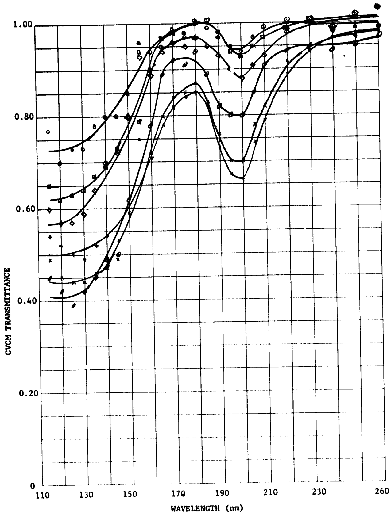
Figure 53. CVCM Transmittance Versus Wavelength, Source Material GY70/Fiberite 934/Spotbound 3M-415 Double Side Tape, JPL#53B-VOD-1, CVCM Thickness In Angstroms \circ 61, \square 88, \diamond 103, \oslash 235, \times 322, + 370.
