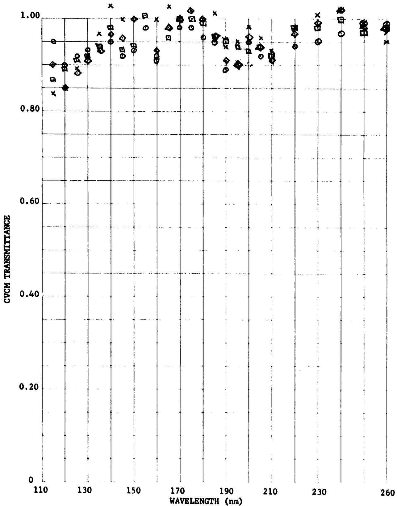
Figure 41. CVCN Transmittance Versus Wavelength, Source Material CAT-A-LAC 463-3-8/463-6-5, JPL#115B-VOD-1, CVCN Thickness In Angstroms \circ 16, \square 10, \diamond 14, \times 12.
