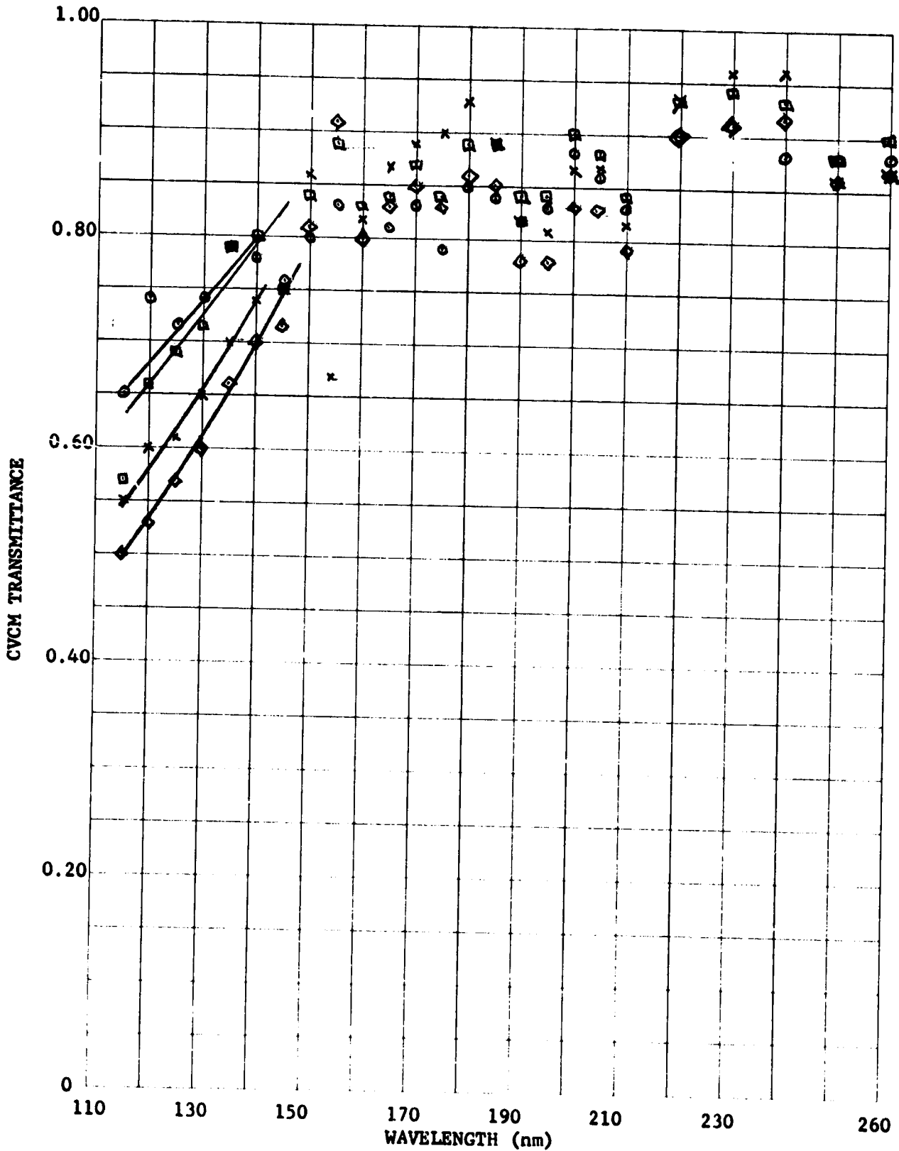
Figure 37. CVCM Transmittance Versus Wavelength, Source Material CAT-A-IAC 463-6-8, JPL#127-VOD-1, CVCM Thickness In Angstroms @ 28, □ 35, ◇ 45, × 50.
