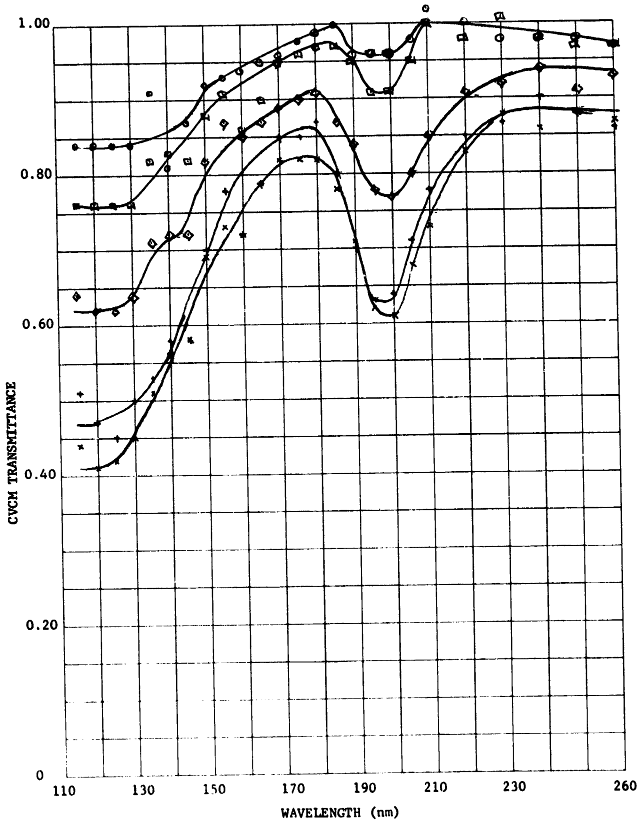
Figure 47. CVCN Transmittance Versus Wavelength, Source Material 3M Nextel 401-C10, JPL#143-VOD-2, CVCN Thickness In Angstroms ○ 26, ◻ 42, ◊ 97, × 222, + 237.
