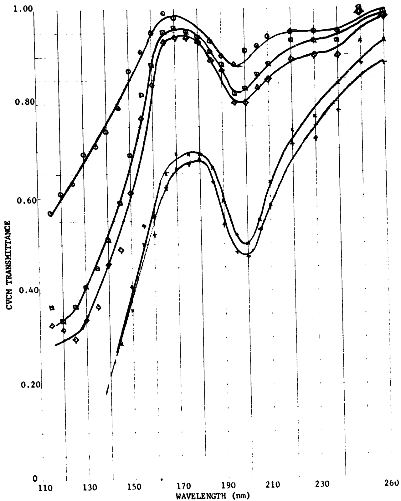
Figure 61. CVCM Transmittance Versus Wavelength, Source Material Lube-Lok 4306, JPL# 135-VOD-1, CVCM Thickness In Angstroms ○ 91, ◻ 164, ◊ 194, × 340, + 424.
