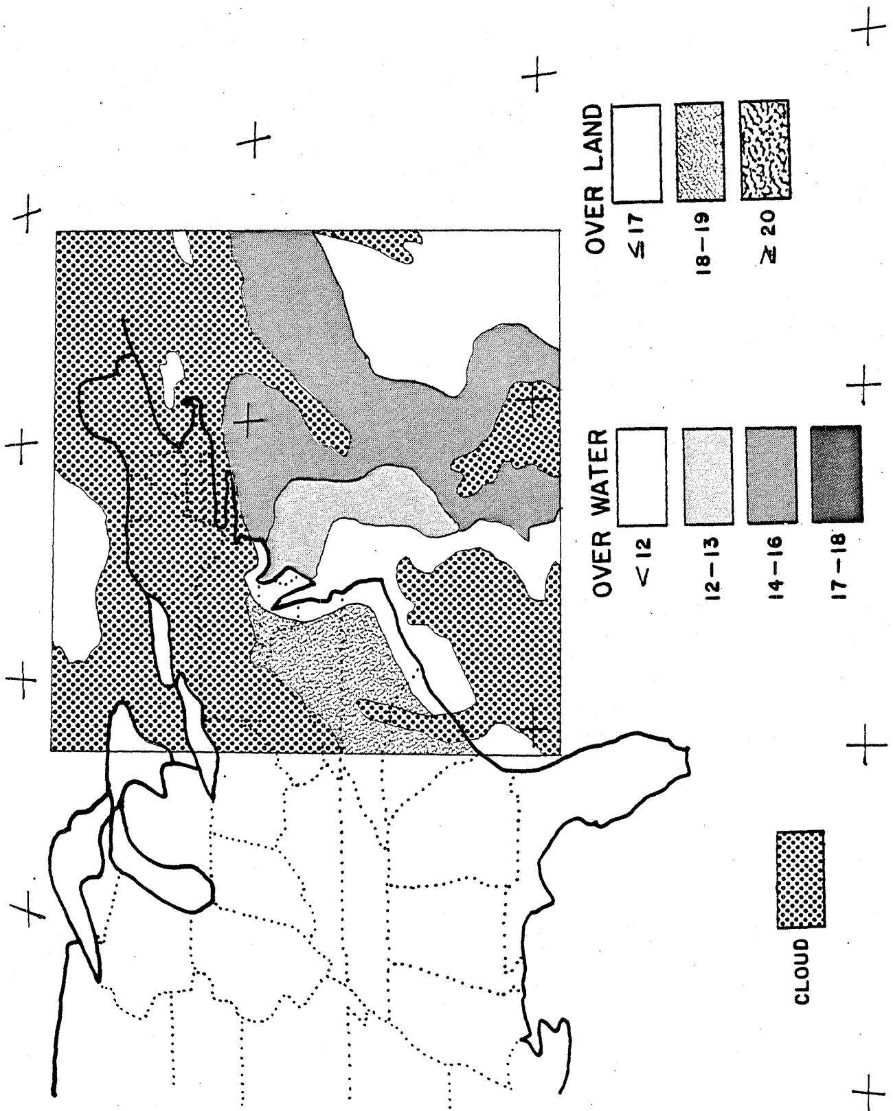
Figure 3-7 Map showing areal averages of digital brightness values for 11 August 1979.
