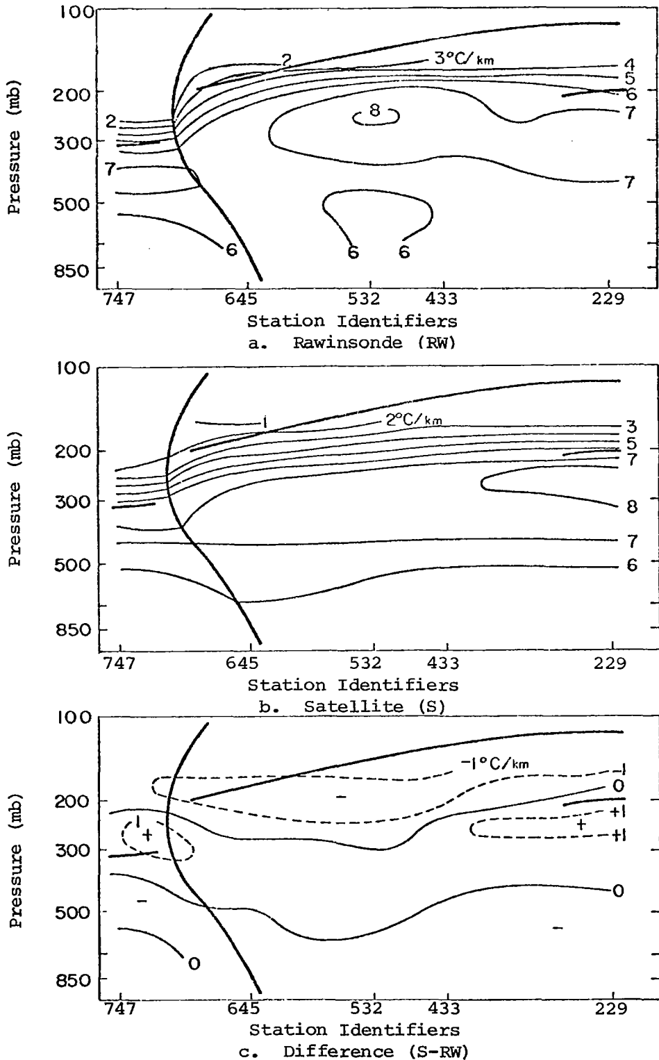
Fig. 35. Cross sections of vertical lapse rate of temperature and lapse rate difference ( ^{\circ}\text{C}/\text{km} ) for the central United States region on 25 August 1975 at 1700 GMT. (See Fig. 2 for path of cross sections.)
