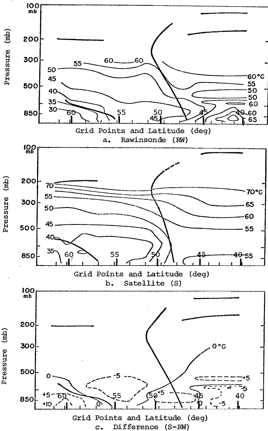
Fig. 45. Cross sections of equivalent potential temperature and equivalent potential temperature difference ( ^{\circ}\text{C} ) for the Canada region on 25 August 1975 at 1700 GMT. (See Fig. 3 for path of cross sections.)
