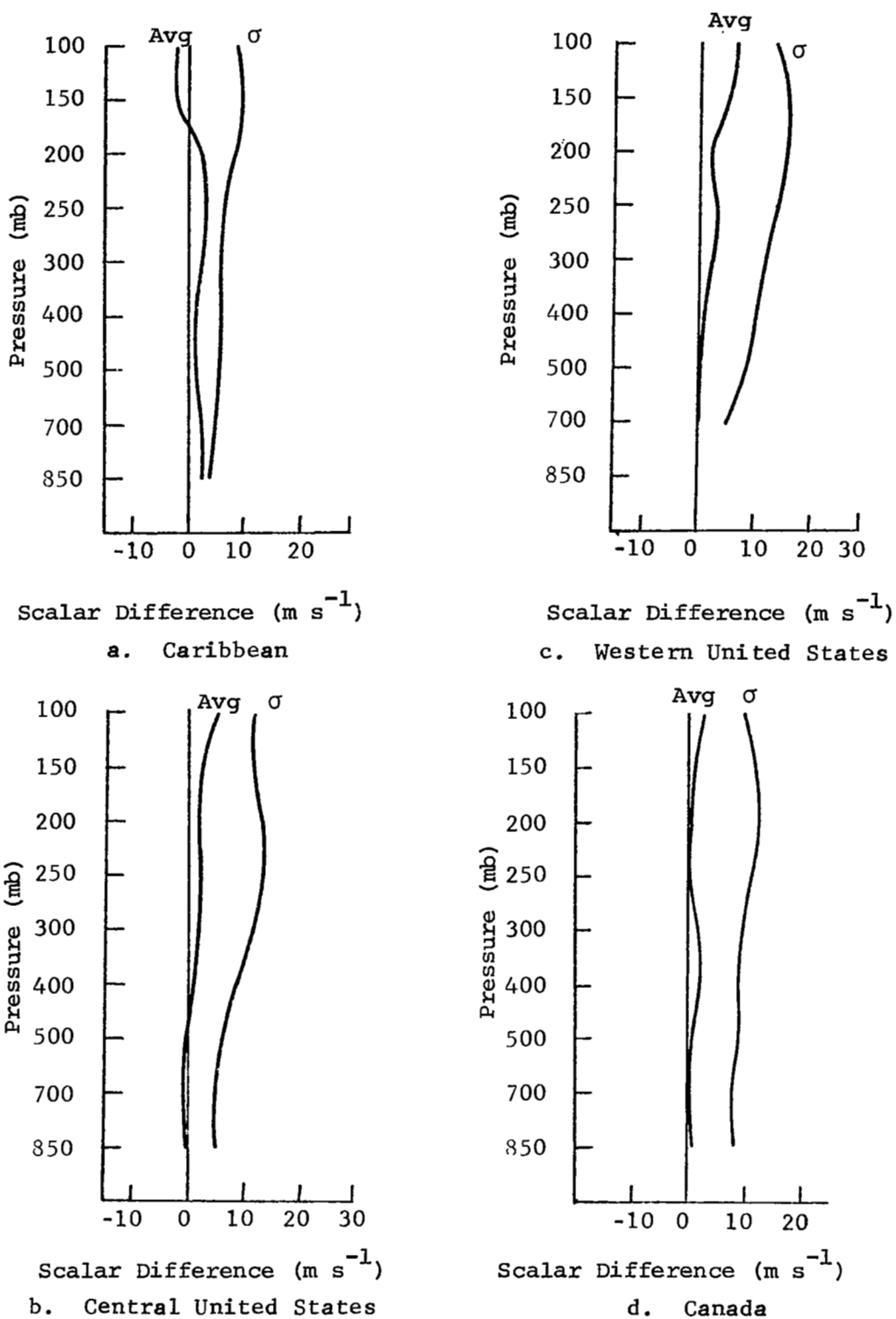
Fig. 13. Profiles of the average difference and standard deviation of the differences between satellite and rawinsonde geostrophic wind speeds (satellite values minus rawinsonde values) for four regions.
