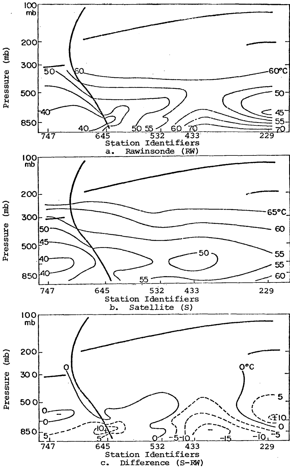
Fig. 44. Cross sections of equivalent potential temperature and equivalent potential temperature difference ( ^{\circ}\text{C} ) for the central United States region on 25 August 1975 at 1700 GMT. (See Fig. 2 for path of cross sections.)
