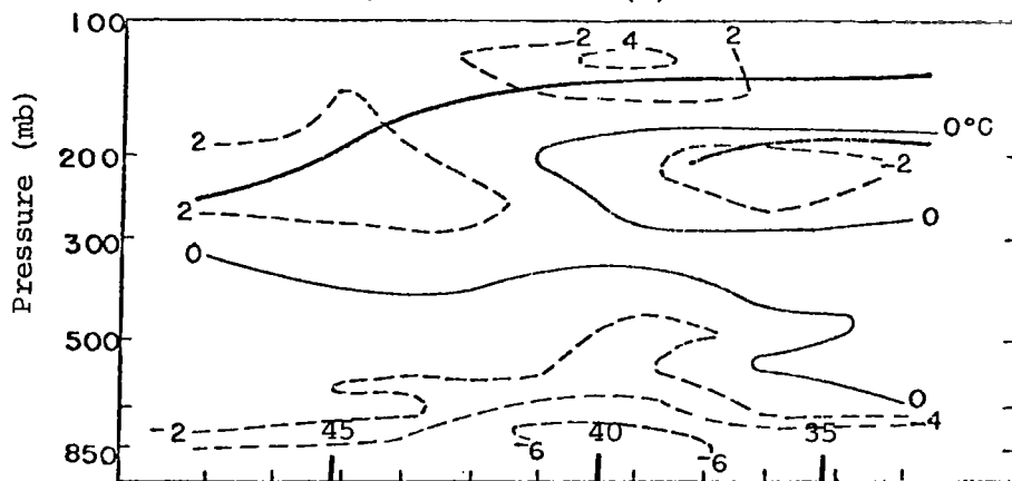
Fig. 33. Cross sections of temperature and temperature difference ( ^{\circ}\text{C} ) for the western United States region on 3 September 1975 at 0730 GMT. (See Fig. 4 for path of cross sections.)
