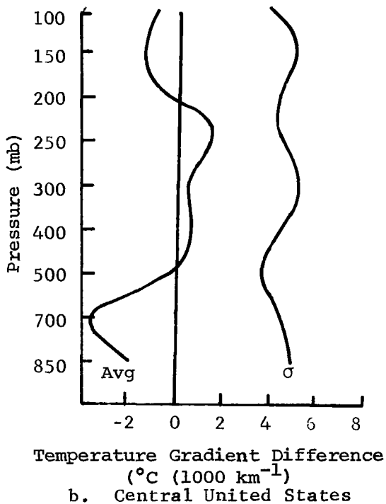
Fig. 7. Profiles of the average difference and standard deviation of the differences between satellite and rawinsonde horizontal temperature gradients (satellite values minus rawinsonde values) for four regions.
