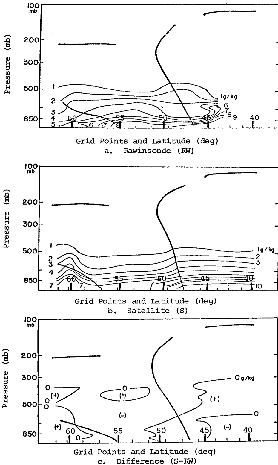
Fig. 43. Cross sections of mixing ratio and mixing ratio difference (g/kg) for the Canada region on 25 August 1975 at 1700 GMT. (See Fig. 3 for path of cross sections.)
