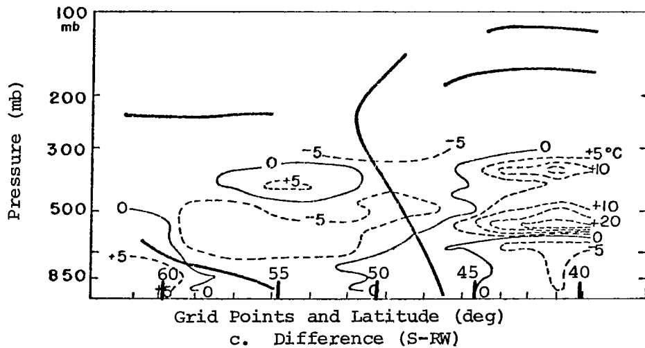
Fig. 42. Cross sections of dew-point temperature and dew point difference ( ^{\circ}\text{C} ) for the Canada region on 25 August 1975 at 1700 GMT. (See Fig. 3 for path of cross sections.)
