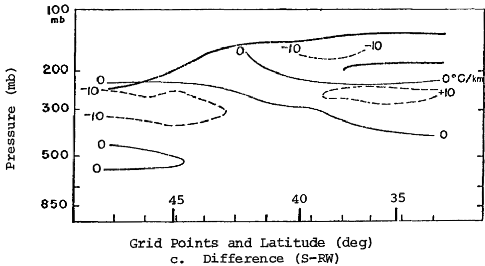
Fig. 36. Cross sections of vertical lapse rate of temperature and lapse rate difference ( ^{\circ}\text{C}/\text{km} ) for the western United States region on 3 September 1975 at 0730 GMT.
