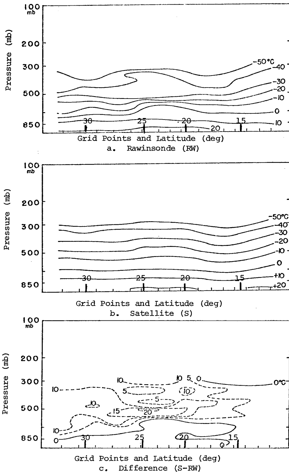
Fig. 40. Cross sections of dew-point temperature and dew point difference ( ^{\circ}\text{C} ) for the Caribbean region on 25 August 1975 at 1700 GMT. (See Fig. 1 for path of cross sections).
