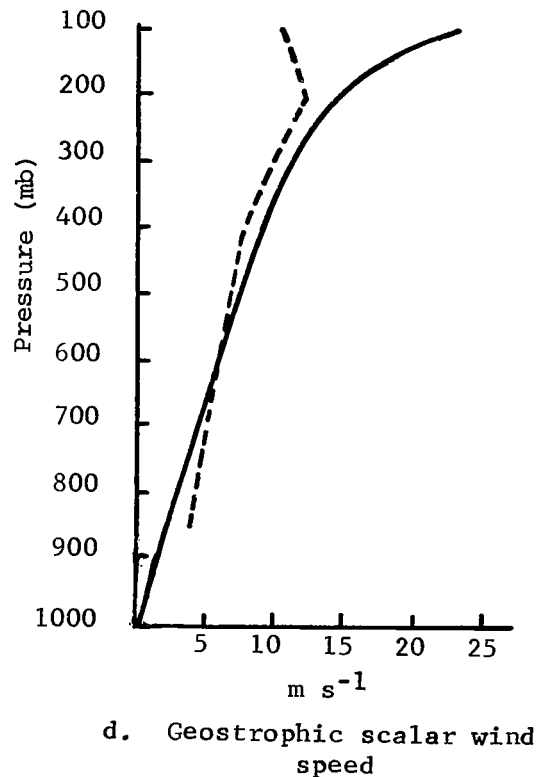
Fig. 15. Vertical profiles of standard deviations of differences between Nimbus satellite data and rawinsonde data. Solid lines are Nimbus-5 (Smith and Woolf, 1974); dashed lines are Nimbus-6 (this study). The dotted line on part (a) is from Waters et al. (1975).
