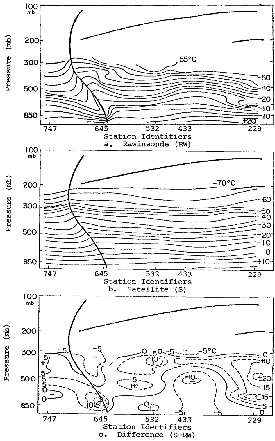
Fig. 41. Cross sections of dew-point temperature and dew point difference ( ^{\circ}\text{C} ) for the central United States region on 25 August 1975 at 1700 GMT. (See Fig. 2 for path of cross sections.)
