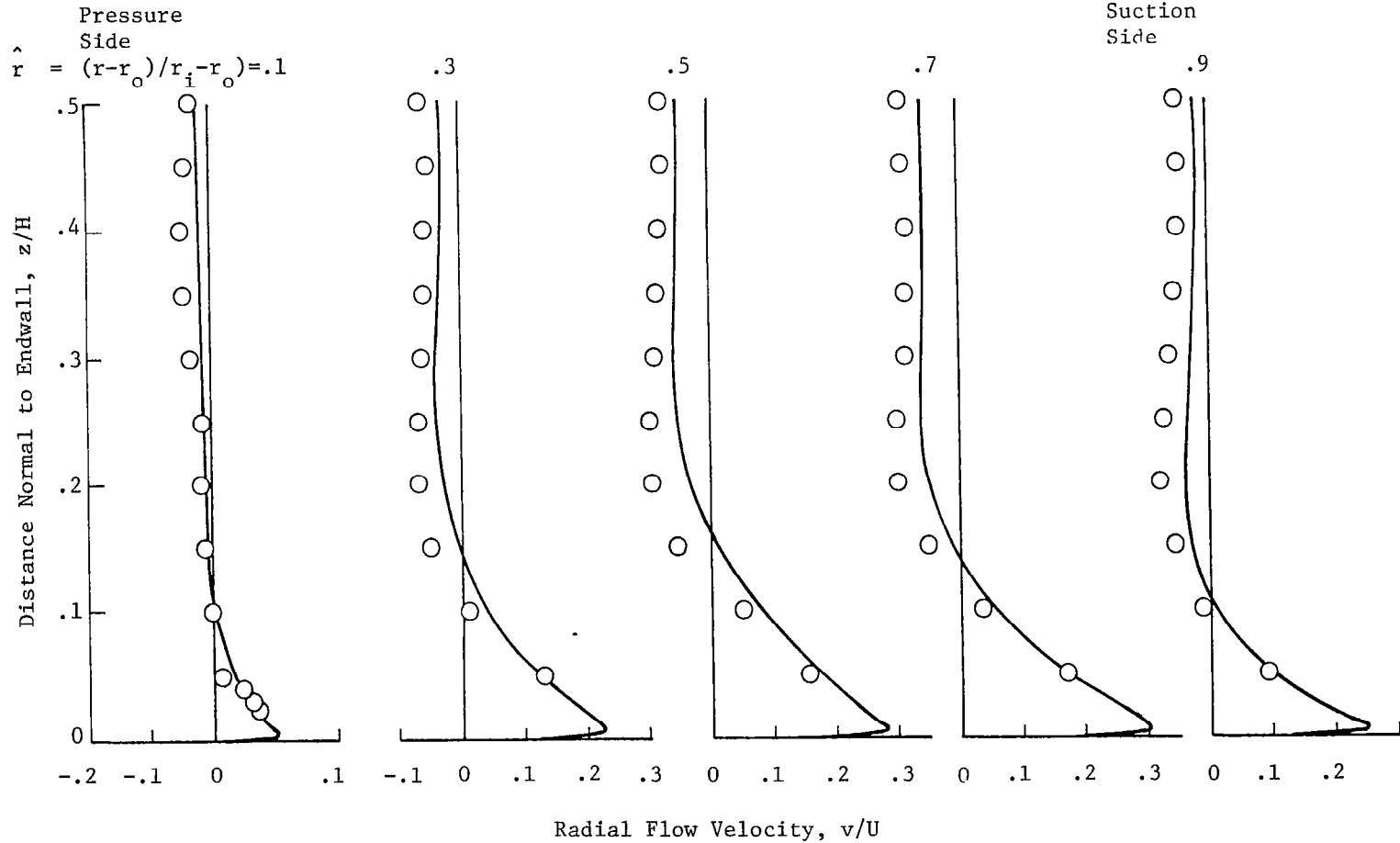
Fig.11b - Radial Flow Velocity Profiles After 30 Degrees of Turning in a Circular Arc Duct of Square Crosssection, R/H=2.3 , Re=40000 , k=26370 .
