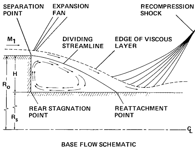
Figure 1.— Separation and recompression regions of axisymmetric flow over a cylindrical step base.
