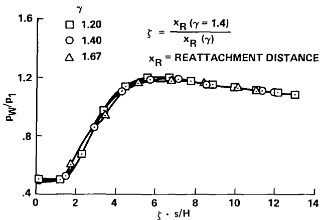
(a) M_1 = 2.09 , R_s/R_0 = 1/2 , and [R] = 75 .
