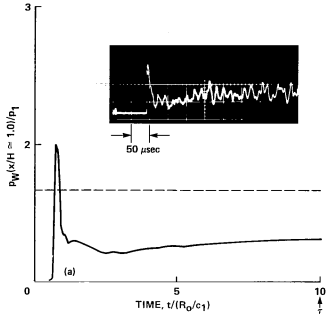
(a) \gamma = 1.2 .
