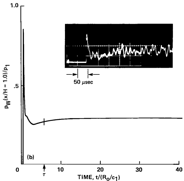
(b) \gamma = 1.4 .
