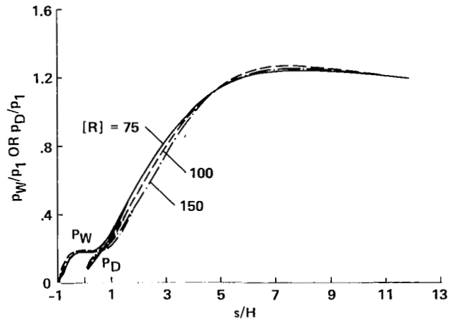
(c) The effect of [R] on pressure distributions at higher Mach number. M_1 = 4.0, \gamma = 1.4, R_s/R_o \cong 1/2 .
