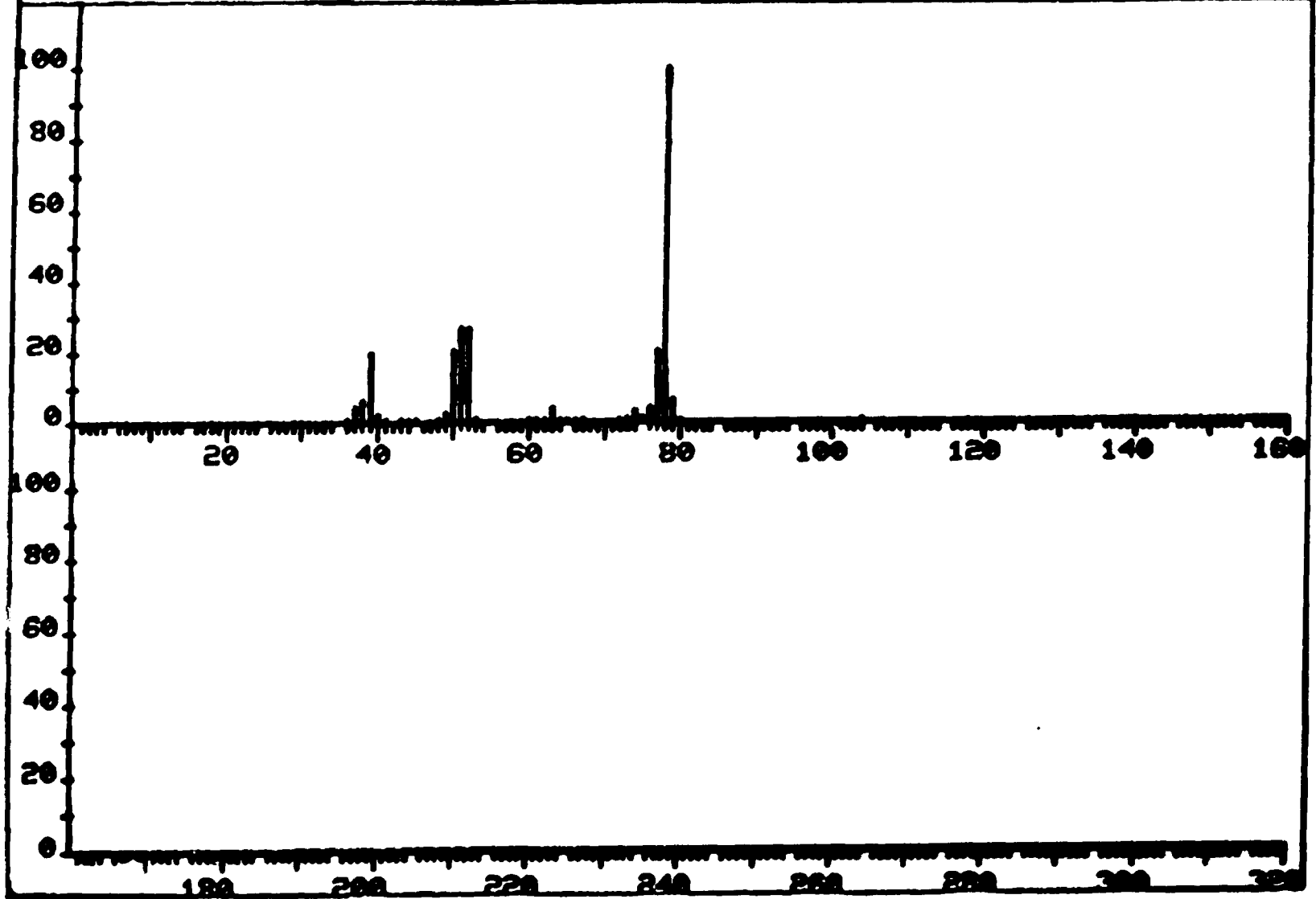
Figure A-11. Mass spectrum of benzene shown in Tables I and II.
