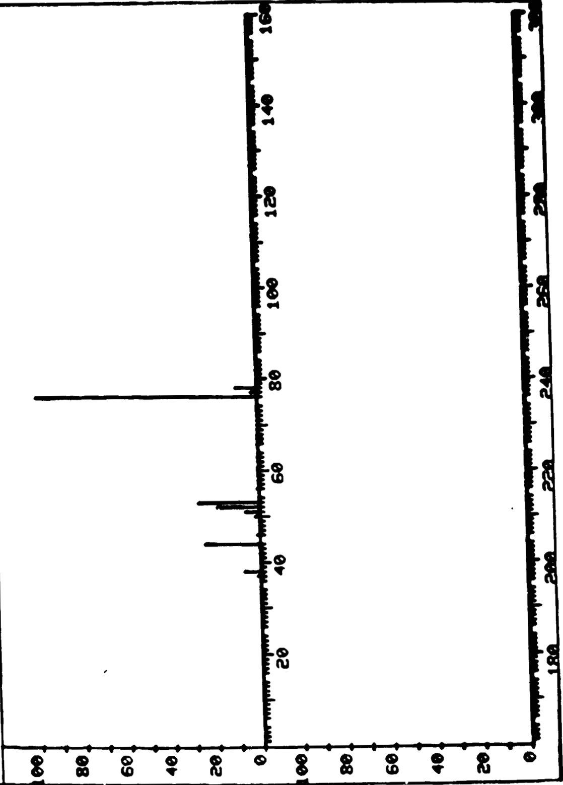
Figure A-7. Mass spectrum of CS 2 reported in Tables I and II.
