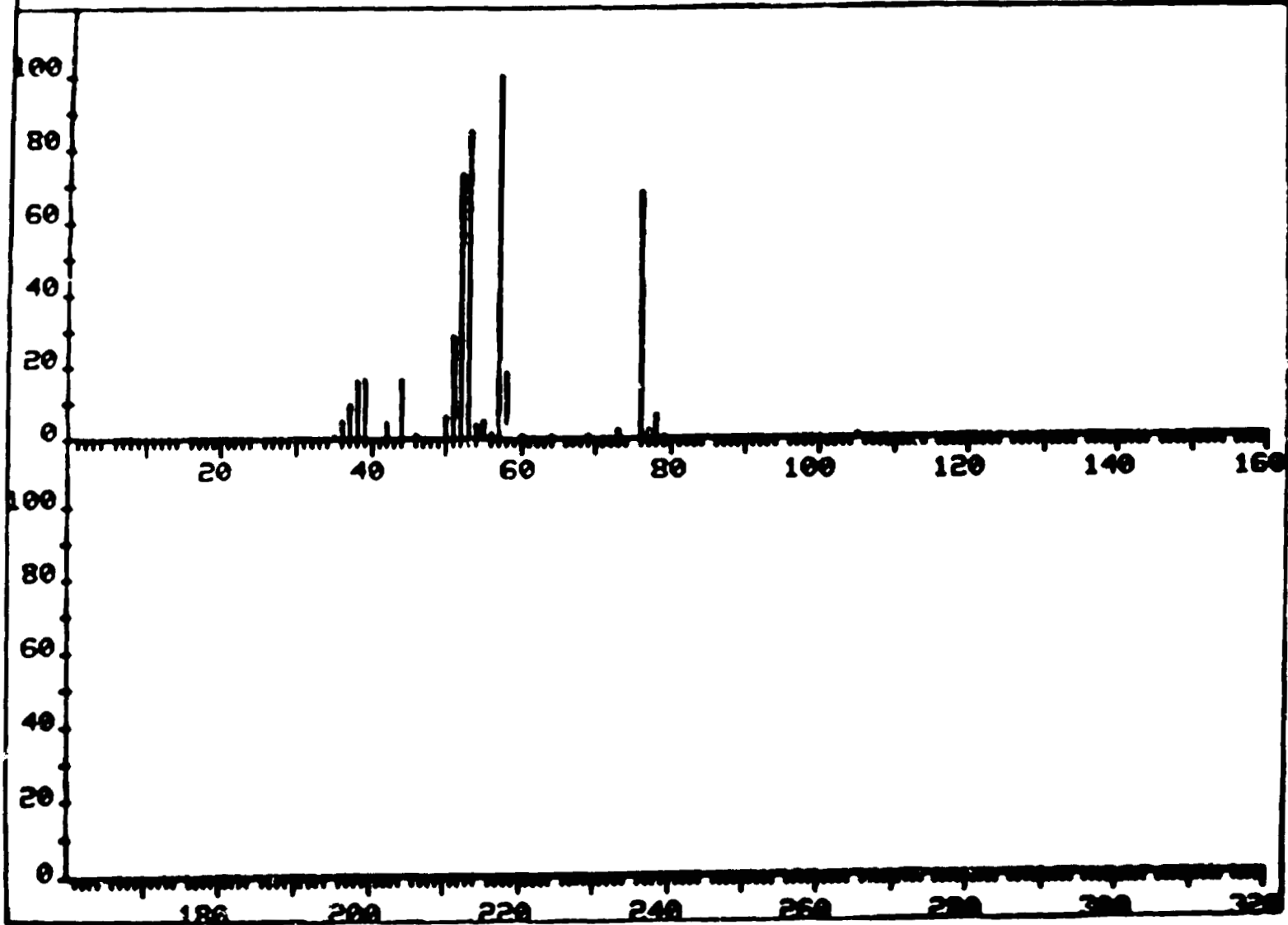
Figure A-8. Mass spectrum of propenenitrile reported in Tables I and II (note the presence of C 3 H 3 N and propene-3-ol).
