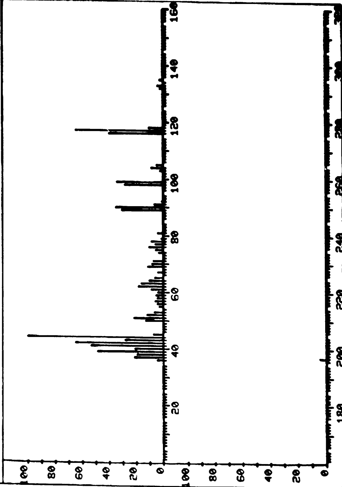
Figure A-27. Mass spectrum of compound with 29.3 minute retention time in Table VI (note presence of N-methyl-2-pyrrolidone spectrum due to incomplete chromatographic resolution).
