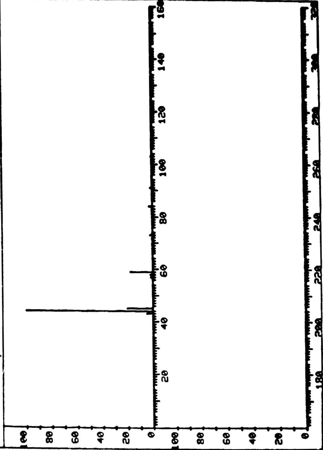
Figure A-20. Mass spectrum of compound with retention time of 25.61 minutes in Table I.
