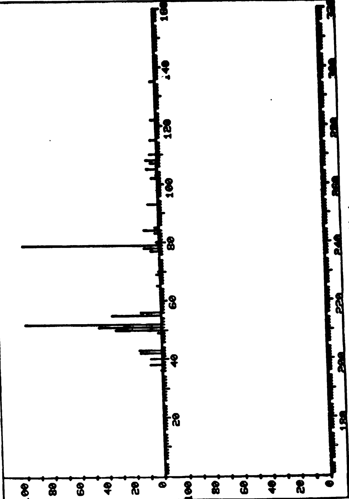
Figure A-14. Mass spectrum of pyridine shown in Table I.
