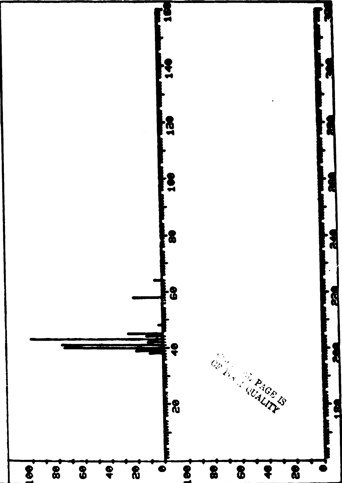
Figure A-21. Mass spectrum of isobutane/butane/propanol shown in Table II.
