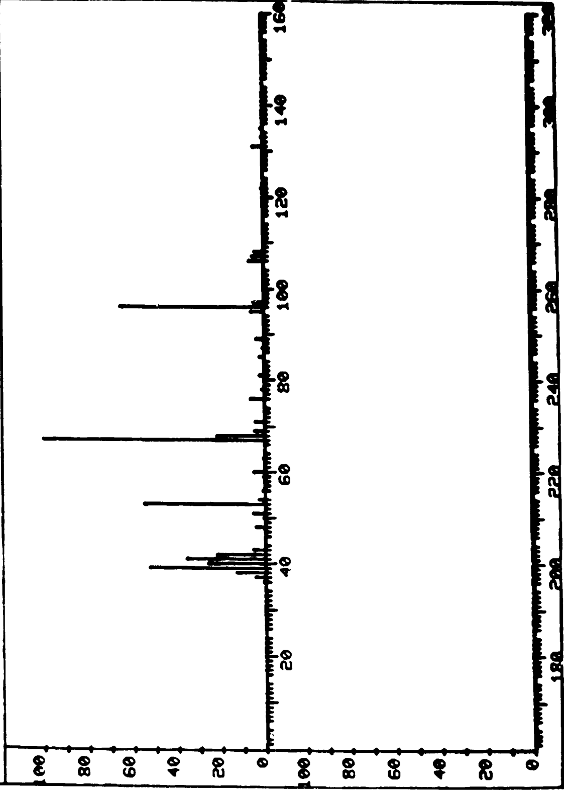
Figure A-18. Mass spectrum of compound with retention time of 22.36 minutes in Table I with probable molecular weight of 96.
