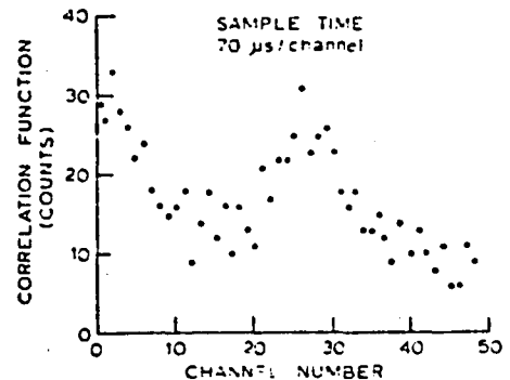
Figure 5. Correlation function obtained when two laser beams are used.
