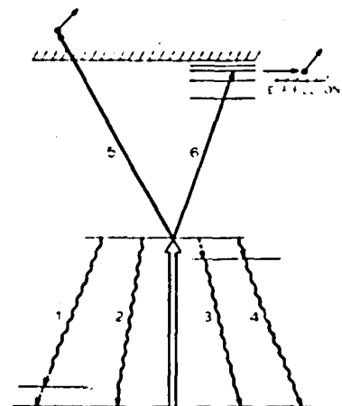
Fig. 1. Different schemes for detecting single atoms with lasers. After an atom is excited by a laser (the large arrow), it may be detected by observing its resonance fluorescence (path 2) or fluorescence at a different frequency (paths 1 and 3), by the method of SONRES (path 4), by photoionization (path 5), and by field ionization (path 6). The nonradiative thermal energy for paths 1 and 3 may also be detected by photoacoustic spectroscopy.
