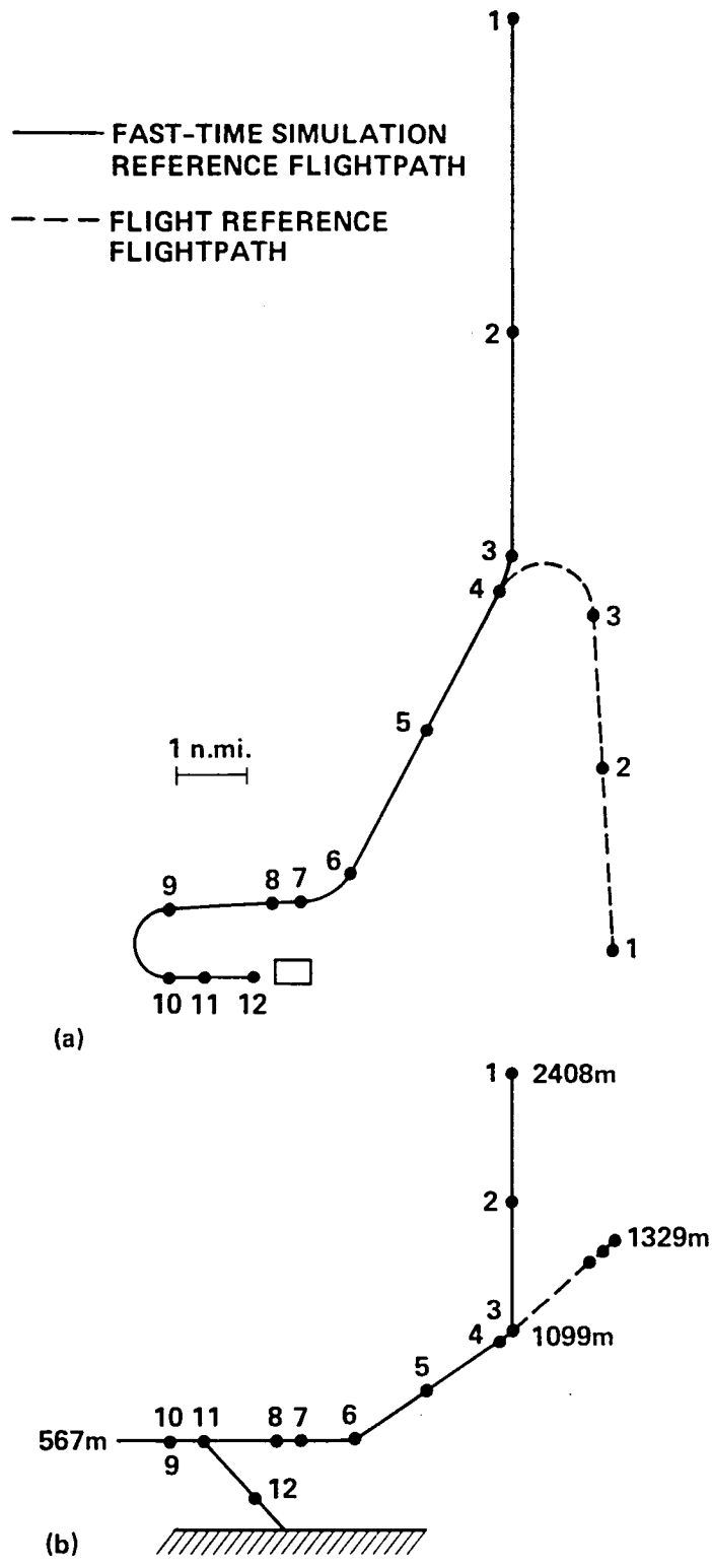
Figure 3.- Reference flightpath.
