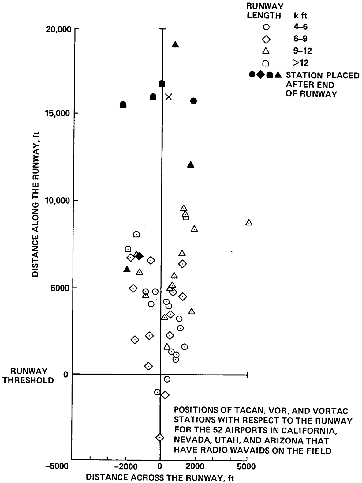
Figure 13.- NAVAID positions.
