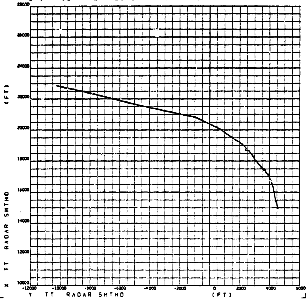
Figure 6-11 X-Y Plot of VOR Capture (Radar)
