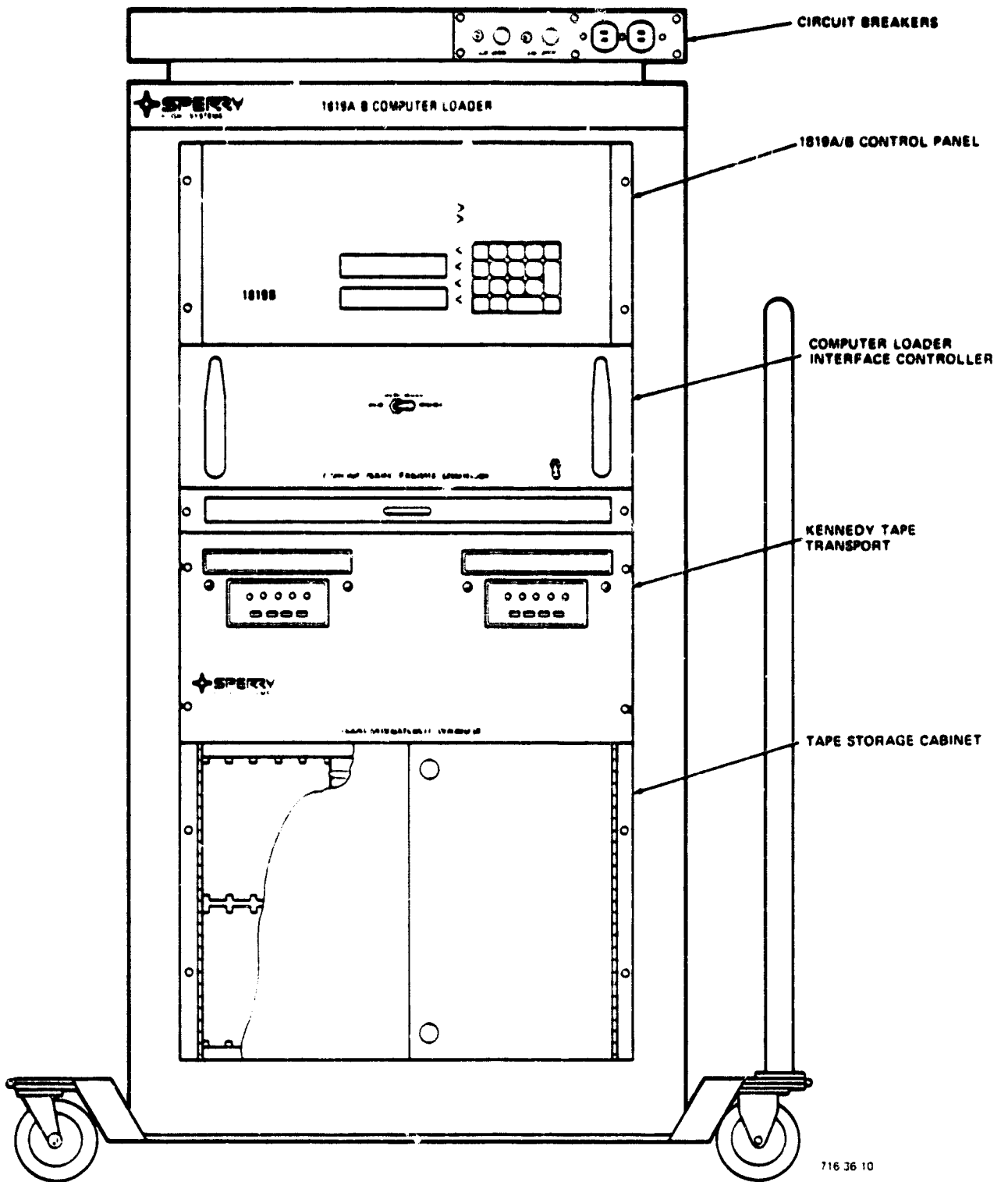
Figure 4-29 The Computer Loader
