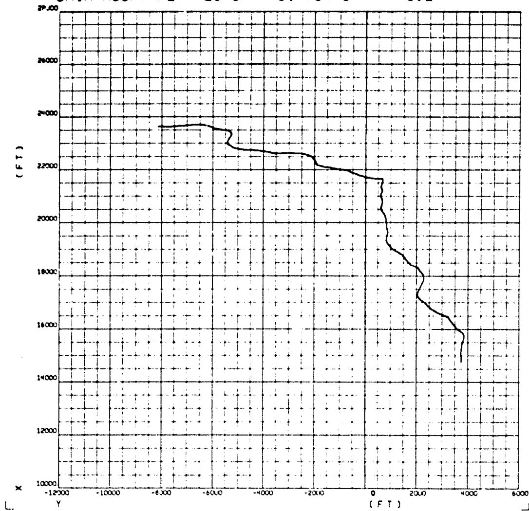
Figure 6-10 X-Y Plot of VOR Capture (Navigation)
