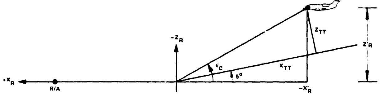
(B) ELEVATION VIEW
