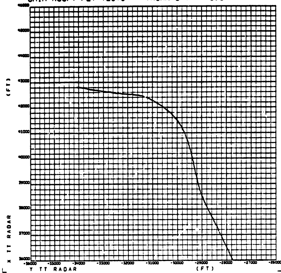
Figure 6-8 X-Y Plot of TACAN Capture (Radar)
