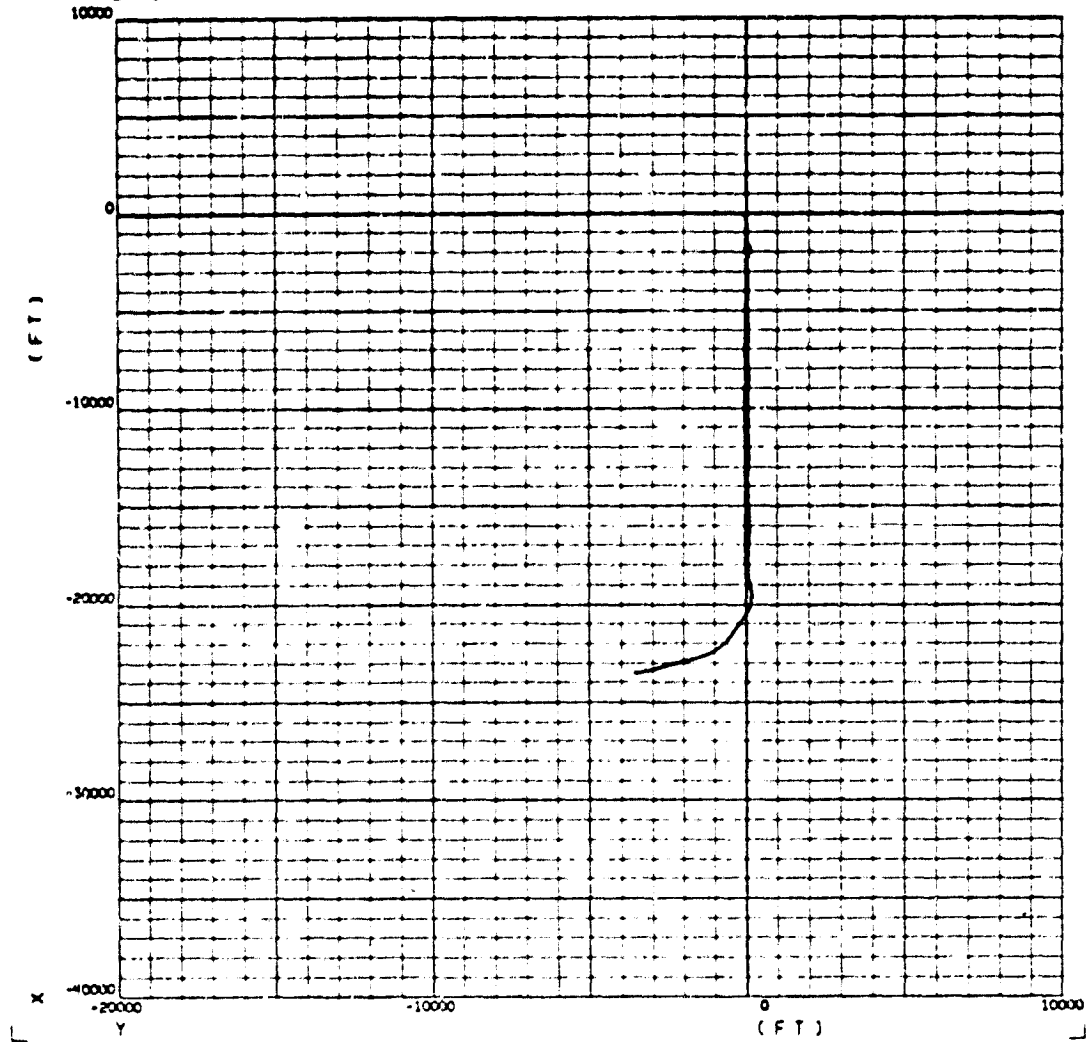
Figure 6-21 X-Y Plot of Straight-In Land, -12.5° Glideslope
