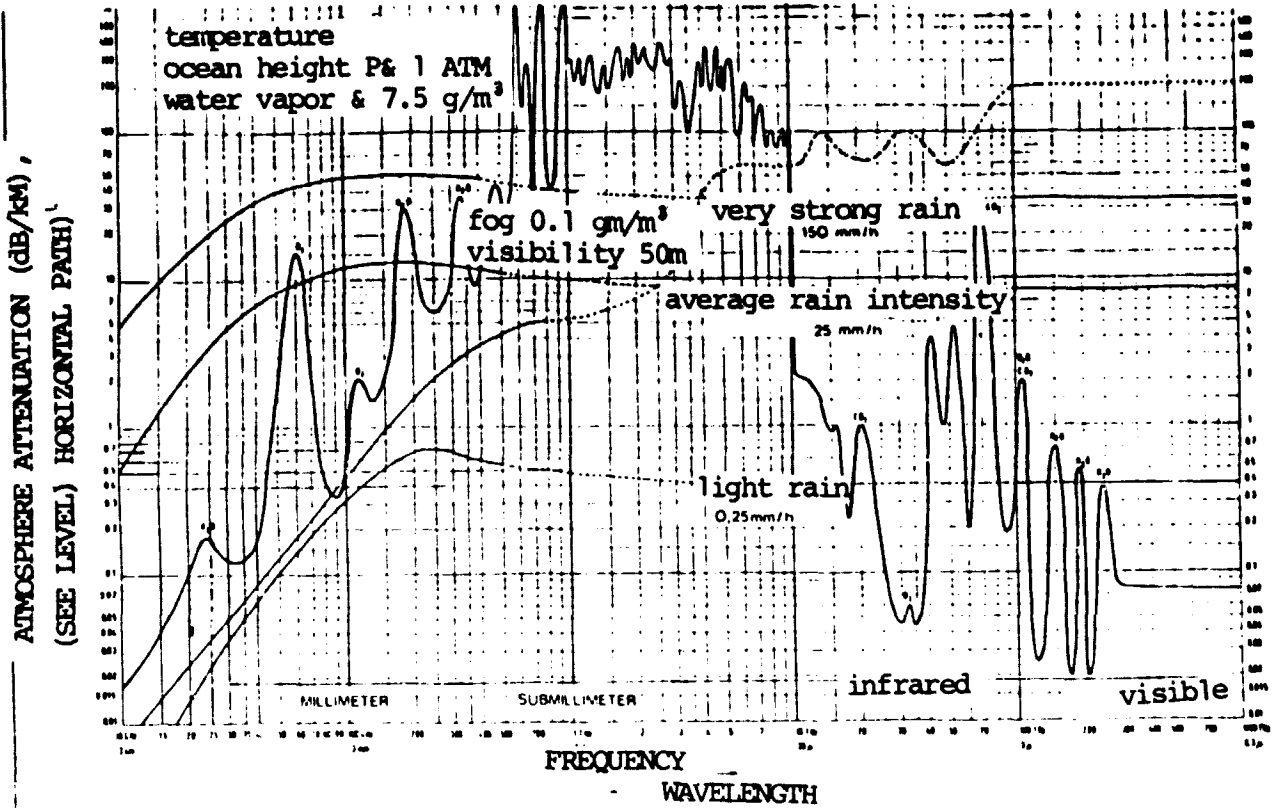
Figure 1. Damping by atmosphere gases, rain and fog.
