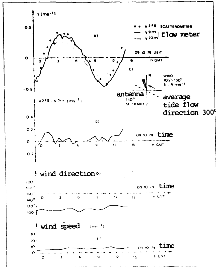
Figure 4. Measurement result of the two-frequency scatterometer.
