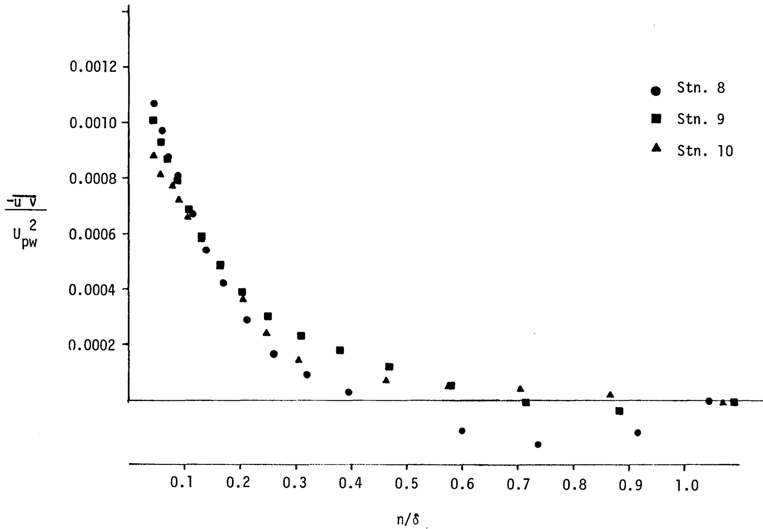
Fig. 41. Partial collapse of shear-stress profiles in curved region for second experiment
