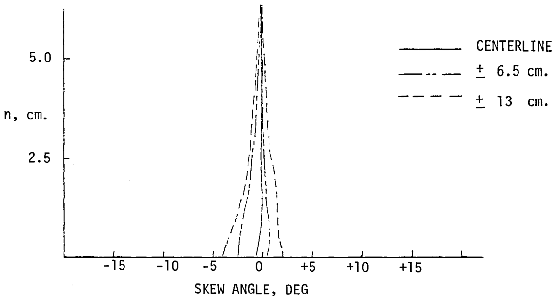
Fig. A-11. Skew-angle profiles for Station 9 (in recovery region), with fences
