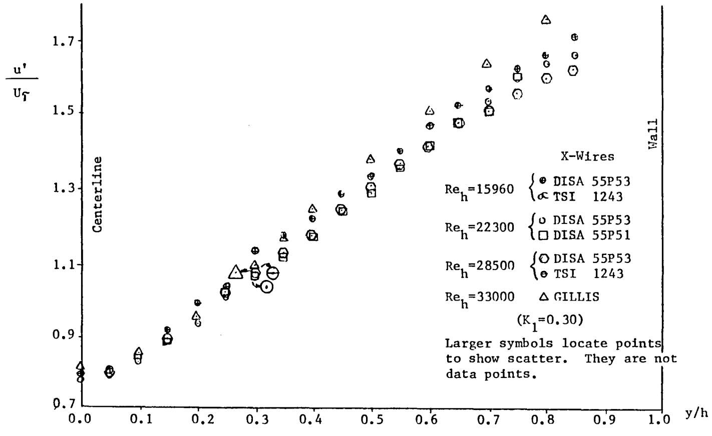
Fig. D-4. Plot of u'/u_T measured in channel
