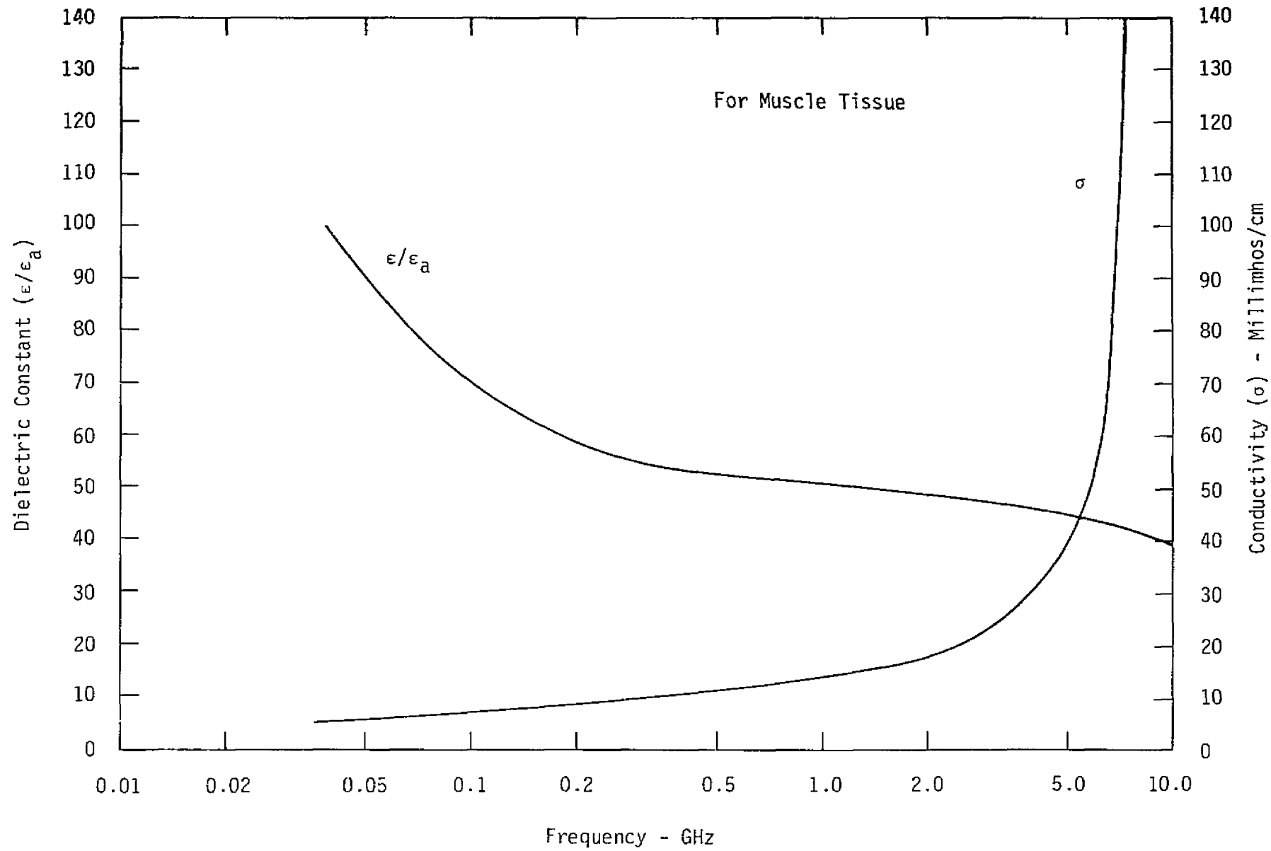
FIGURE 5-2 VARIATION OF DIELECTRIC CONSTANT AND ELECTRICAL CONDUCTIVITY WITH FREQUENCY FOR MUSCLE TISSUE
