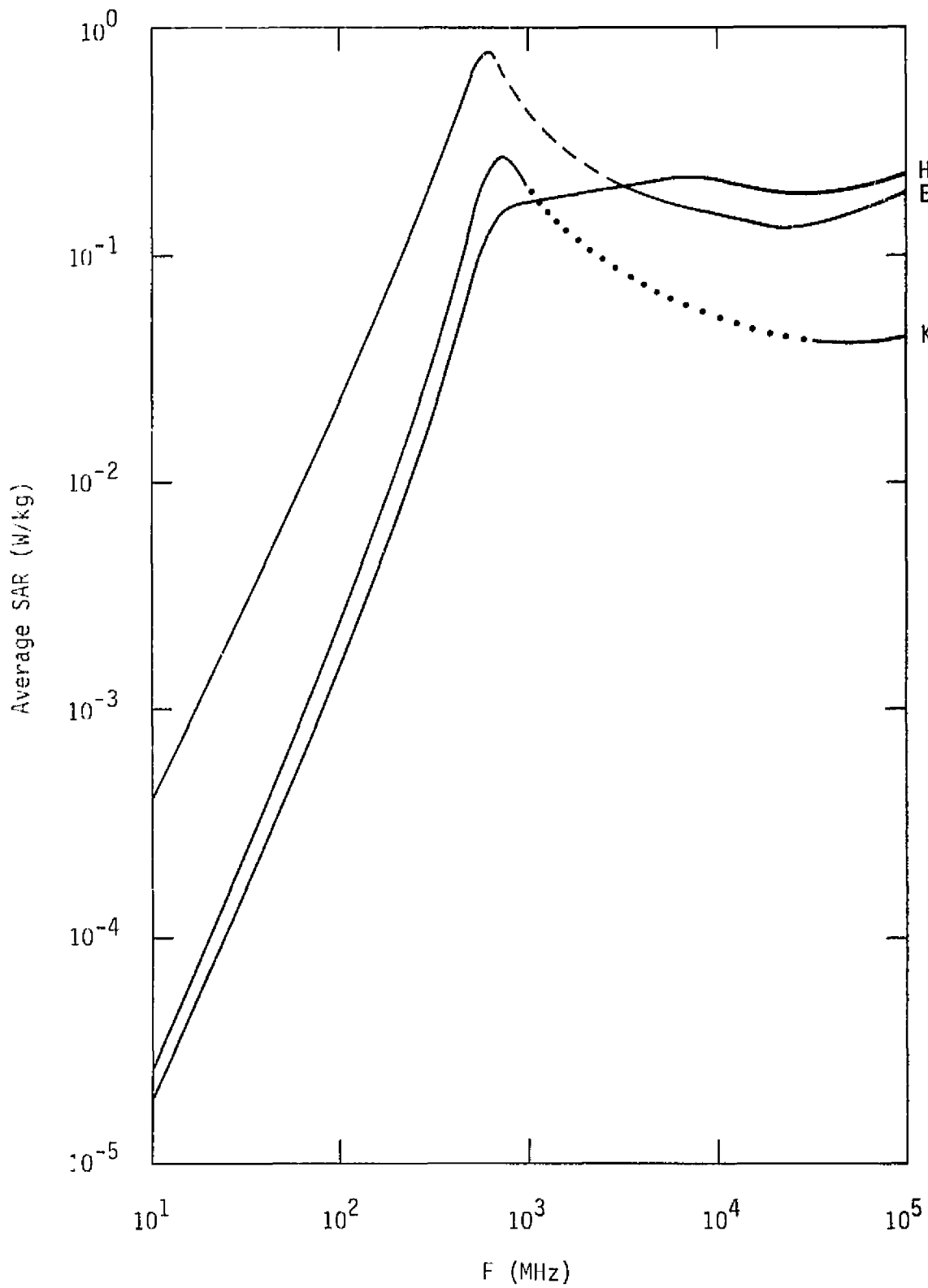
FIGURE 5-6 MEAN SAR FOR PROLATE-SPHEROIDAL MODEL OF "MEDIUM" RAT EXPOSED TO 1 \text{ mW/cm}^2 OF RFR
