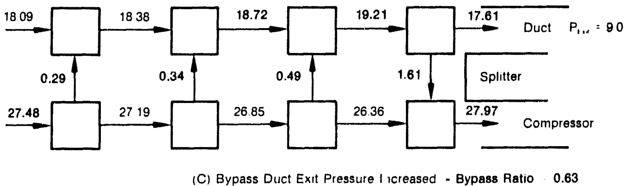
Figure 32. Physical Flows through Fan as Bypass Duct Exit Pressure is Changed (F100 Remote Splitter)
