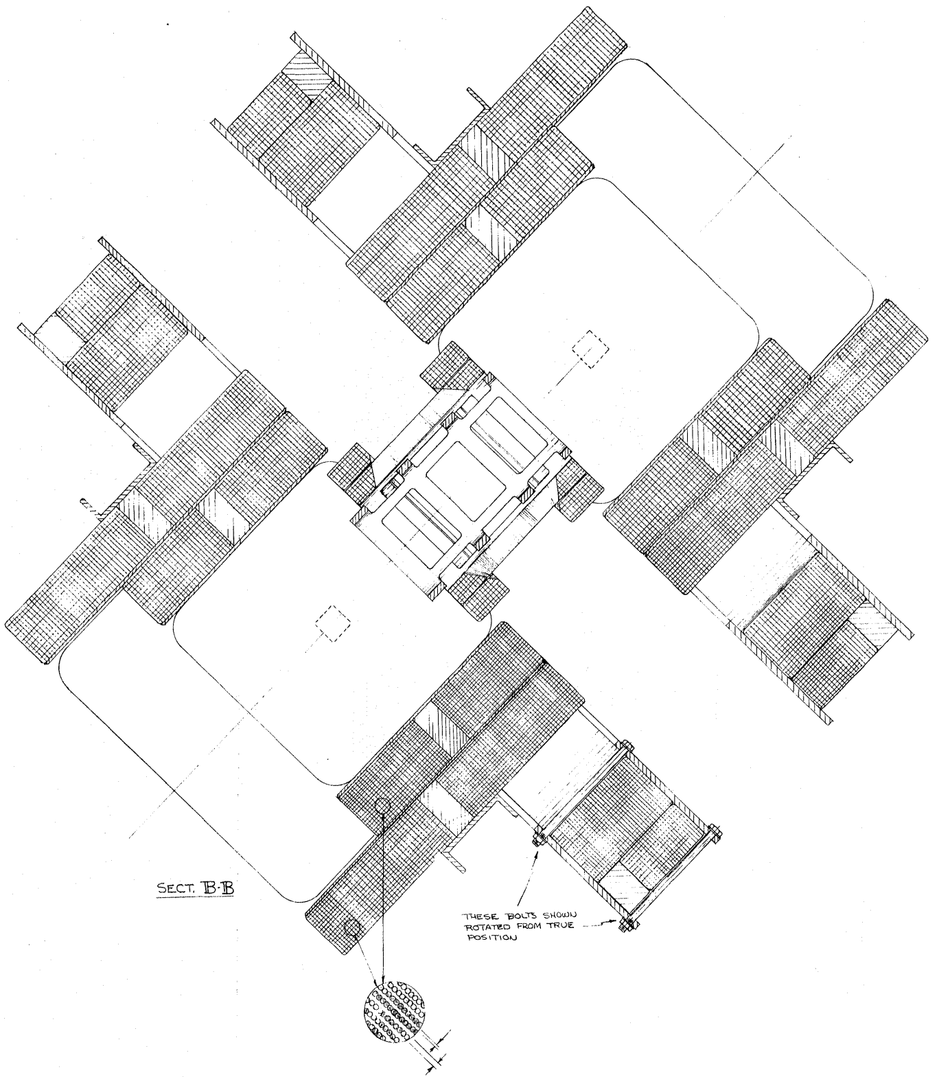
Figure 39c 45-degree Section
