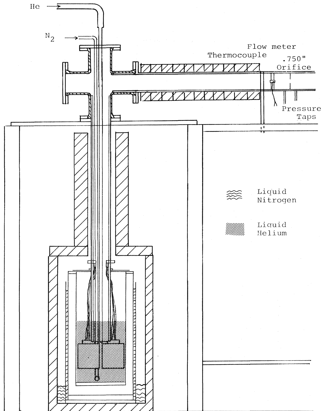
Figure 21 Experimental Schematic
