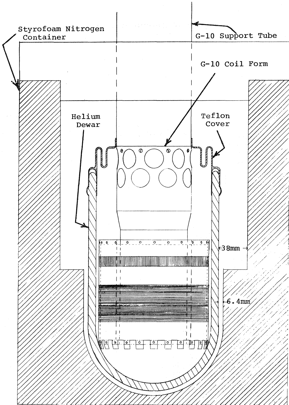
Figure 15 Dewar Assembly
