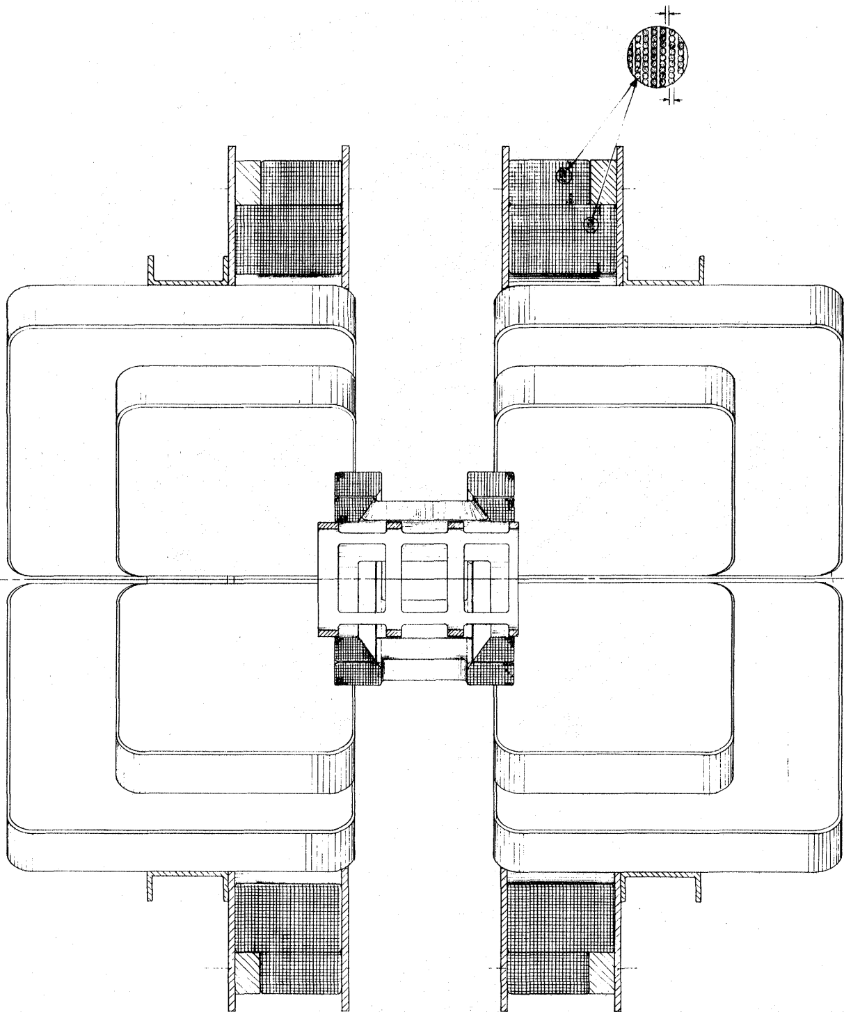
SECT. A-A
