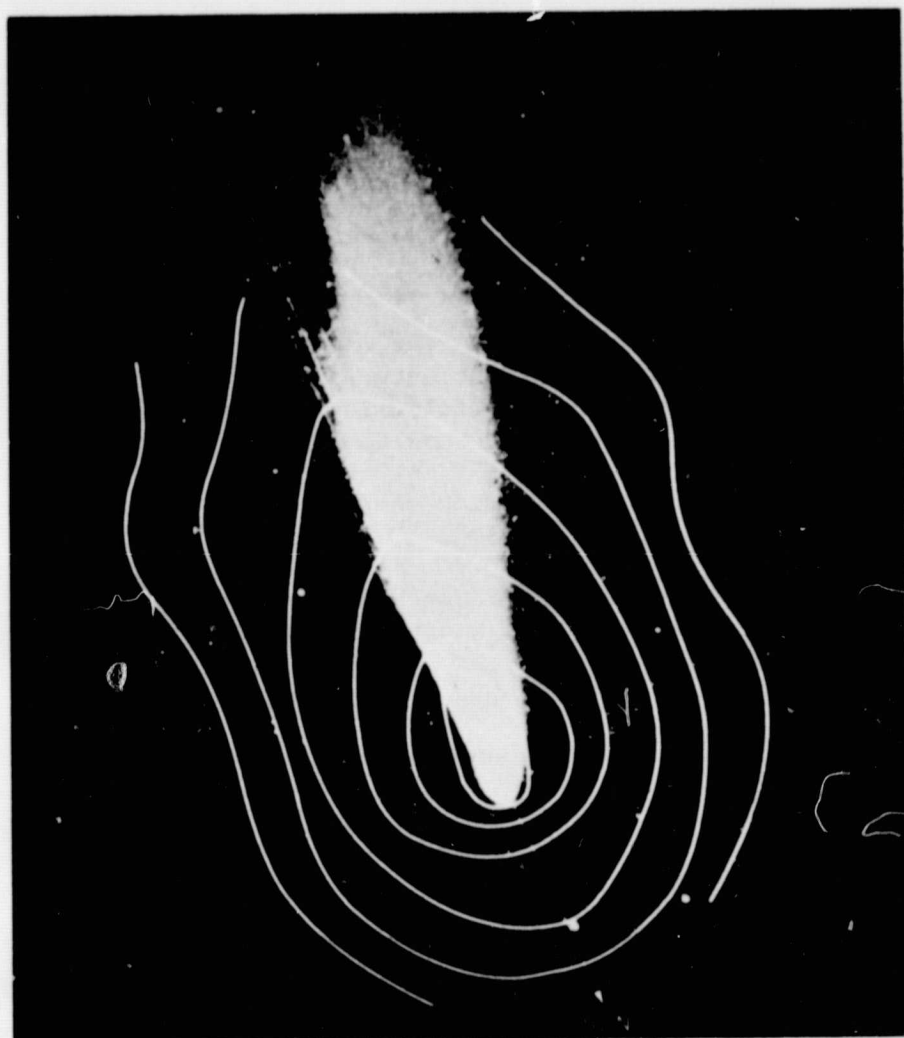
Figure 4(b). Lyman-Alpha Brightness Contours Superimposed on a Photograph of Comet Bennett (After C. Lillie).
