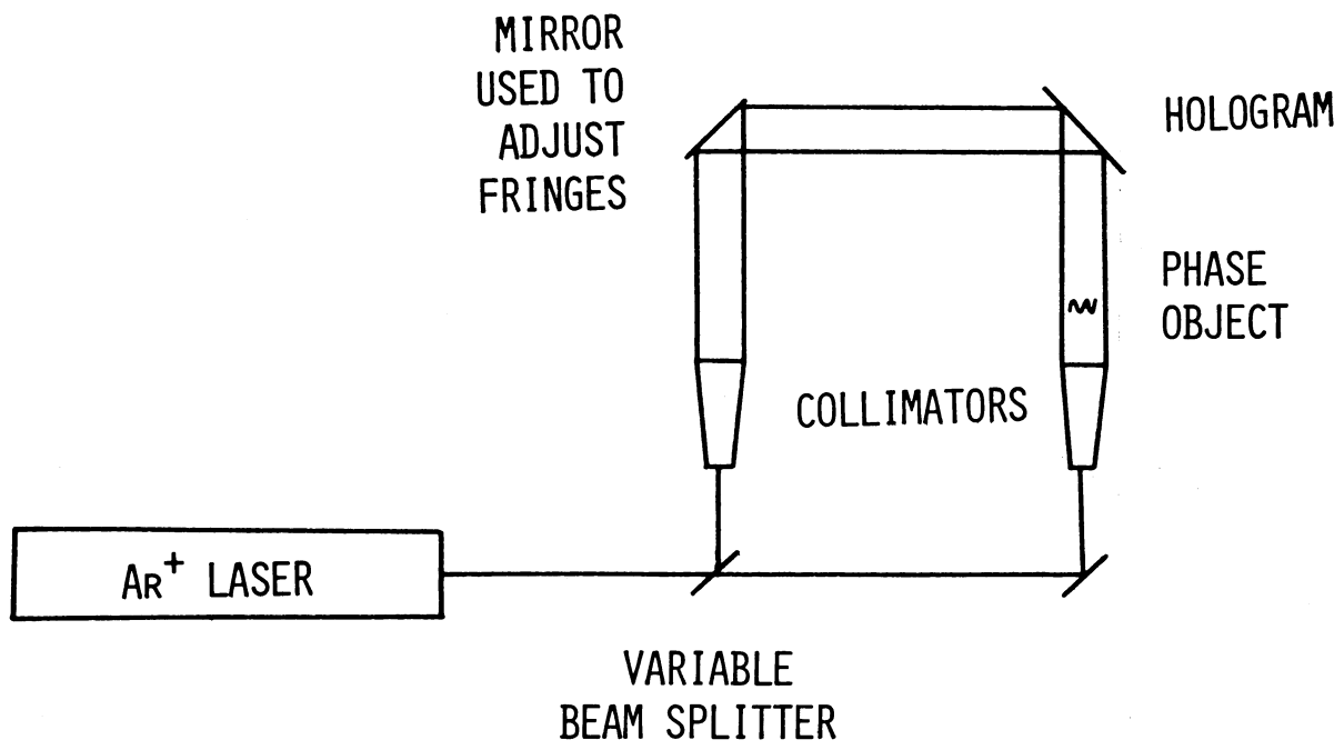
Figure 1.- Experimental arrangement.
