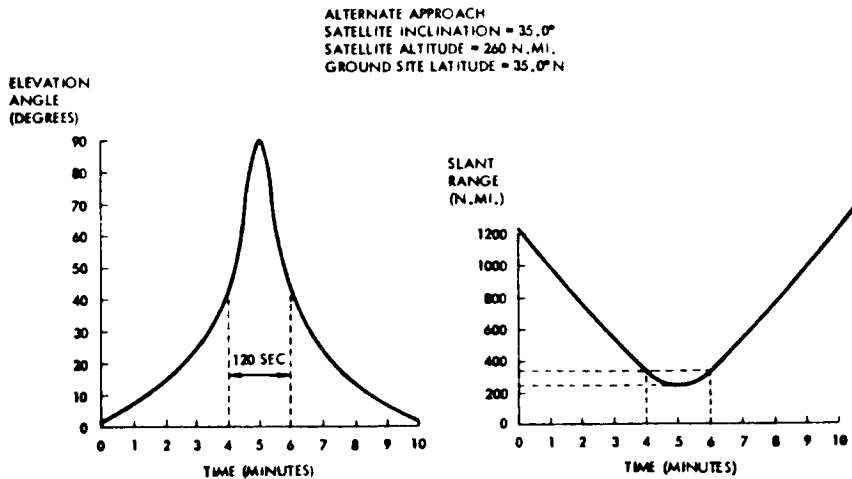
Figure 3.5-15. Flight Data Relative to Ground Site
