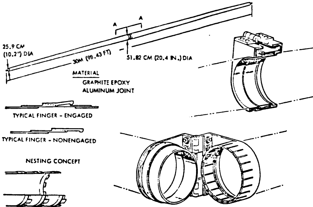
Figure 3.5-9. Hinged Nestable Tapered Strut
