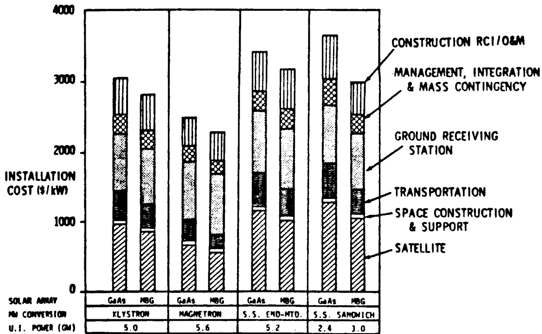
Figure 2.2-3. Installation Cost Comparisons
