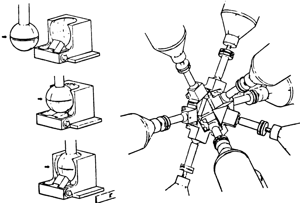
Figure 3.5-10. Ball-Socket Swivel Joint Concept
