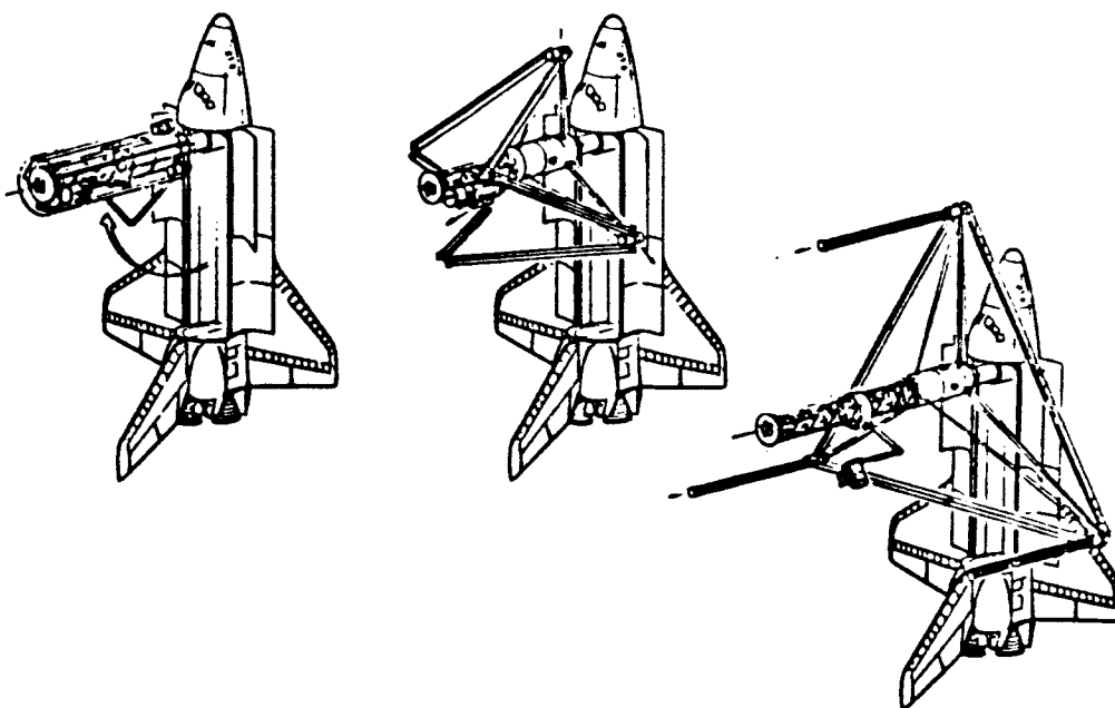
Figure 3.5-13. Concept for Antenna Structural Jig Deployment
