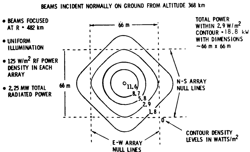
Figure 3.5-16. Ground Receiving Facility
