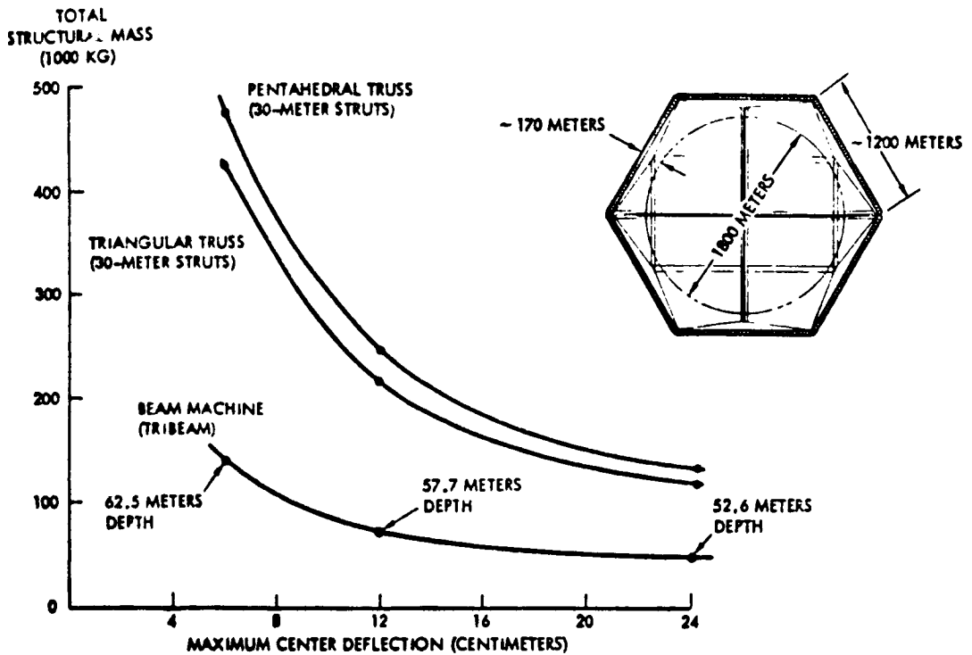
Figure 3.5-11. Candidate Structural Concept Trades
