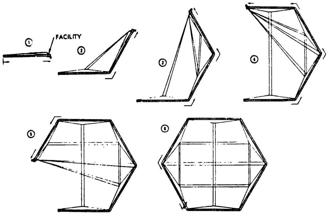
Figure 3.5-14. Cable Network Deployment
