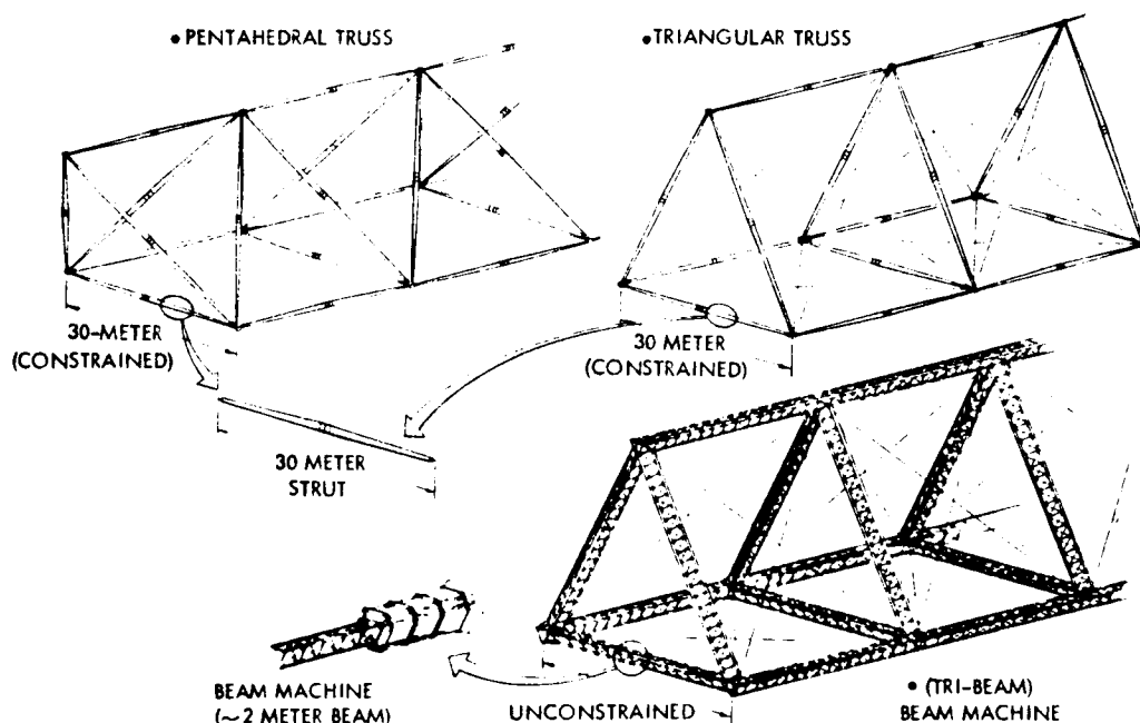
Figure 3.5-8. Candidate Antenna Structural Concepts
