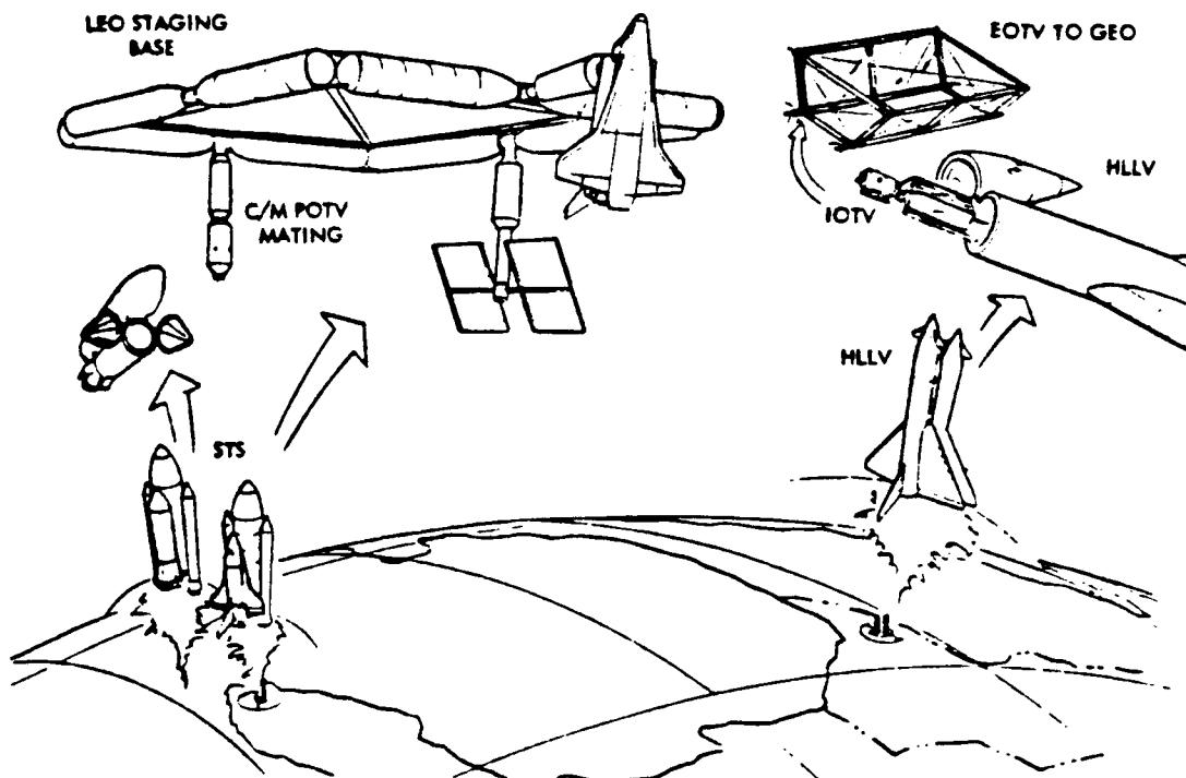
Figure 1.1-3. SPS Transportation System—LEO Operations Operational Program
