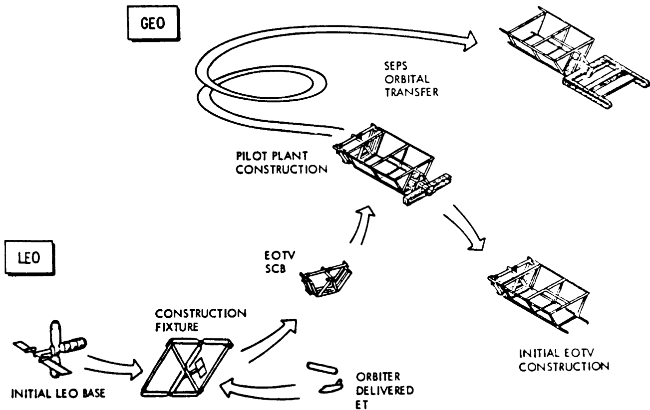
Figure 3.5-3. EOTV-Precursor Construction Scenario
