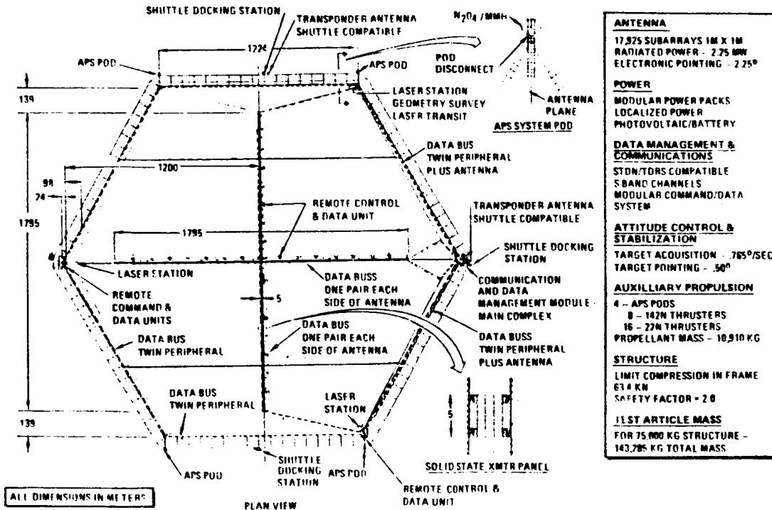
Figure 3.5-7. Demonstration/Test Article Configuration
