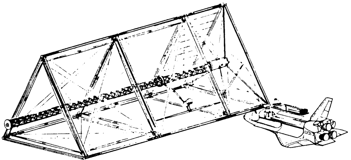
Figure 3.5-12. Structural Jig Concept for Triangular Truss
