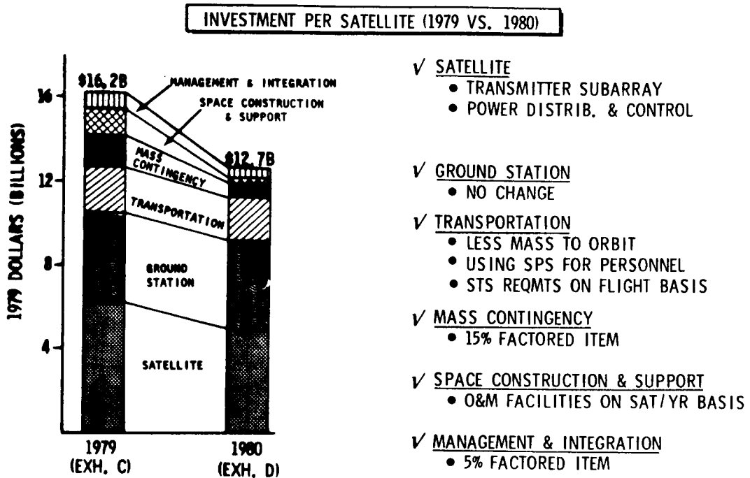
Figure 2.2-4. Rockwell SPS Reference Concept Comparison (3-Trough/Planar/Klystron)
