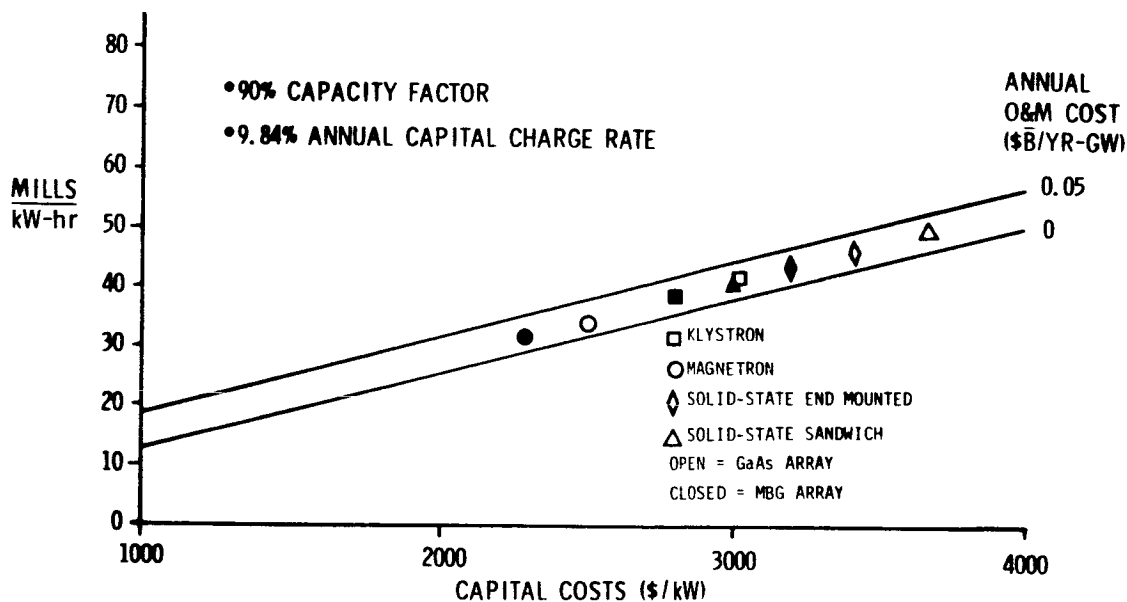
Figure 4.1-1. Utility Bus-Bar Comparisons
