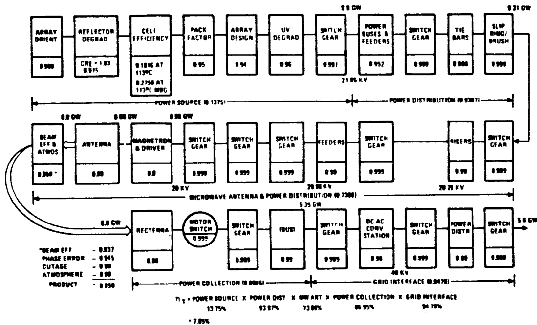
Figure 1.2-2. System Efficiency Chain—Magnetron Concept (June 1980)
