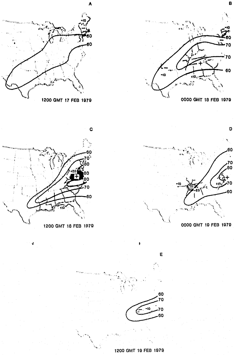
Figure 14. Evolution of the ageostrophic nature of the 332^{\circ}\text{K} winds from 1200 GMT 17 February 1979 to 1200 GMT 19 February 1979. Contours indicate actual wind velocities ( \text{ms}^{-1} ). Shading represents whether winds are subgeostrophic (-) or supergeostrophic (+) by at least 10\text{ms}^{-1} or 20\text{ms}^{-1} (heavy shading).
