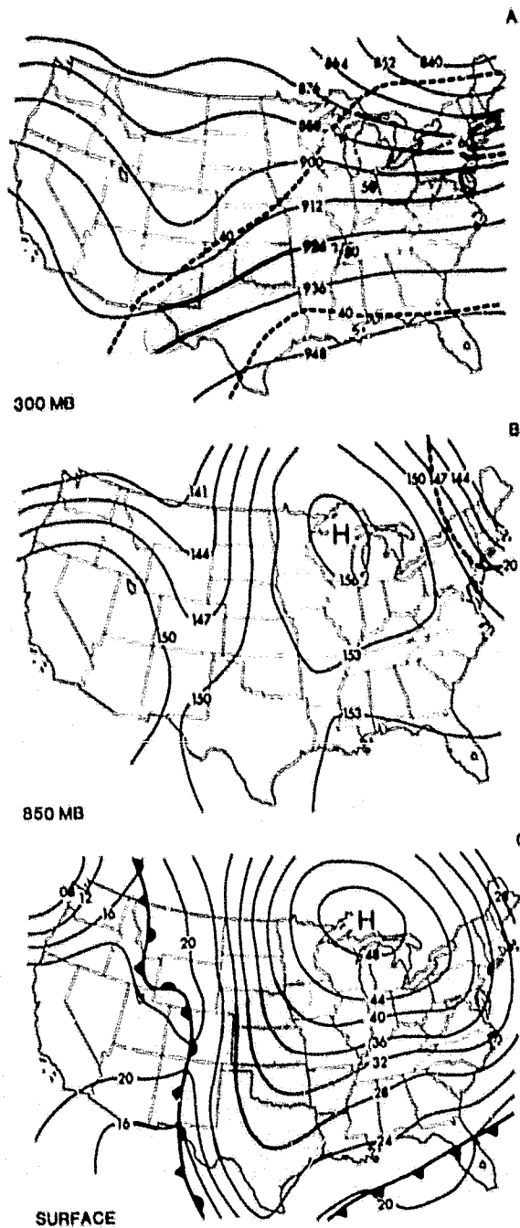
Figure 1. Isobaric and surface analyses for 1200 GMT 17 February 1979. (A) 300 mb geopotential height (solid, 900 = 9000 m) and isotach (dashed, \text{ms}^{-1} ; shaded region represents velocities between 50\text{ms}^{-1} and 60\text{ms}^{-1} ). (B) 850 mb geopotential height (solid, 150 = 1500 m) and isotach (dashed, \text{ms}^{-1} ). (C) Surface isobars (solid, 40 = 1040 millibars), precipitation (shaded).
