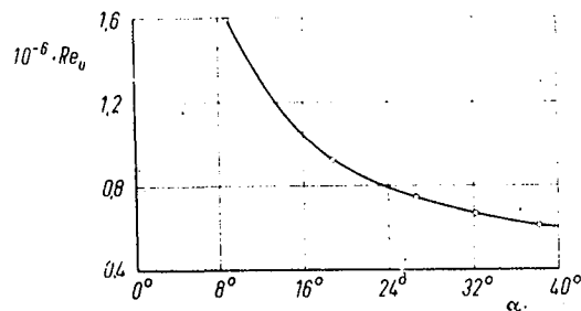
Figure 4. Dependence of the Reynolds number Re_0 = U_\infty x_{LE} / \nu on the incidence angle \alpha for the Delta wing with the aspect ratio of \Lambda=1.0
