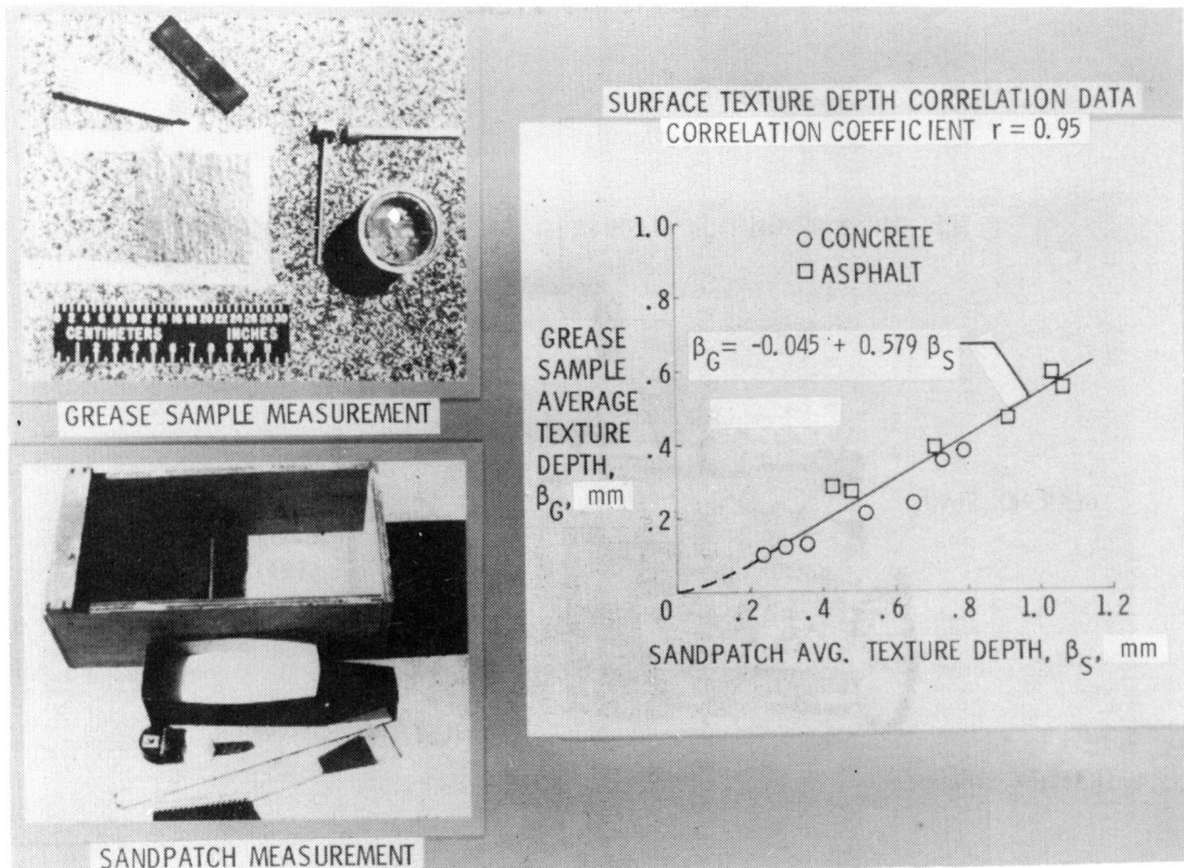
Figure 11.- Example of surface texture measurement correlation.
