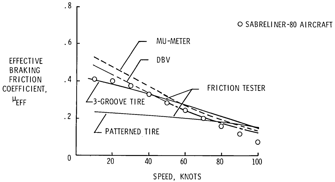
(c) Small aggregate asphalt surface.
