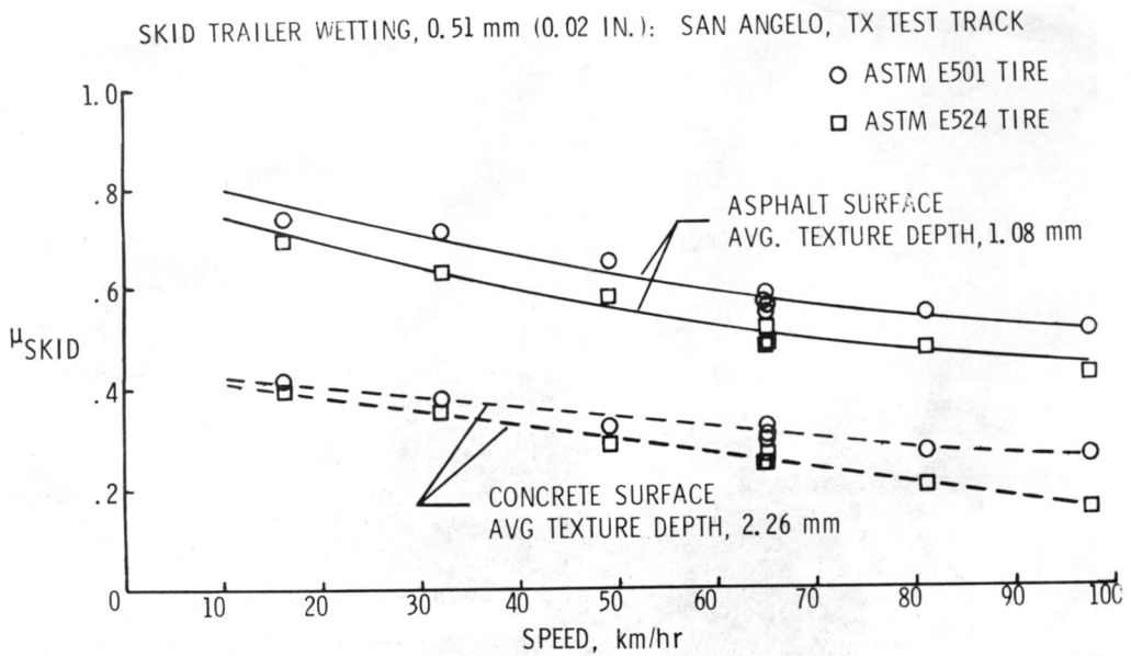
Figure 10.- Friction performance of two ground vehicle test tires.
