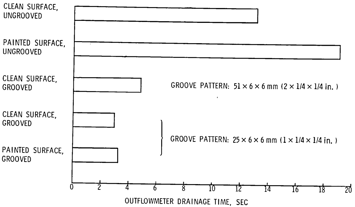
Figure 12.- Effect of surface treatments on outflowmeter drainage measurements.
