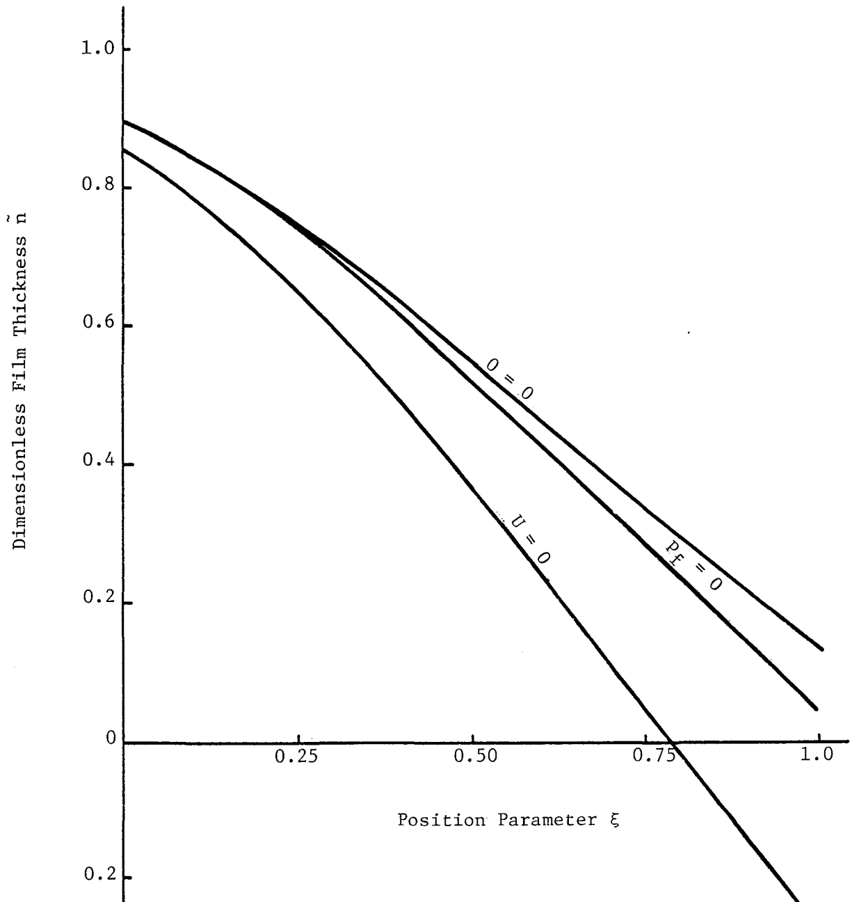
Fig. 38 Dimensionless Film Thickness Profiles, Stroke = 25.4 mm
