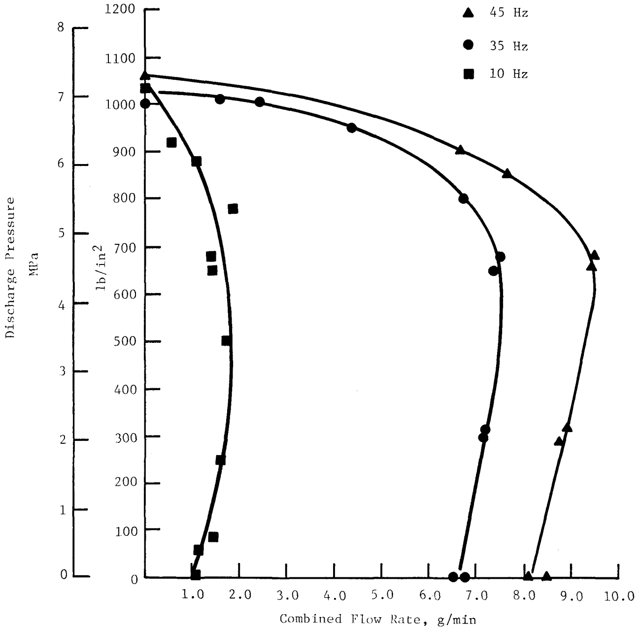
Fig. 17 Pressure-Flow Characteristic, Data Point 1.X.X.3
