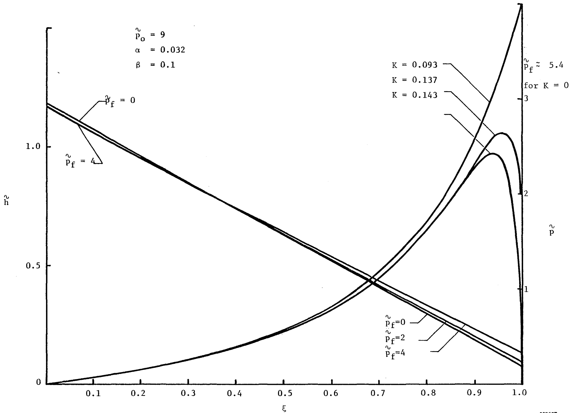
Fig. 32 Pressure and Film Thickness, \beta = 0.1 , \tilde{\beta}\tilde{p}_o = 0.9
