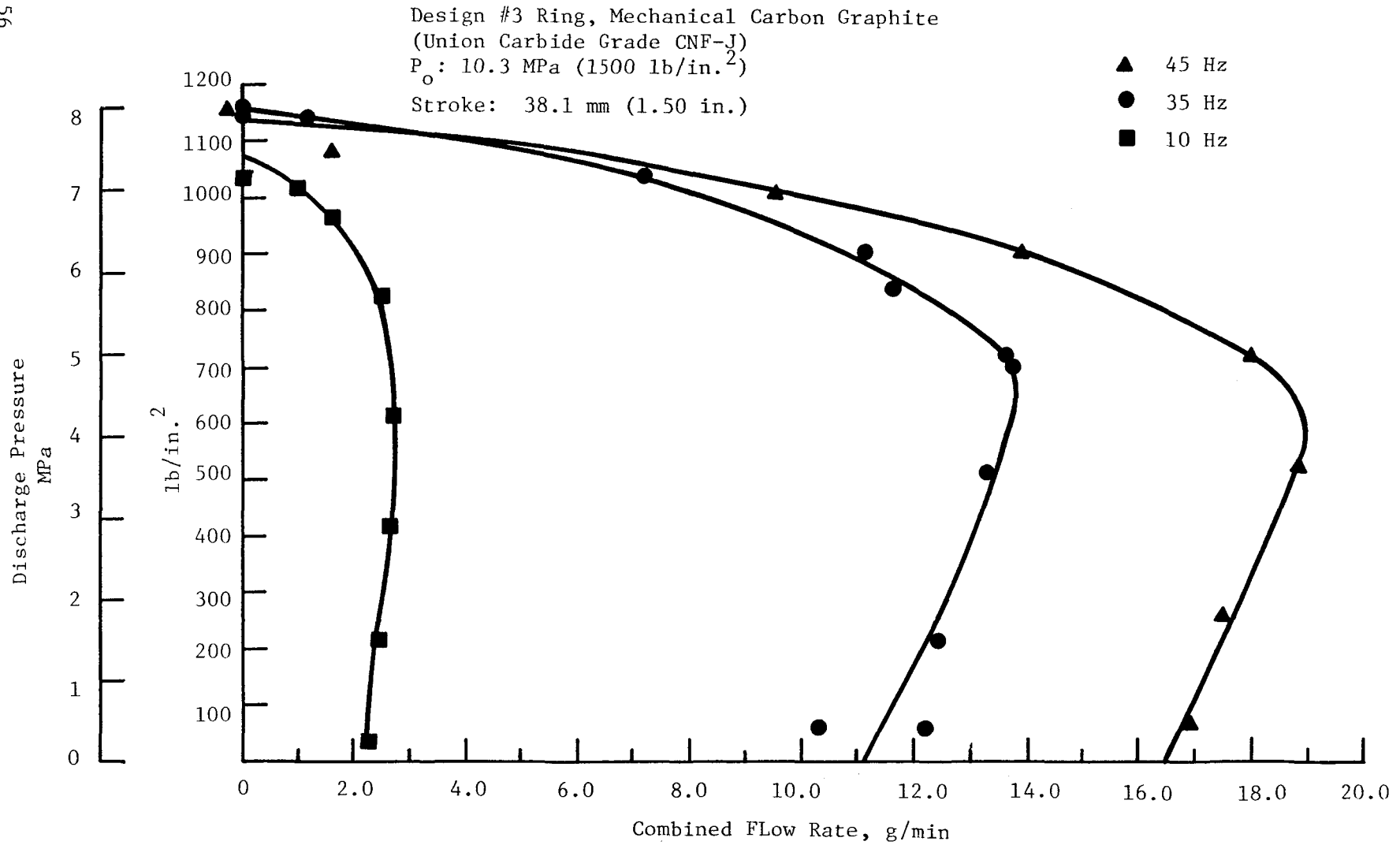
Fig. 18 Pressure-Flow Characteristic, Data Point 2.X.X.3
