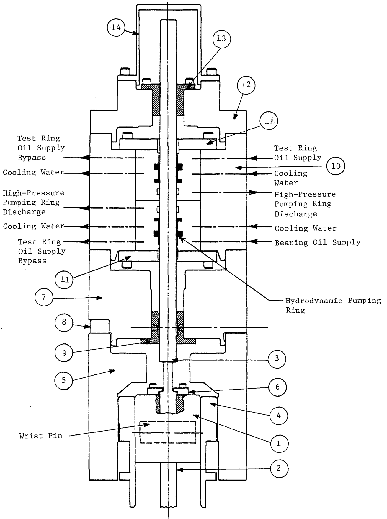
Fig. 1 Test Head Assembly
