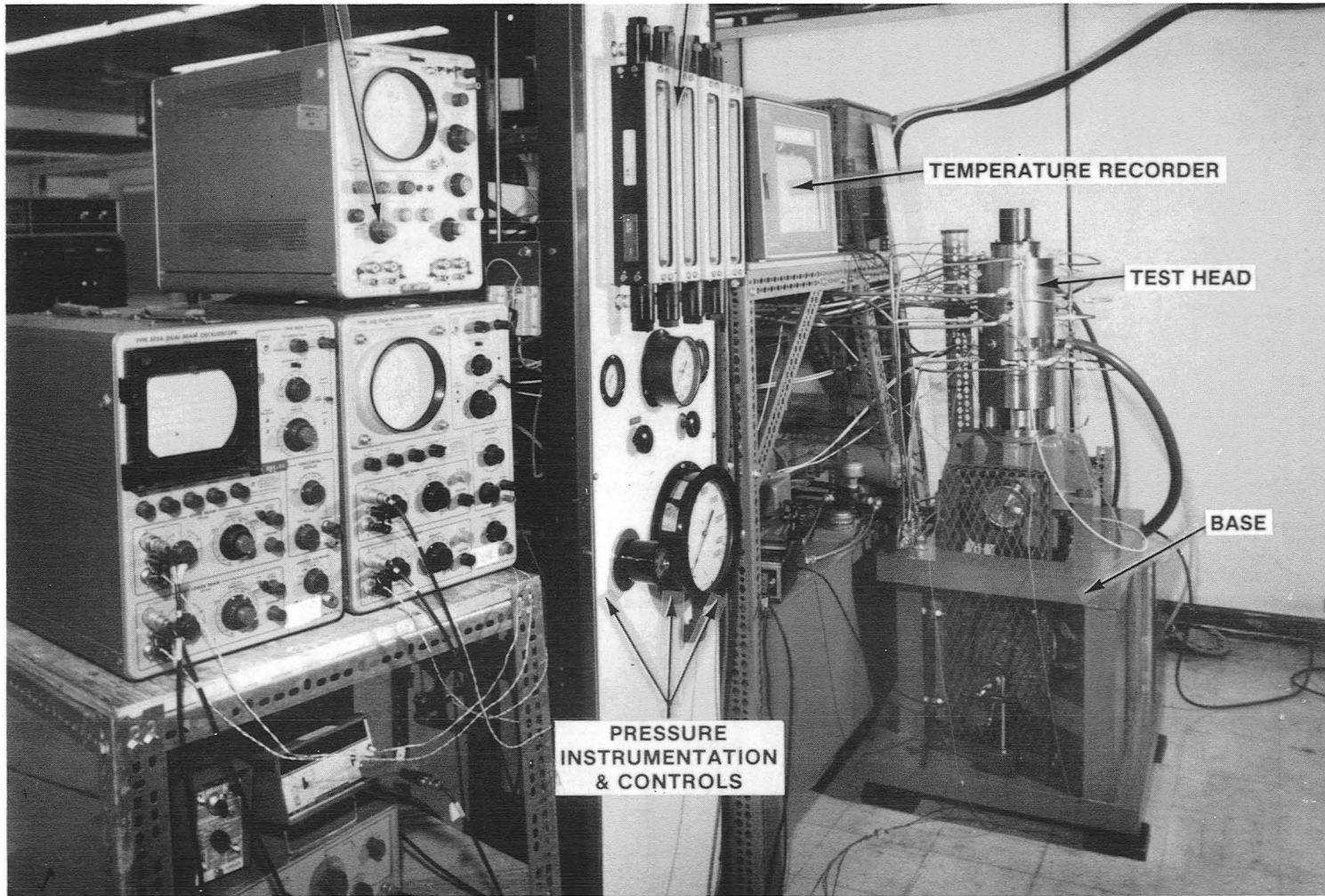
Fig. 9 Installed Tester
