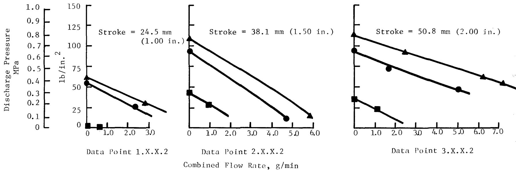
Fig. 16 Pressure-Flow Characteristic
