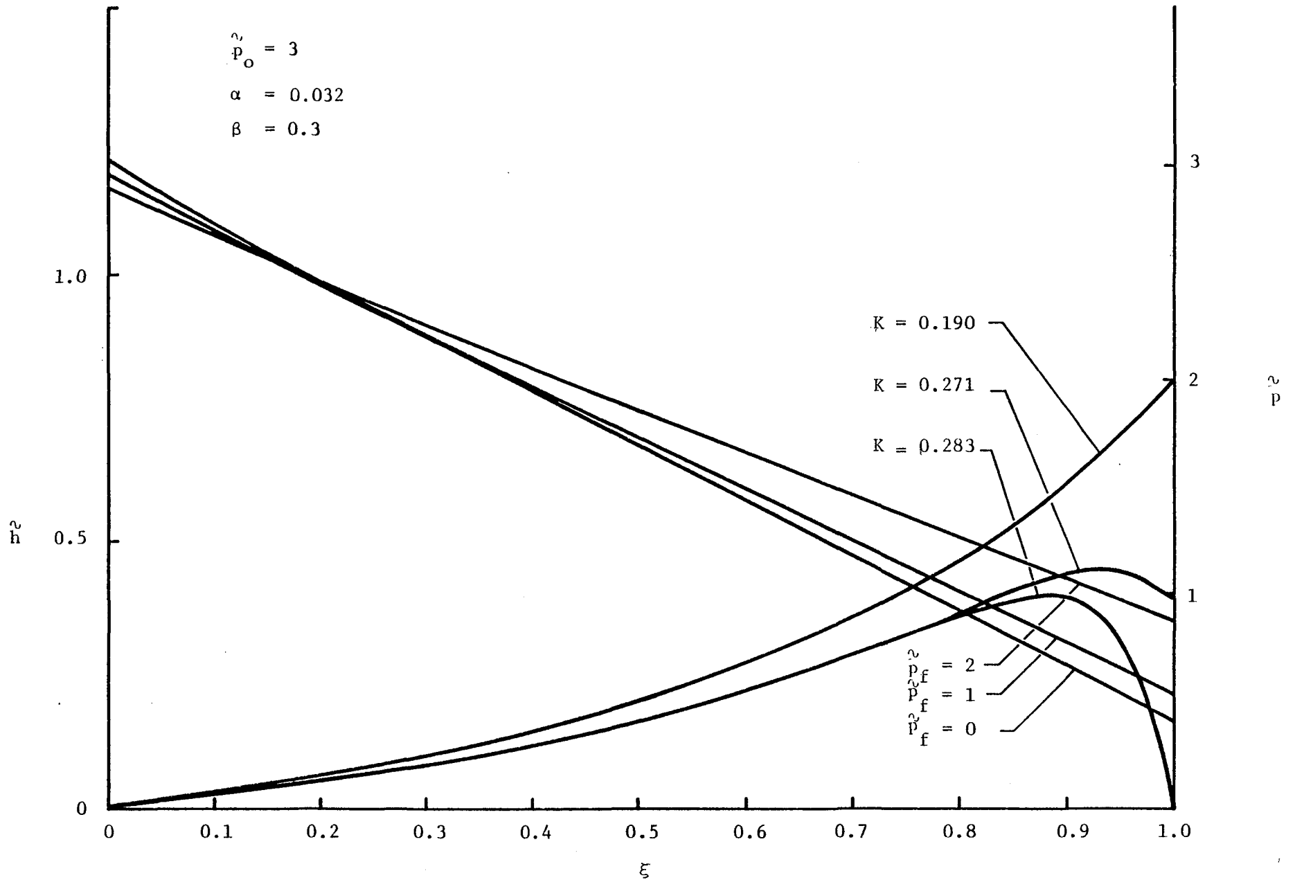
Fig. 31 Pressure and Film Thickness, \beta = 0.3 , \tilde{p}_0 = 0.9
