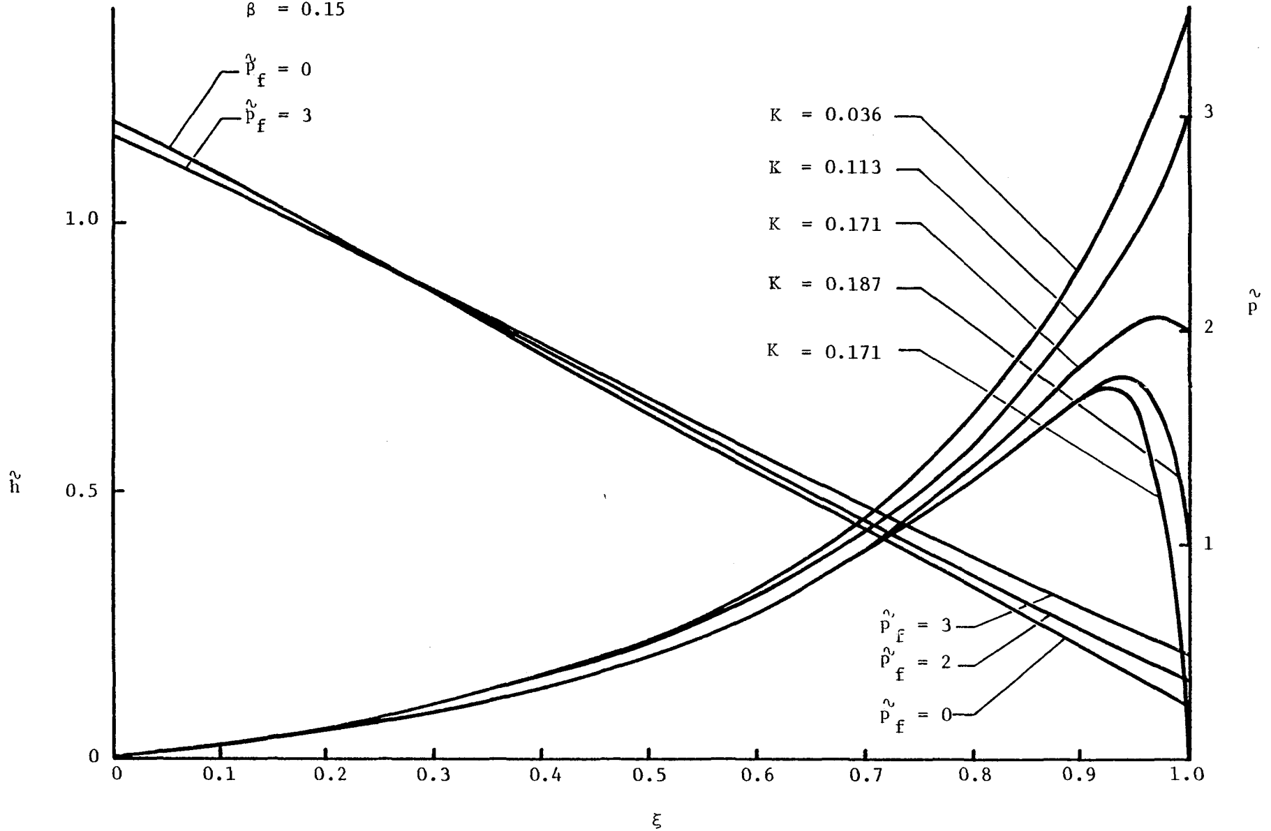
Fig. 26 Pressure and Film Thickness, Central Case
