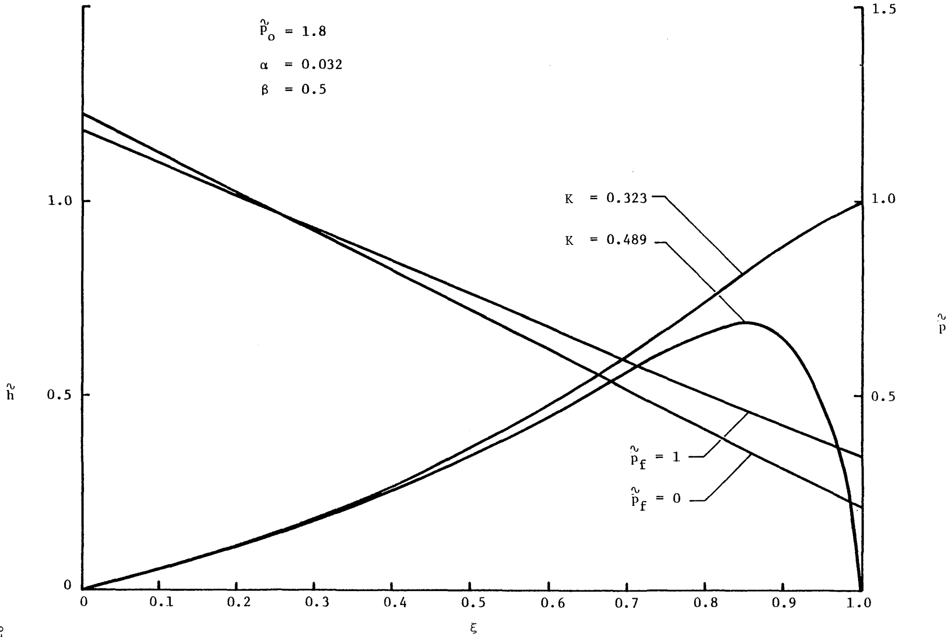
Fig. 30 Pressure and Film Thickness, \beta = 0.5 , \beta_{p_0} = 0.9
