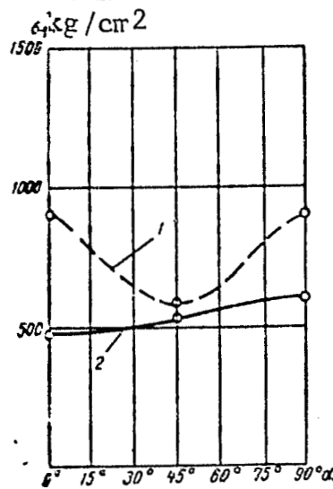
Figure 3.36. Endurance Limits in Pure Planar Bending 1--for SVAM on epoxy-phenol binder with 1:1 fiber ratio; 2--for fiber glass-reinforced plastic fiber of cold hardening (on PN-1).
