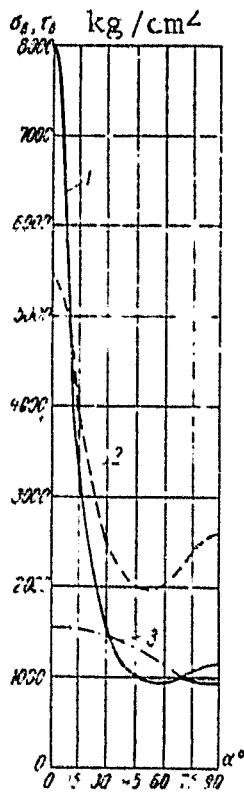
Figure 3.34. Dependence of Ultimate Strength on Orientation of Samples for SVAM with Fiber Ratio 1:13. 1--in stretching; 2--in compression; 3--in shear.
