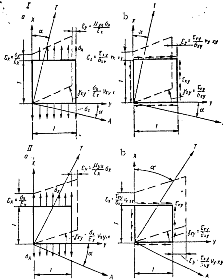
Figure 2.2. Schematic Illustration of Deformation of Anisotropic Material a--with free stretching; b--with pure shear; I--with positive and II--with negative value of coefficient of cross deformation
