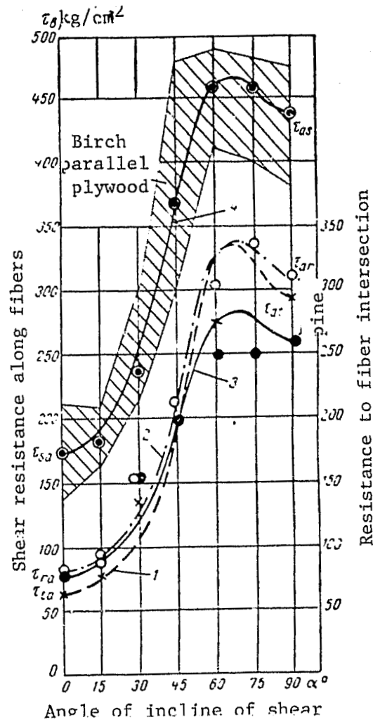
area to fibers Figure. 3.9. Results of Testing Pine (1,2,3) and Parallel Birch Plywood (4) for Shear Average values of ultimate strength for pine: X--for curve 1; o--for curve 2; ●--for curve 3; θ--for birch plywood.
