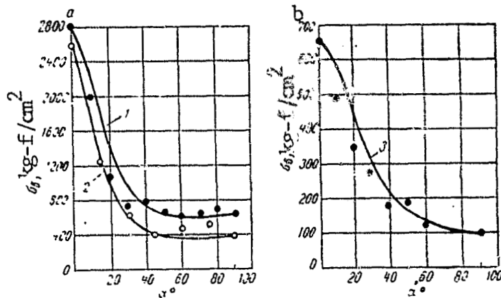
Figure 3.19. Change in Ultimate Strength of Films 1--caprone; 2--polyethylene terephthalate; 3--polyethylene depending on angle \alpha between direction of stretching and direction of orientation of the film. Experimental average quantities of ultimate strength: ●--for caprone and polyethylene; ○--for lavsan.
