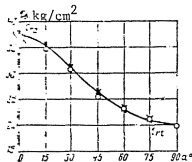
Figure 3.11. Ultimate Strength of Pine to Shearing in Tangential Plane Depending on Angle \alpha between the Direction of Tangential Stresses and Direction of the Fibers o -- average values of 5 experiments according to Karlsen [41]; X -- according to formula (1.25).
