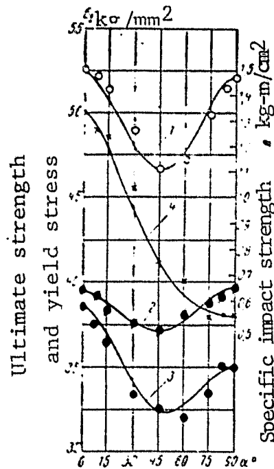
Figure 3.43. Dependence of Characteristics of Plastic Deformation Resistance during Rupture and Impact Strength \sigma_u of Aluminum Alloys on the Angle of Incline of the Force to the Direction of Rolling (according to data of Gatto and Mori): 1, 3-- \sigma_u and \sigma_y for avional; 2, 4-- \sigma_u and \sigma_y for 6061.
