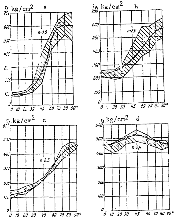
Figure 3.14. Testing Results a and b--beech laminated wood sheet Sch-T-Bu-20; c and d--multilayer plywood according to Keyl- werth [102]. Hatched region is actual dispersion of experimental data.
