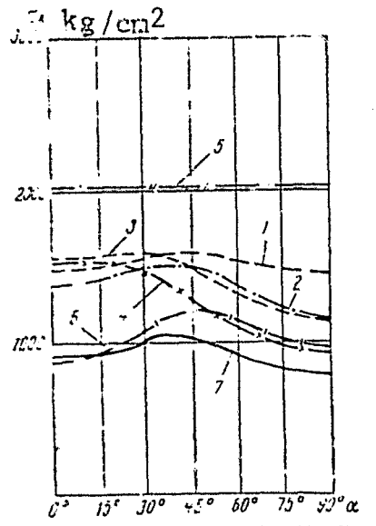
Figure 3.33. Summary Graph of Anisotropy of Fiber Glass-Reinforced Plastic in Shear 1, 2, 3, 4, 5--SVAM on epoxy-phenol binder with sheet thickness 10 mm; [continued on next page]
