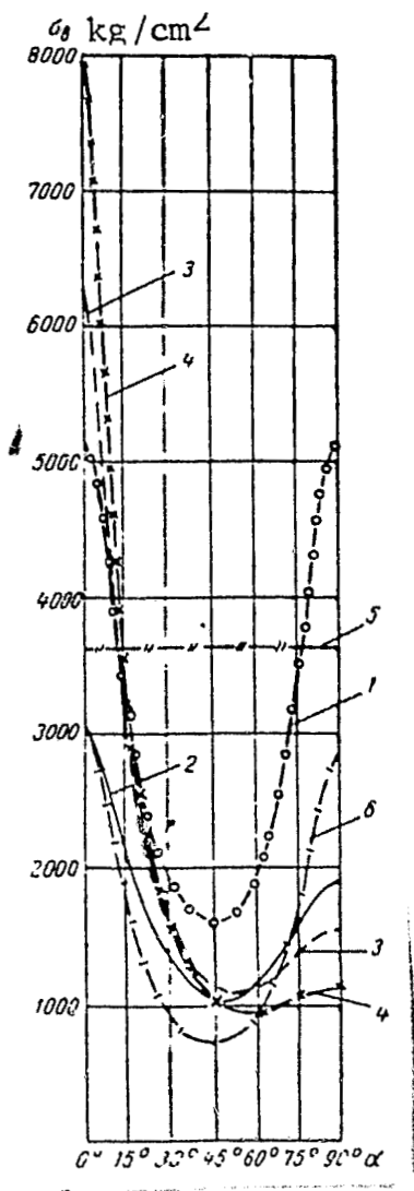
Figure 3.23. Summary Graph of Strength Anisotropy of Fiber Glass-Reinforced Plastics in Stretching
