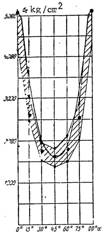
Figure 3.24. Results of Stretching Testing of SVAM 10 mm Thick on Epoxy-Phenol Binder with Fiber Ratio of 1:1 ●--average and X--extreme values of ultimate strength.
