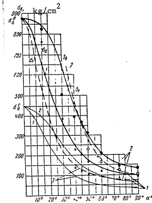
Figure 3.18. Strength of Pine in Impact Compression Depending on Angle of Incline of Fibers.
