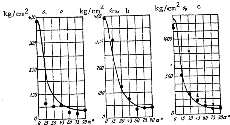
Figure 3.15. Dependence of Endurance Limits of Parallel Plywood on Angle of Fiber Incline a and b--with N=10^7 cycles; c--tests for static rupture; ●-- \sigma_e ; X-- \sigma_{max}
