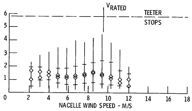
(a) VS. NACELLE WIND SPEED.
