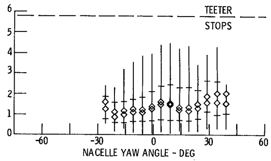
(b) VS. NACELLE YAW ANGLE.
