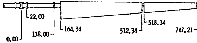
(a) BLADE PLANFORM.
