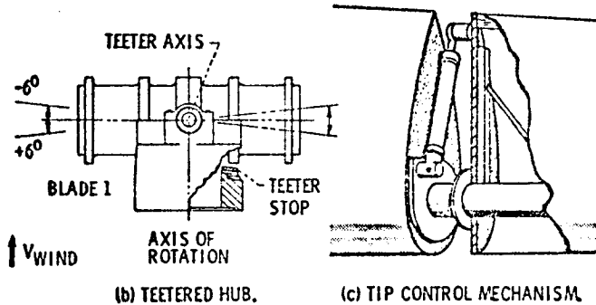
Figure 3. - Mod-0 rotor details.
