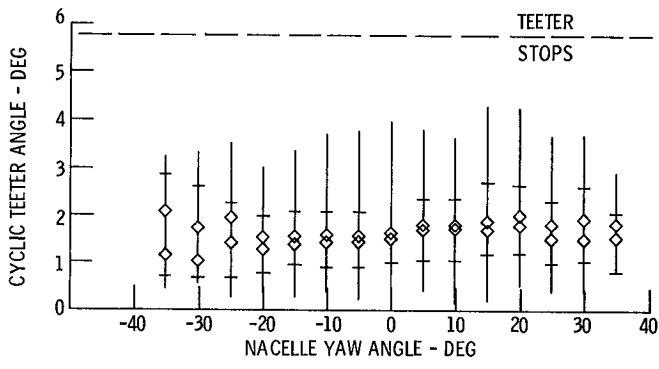
(b) VS. NACELLE YAW ANGLE.
