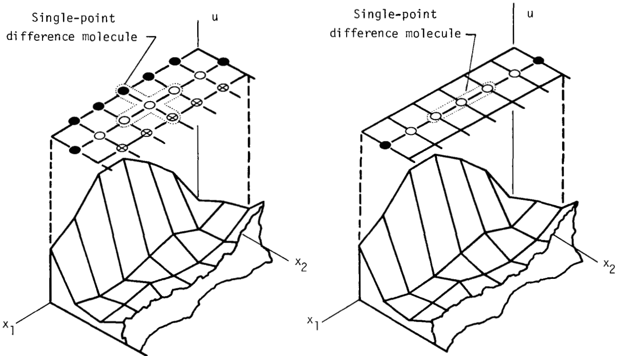
(b) LOD methods: x_1 line algorithm.
