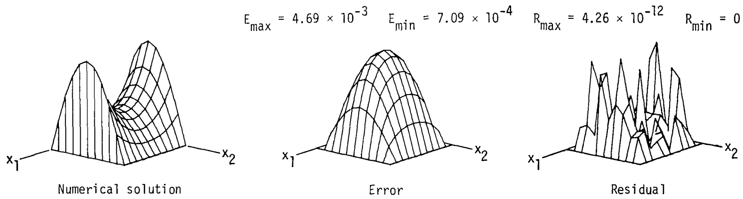
Figure 9.- Numerical results - consistent LOD backward Euler scheme with MUDF applied to TP2. \tau = 10 ; h = 0.1 .
