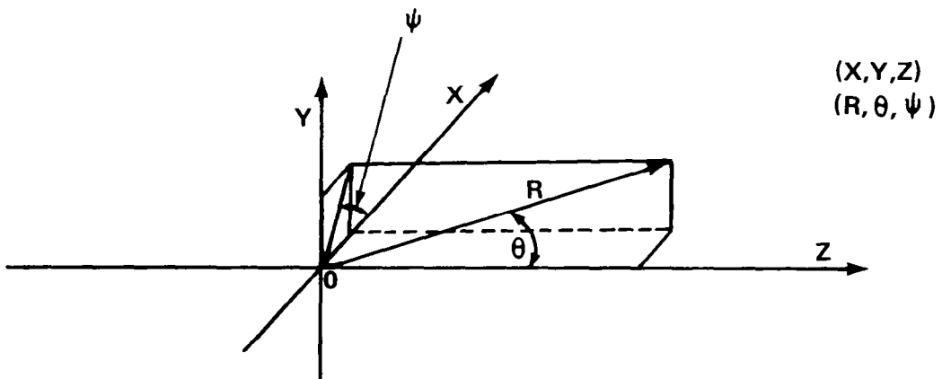
Figure 11. - Coordinate System
