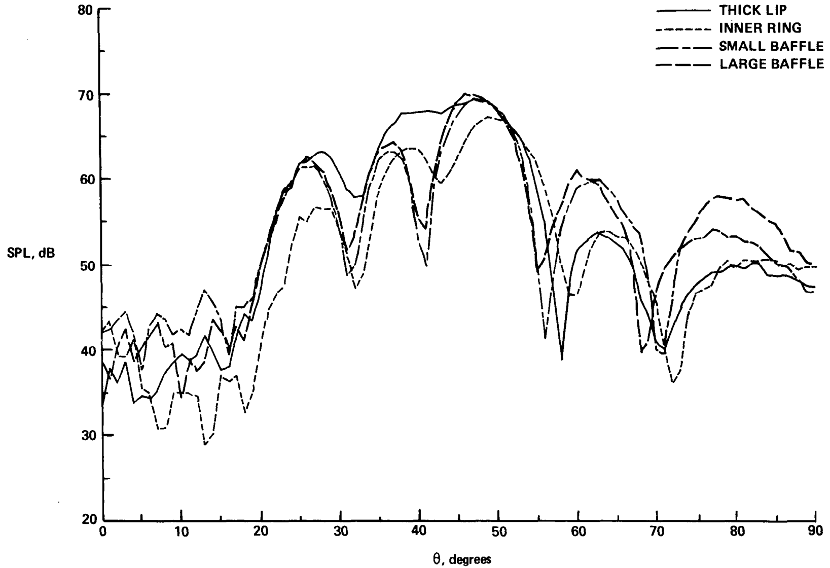
Figure 15. - Experimental Directivity Patterns of the Straight Pipe Inlets for the Plate Mode (13,2)
