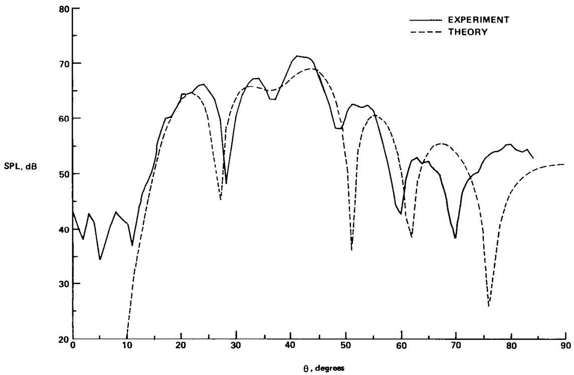
(b) LARGE BAFFLE
