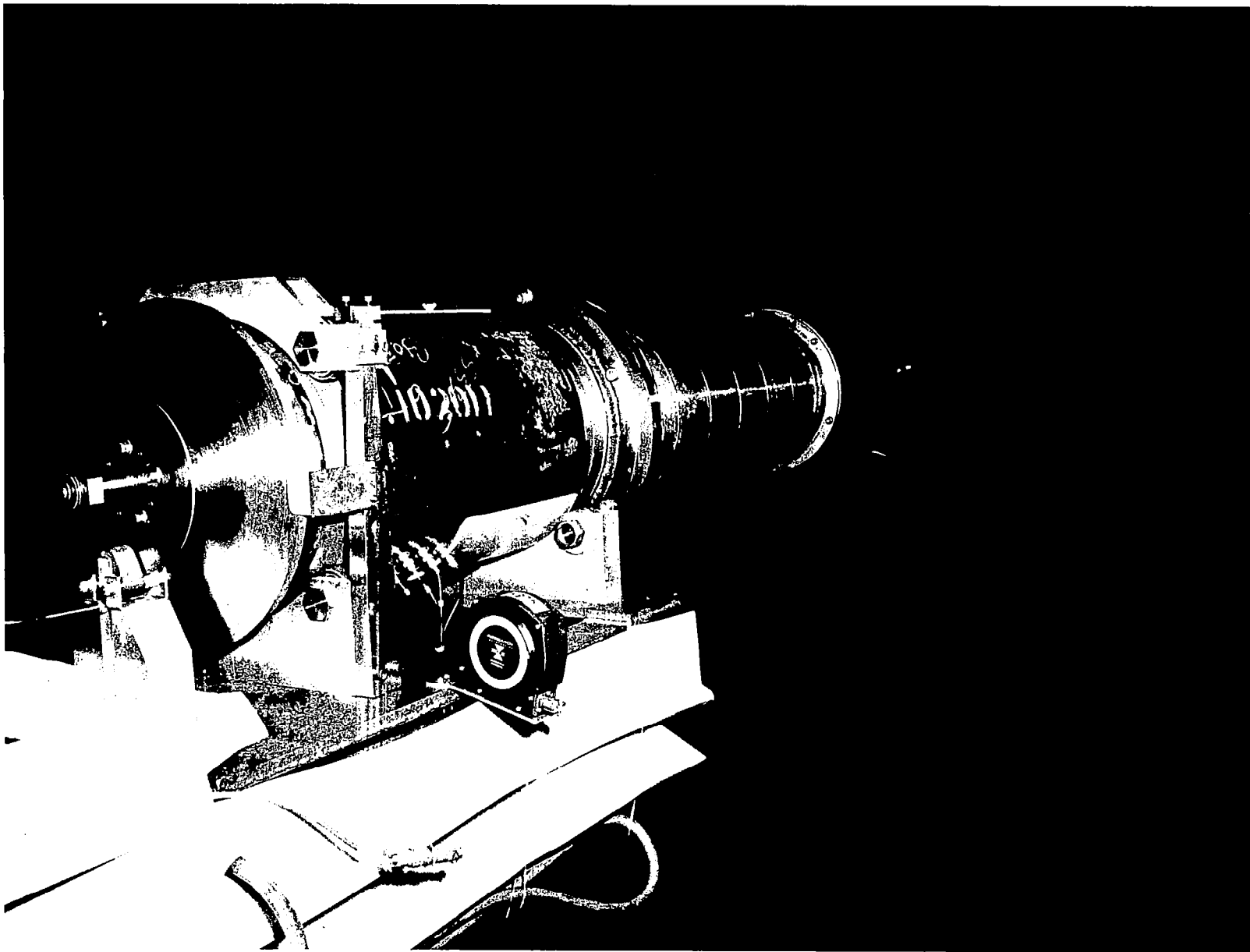
Figure 2. – Inlet-Duct-Source Assembly
