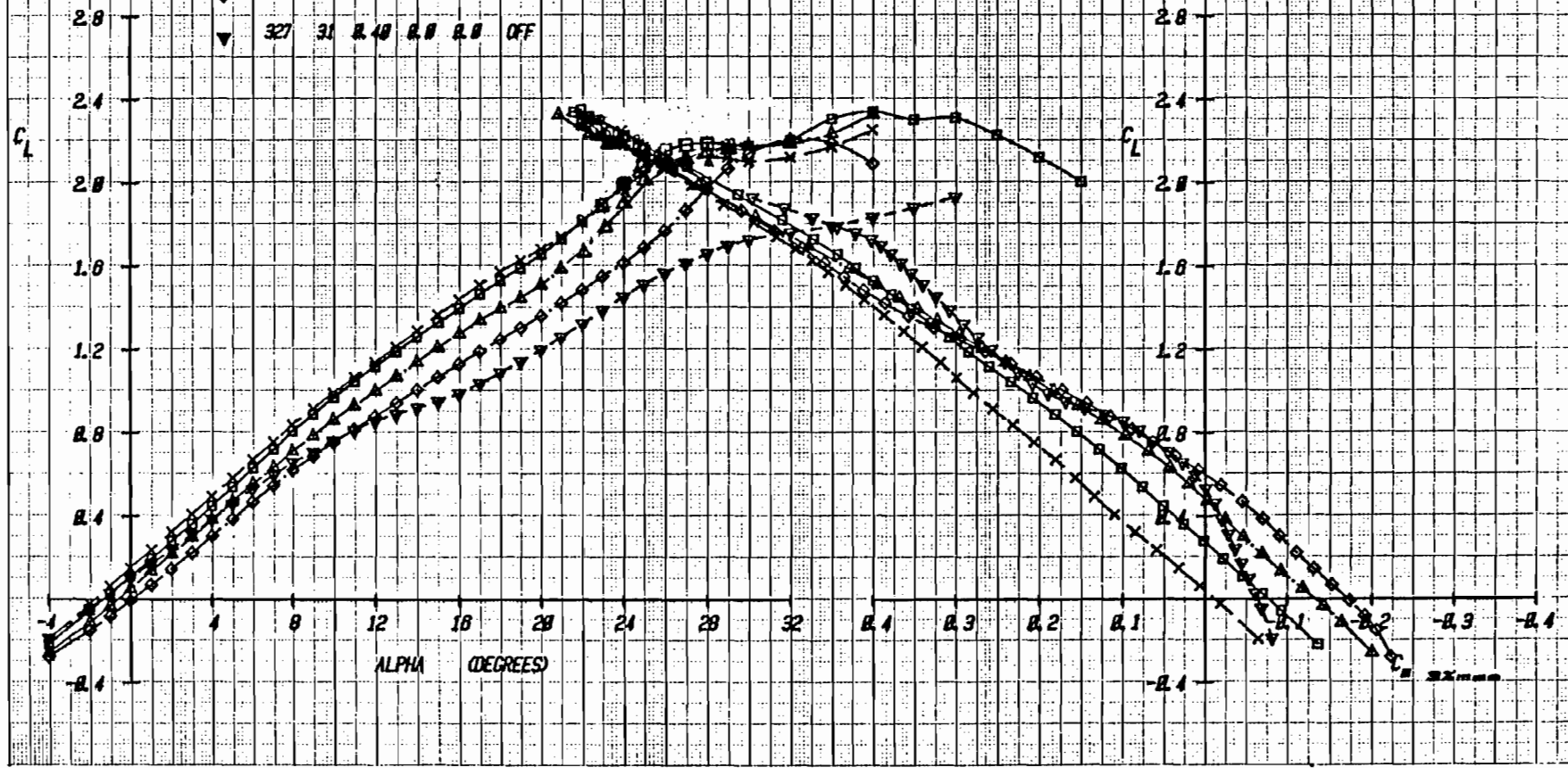
Figure 2-5a Effect of Canard Deflection on Lift and Moment with Wing Trailing-Edge Flap Undeformed, Mach = .4
