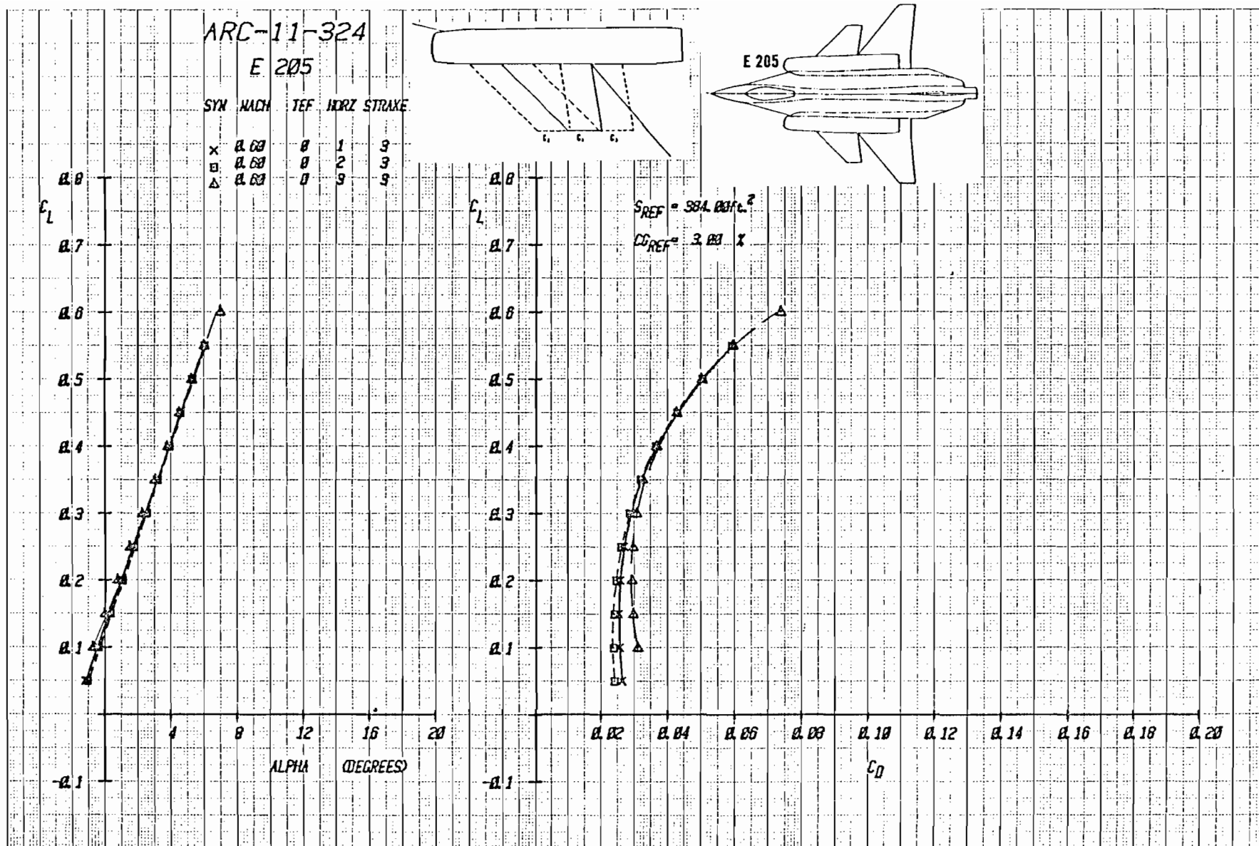
Figure 3-90 Trimméd Lift and Drag With Variations in Canard Longitudinal Location and Strake S_3 , Mach = .6
