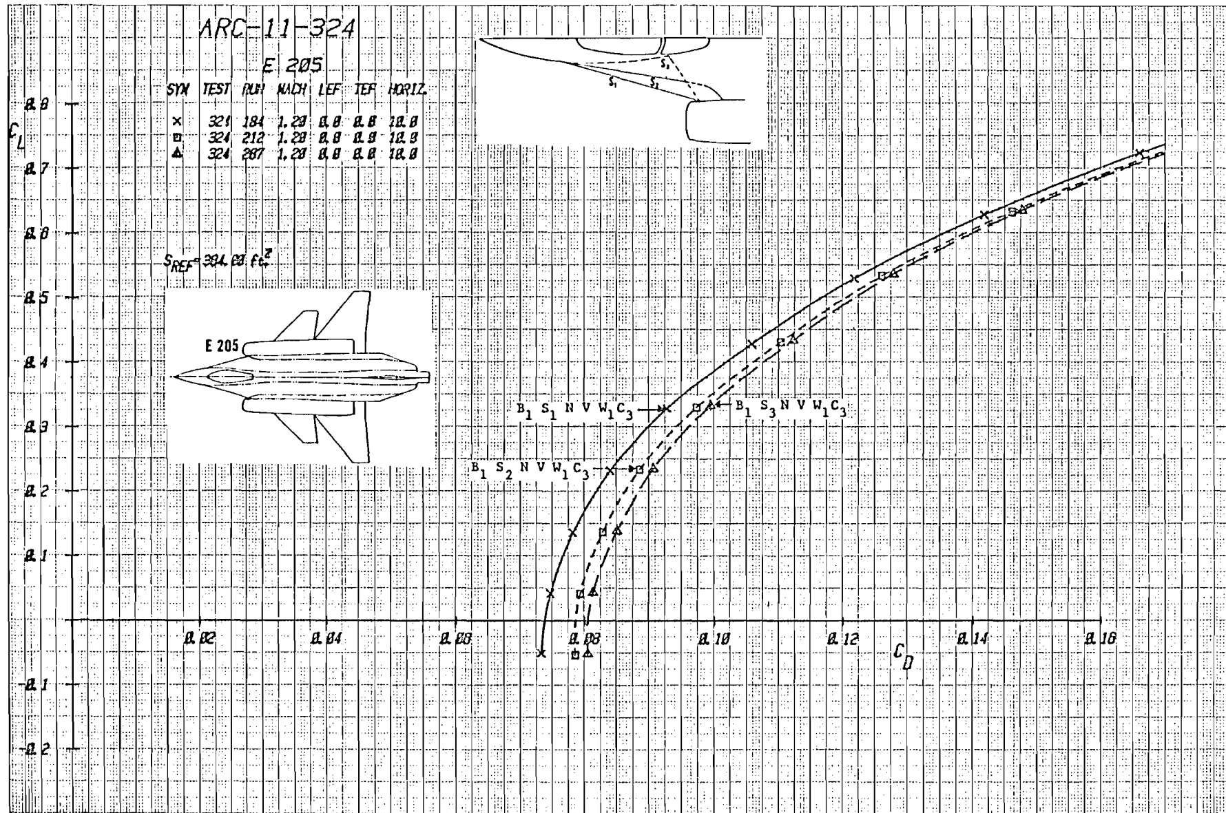
Figure 3-49b Effect of Strake Shape on Drag with Canard C_3 Deflected +10^\circ , Mach = 1.2
