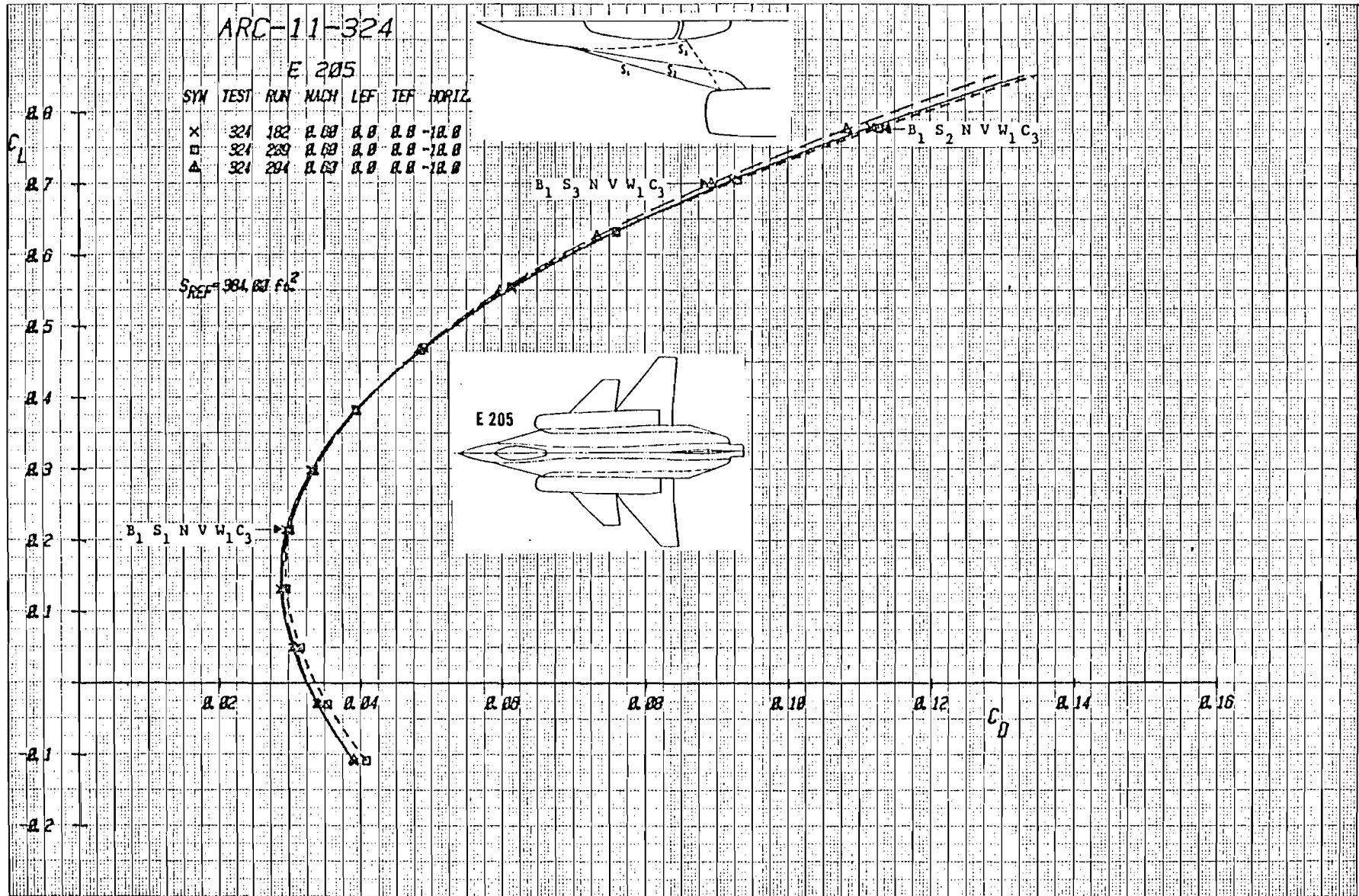
Figure3-21bEffect of Strake Shape on Drag with Canard C 3 Deflected -10°, Mach = .6
