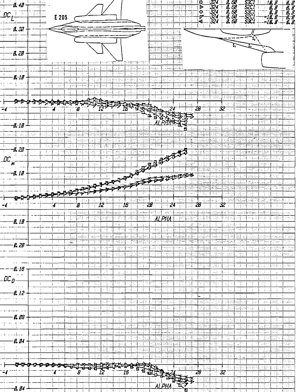
Figure 3-68 Incremental Effects of Strake Shape with Canard C 1 at Various Deflections, Mach = .6
