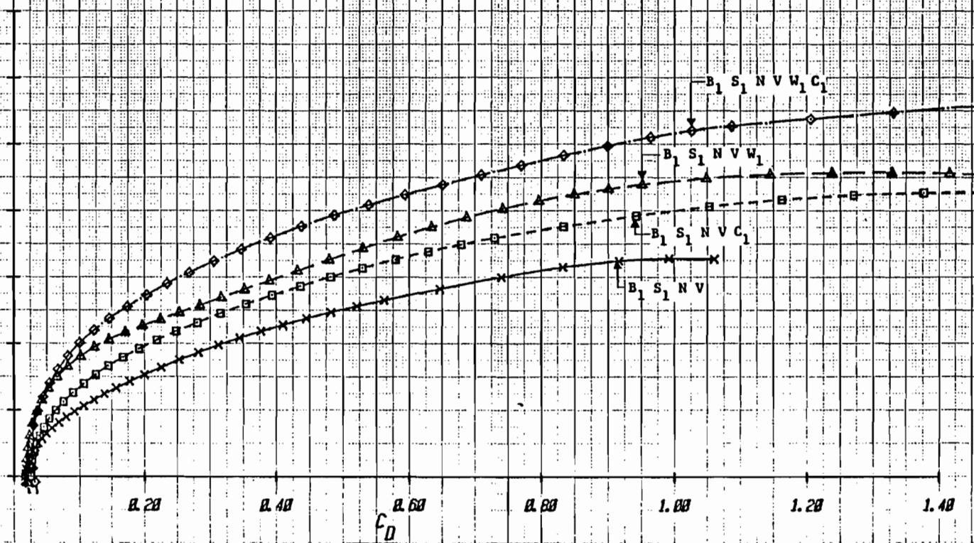
Figure 1-3c Drag Interference Data for E205 Configuration, \delta_c = -10^\circ , Mach = .2
