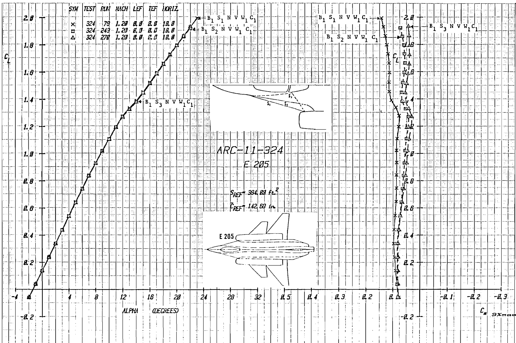
Figure 3-43a Effect of Strake Shape on Lift and Moment with Canard C_1 Deflected +10^\circ , Mach = 1.2
