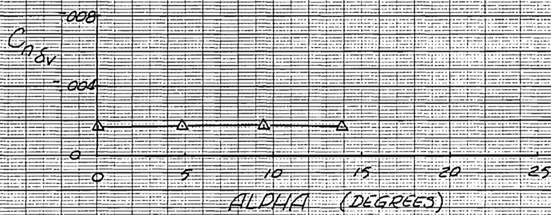
Figure 2-68 Vertical Tail Effectiveness for the E205 Baseline Configuration, Mach = 2.0
