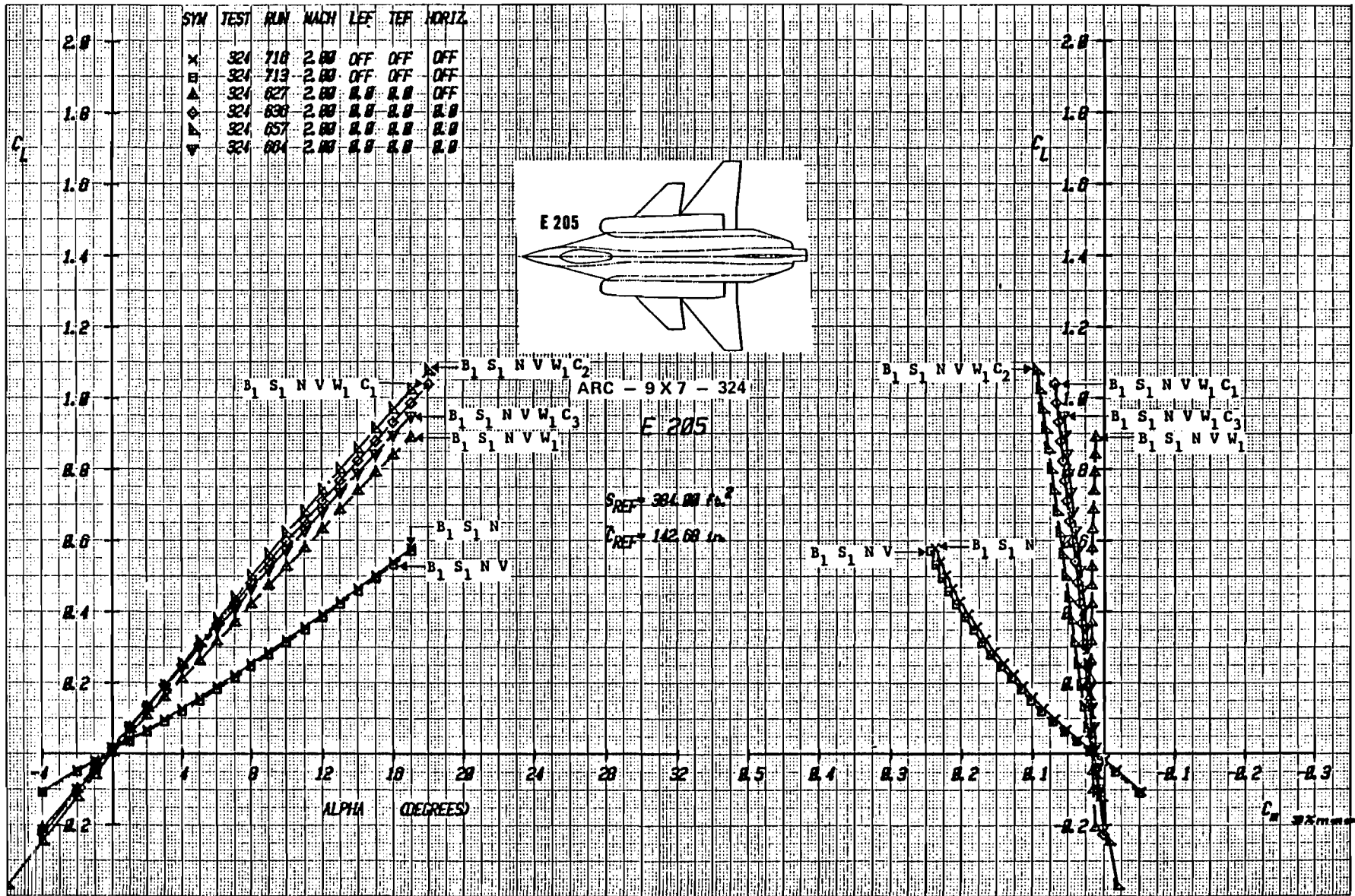
Figure-11a Effect of Component Buildup on Lift and Moment, Mach = 2.0
