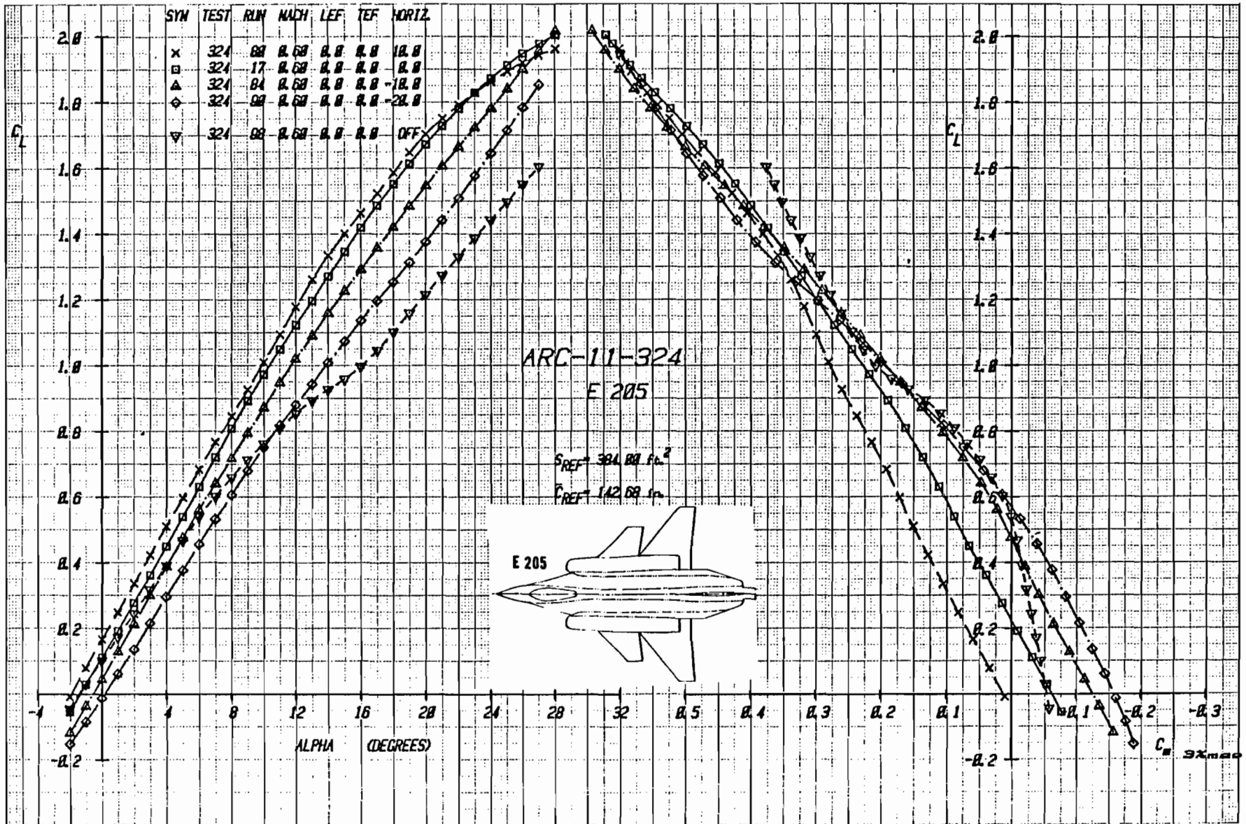
Figure 2-6a Effect of Canard Deflection on Lift and Moment With Wing Trailing-Edge Flap Undelected, Mach = .6
