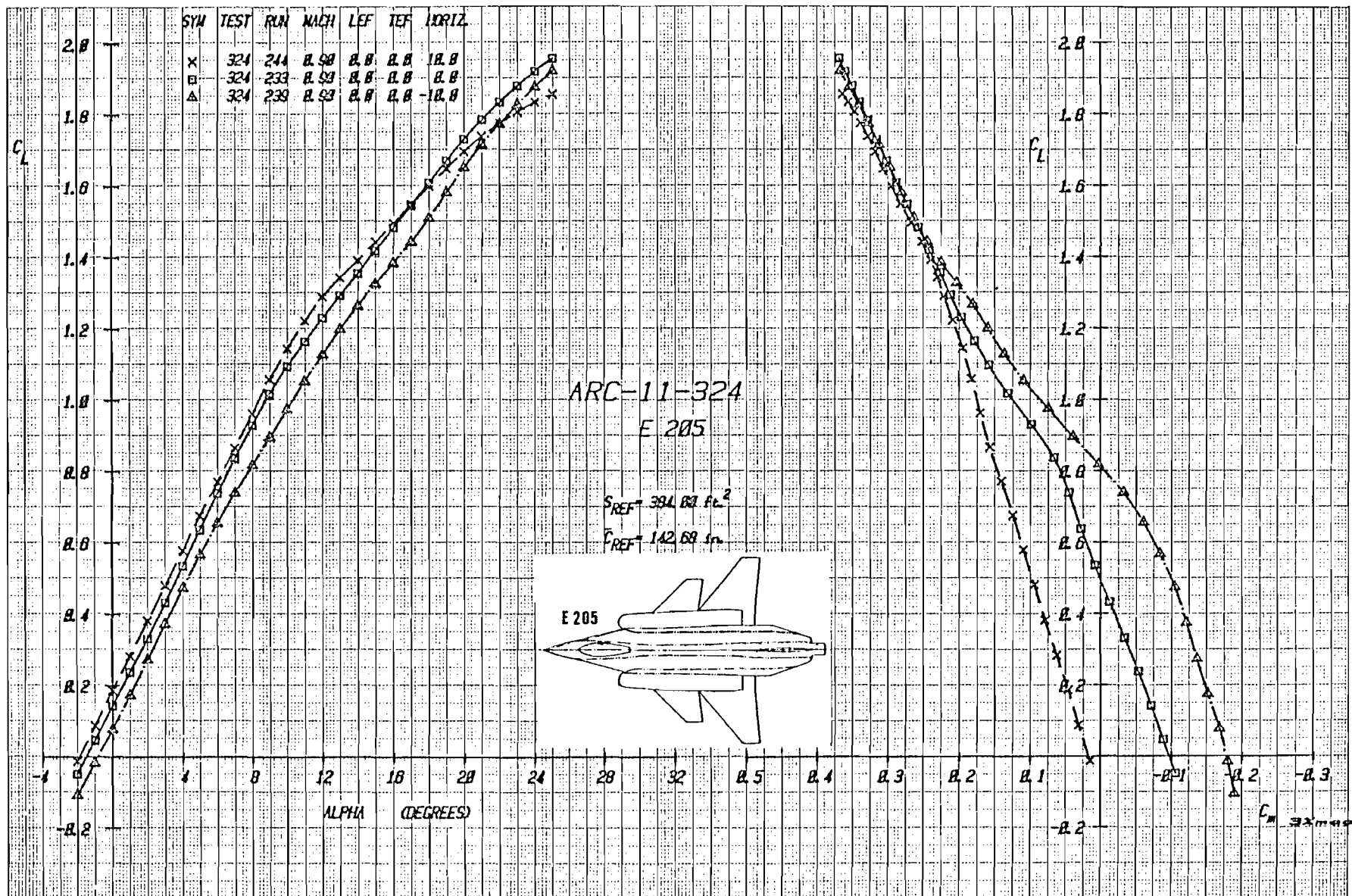
Figure 3-37a Effect of Canard Deflection on Lift and Moment with Canard C_1 , and Stroke S_2 , Mach = .9
