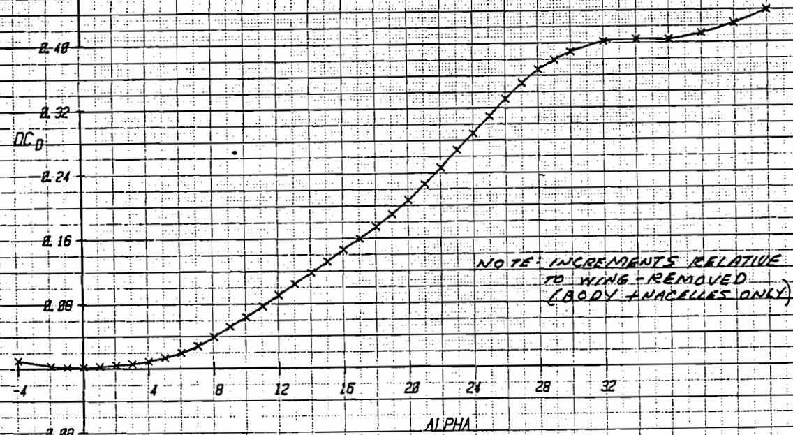
Figure 1-13 Lift, Drag, and Pitching Moment Increments for E205 Wing-Alone, M = .2
