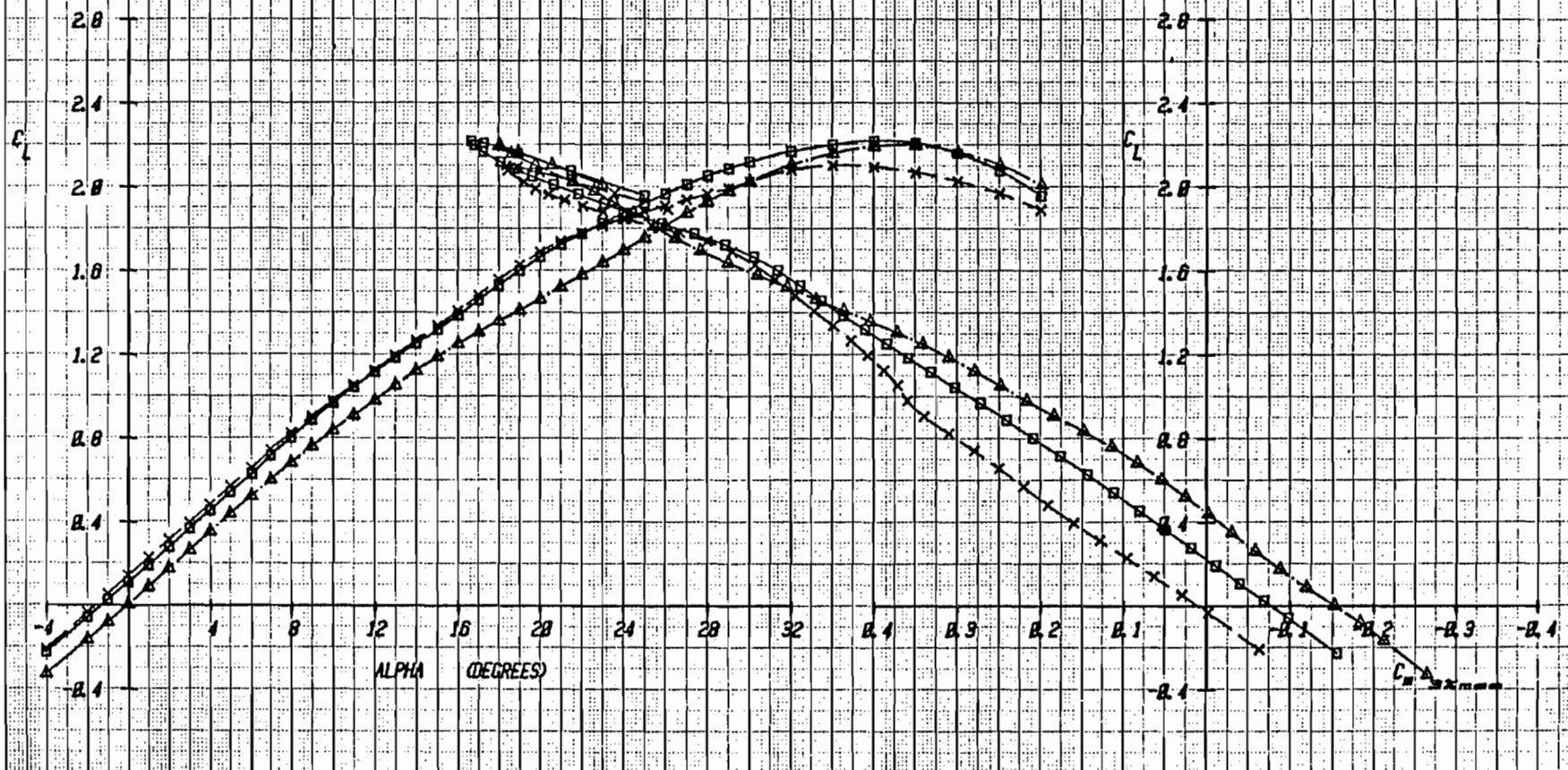
Figure 2-2a Effect of Canard Deflection on Lift and Moment with Forward Canard Longitudinal Location, C_2 , and Baseline Strake, S_1 , Mach = .2
