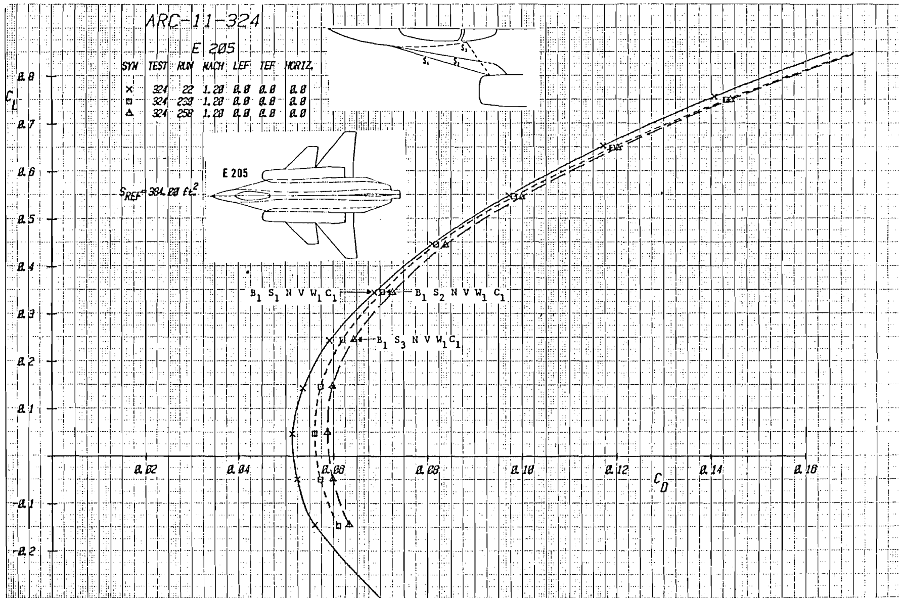
Figure 3-44b Effect of Strake Shape on Drag with Canard C_1 Undelected, Mach = 1.2
