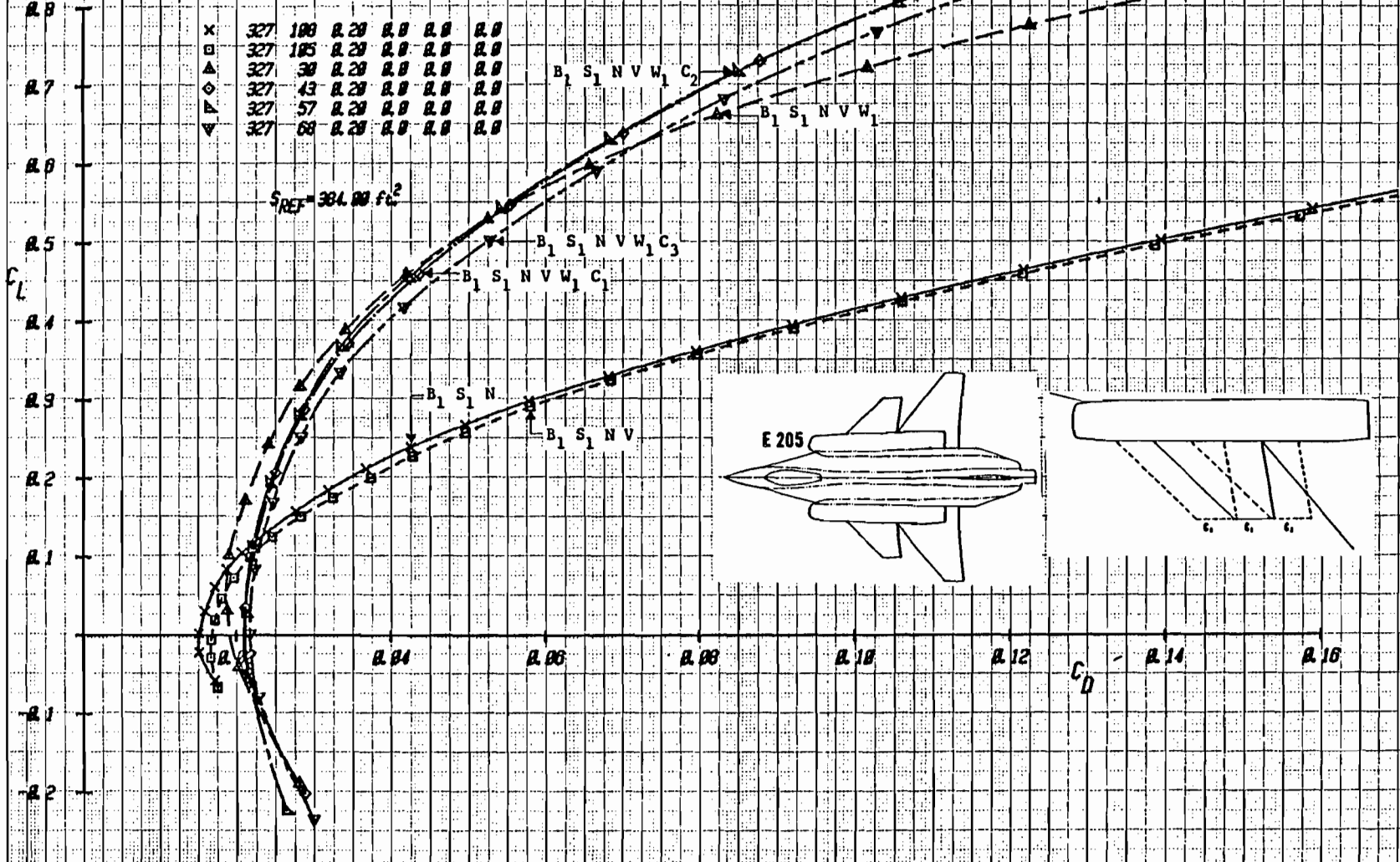
Figure 1-b Effect of Component Buildup on Drag, (Expanded Drag Scale), Mach = .2
