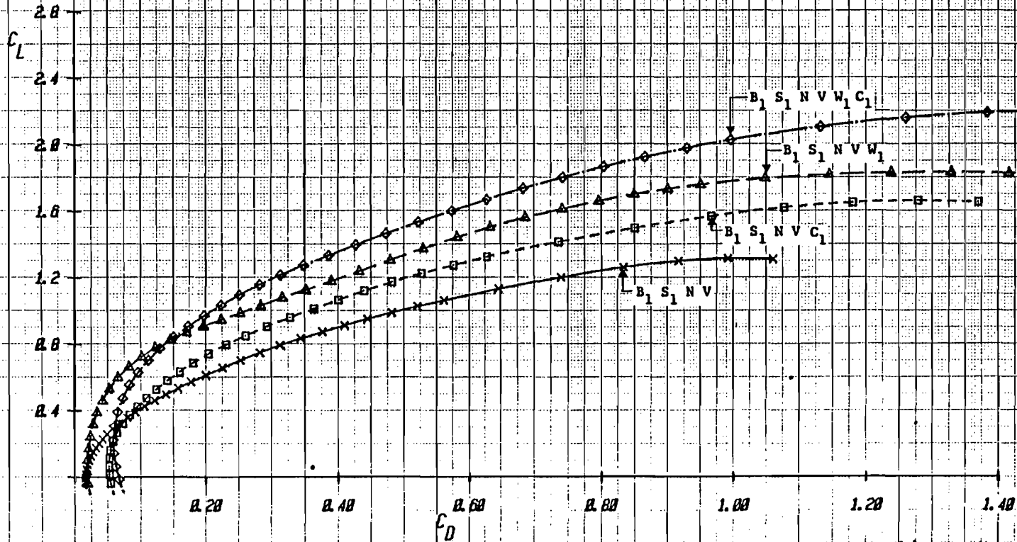
Figure 1-4c Drag Interference Data for E205 Configuration, \delta_c = -20^\circ , Mach = .2
