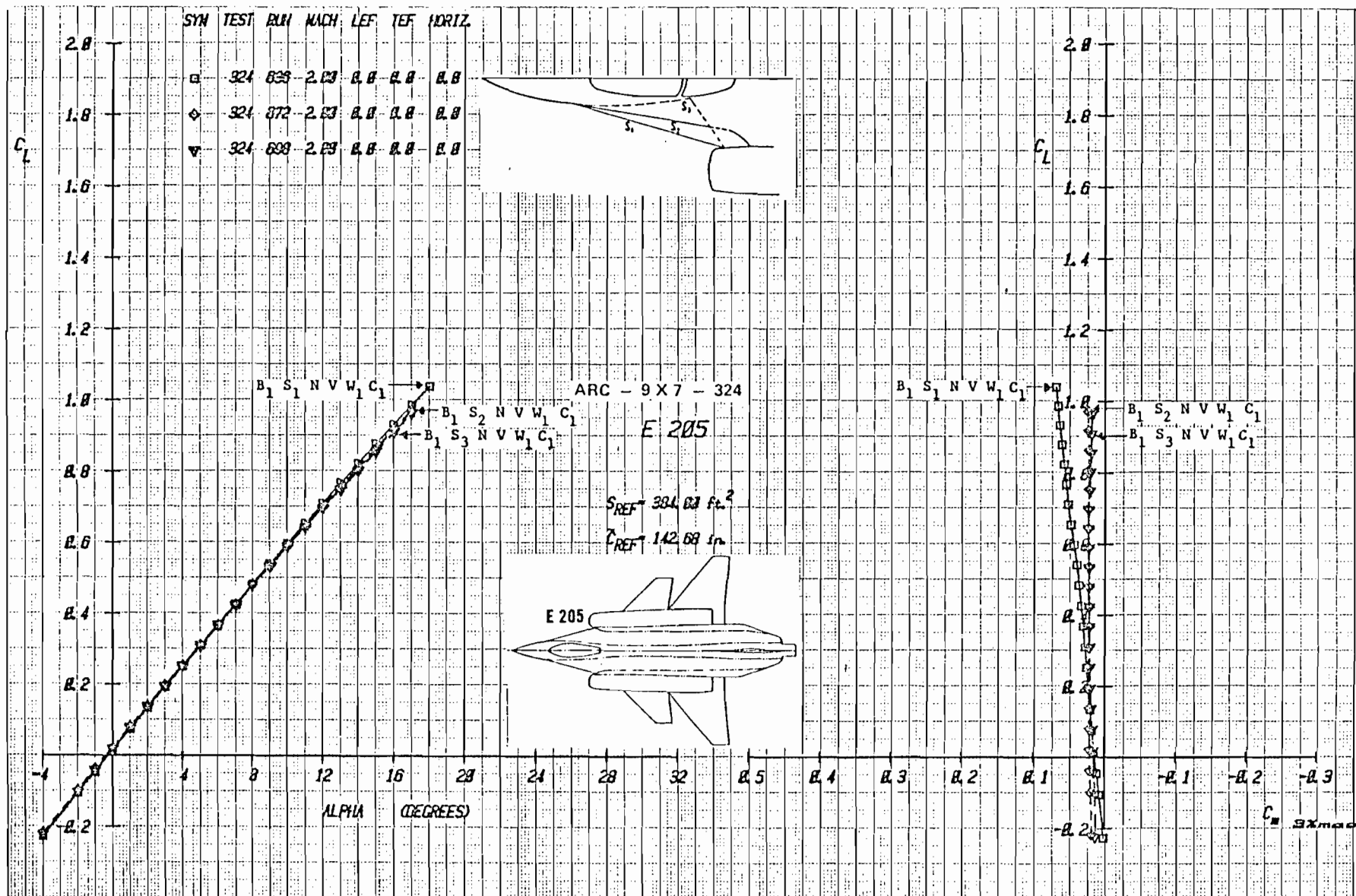
Figure 3-63a Effect of Strake Variation on Lift and Moment with Baseline Canard Longitudinal Location, C_1 , and \delta i = 0^\circ , Mach = 2.0
