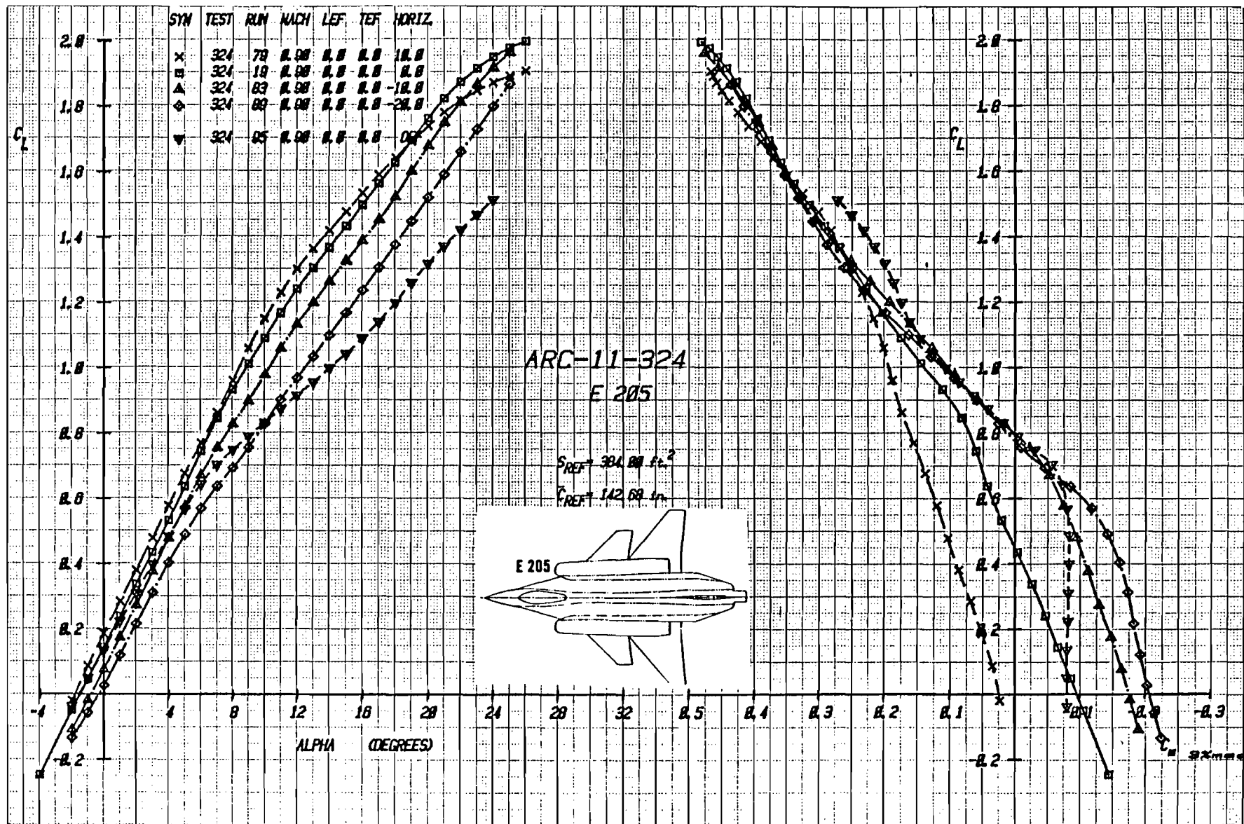
Figure 2-7a Effect of Canard Deflection on Lift and Moment With Wing Trailing-Edge Flap Undelected, Mach = .9
