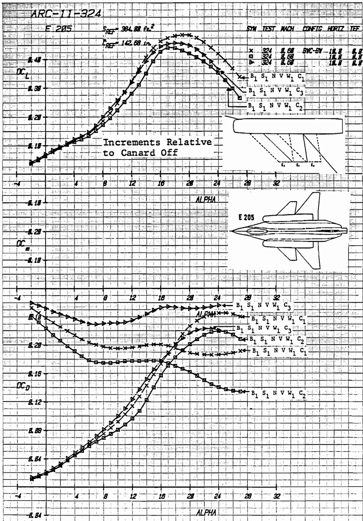
Figure 2-23 Incremental Effects of Canard Longitudinal Location on Canard Effectiveness at \delta_i = 10^\circ . Mach = .6
