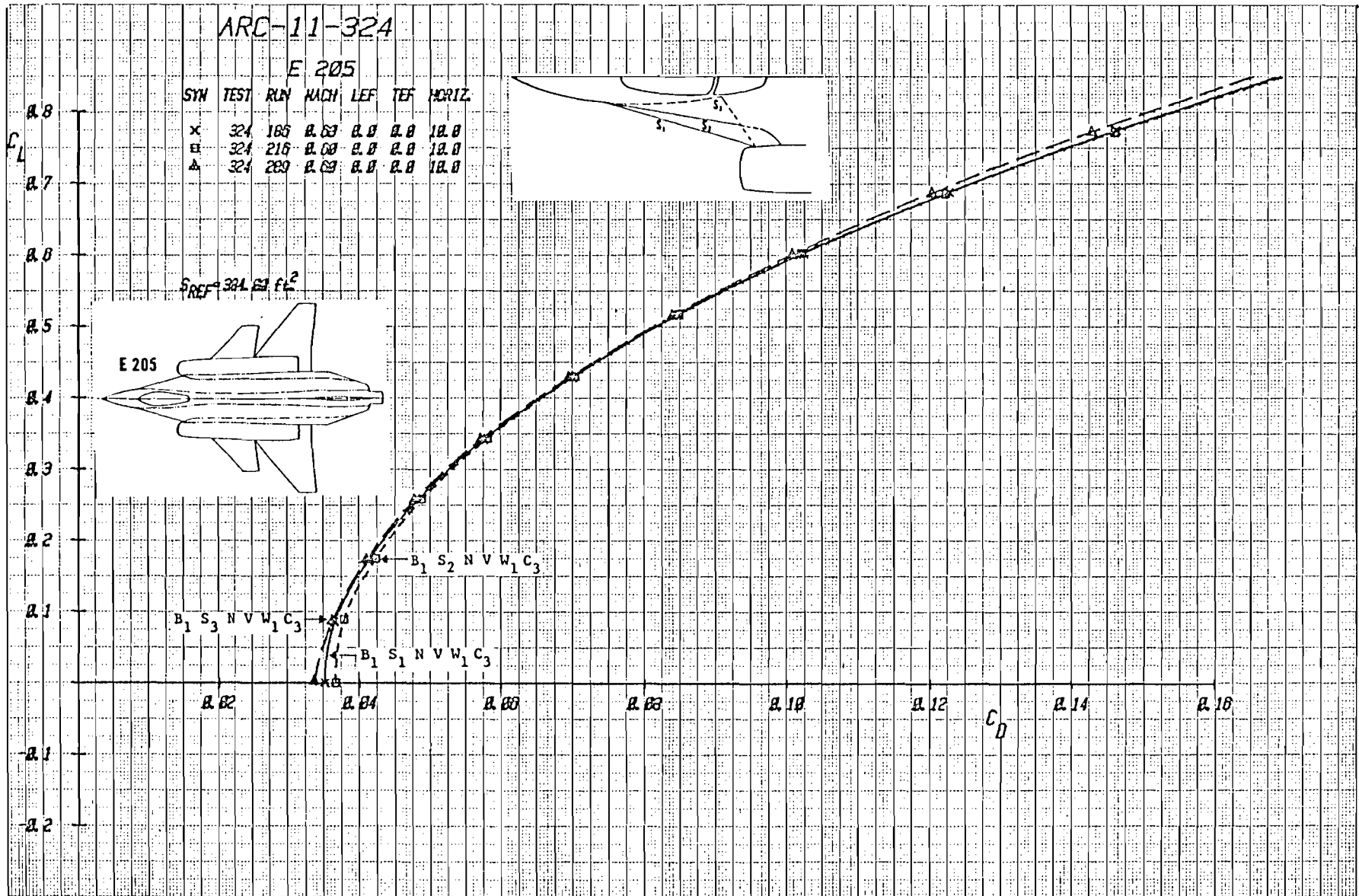
Figure 3-19b Effect of Strake Shape on Drag with Canard C_3 Deflected +10^\circ , Mach = .6
