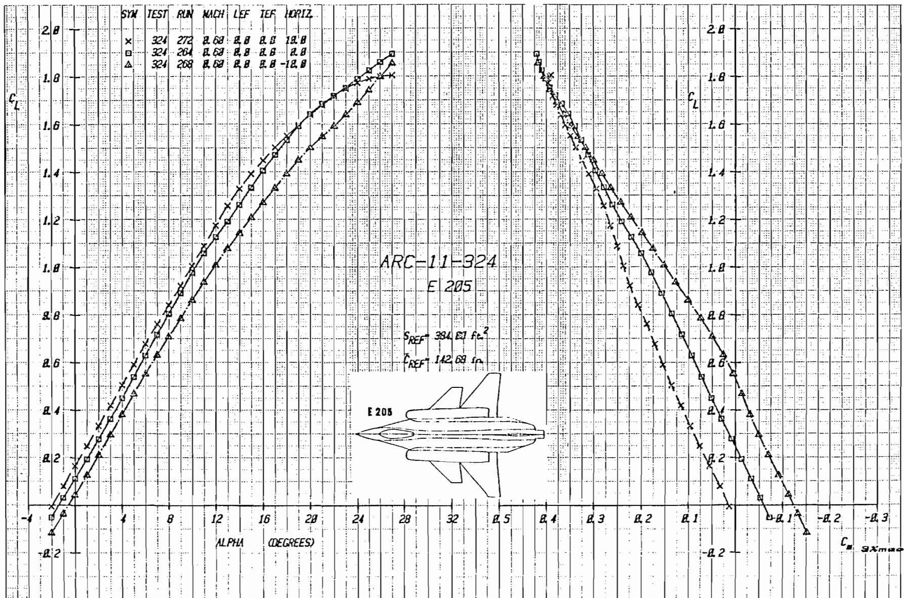
Figure 3-25a Effect of Canard Deflection on Lift and Moment with Canard C_1 , and Stroke S_3 , Mach = .6
