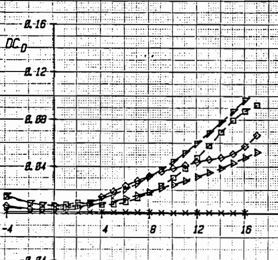
Figure 1-19 Lift, Drag, and Pitching Moment Increments for E205 Vertical Tail (Wing and Canard Removed), Wing (In Presence of Canard), Canard (In Presence of Wing), Canard (Wing Removed), Wing (Canard Removed), M = 1.8
