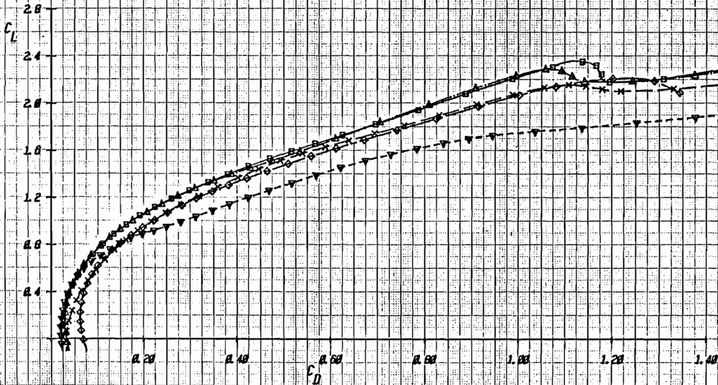
Figure 2-5c Effect of Canard Deflection on Drag with Wing Trailing-Edge Flap Undelected, Mach = .4
