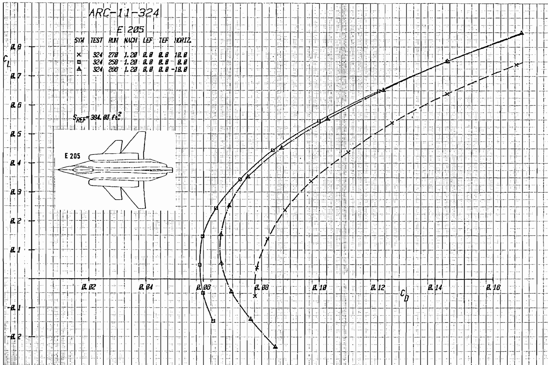
Figure 3-55b Effect of Canard Deflection on Drag with Canard C_1 , and Strake S_3 , Mach = 1.2
