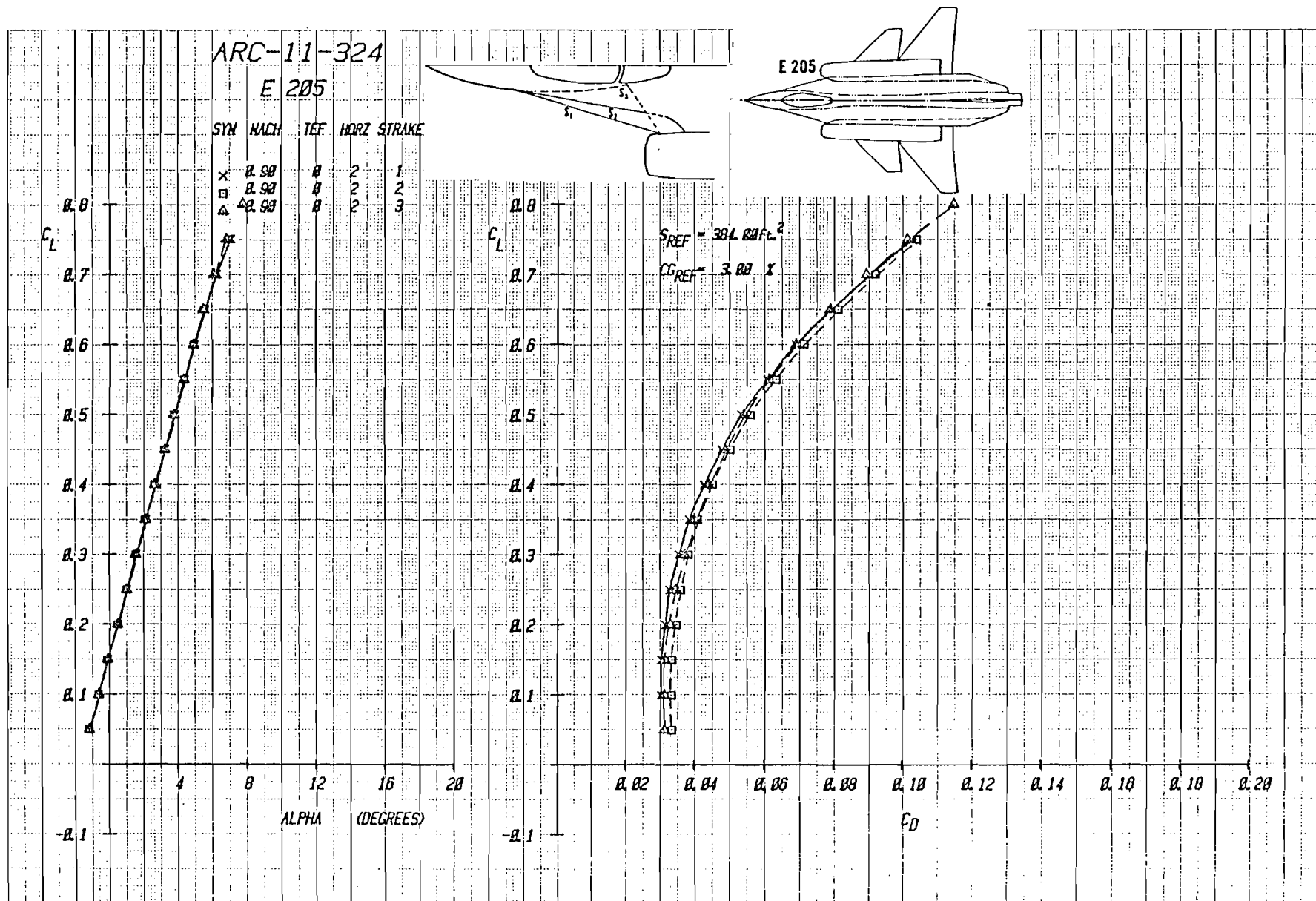
Figure 3-82 Trimmed Lift and Drag With Variations in Strake and Canard C_2 , Mach = .9
