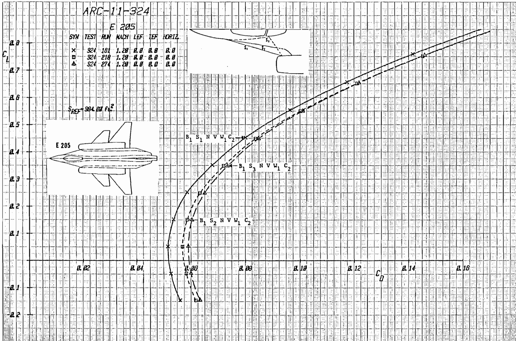
Figure 3-47b Effect of Strake Shape on Drag with Canard C_2 Undelected, Mach = 1.2
