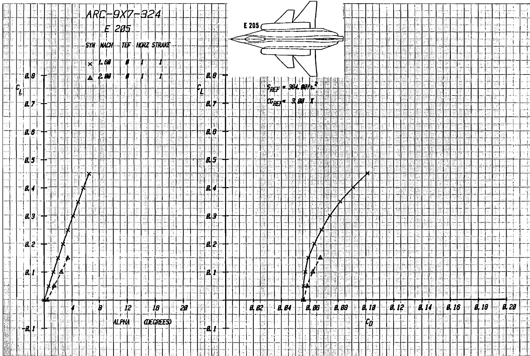
Figure 2-42 Trimmed Lift and Drag for Baseline E205 Configuration with Wing Trailing-Edge Flap Undelected
