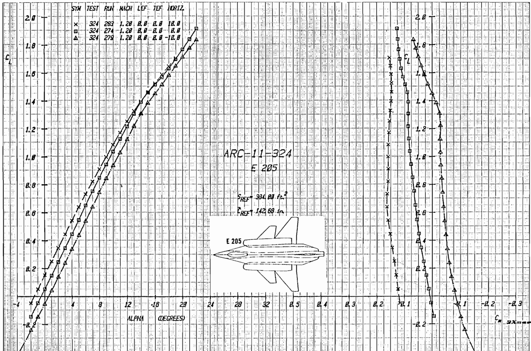
Figure 3-56a Effect of Canard Deflection on Lift and Moment with Canard C_2 , and Strike S_3 , Mach = 1.2
