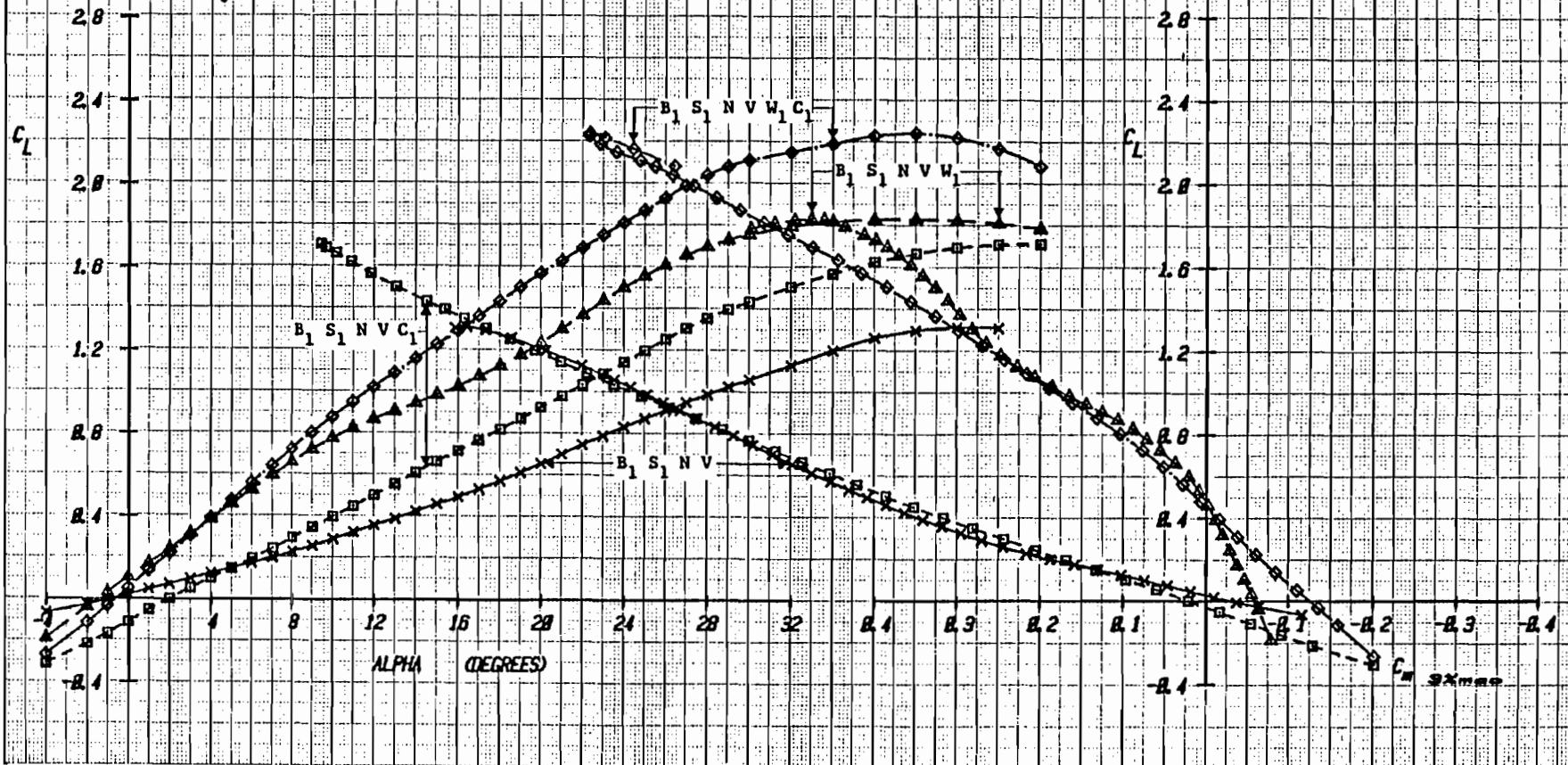
Figurel-3a Lift and Moment Inteferece Data for E205 Configuration, \delta_c = -10^\circ , Mach = .2
