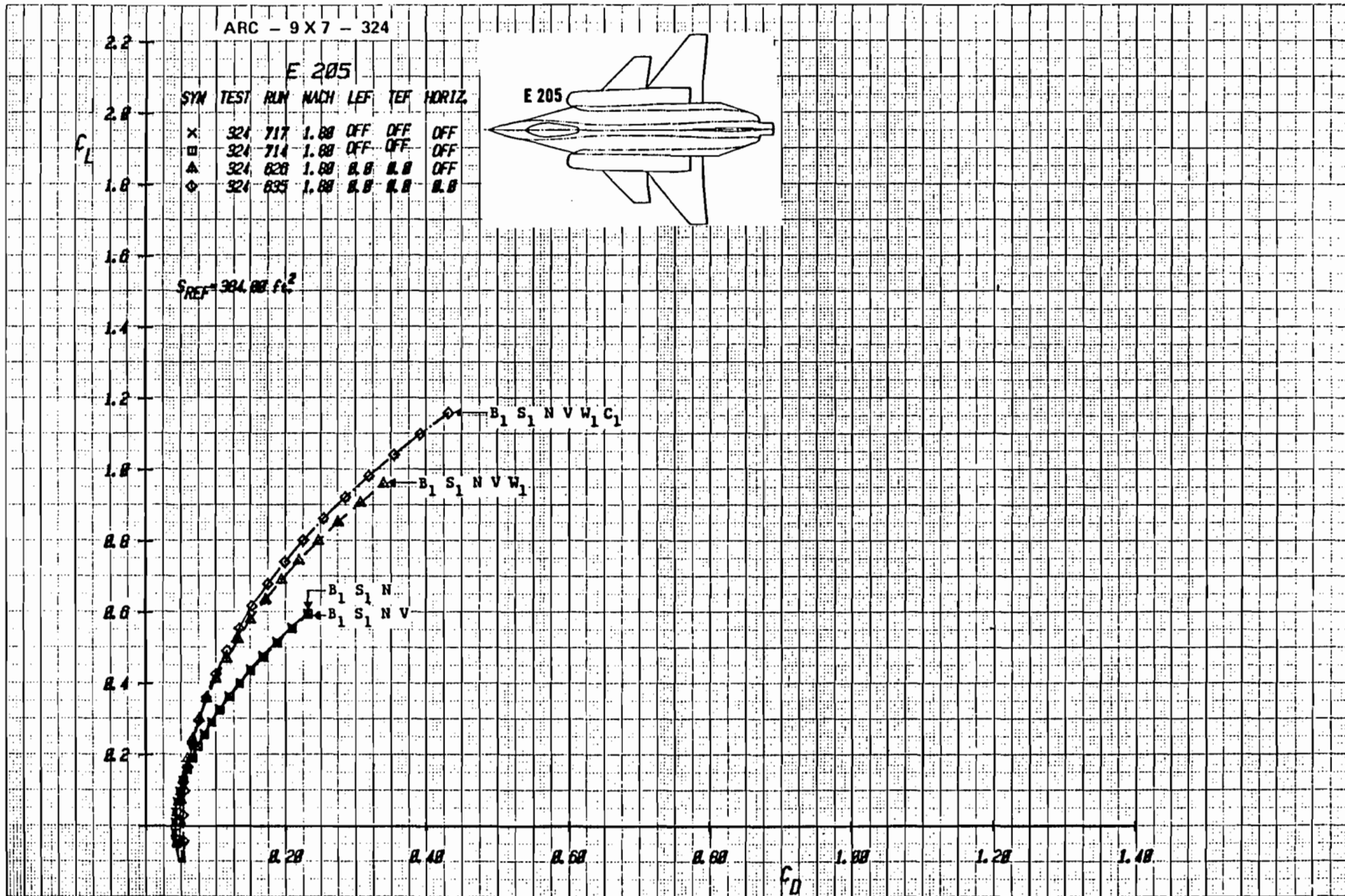
Figure 10c Effect of Component Buildup on Drag, Mach = 1.8
