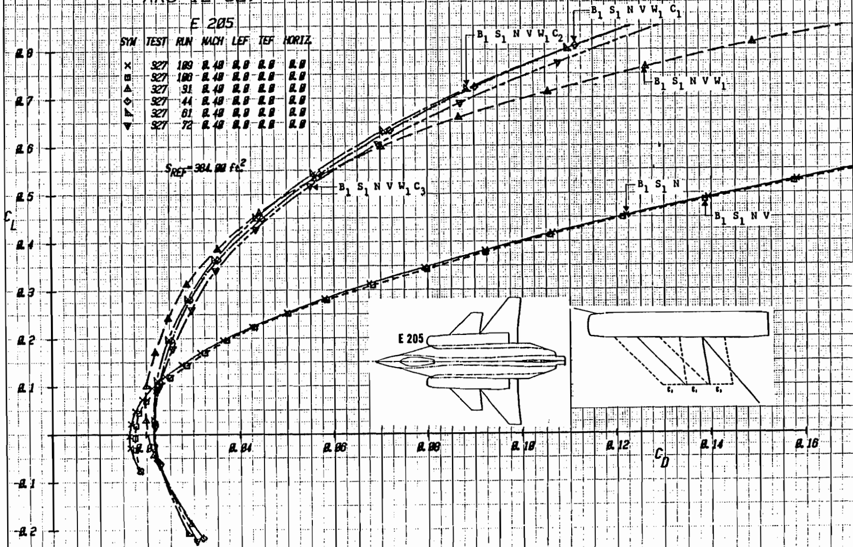
Figure 1-5b Effect of Component Buildup on Drag, (Expanded Drag Scale), Mach = .4
