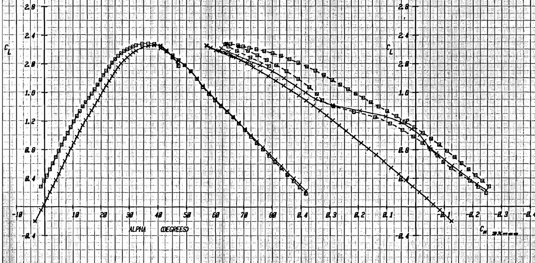
Figure 2-34a Effect of Wing Trailing-Edge Flap Deflection on E205 Baseline Lift and Pitching Moment ( \alpha = 0^\circ to 90^\circ ), M = .2 , \delta c = 0^\circ
