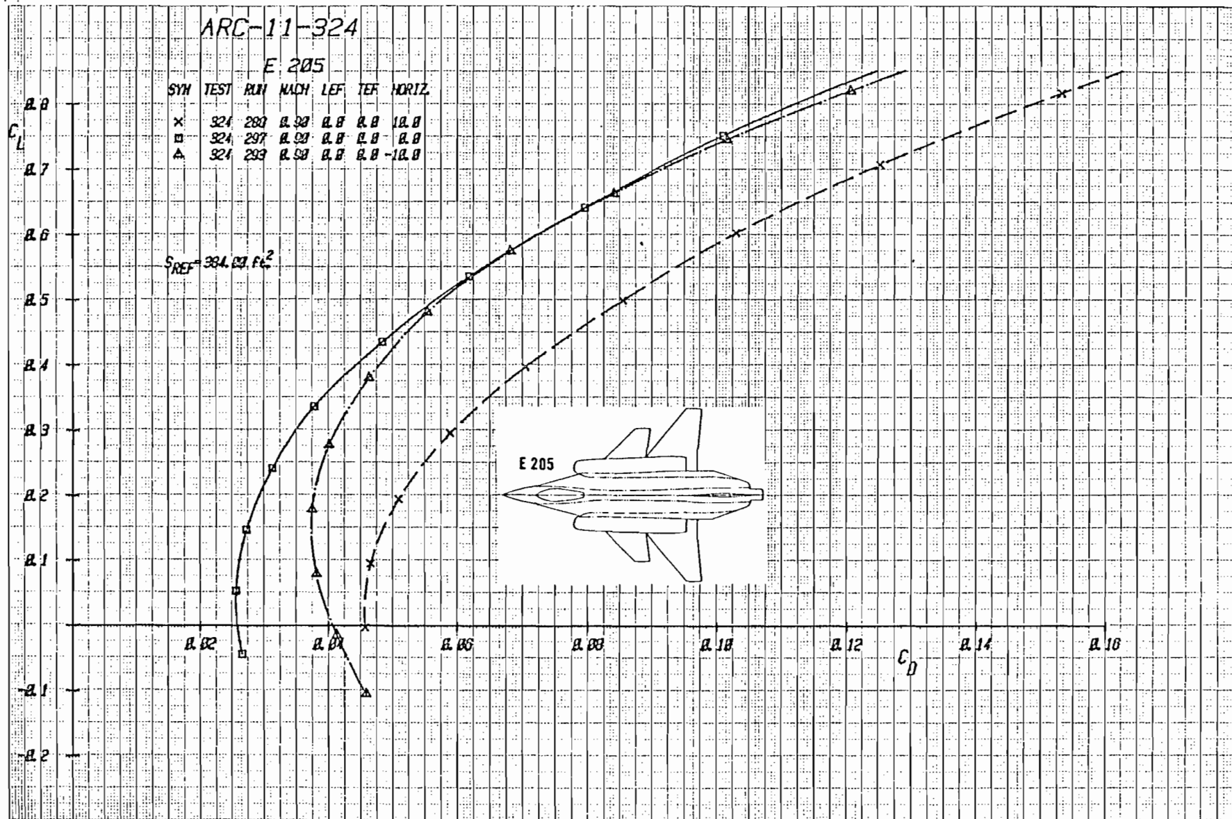
Figure 3-42b Effect of Canard Deflection on Drag with Canard C_3 , and Strake S_3 , Mach = 0.9
