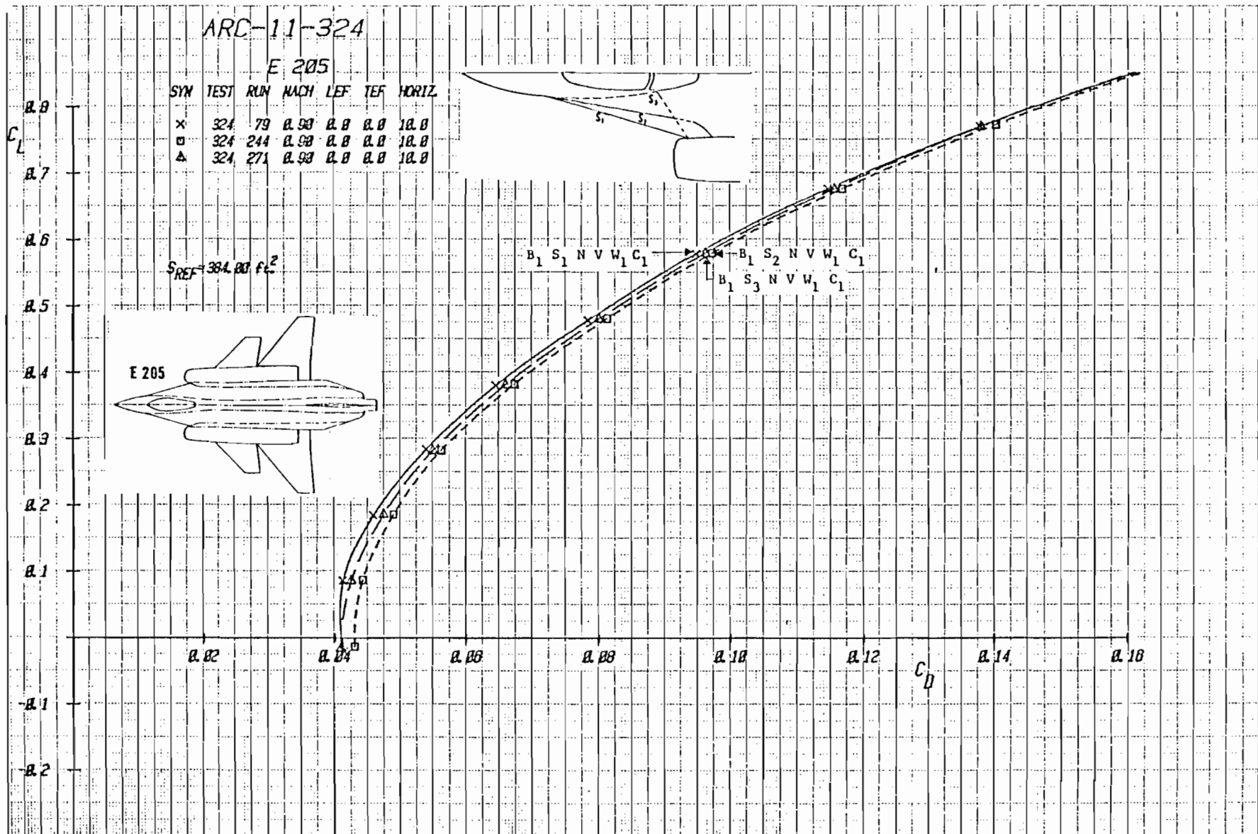
Figure 3-28b Effect of Strake Shape on Drag with Canard C_1 Deflected +10^\circ , Mach = .9
