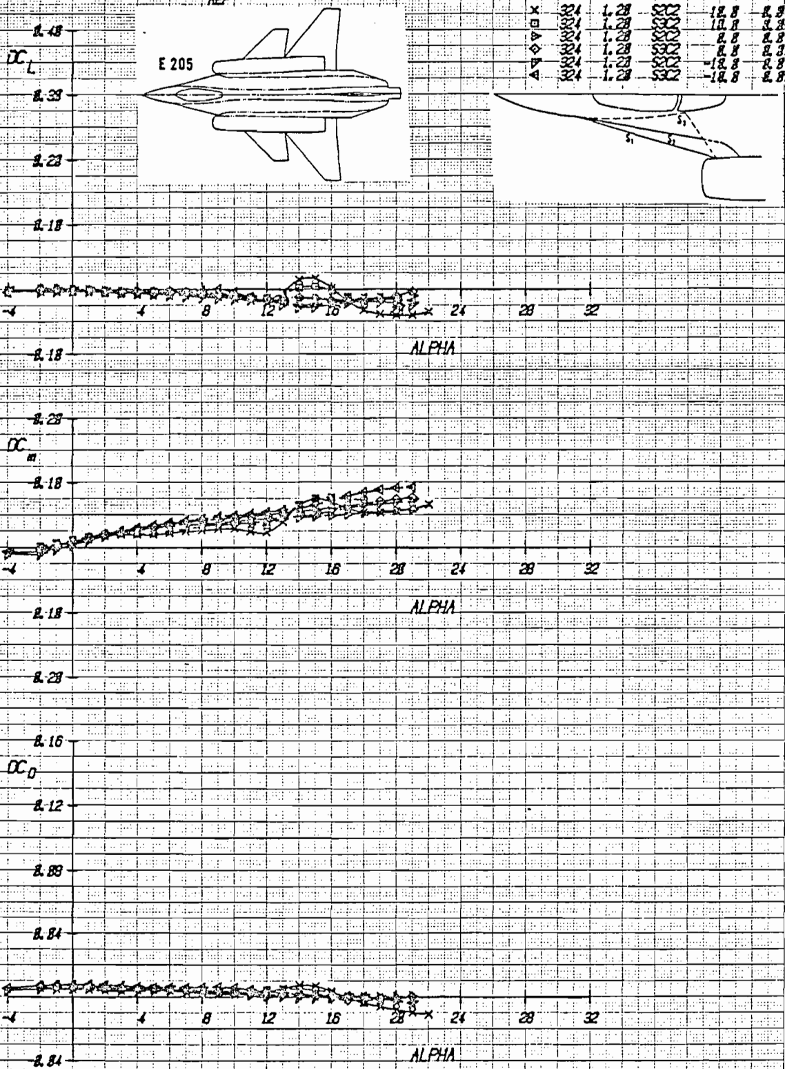
Figure 3-75 Incremental Effects of Strake Shape with Canard C_2 at Various Deflections, Mach = 1.2
