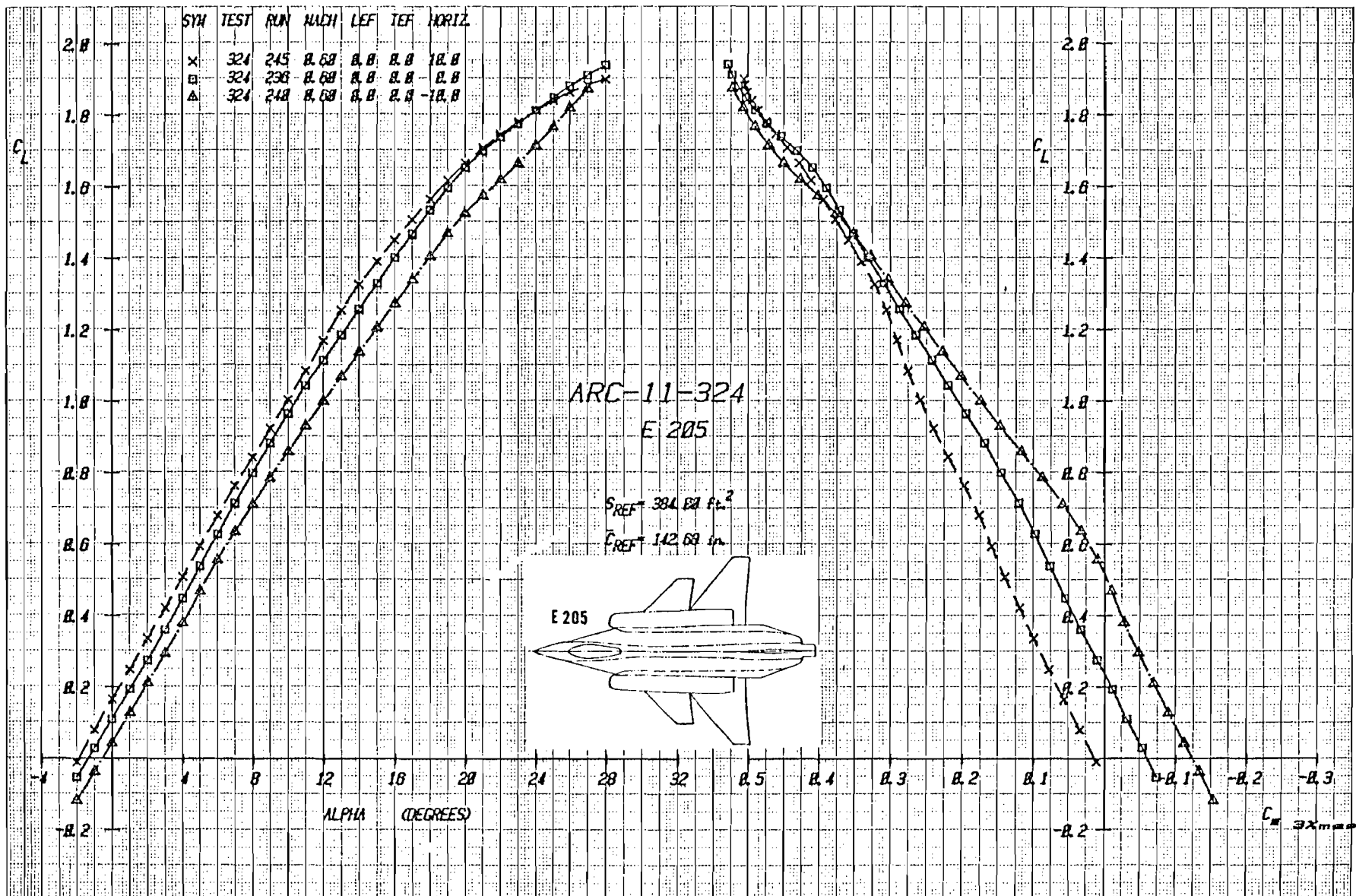
Figure 3-22a Effect of Canard Deflection on Lift and Moment With Canard, C_L , and Strike S_2 , Mach = .6
