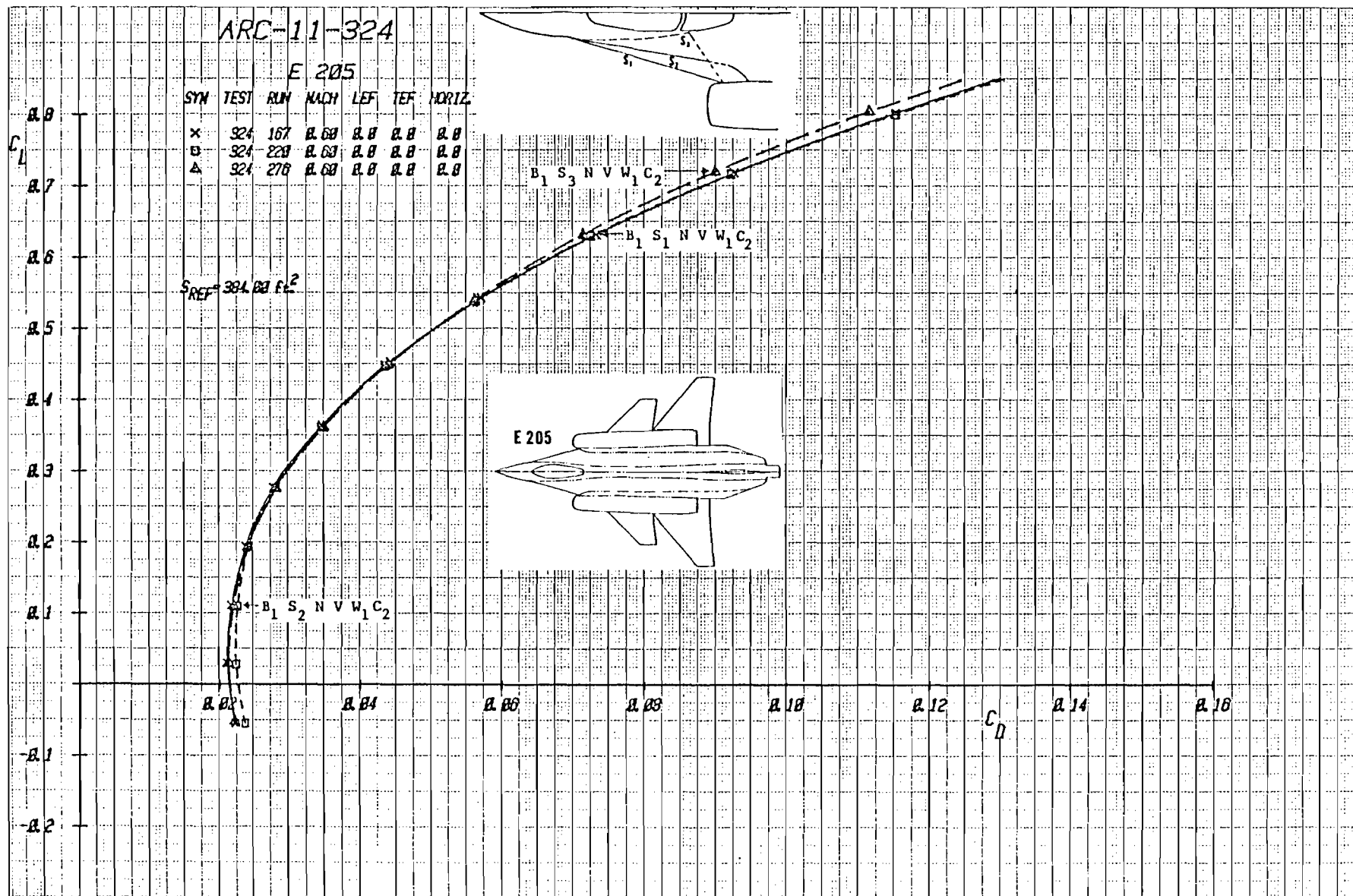
Figure 3-17b Effect of Strake Shape on Drag with Canard C_2 Undelected, Mach = .6
