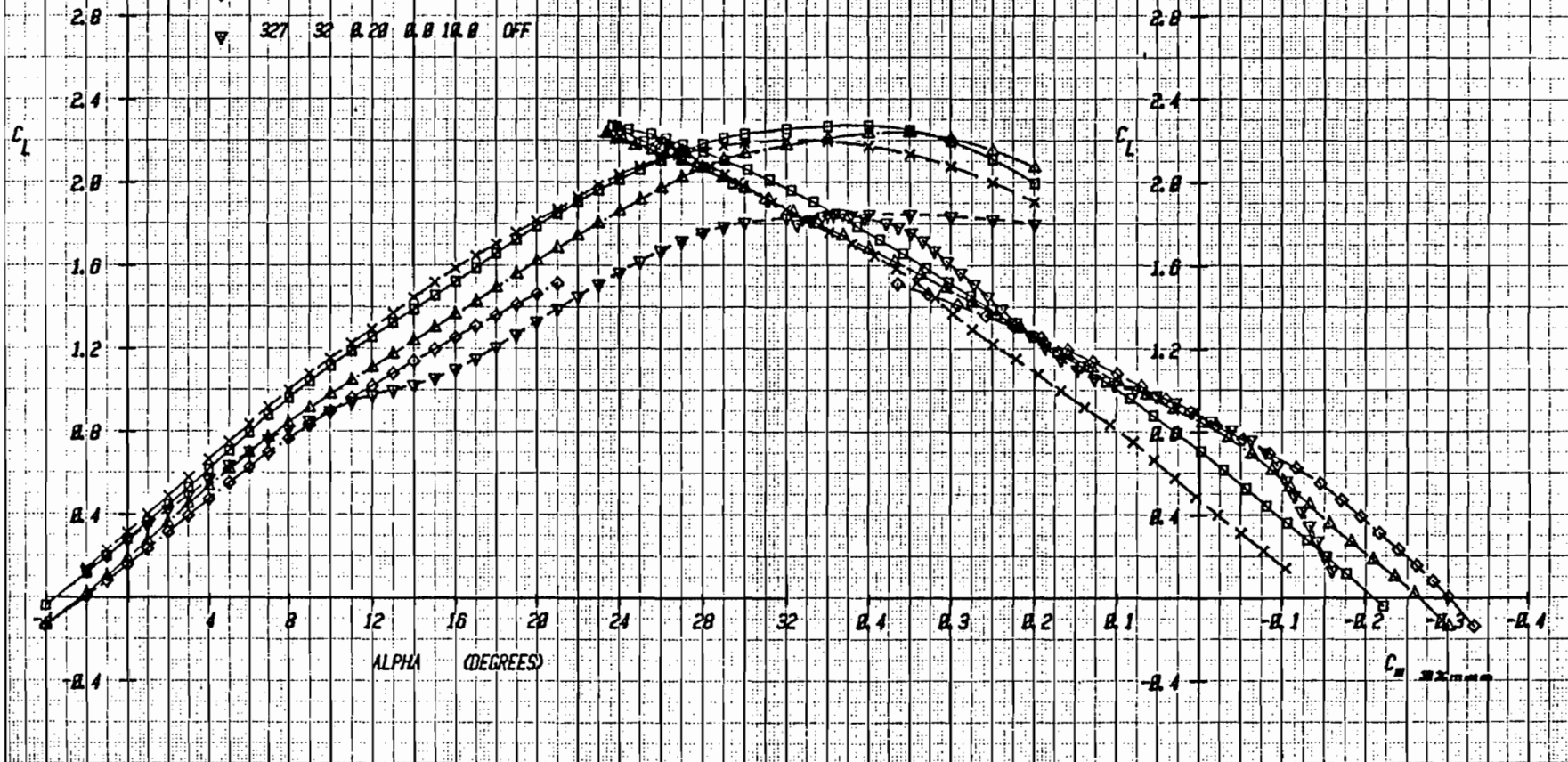
Figure 2-32a Effect of Canard Deflection on Lift and Moment with Wing Trailing-Edge Flap Deflected +10°, Mach = .2
