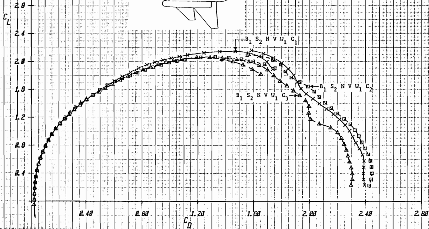
Figure 3-8h Effect of Canard Location with Strake S_2 , on E205 Drag ( \alpha = 0^\circ to 90^\circ ), \delta_c = 0^\circ , M = .2
