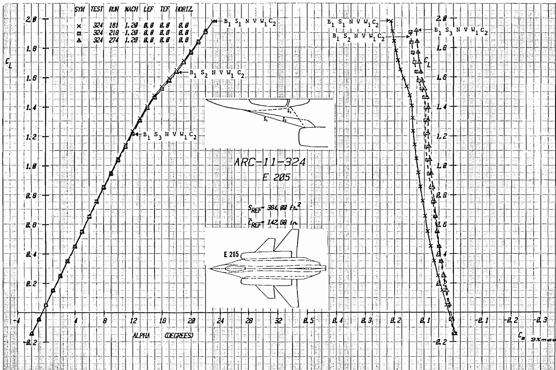
Figure 3-47a Effect of Strake Shape on Lift and Moment with Canard C_2 Undelected, Mach = 1.2
