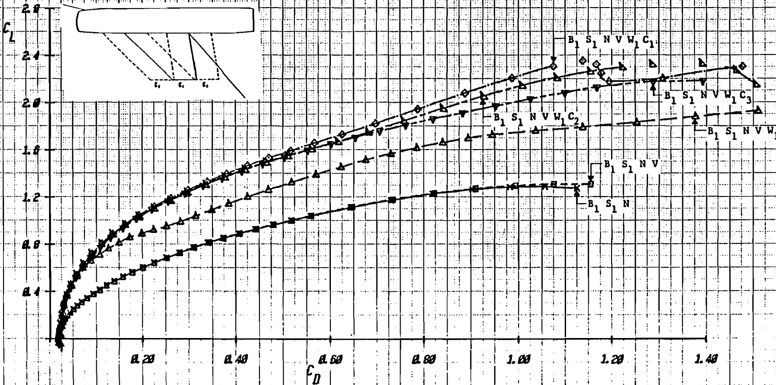
Figure 1-5c Effect of Component Buildup on Drag, Mach = .4
