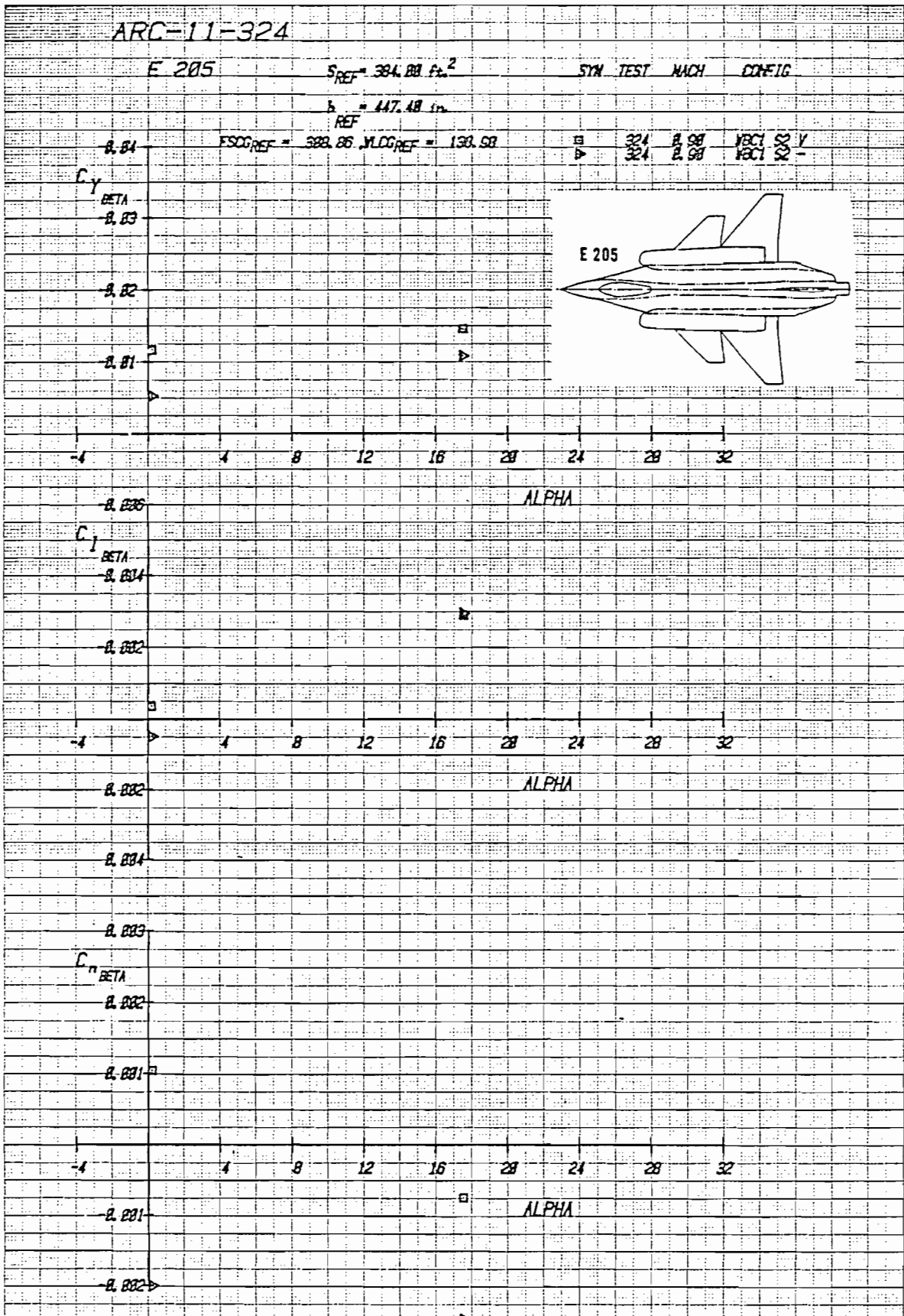
Figure 3-94 Vertical Tail Effectiveness for the E205 Configuration, with Strake S_2 , Canard C_1 , Mach = .9
