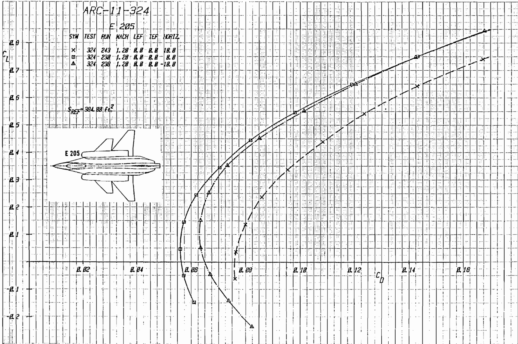
Figure 3-52b Effect of Canard Deflection on Drag With Canard C_1 , and Strake S_2 , Mach = 1.2
