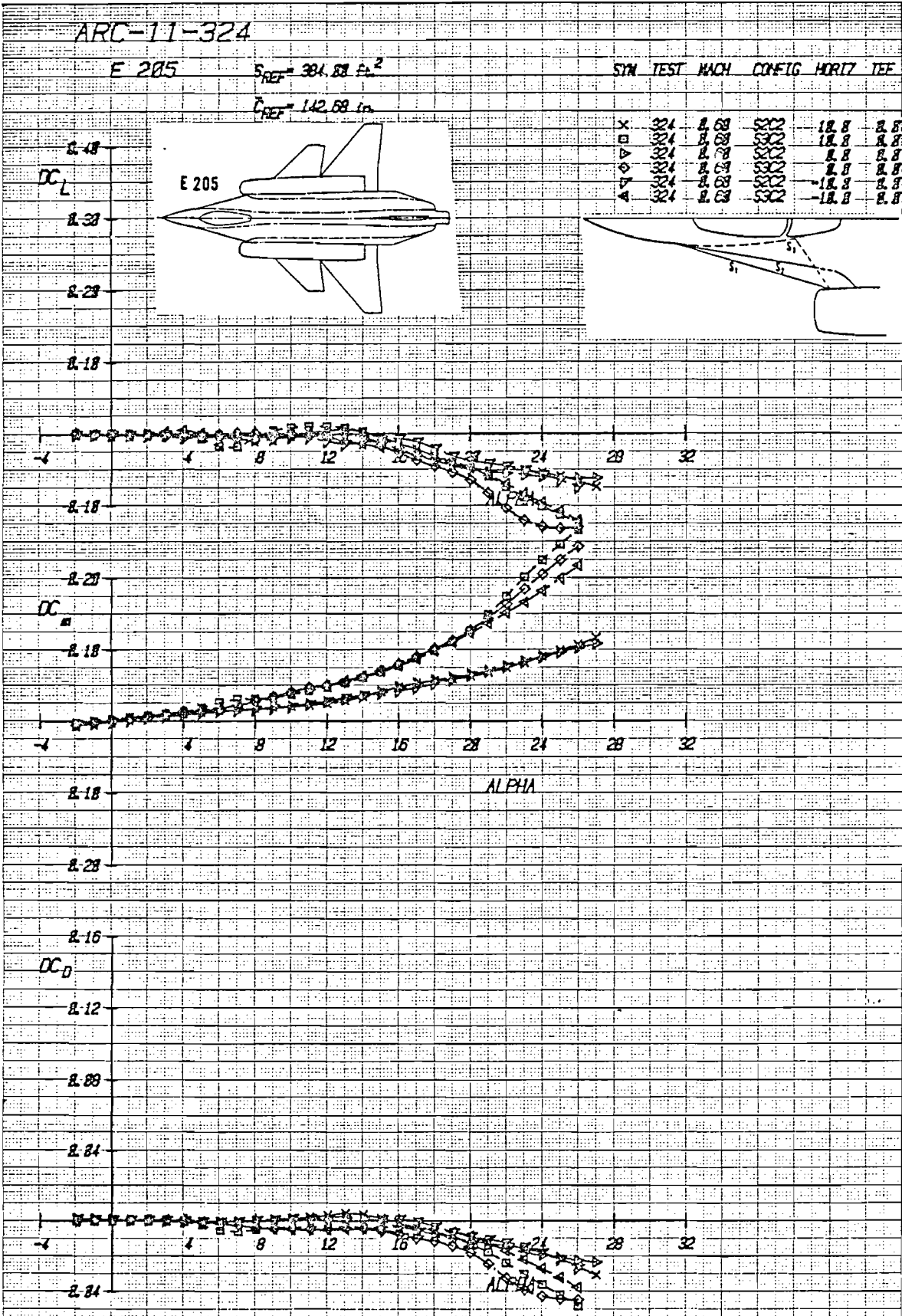
Figure 3-69 Incremental Effects of Strake Shape with Canard C_2 at Various Deflections, Mach = .6
