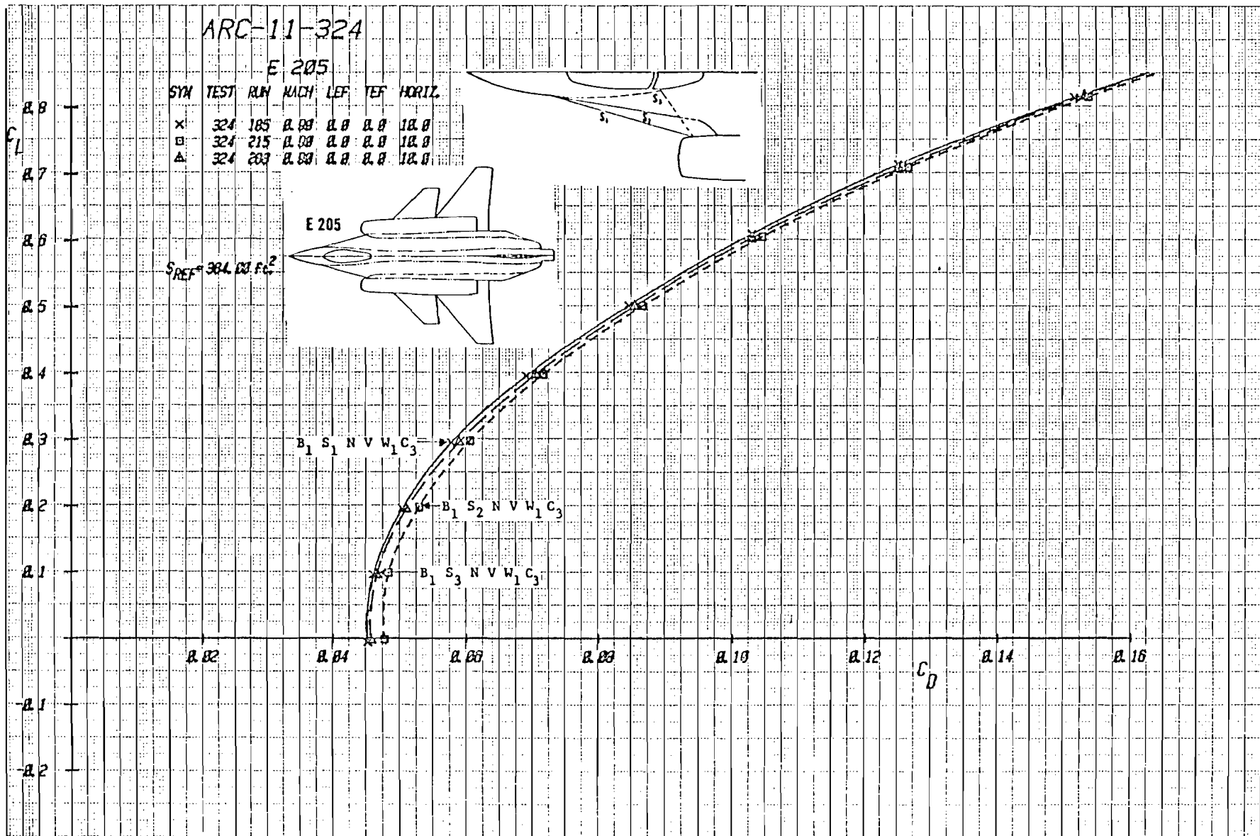
Figure 3-34b Effect of Strake Shape on Drag with Canard C_3 Deflected +10^\circ , Mach = .9
