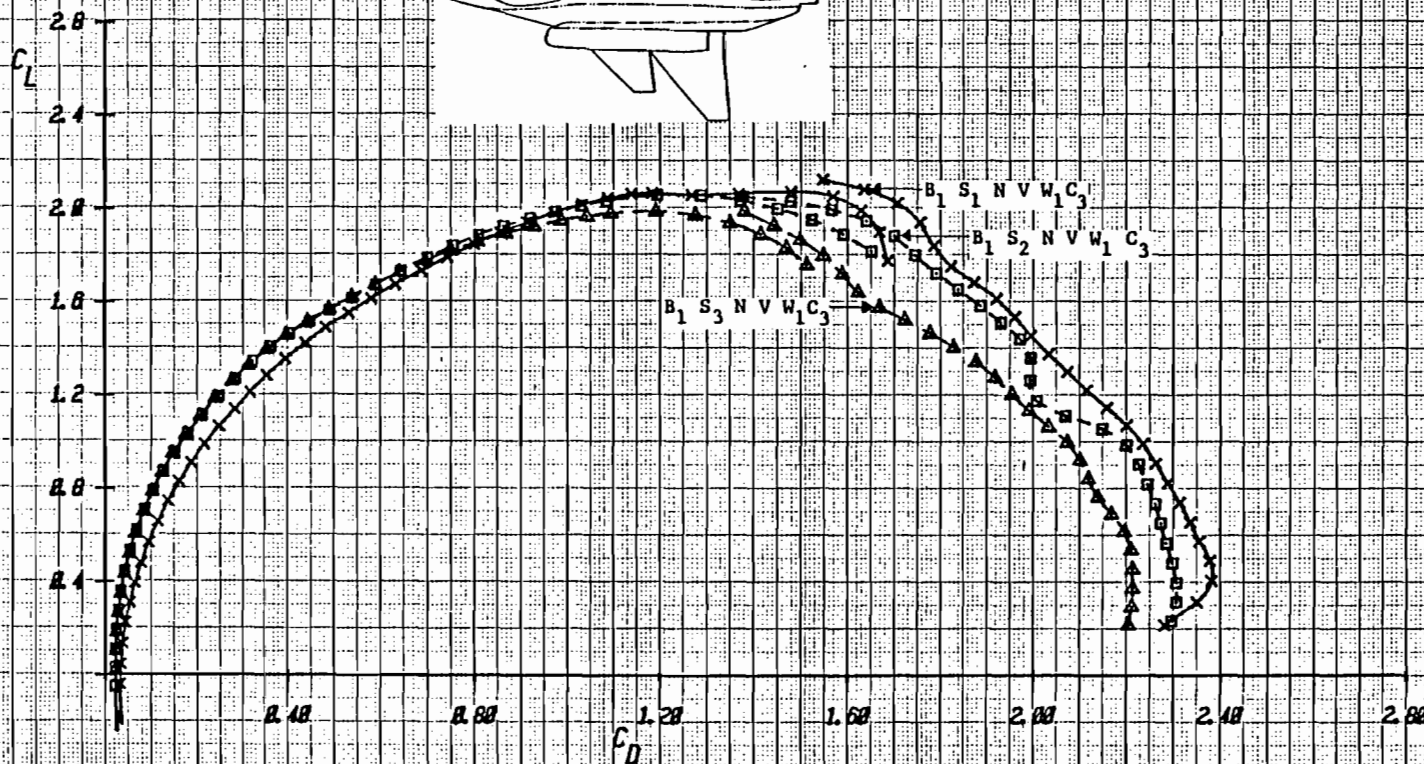
Figure 3-6b Effect of Strake Shape with Aft Canard Location, C_3 , on E205 Drag ( \alpha = 0^\circ to 90^\circ ), \delta_c = 0^\circ , M = .2
