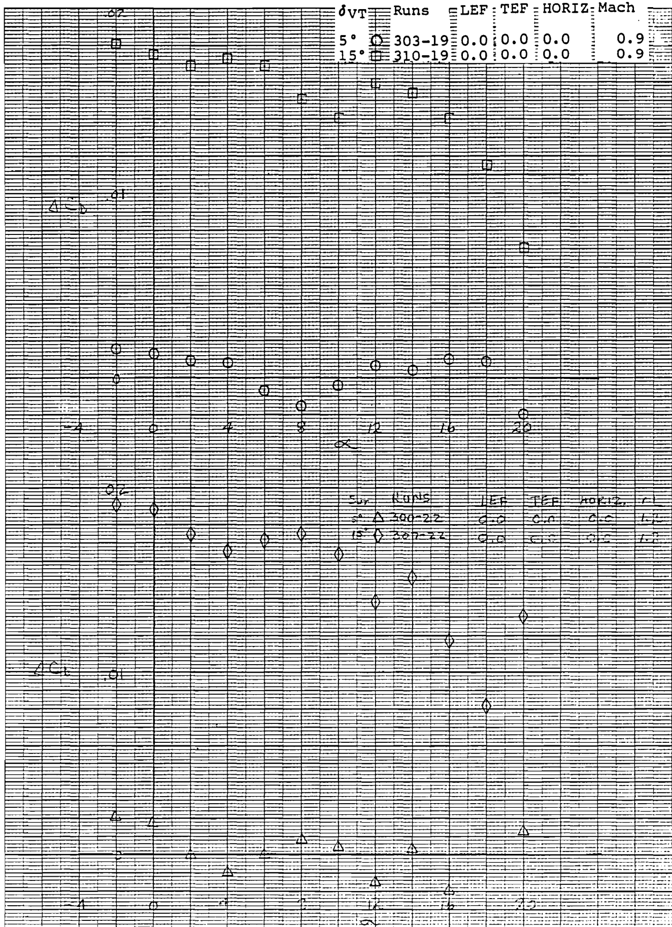
Figure 2-66 Incremental Effect of Vertical Tail Deflection on Drag, Mach = .9, Mach = 1.2
