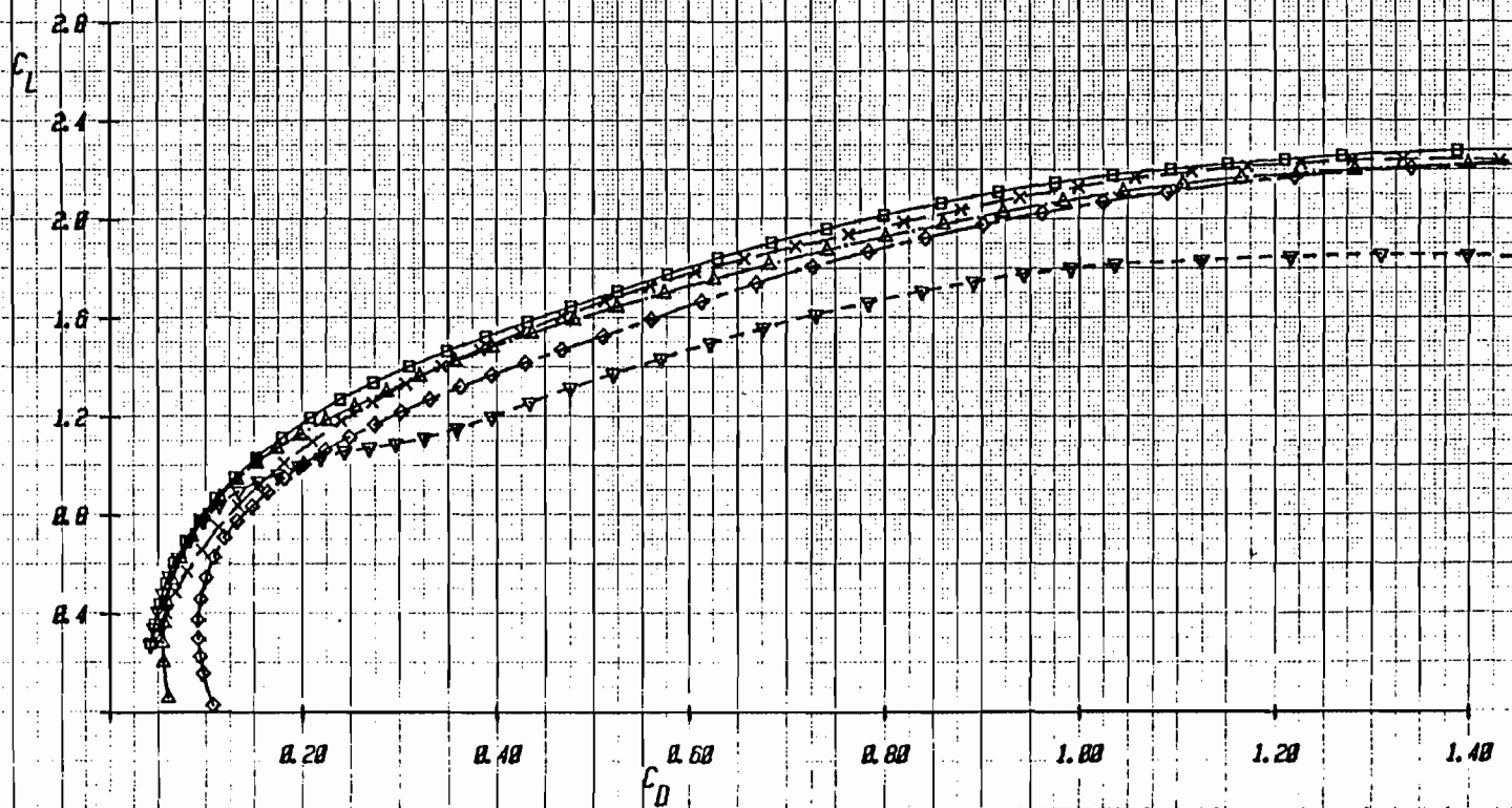
Figure 2-33c Effect of Canard Deflection on Drag with Wing Trailing-Edge Flap Deflected +25°, Mach = .2
