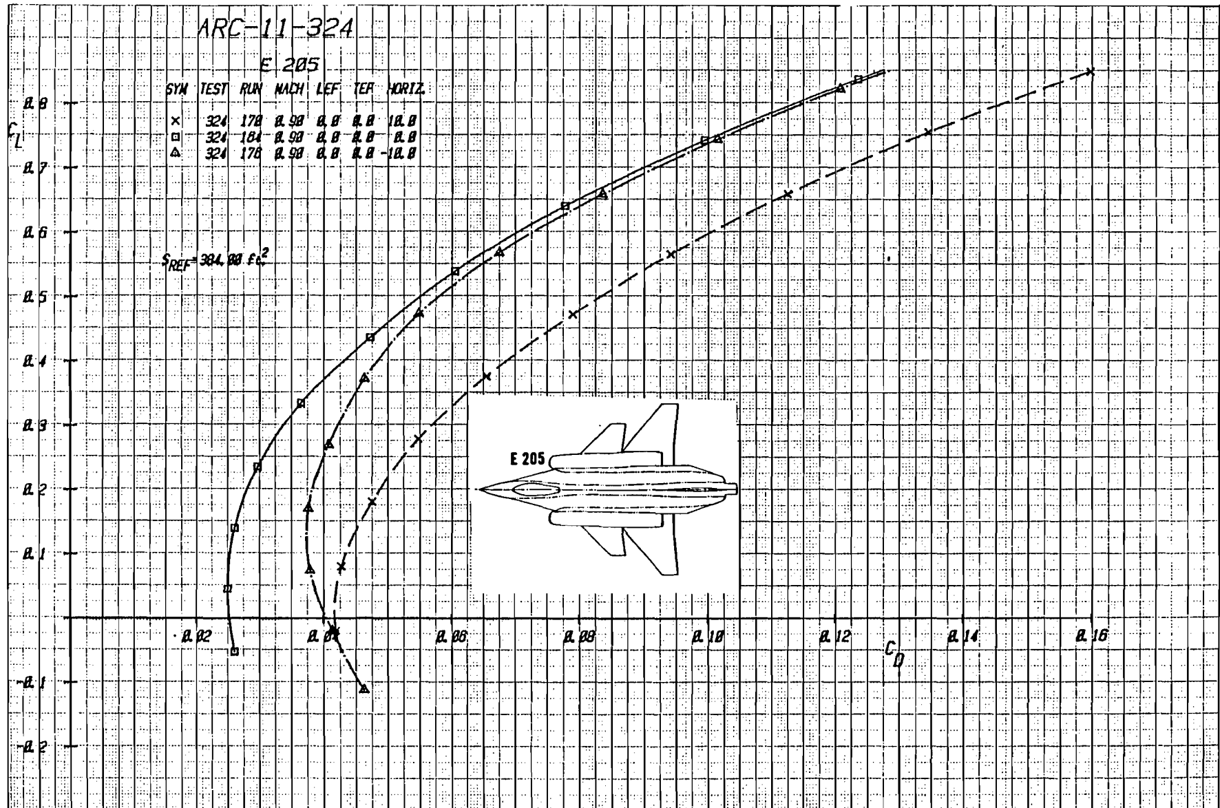
Figure 2-10b Effect of Canard Deflection on Drag with Forward Canard Longitudinal Location, C_2 , and Baseline Stroke, S_1 , Mach = .9
