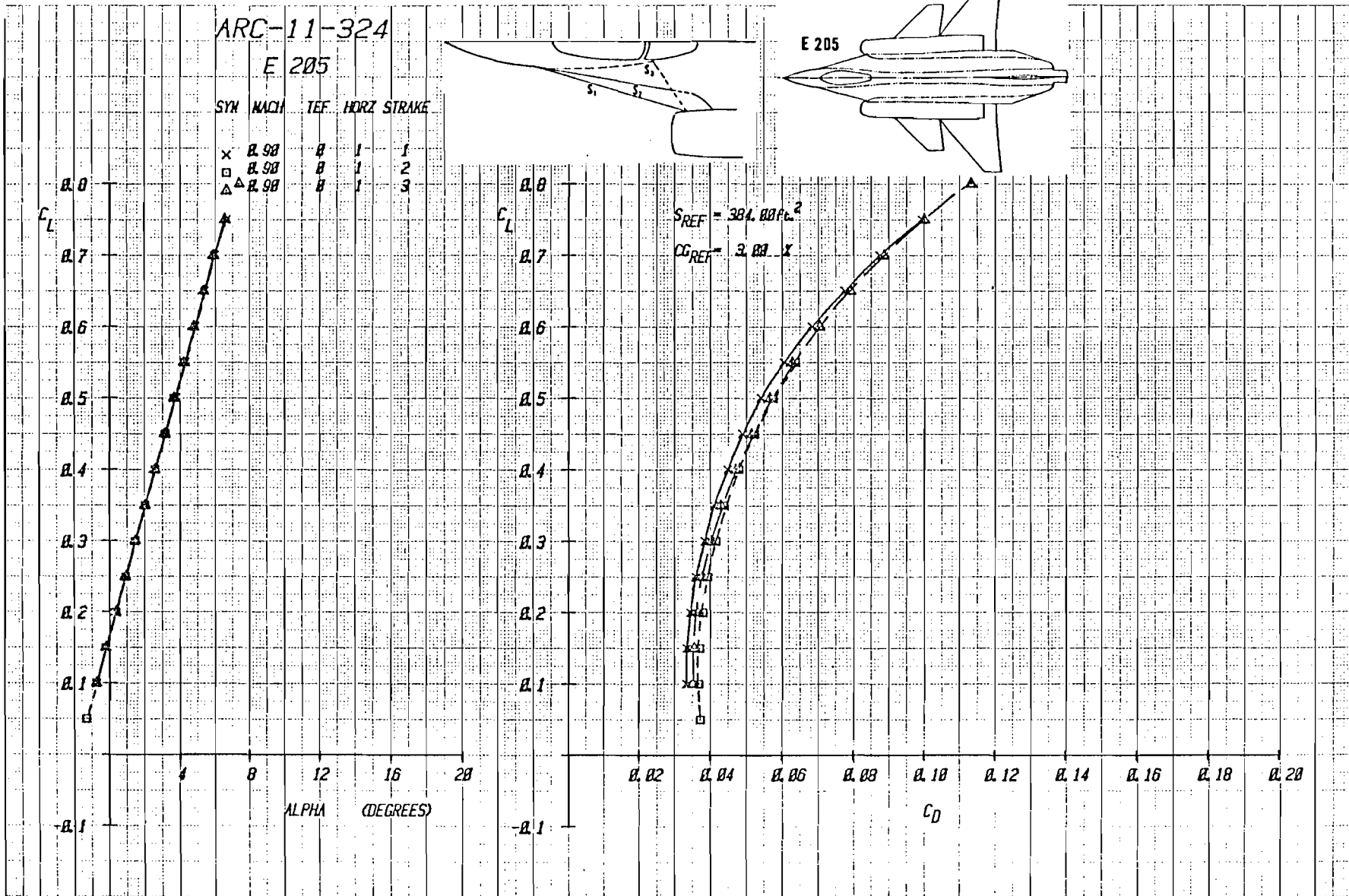
Figure 3-81 Trimmed Lift and Drag With Variations in Strake and Canard C_L , Mach = .9
