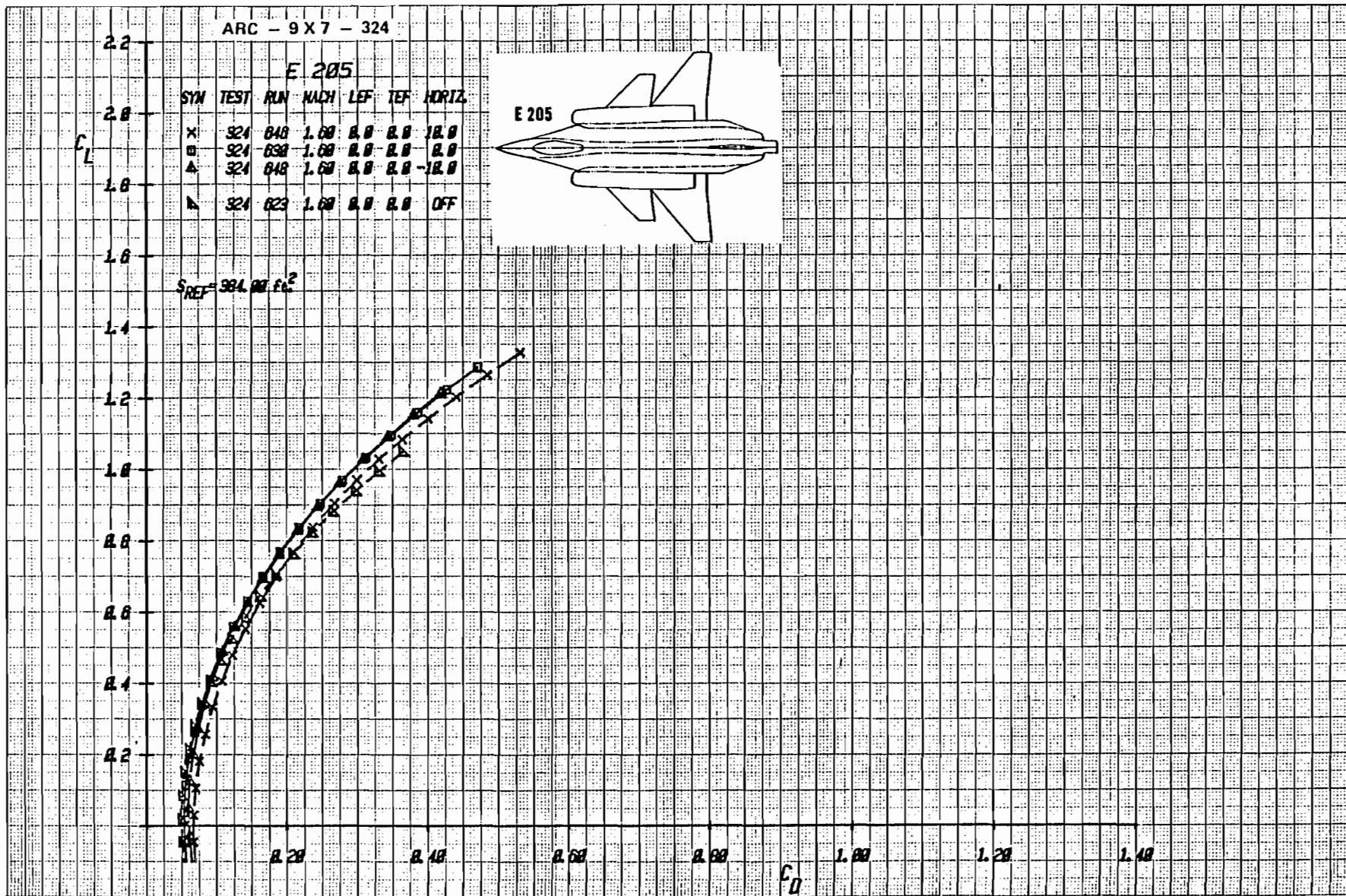
Figure 2-15c Effect of Canard Deflection on Drag With Wing Trailing-Edge Flap Undeflected, Mach = 1.6
