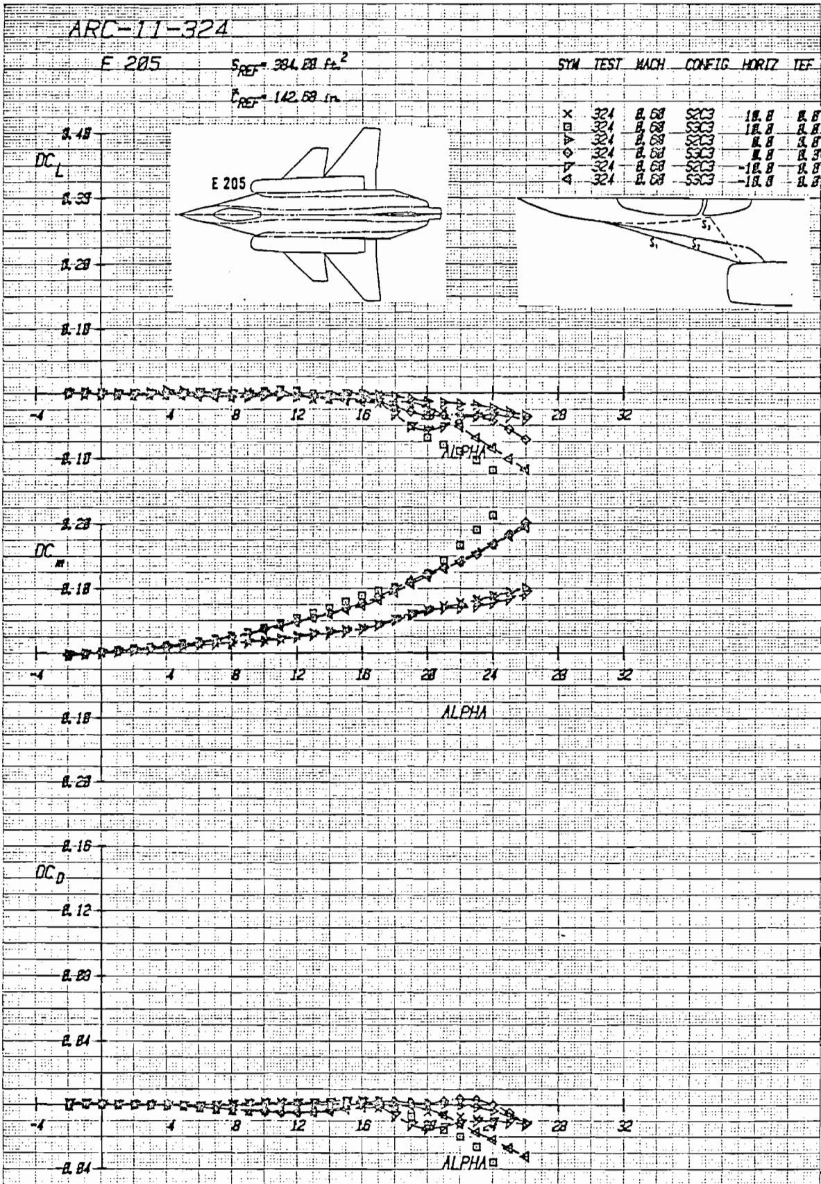
Figure 3-70 Incremental Effects of Strake Shape with Canard C 3 at Various Deflections, Mach = .6
