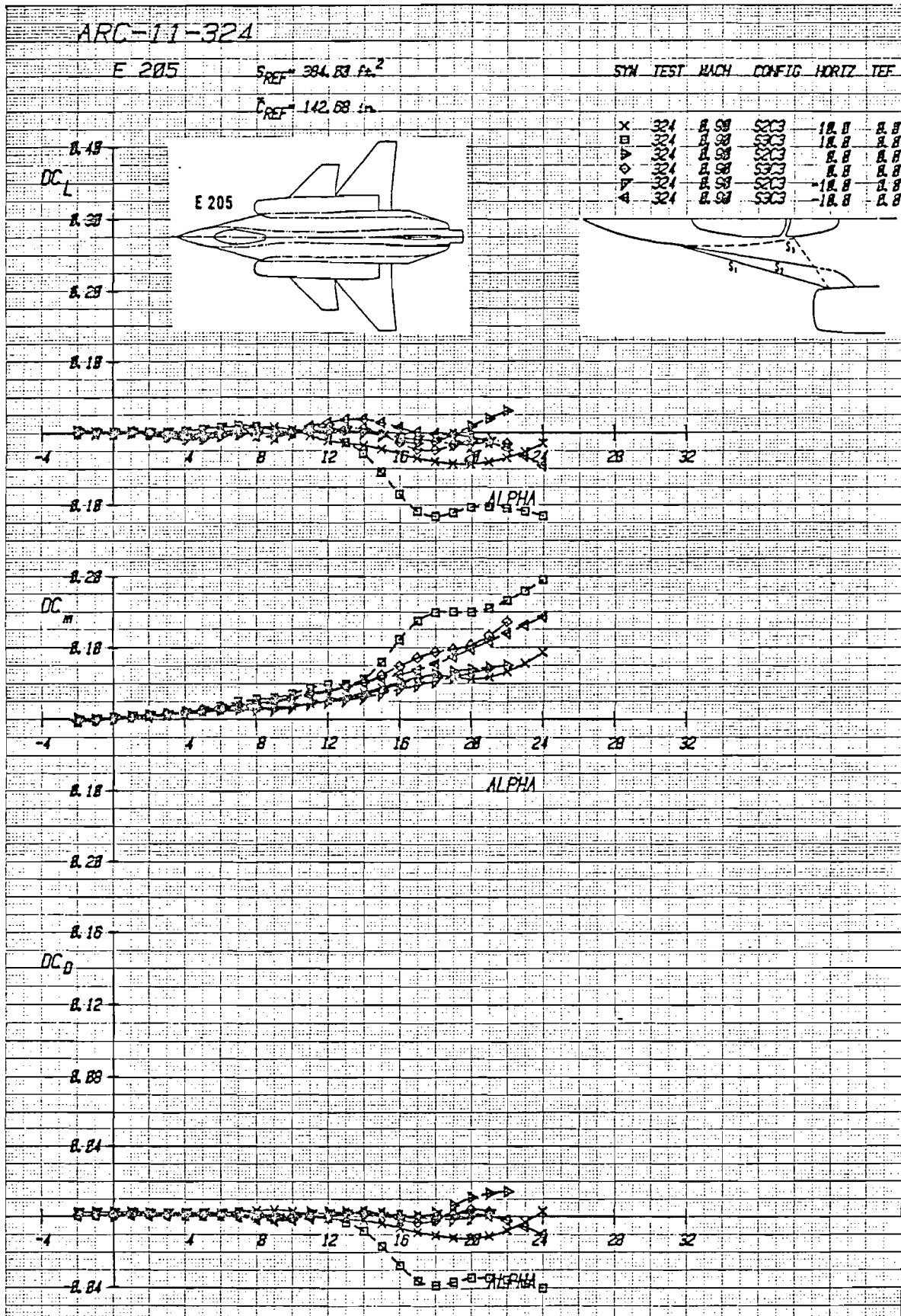
Figure 3-73 Incremental Effects of Strake Shape with Canard C 3 at Various Deflections, Mach = .9
