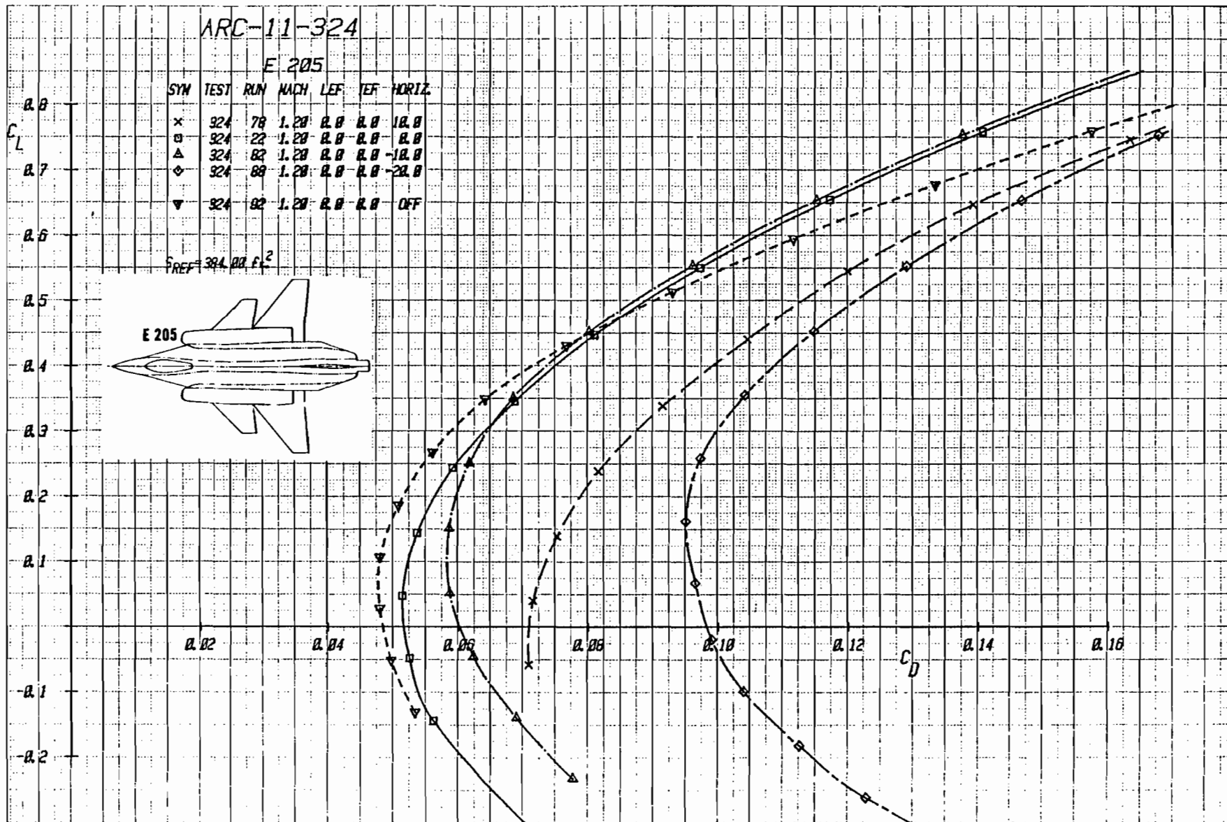
Figure 2-8b Effect of Canard Deflection on Drag With Wing Trailing-Edge Flap Undelected, Mach = 1.2
