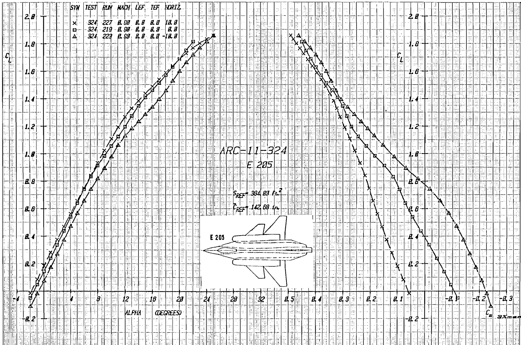
Figure 3-38a Effect of Canard Deflection on Lift and Moment with Canard C_2 , and Strike S_2 , Mach = .9
