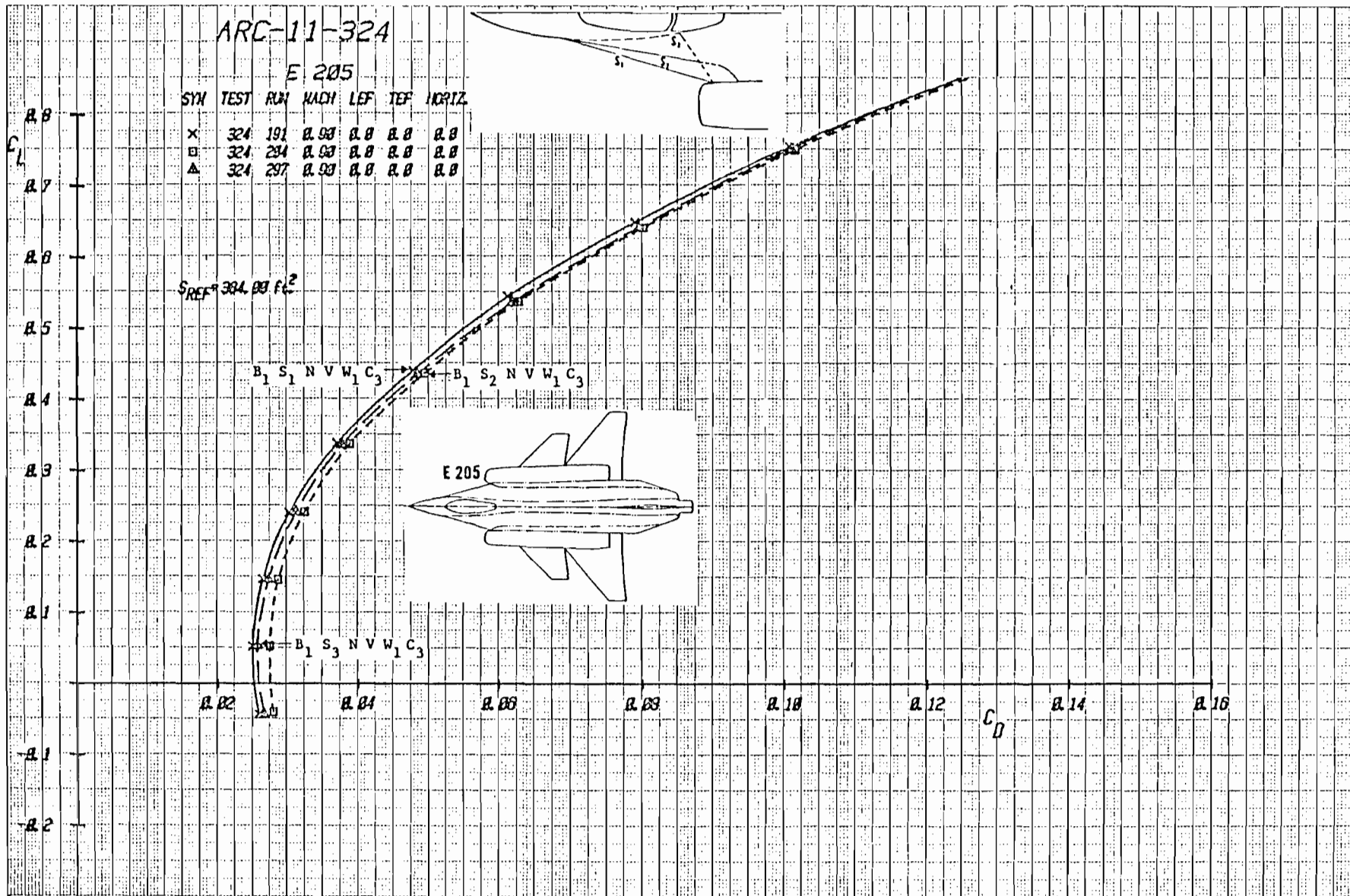
Figure 3-35b Effect of Strake Shape on Drag with Canard C_3 Undelected, Mach = .9
