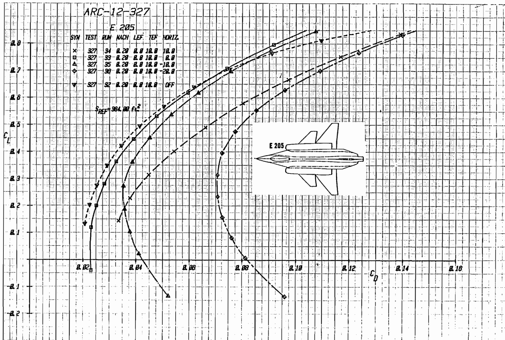
Figure 2-32b Effect of Canard Deflection on Drag with Wing Trailing-Edge Flap Deflected +10^\circ , (Expanded Drag Scale), Mach = .2
