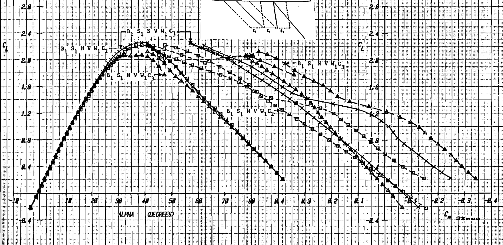
Figure 2-4a Effect of Canard Location with Baseline Strake, S_1 , on E205 Lift and Pitching Moment ( \alpha = 0^\circ to 90^\circ ), M = .2
