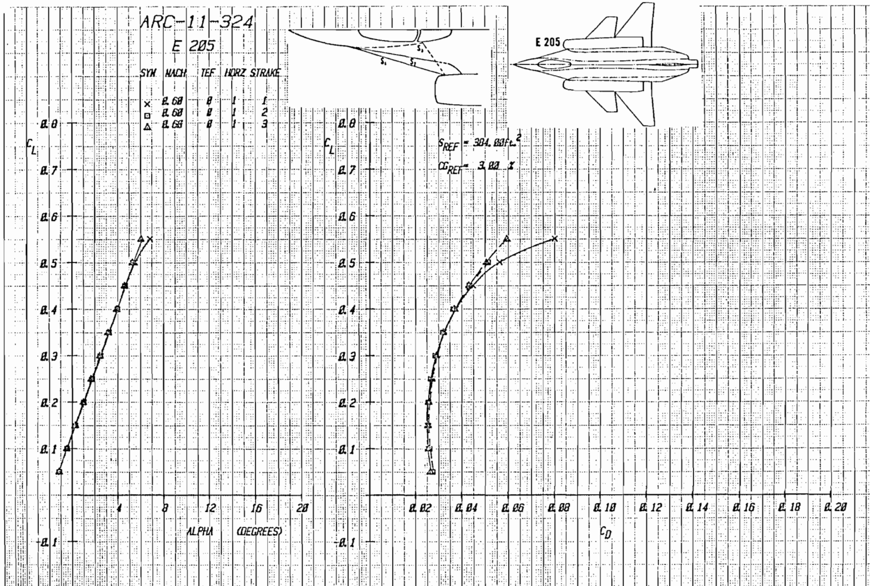
Figure 3-78 Trimmed Lift and Drag With Variations in Strake and Canard C_L , Mach =
