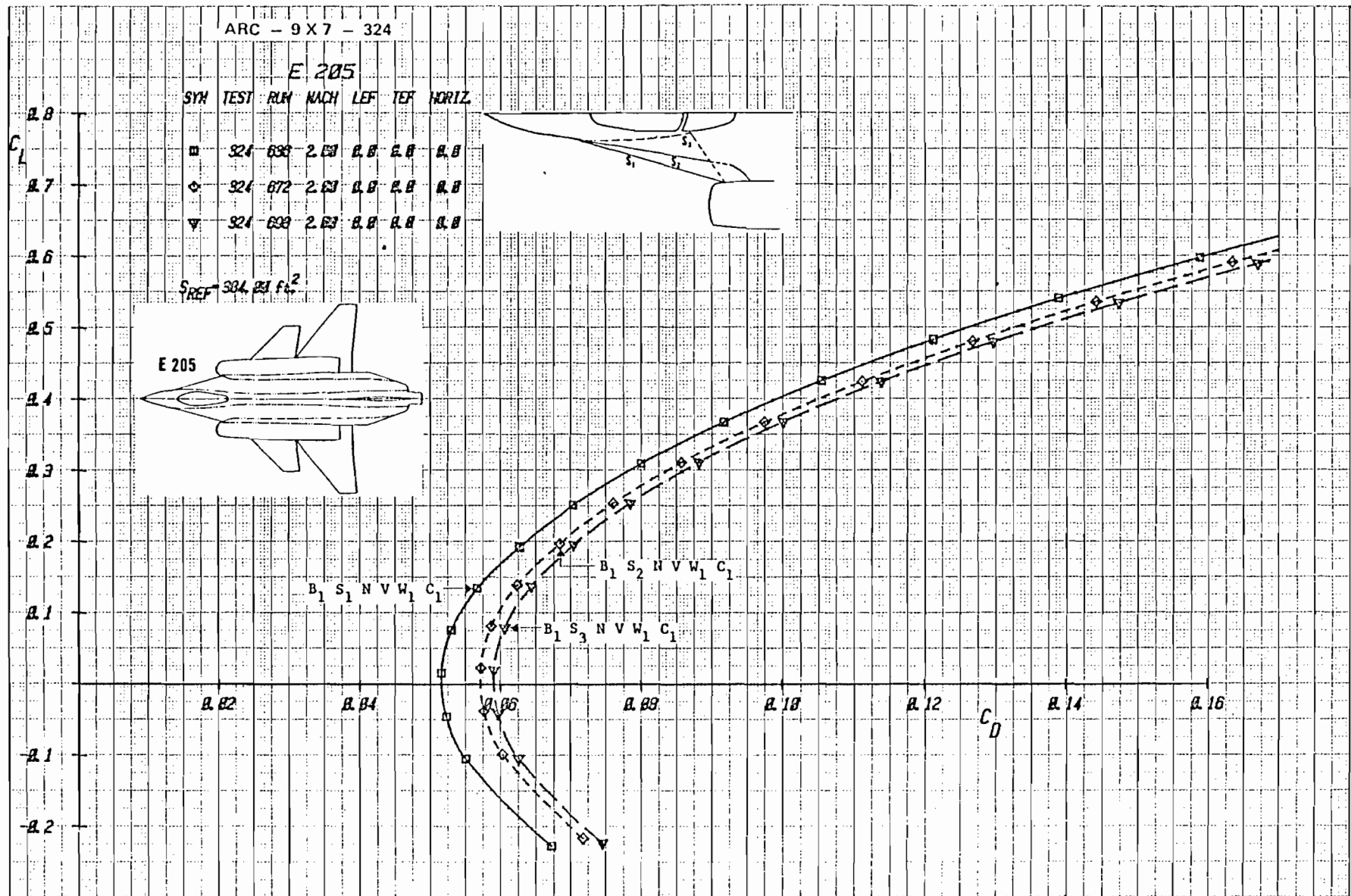
Figure 3-63b Effect of Strake Variation on Drag with Baseline Canard Longitudinal Location, C_1 , and \delta_i = 0^\circ , (Expanded Drag Scale), Mach = 2.0.
