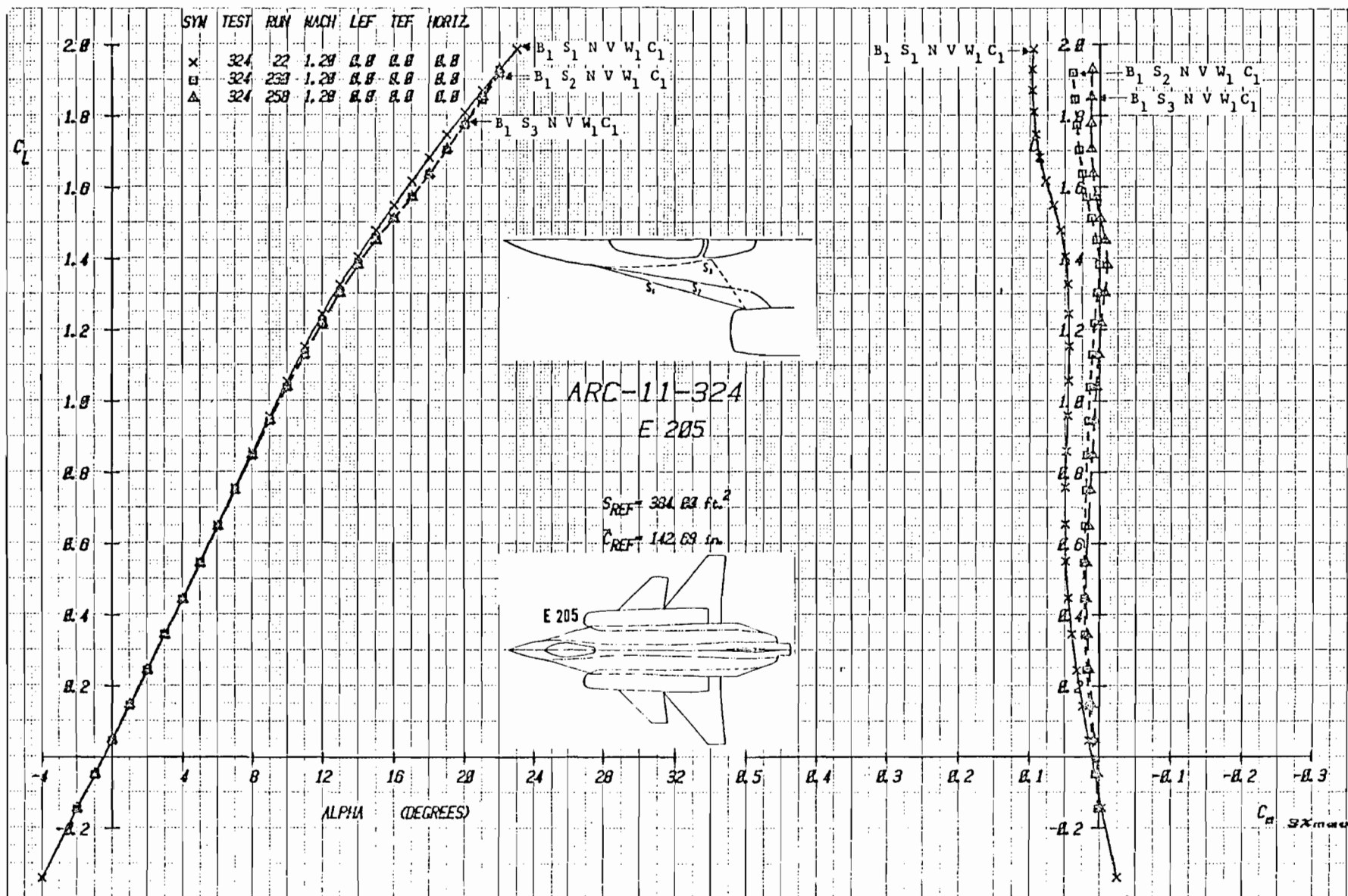
Figure 3-44a Effect of Strake Shape on Lift and Moment with Canard C_1 Undeflected, Mach = 1.2
