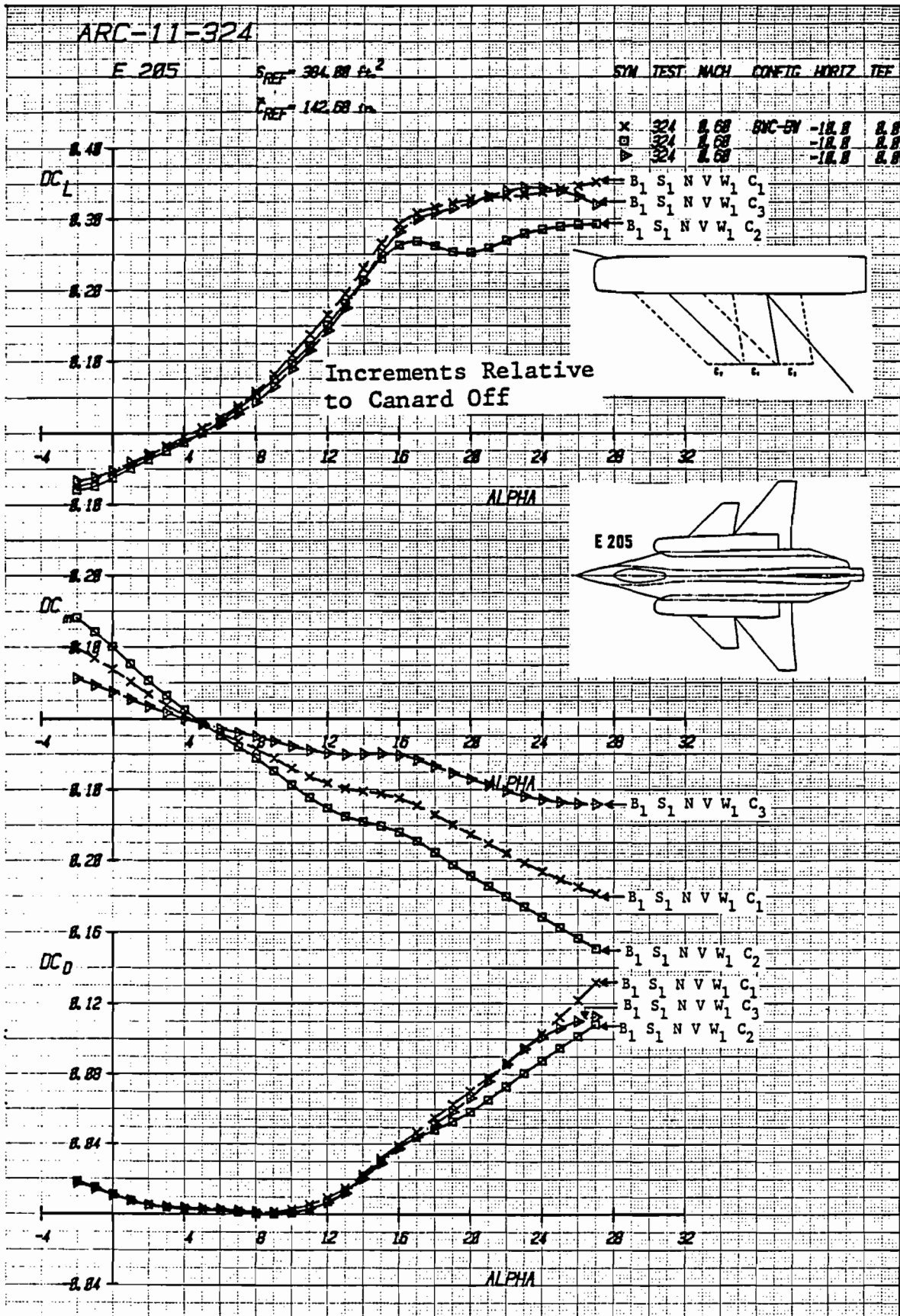
Figure 2-25 Incremental Effects of Canard Longitudinal Location on Canard Effectiveness at \delta_i = -10^\circ , Mach = .6
