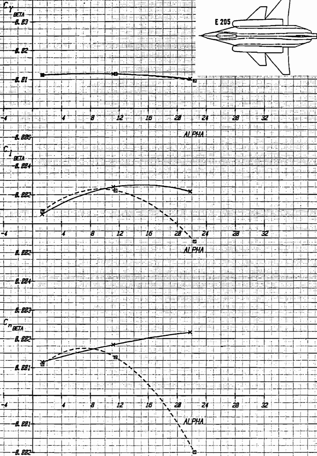
Figure 2-46 Vertical Tail Effectiveness for the E 205 Configuration, with Strake S_1 , Canard C_2 , on and off, \delta_{VT} = 0^\circ , Mach = .2
