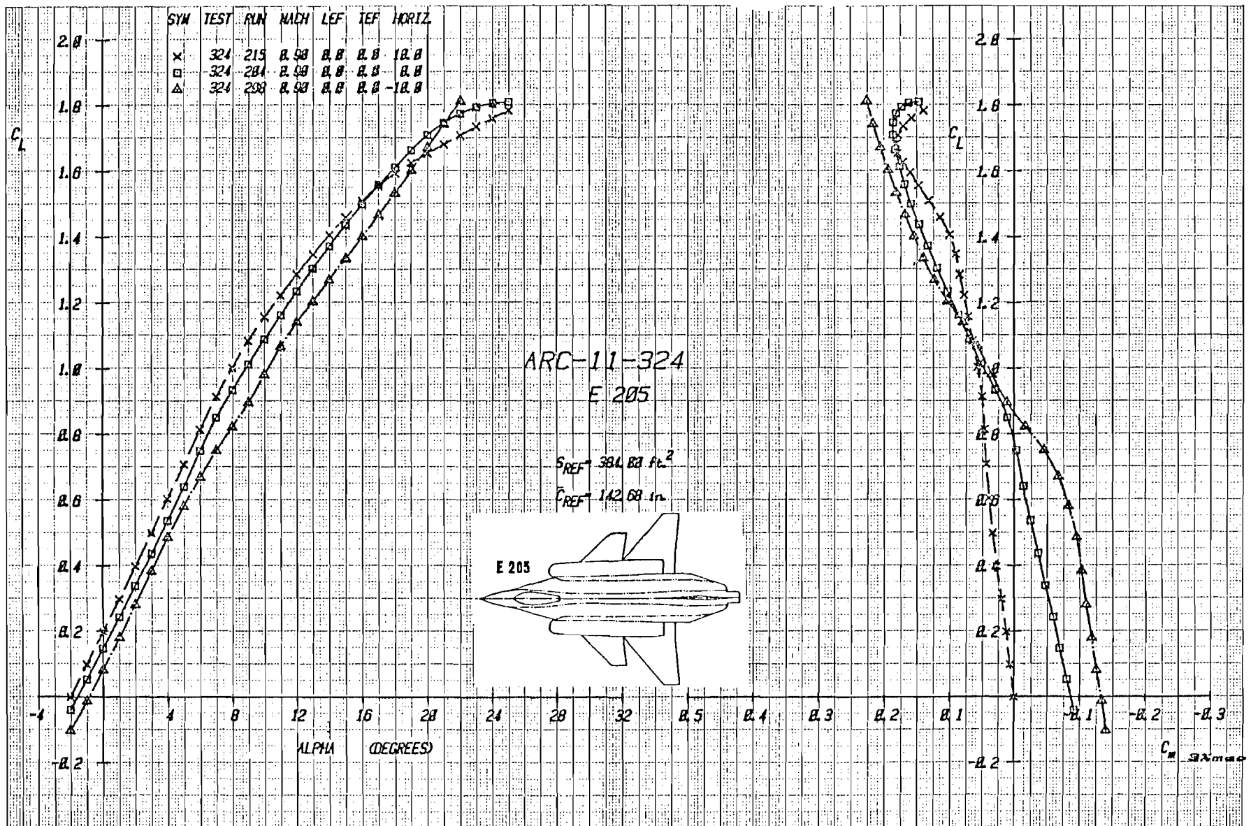
Figure 3-39a Effect of Canard Deflection on Lift and Moment With Canard C_1 , and Strike S_2 , Mach = .9
