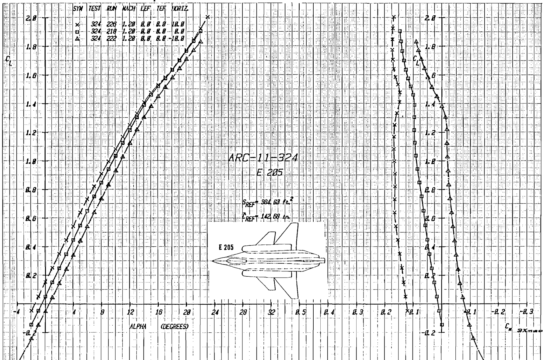
Figure 3-53a Effect of Canard Deflection on Lift and Moment With Canard C_2 , and Strike S_2 , Mach = 1.2
