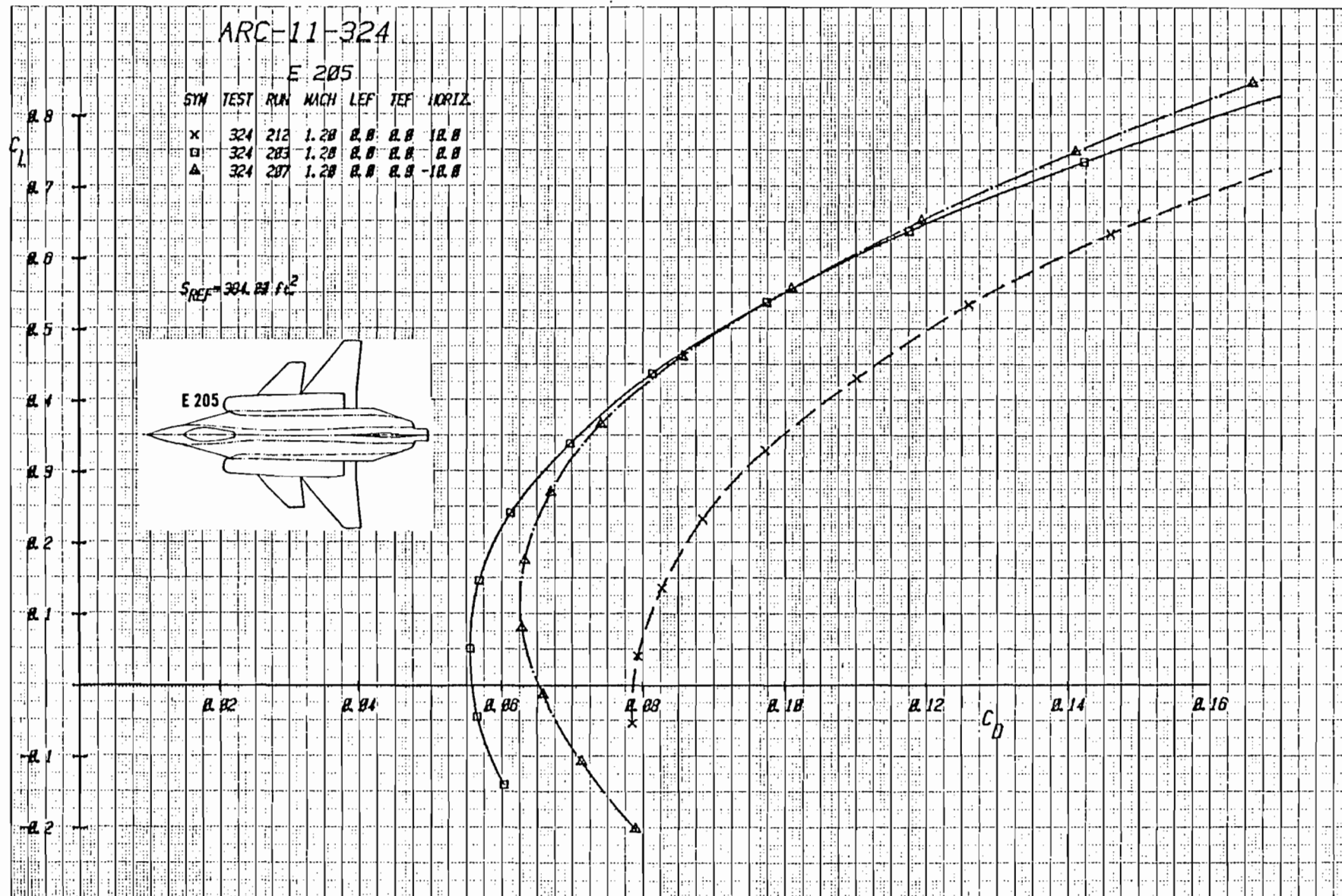
Figure 3-54b Effect of Canard Deflection on Drag with Canard C_3 , and Strake S_2 , Mach = 1.2
