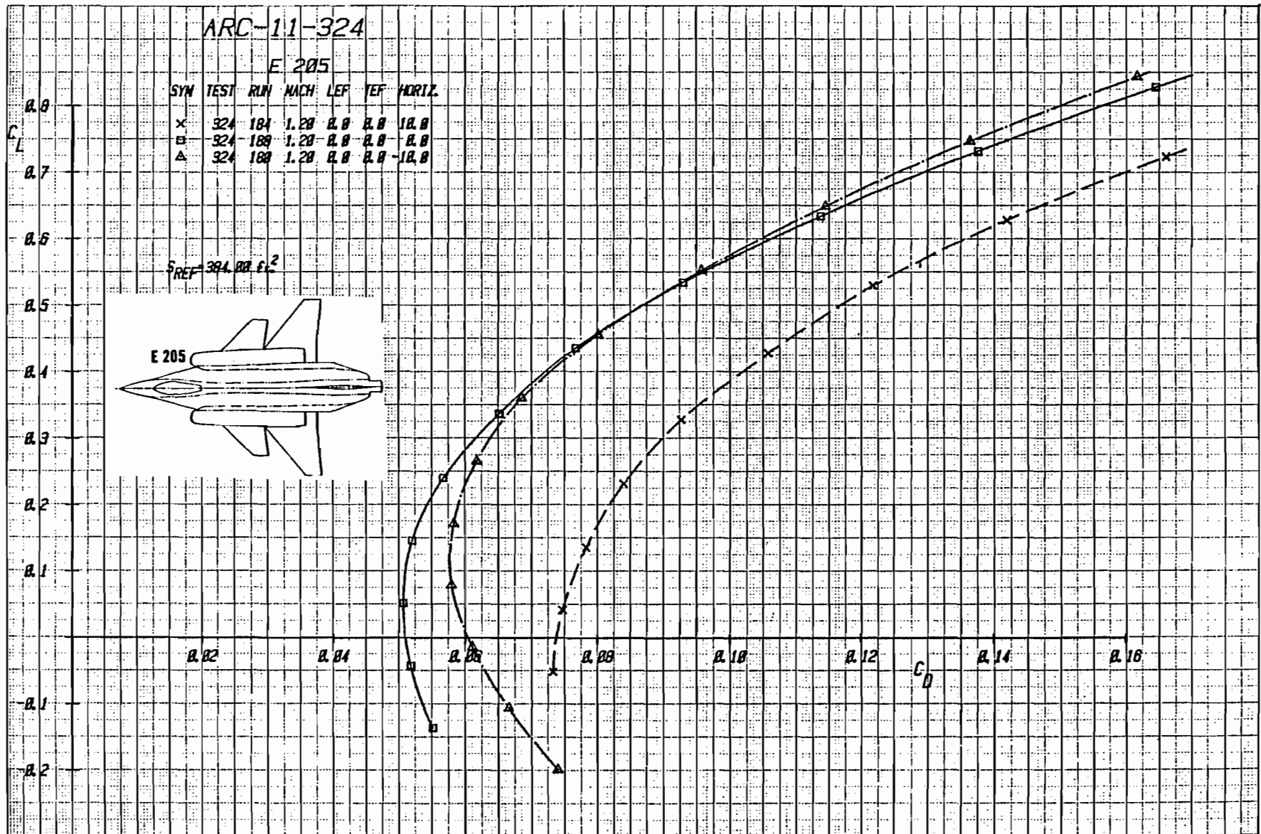
Figure 2-14b Effect of Canard Deflection on Drag With Aft Canard Longitudinal Location, C_3 , and Baseline Stroke, S_1 , Mach = 1.2
