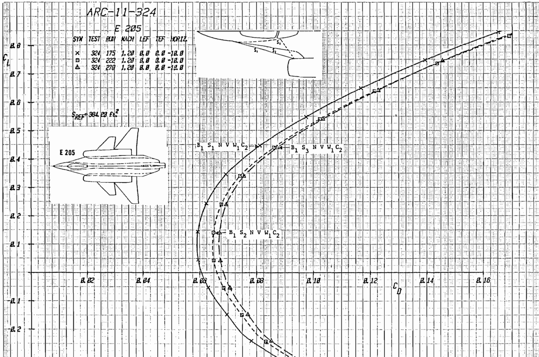
Figure 3-48b Effect of Strake Shape on Drag with Canard C 2 Deflected -10°, Mach = 1.2
