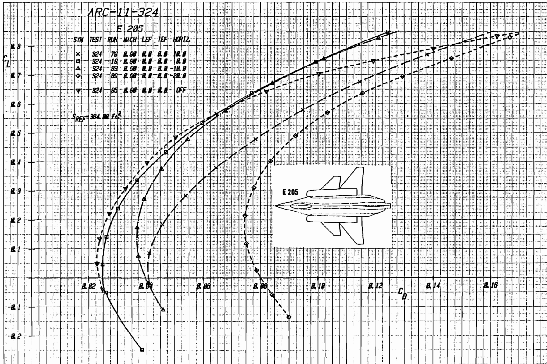
Figure 2-7b Effect of Canard Deflection on Drag with Wing Trailing-Edge Flap Undeflected, (Expanded Drag Scale), Mach = .9
