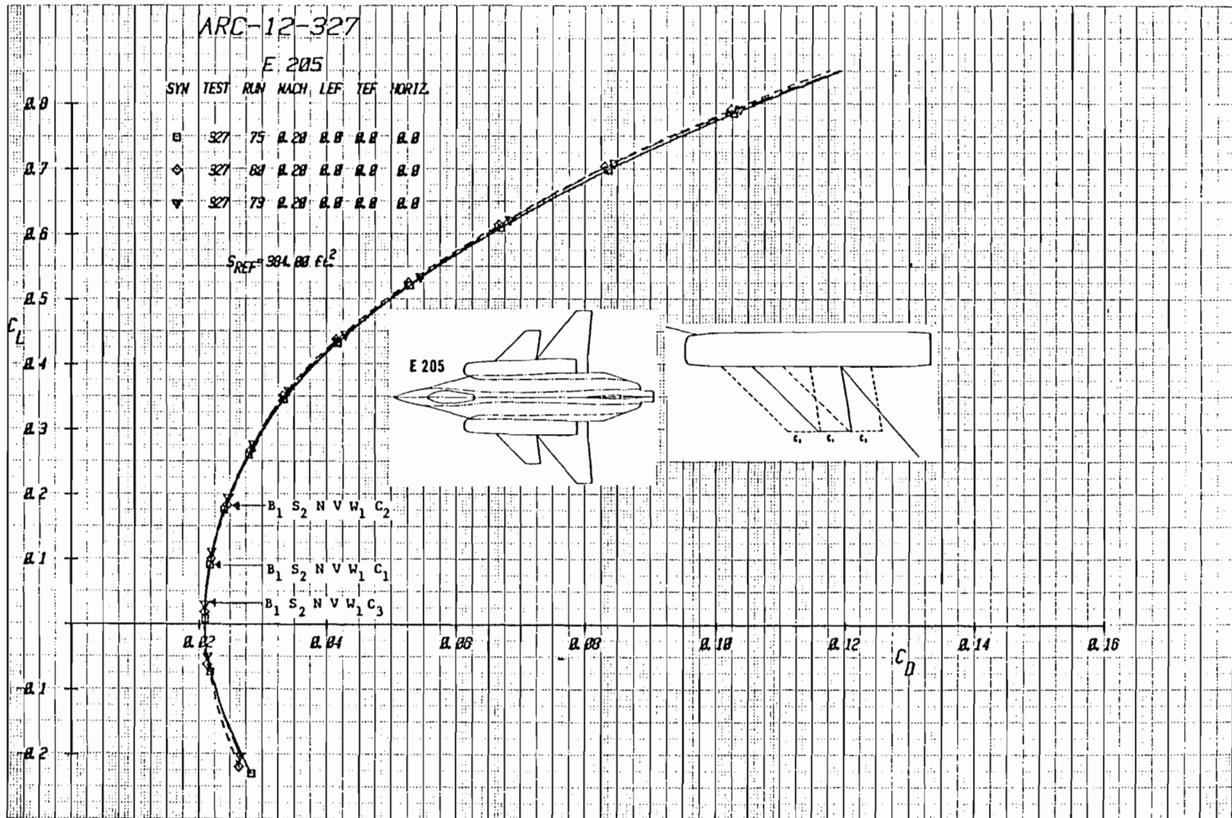
Figure 3-7b Effect of Canard Longitudinal Location on Drag with Strake S_2 , (Expanded Drag Scale), Mach = .2
