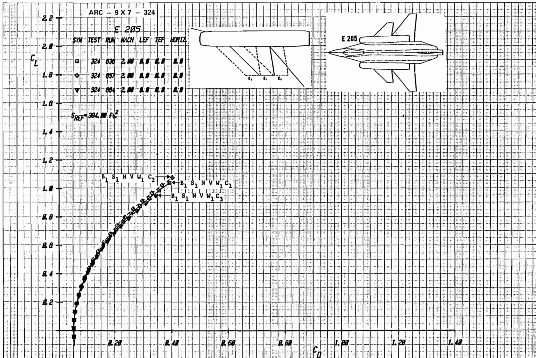
Figure 2-18 Effect of Canard Longitudinal Location on Drag With Baseline Strake, Mach = 2.0
