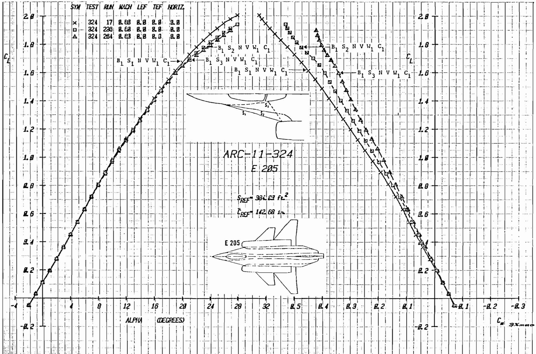
Figure 3-14a Effect of Strake Shape on Lift and Moment with Canard C_1 Undeflected, Mach = .6
