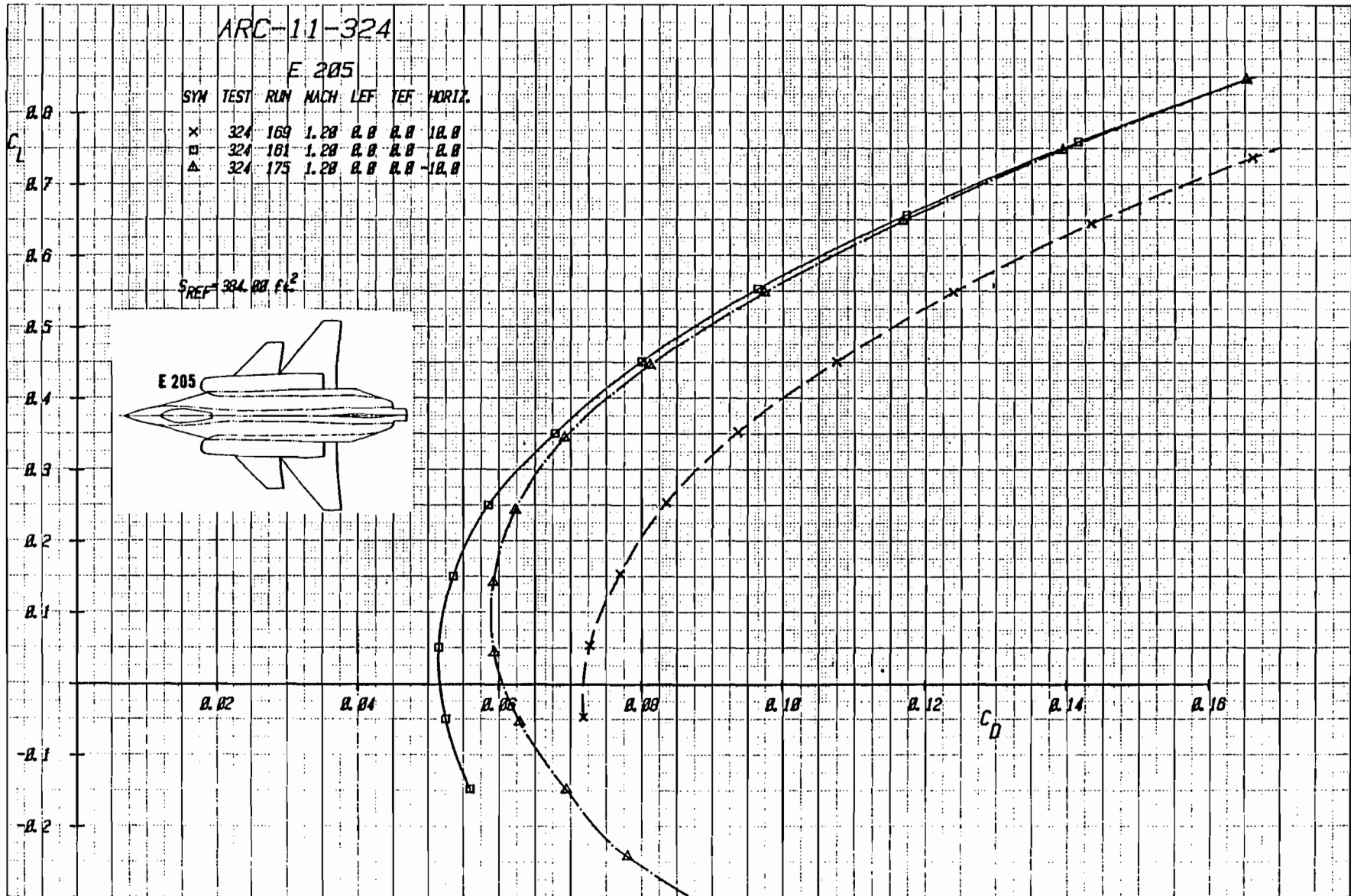
Figure 2-11b Effect of Canard Deflection on Drag With Forward Canard Longitudinal Location, C_2 , and Baseline Strake, S_1 , Mach = 1.2
