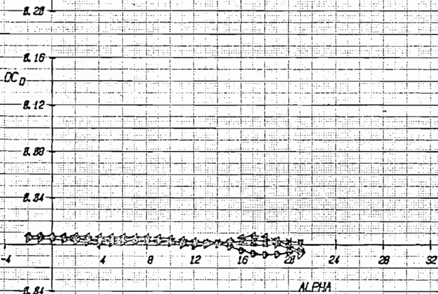
Figure 3-74 Incremental Effects of Strake Shape with Canard C 1 at Various Deflections, Mach = 1.2
