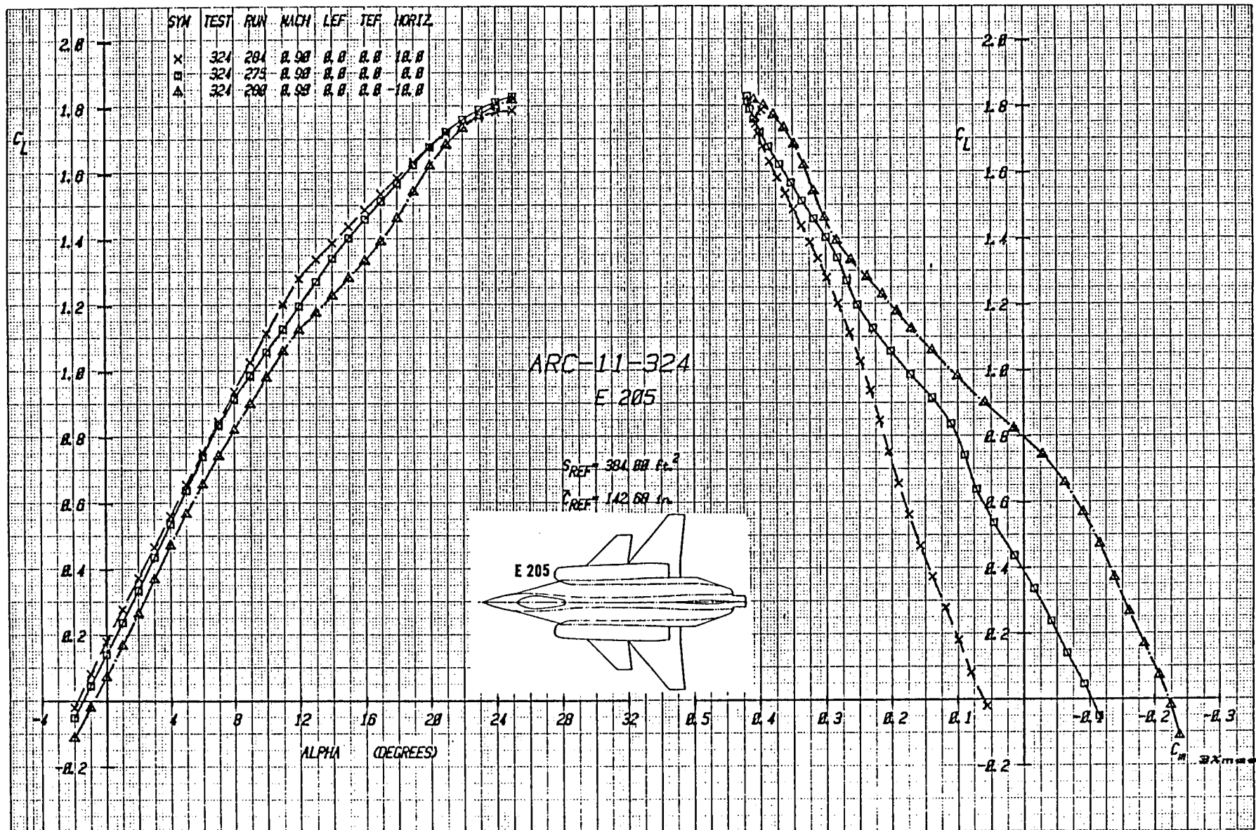
Figure 3-41a Effect of Canard Deflection on Lift and Moment with Canard C_2 , and Stroke S_1 , Mach = .9
