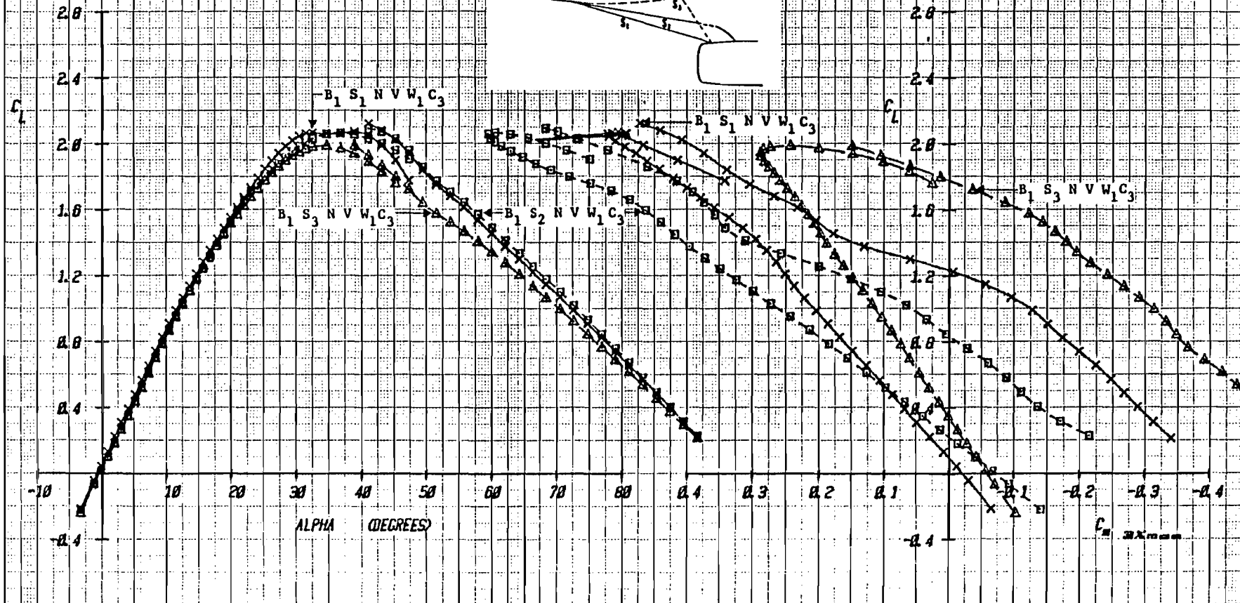
Figure 3-6a Effect of Strake Shape with Aft Canard Location, C_3 , on E205 Lift and Pitching Moment ( \alpha = 0^\circ to 90^\circ ), \delta_c = 0^\circ , M = .2
