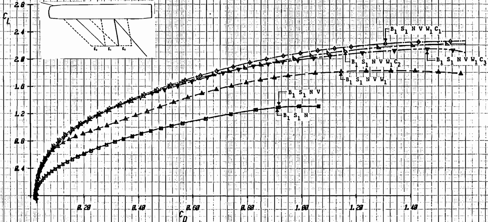
Figure 1-c Effect of Component Buildup on Drag, Mach = .2
