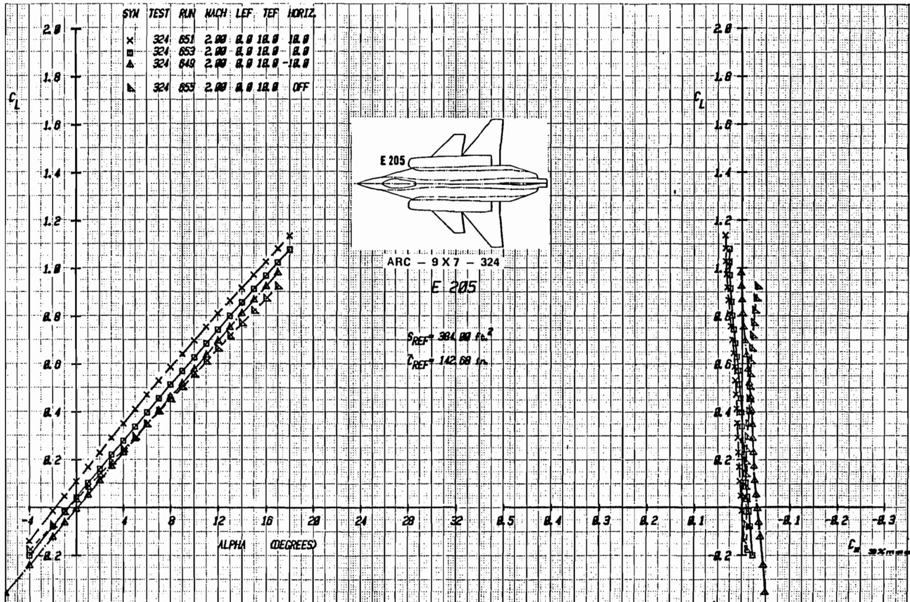
Figure 2-37a Effect of Canard Deflection on Lift and Moment With Wing Trailing-Edge Flap Deflected +10^\circ , Mach = 2.0
