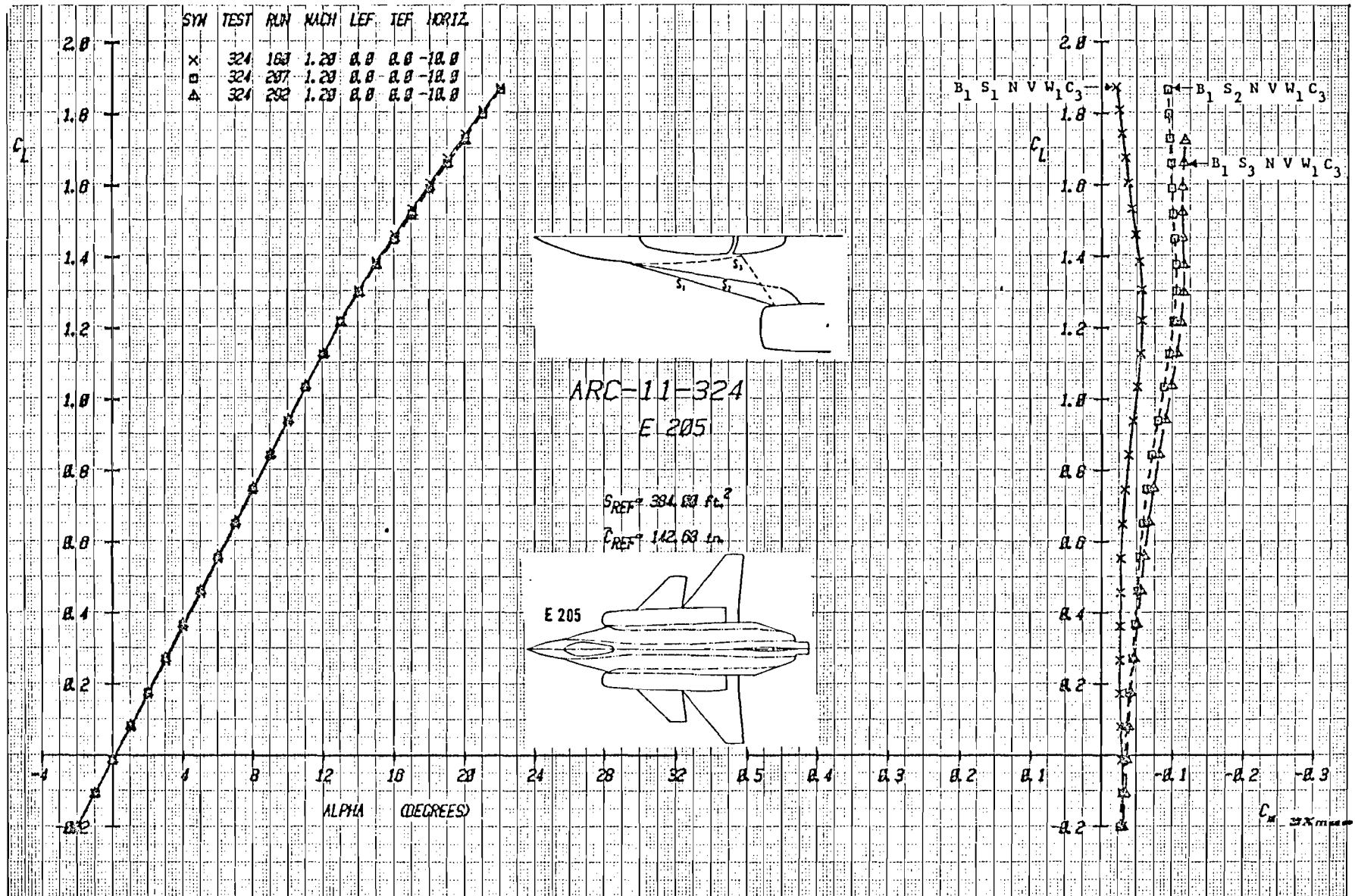
Figure 3-51a Effect of Strake Shape on Lift and Moment with Canard C_3 Deflected -10^\circ , Mach = 1.2
