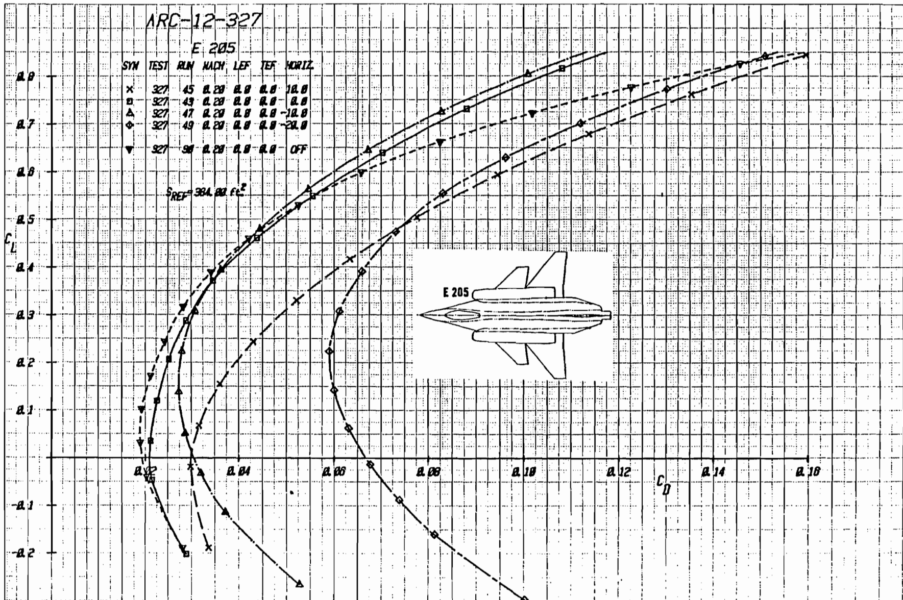
Figure 2-1b Effect of Canard Deflection on Drag with Wing Trailing-Edge Flap Undeflected, (Expanded Drag Scale), Mach = .2
