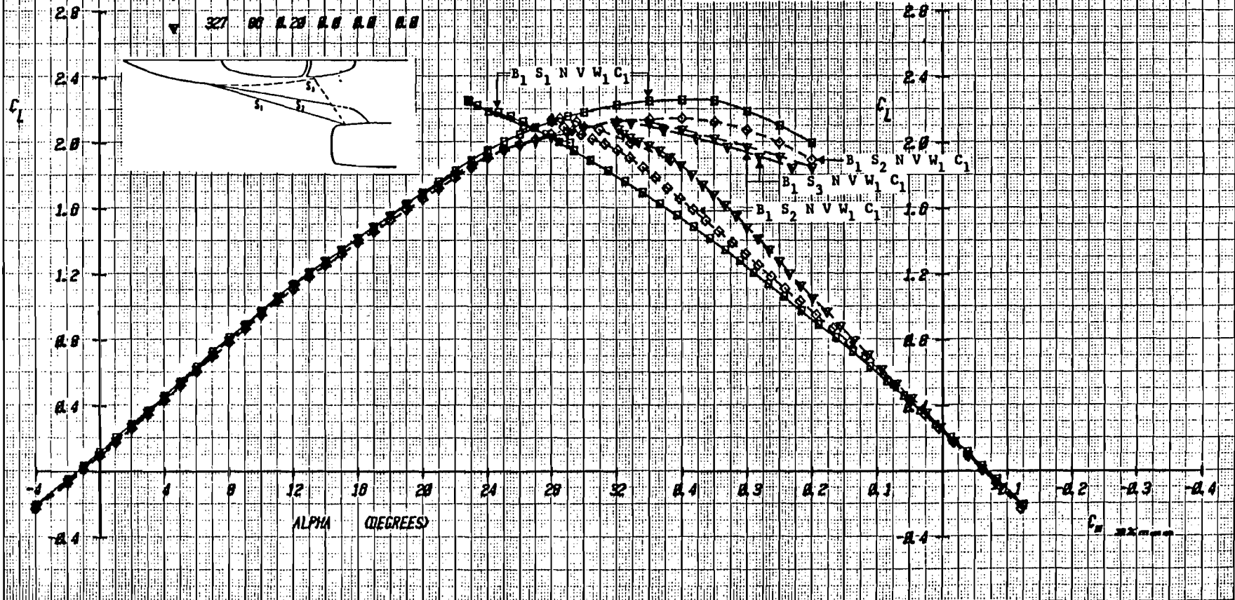
Figure 3-1a Effect of Strake Variation on Lift and Moment with Baseline Canard Longitudinal Location, C_L , and \delta_i = 0^\circ , Mach = .2
