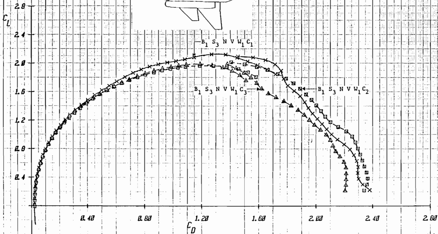
Figure 3-10b Effect of Canard Location with Strake S_3 on E205 Drag ( \alpha = 0^\circ to 90^\circ ), \delta_c = 0^\circ , M = .2
