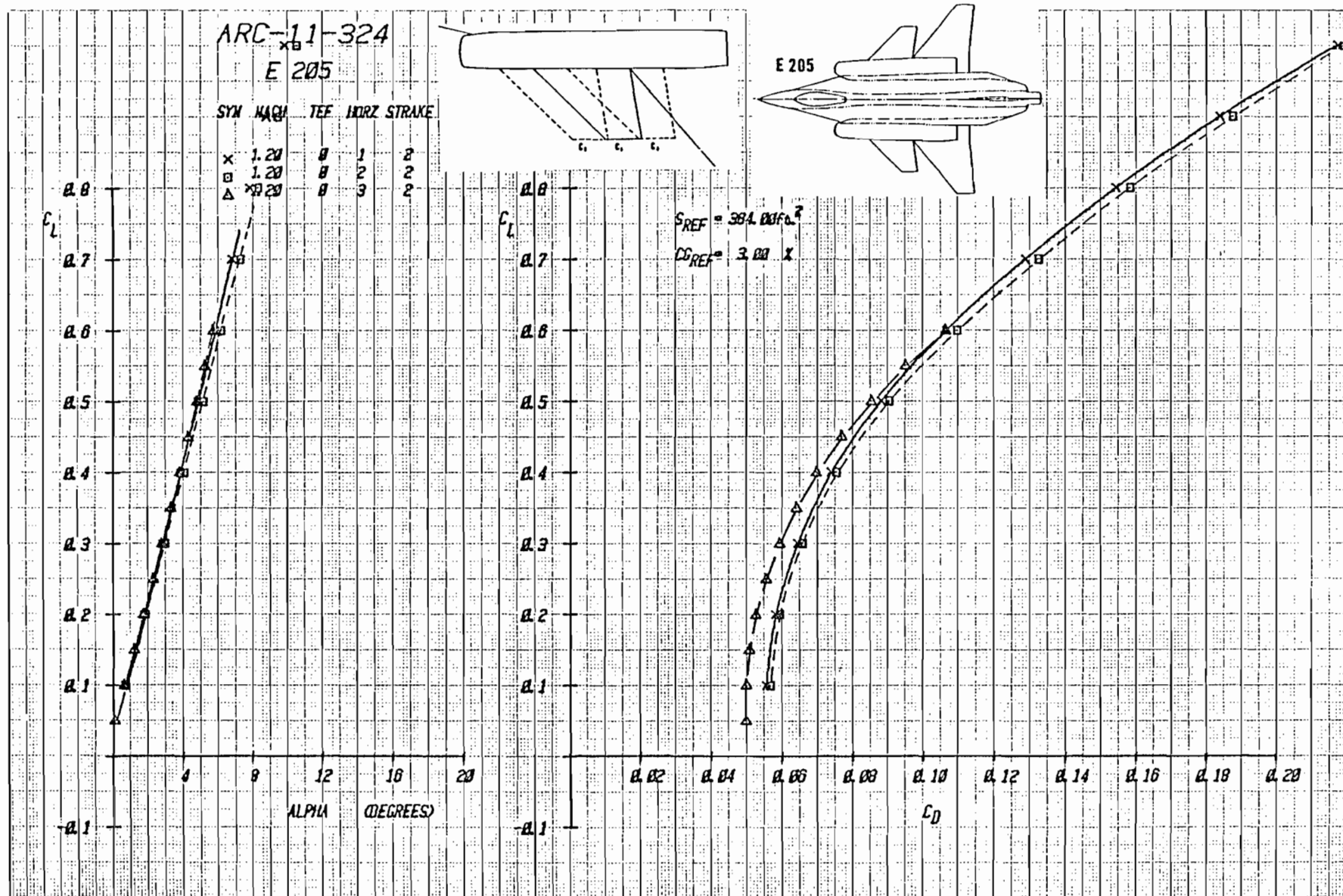
Figure 3-89 Trimmable Lift and Drag With Variations in Canard Longitudinal Location and Strake S_2 , Mach = 1.2
