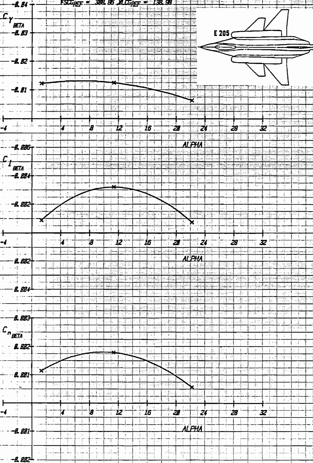
Figure 2-45 Vertical Tail Effectiveness for the E 205 Configuration, with Strake S_1 , Canard C_3 , \delta_{VT} = 0^\circ , Mach = .2
