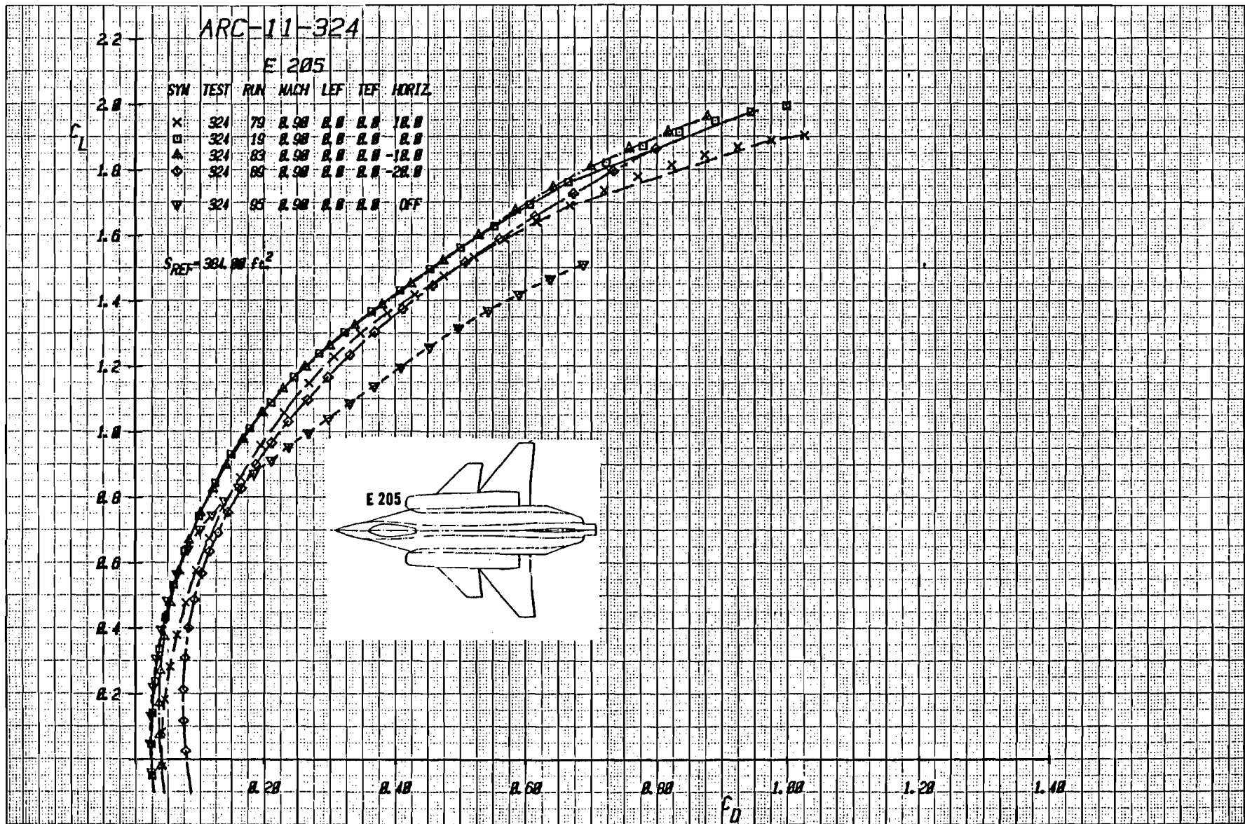
Figure 2-7c Effect of Canard Deflection on Drag With Wing Trailing-Edge Flap Undelected, Mach = .9
