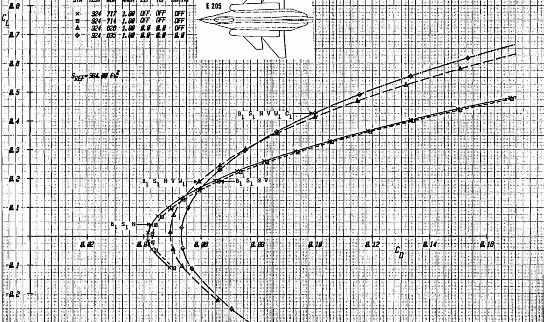
Figure 1-10b Effect of Component Buildup on Drag, (Expanded Drag Scale), Mach = 1.8
