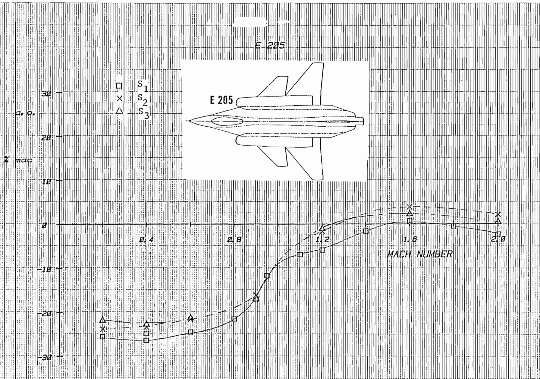
Figure 3-77 Effect of Strake Shape on Aerodynamic Center Variation with Mach Number (with Baseline Canard Location)
