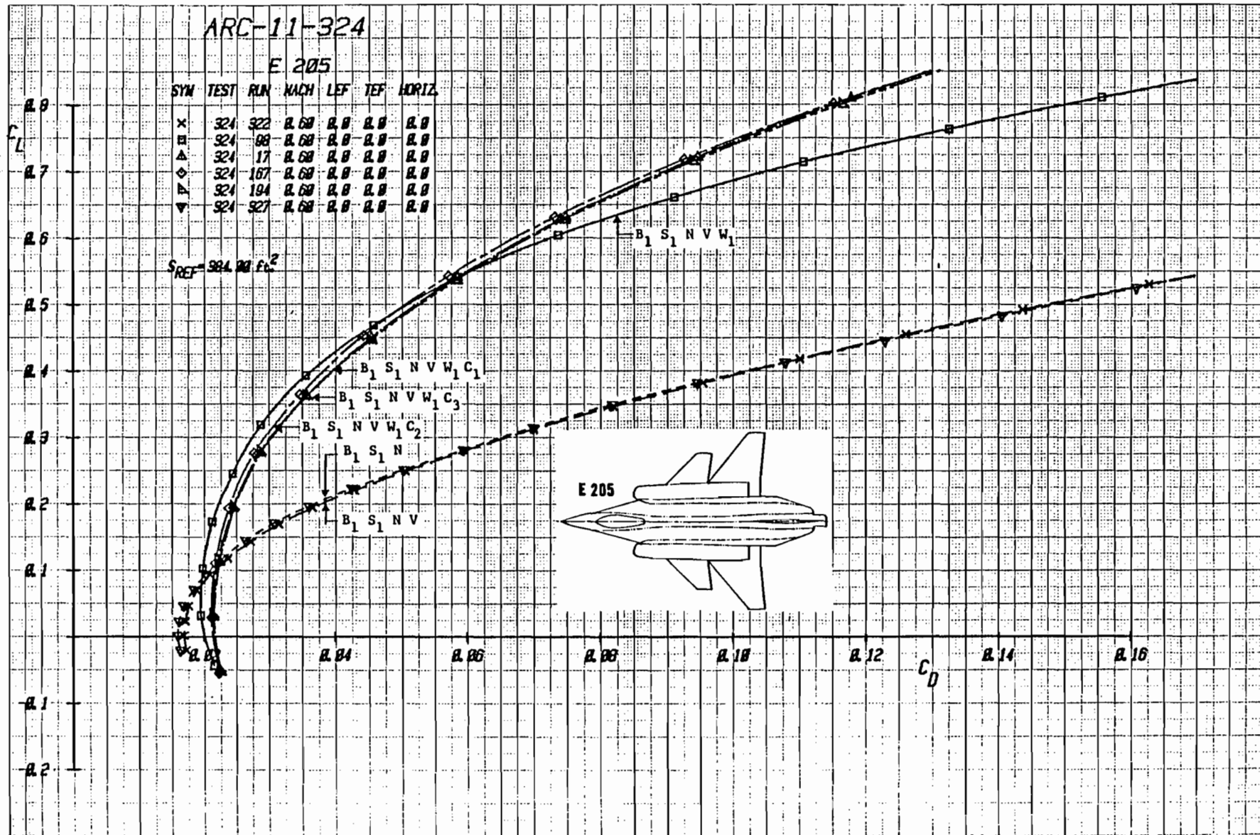
Figure 1-6b Effect of Component Buildup on Drag, Mach = .6
