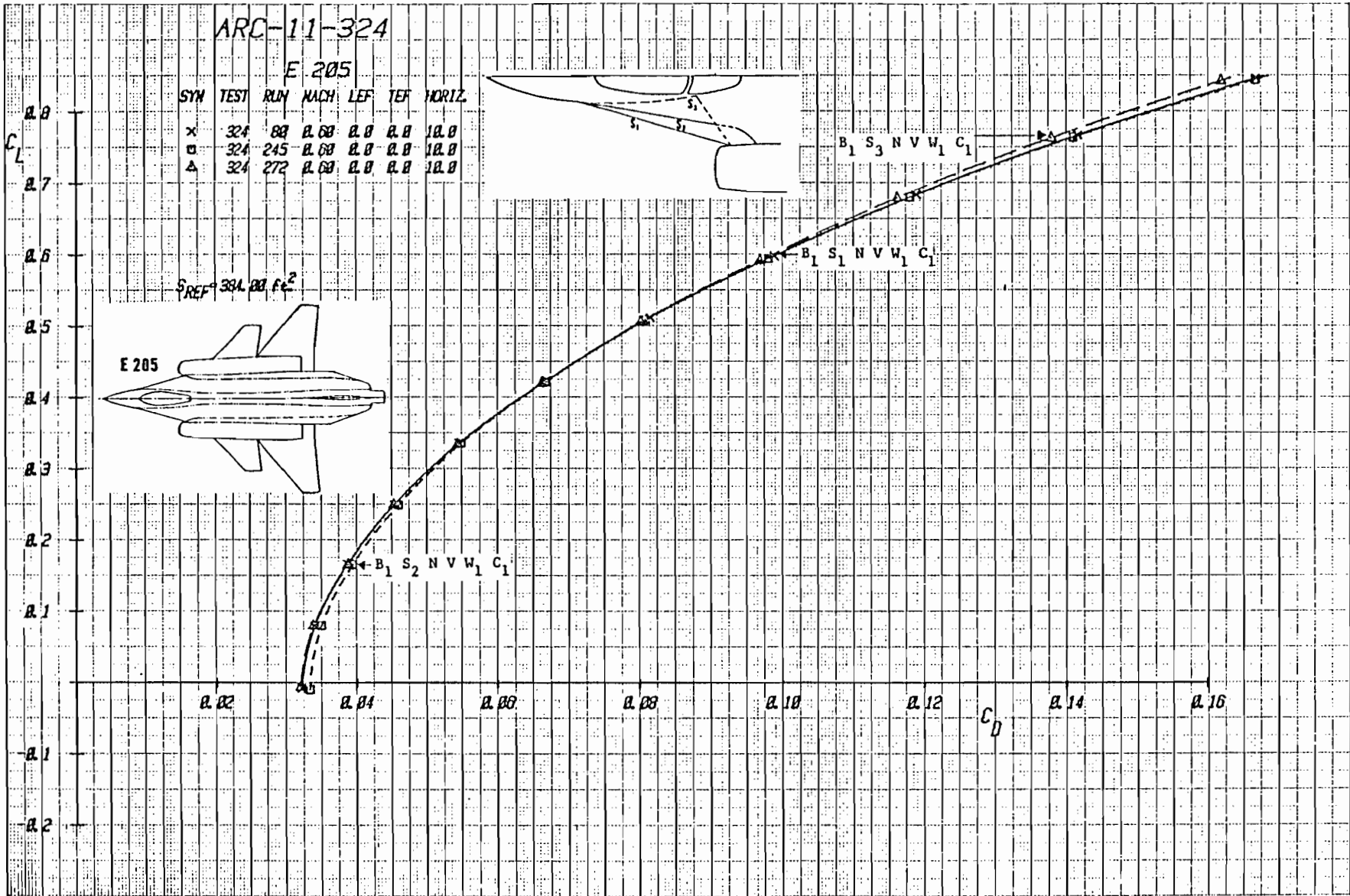
Figure 3-13b Effect of Strake Shape on Drag with Canard C 1 Deflected + 10°, Mach =
