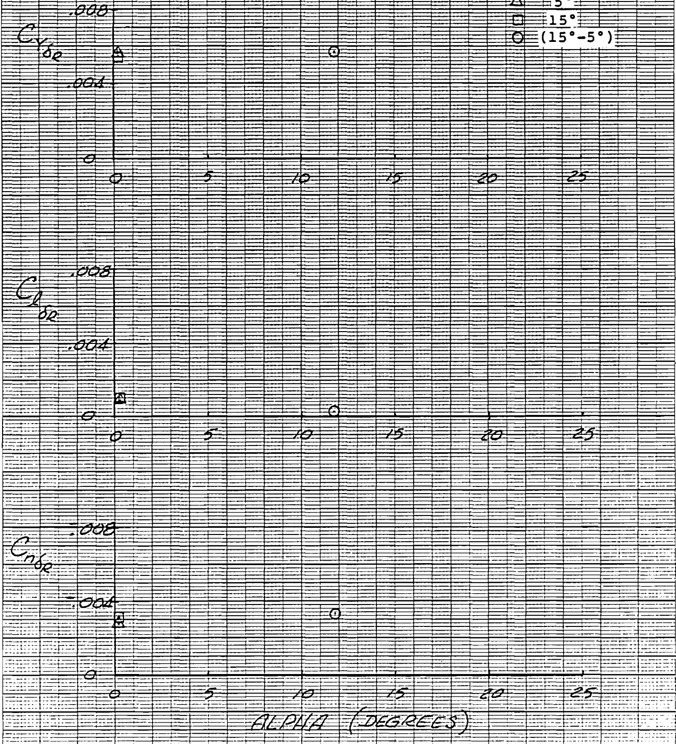
Figure 2-65 Effect of Vertical Tail Deflection, M = 1.2
