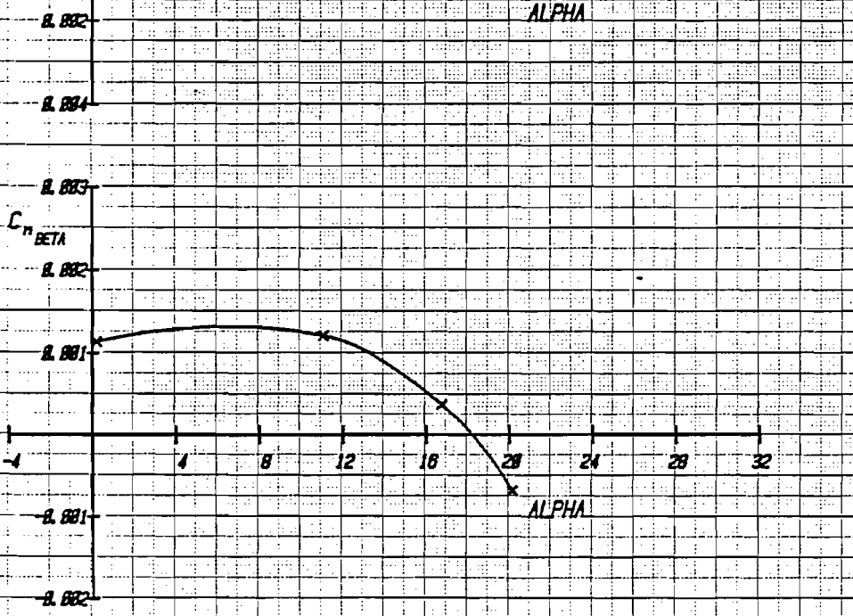
Figure 2-48 Lateral-Directional Characteristics for Baseline E205 Configuration, M = .6
