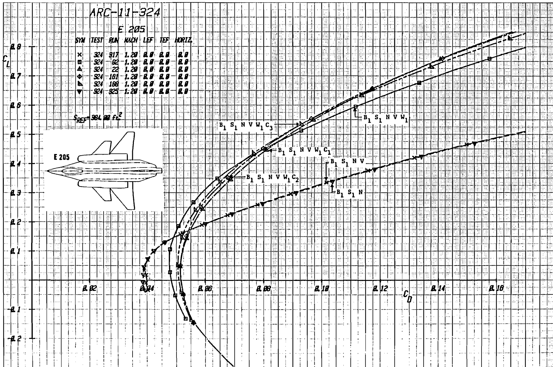
Figure 1-8b Effect of Component Buildup on Drag, Mach = 1.2
