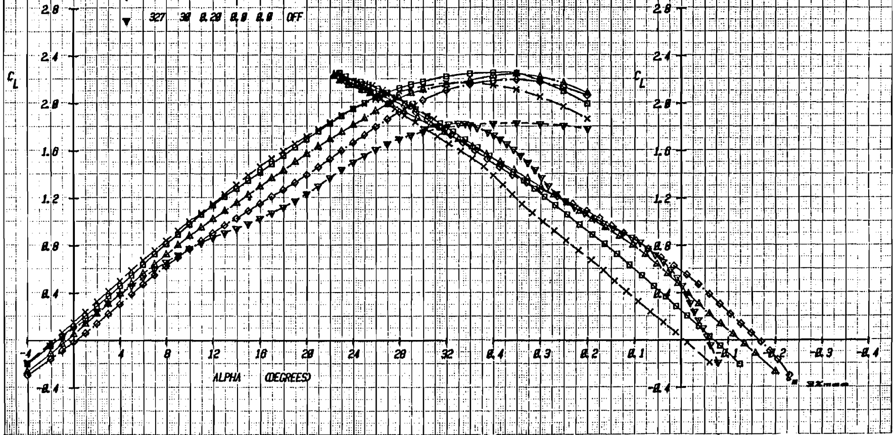
Figure 2-1a Effect of Canard Deflection on Lift and Moment with Wing Trailing-Edge Flap Undelected, Mach = .2
