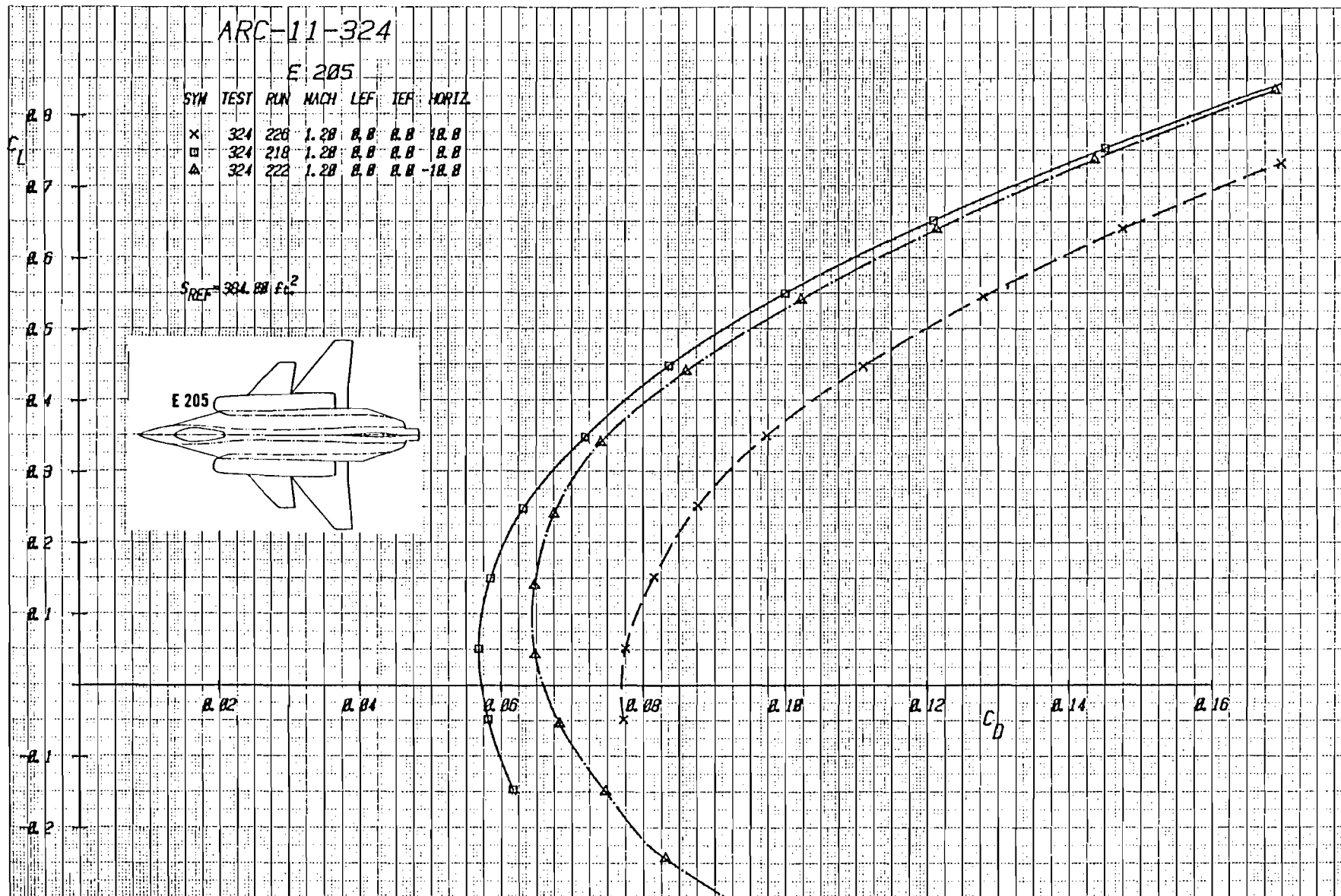
Figure 3-53b Effect of Canard Deflection on Drag With Canard C_2 , and Strake S_2 , Mach = 1.2
