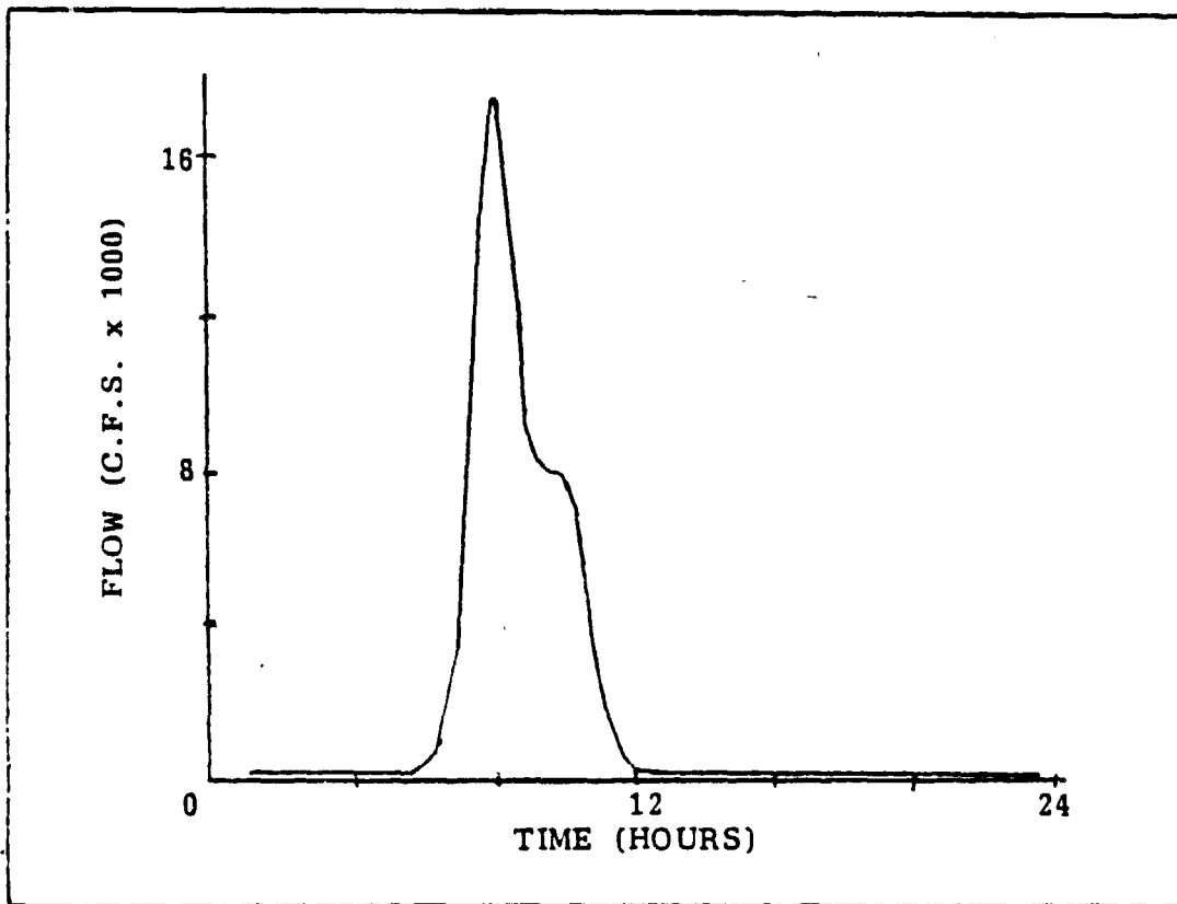
Figure 16. Keowee hydro discharge (February 27, 1979)
