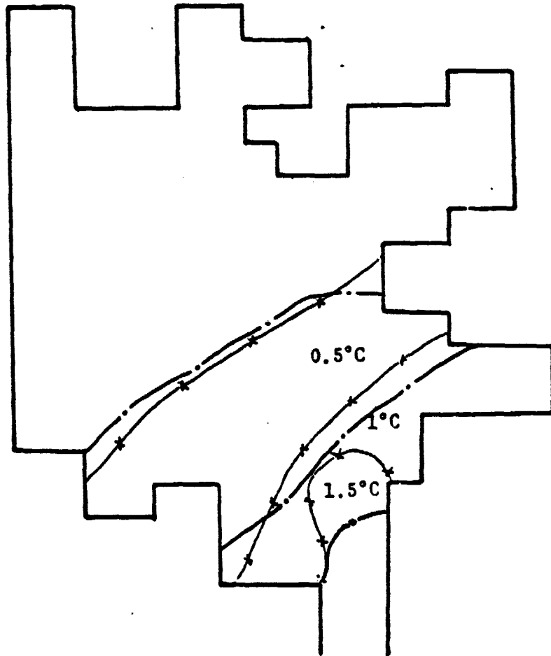
Figure 30. Isotherms: measured and predicted (temperatures above ambient)
