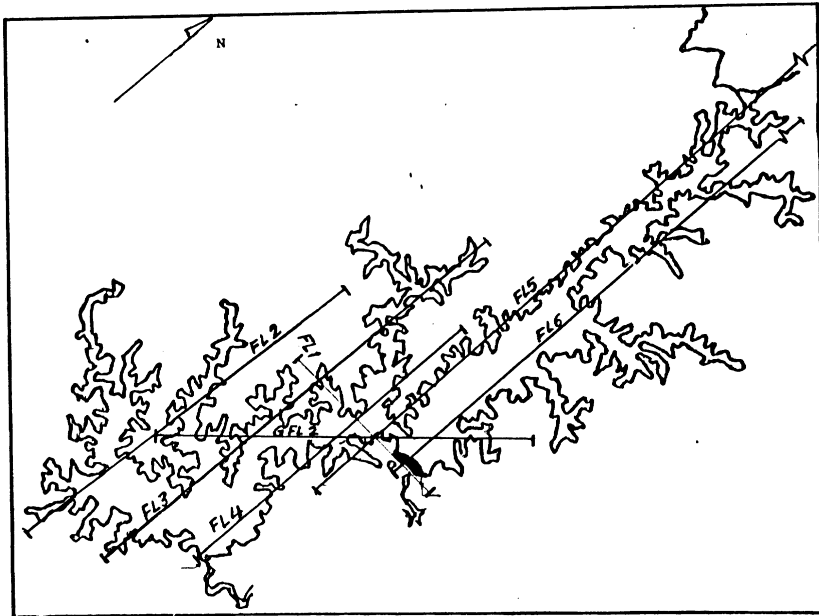
Figure 8. Flight plans for IR data (August and February missions)
