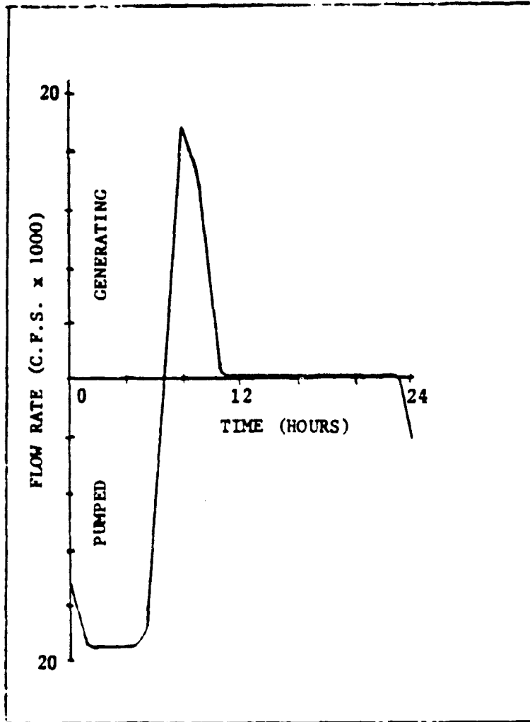
Figure 14. Jocassee-pumped storage station discharge data (February 27, 1979)
