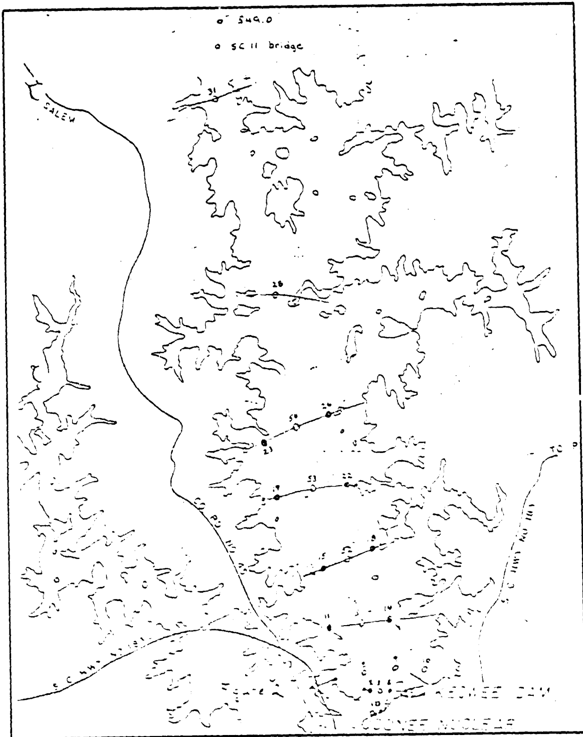
Figure 7. August ground truth data (measuring stations)
