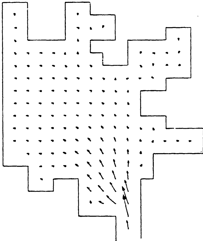
Figure 21. Velocities at K = 1, Lake Keowee (rigid-lid model)
