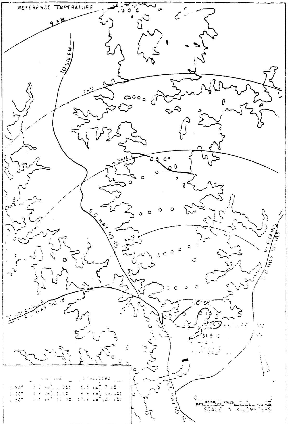
Figure 6. Measured isotherms (Archival 9/10/75)
