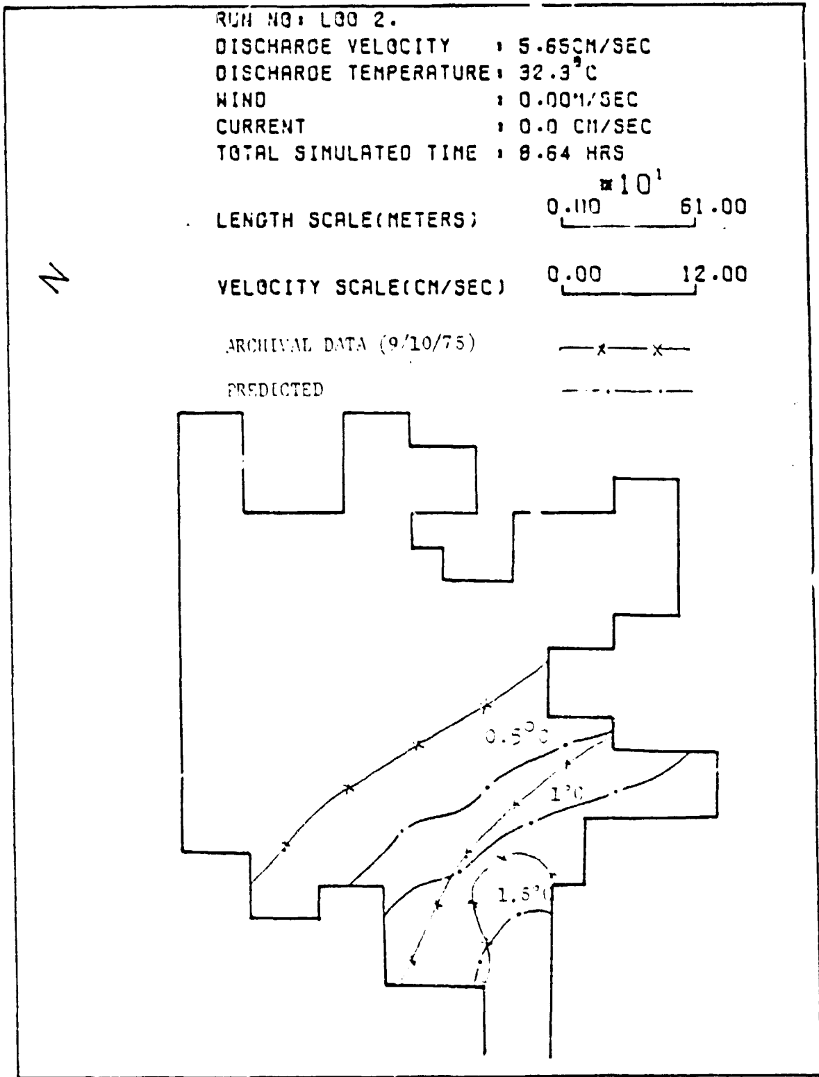
Figure 23. Isotherms: measured and predicted (temperatures above ambient)
