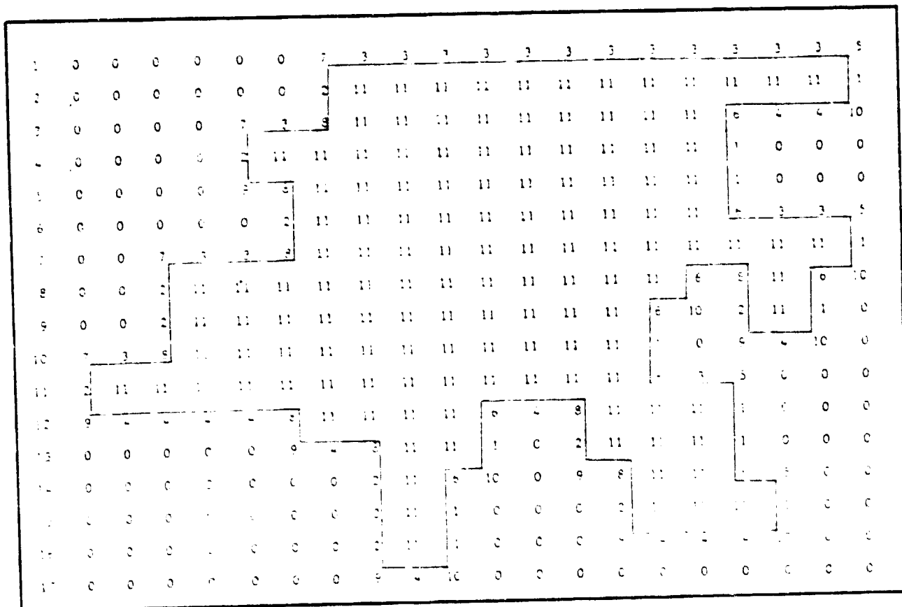
Figure 3. MAR marker matrix (main grid points)
