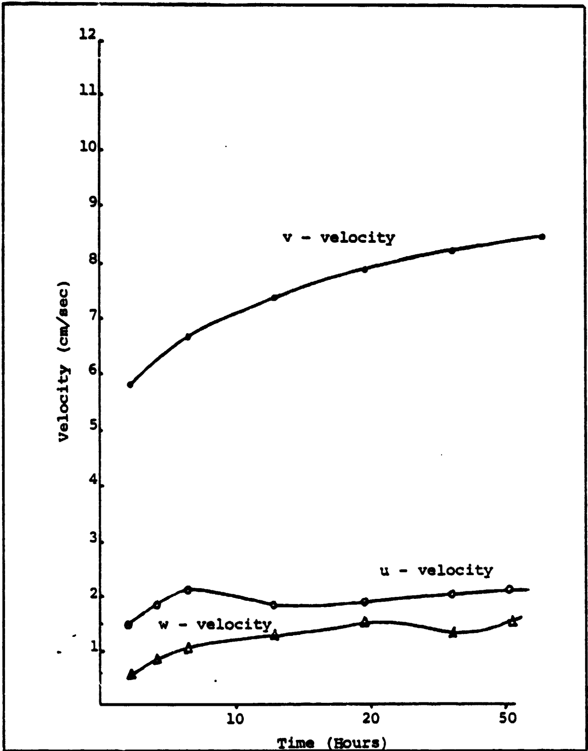
Figure 33. L005, velocity vs. time, I = 11, J = 2, K = 1
