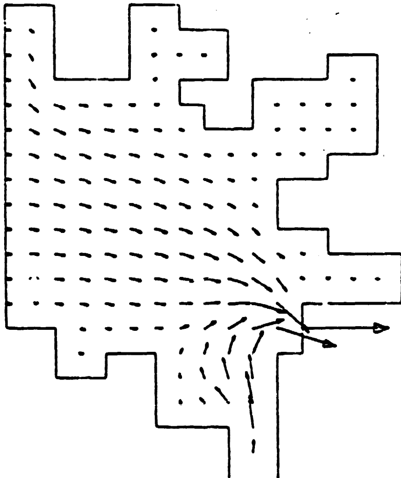
Figure 28. Velocities at K = 1, Lake Keowee (rigid-lid model)
