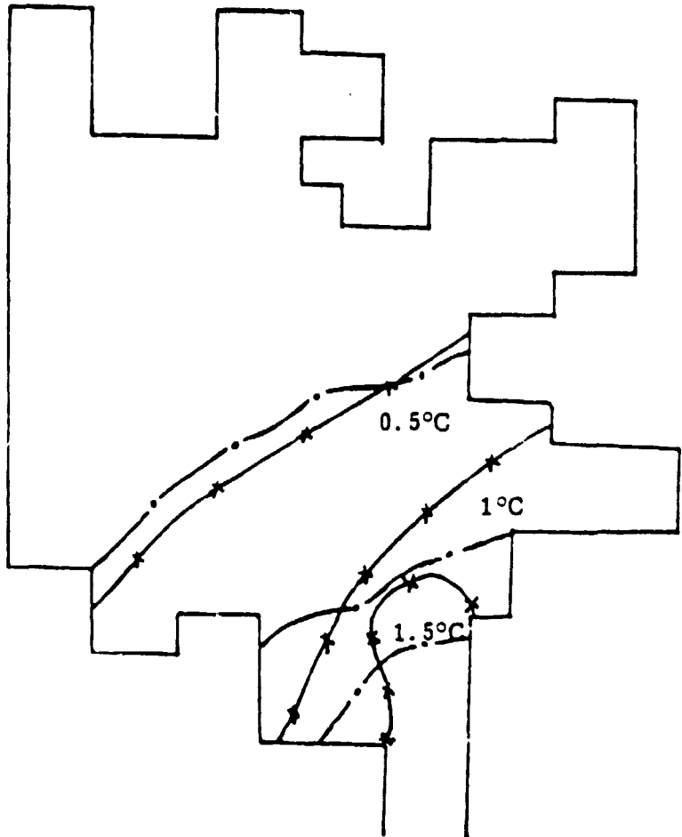
Figure 27. Isotherms: measured and predicted (temperatures above ambient)
