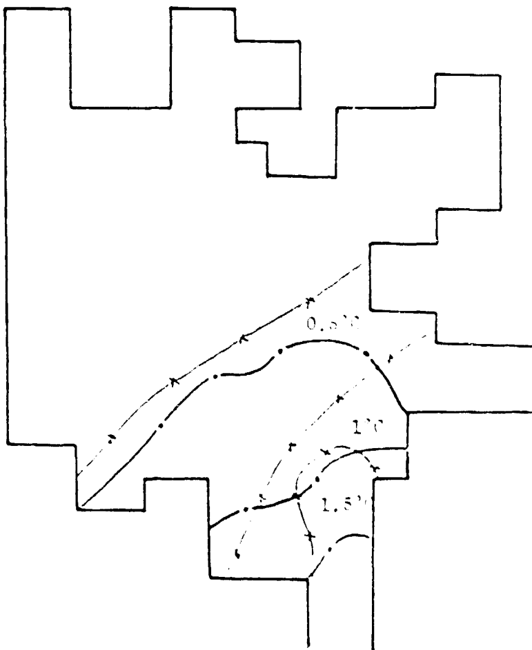
Figure 20. Isotherms: measured and predicted (temperatures above ambient)
