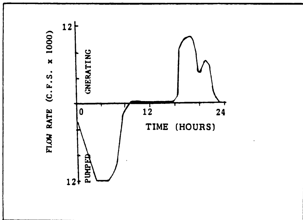
Figure 11. Jocassee-pumped storage station discharge data (August 24, 1978)
