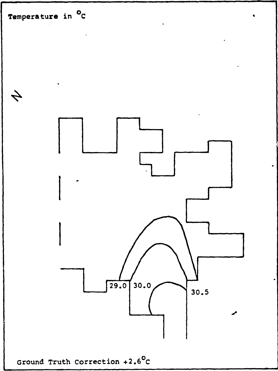
Figure 37. IR data corresponding to 0903-0953 hrs, August 25, 1978 Lake Keowee
