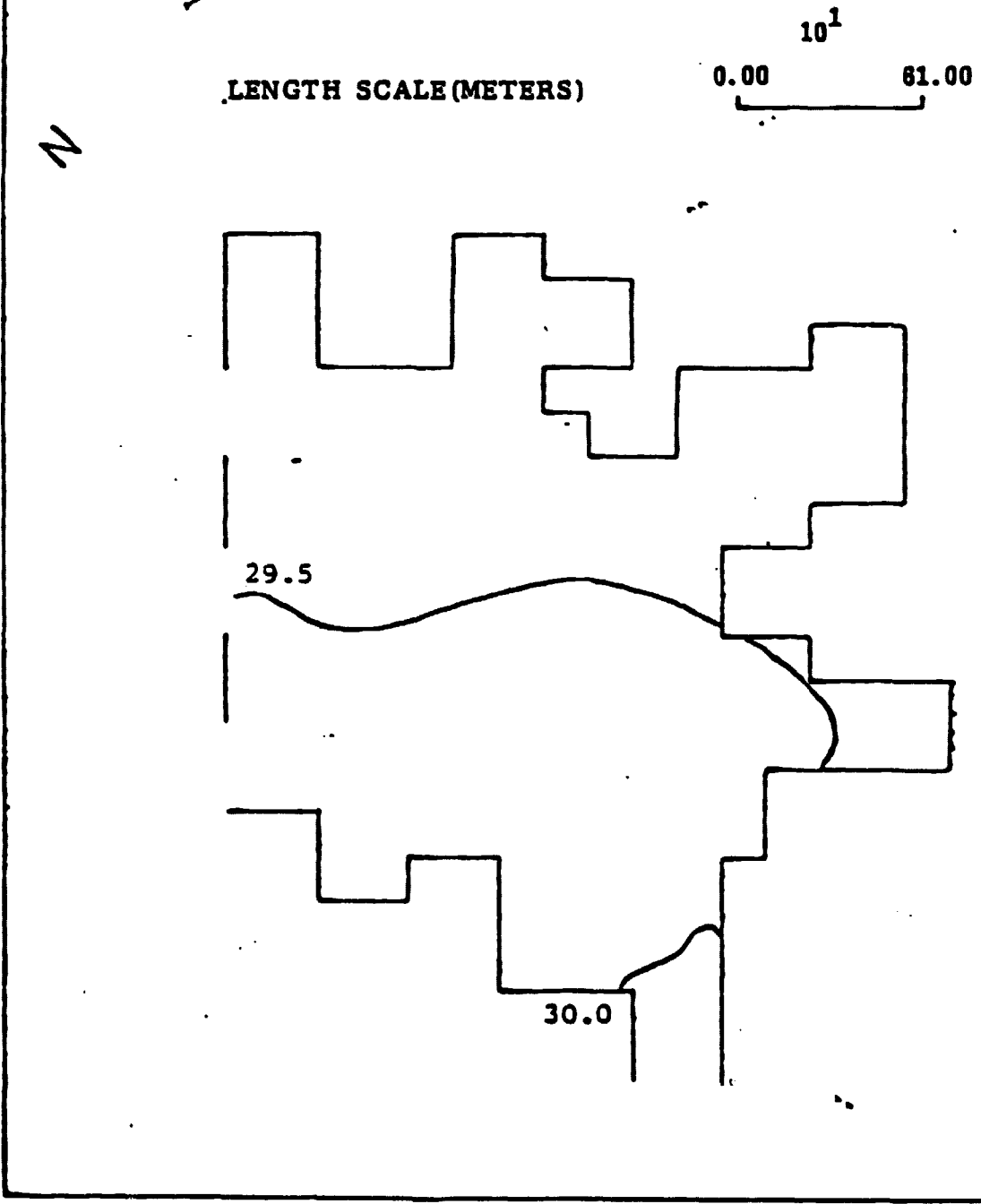
Figure 38. Isotherms at K = 1 , Lake Keowee (rigid-lid model), simulations for August 25, 1978
