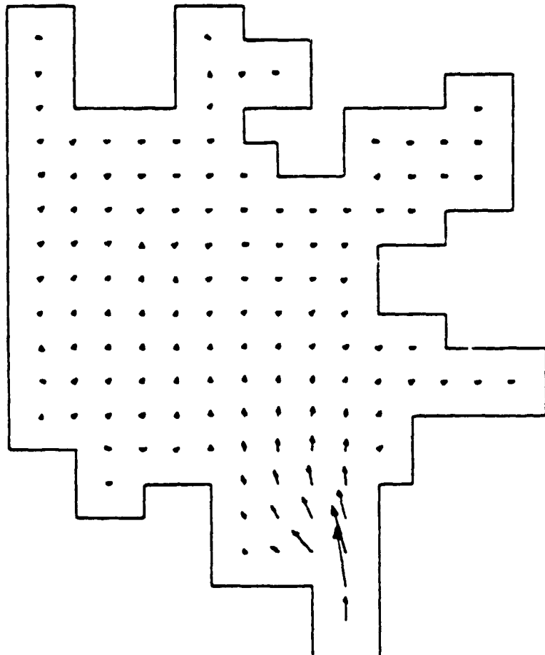
Figure 24. Velocities at K = 1, Lake Keowee (rigid-lid model)
