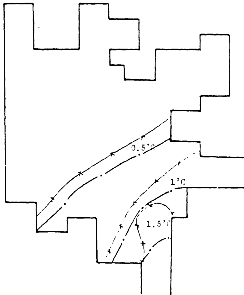
Figure 26. Isotherms: measured and predicted (temperatures above ambient)
