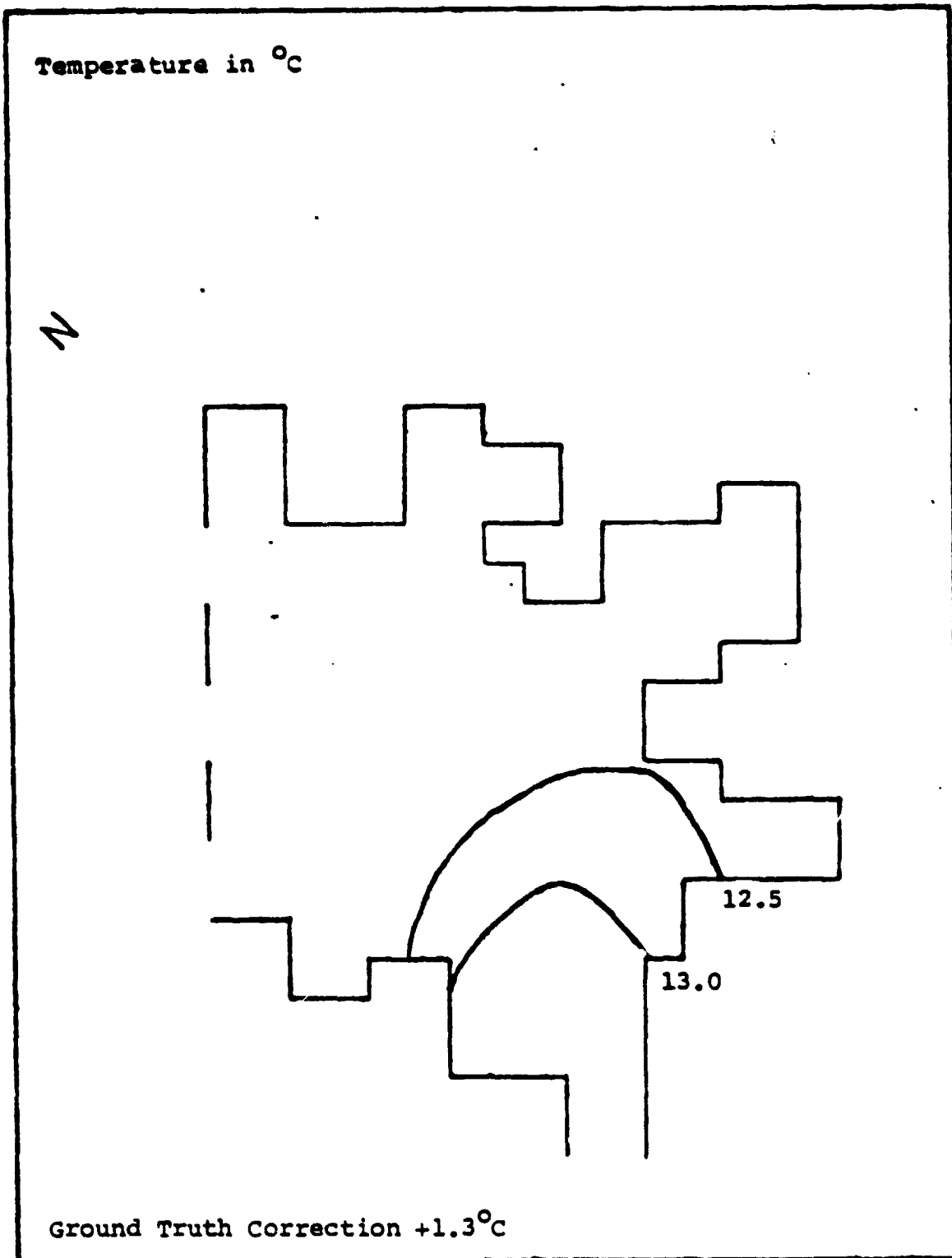
Figure 45. IR data corresponding to 0948-0957 hrs, February 28, 1979 Lake Keowee
