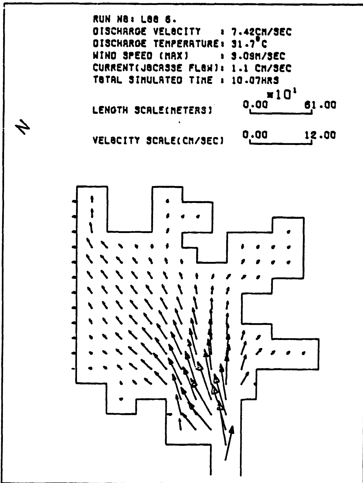
Figure 40. Velocities at K = 1 , Lake Keowee (rigid-lid model), simulations for August 24, 1978
