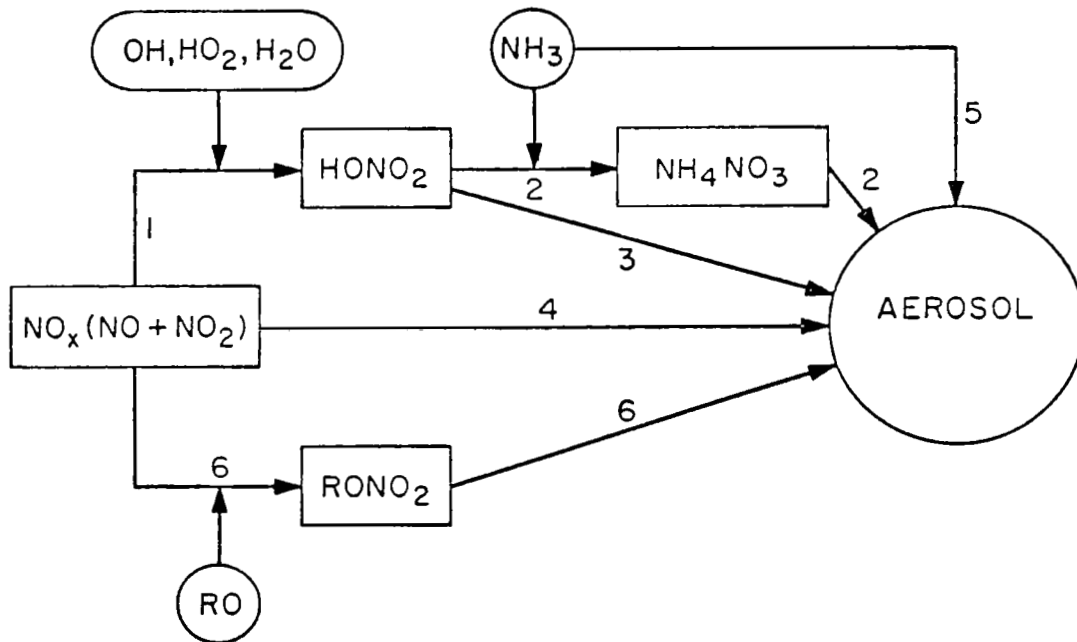
Figure A1.- Paths of nitrate formation in the atmosphere.
