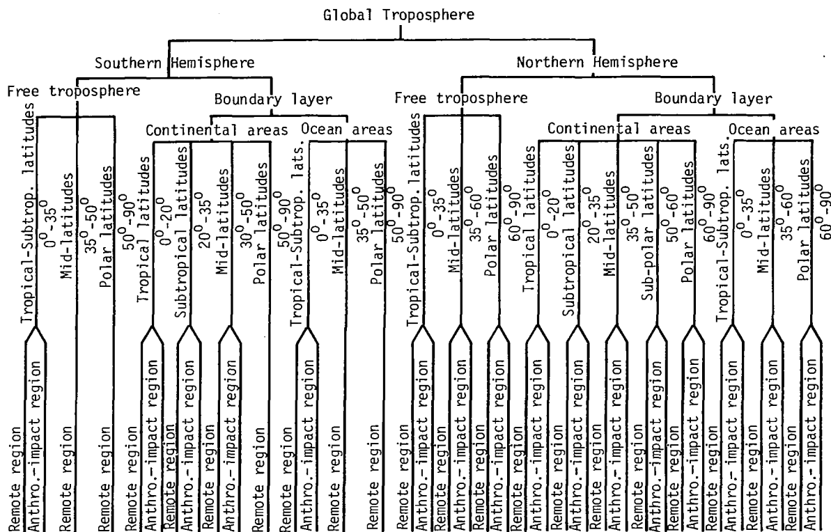
Figure 11.- A medium-resolution tropospheric distribution scheme.
