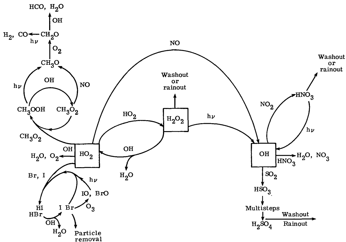
Figure 1.- Illustration of H_xO_y radical-loss paths.
