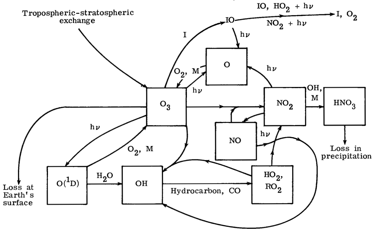
Figure 6.- Schematic diagram of the major sources and sinks of tropospheric ozone.
