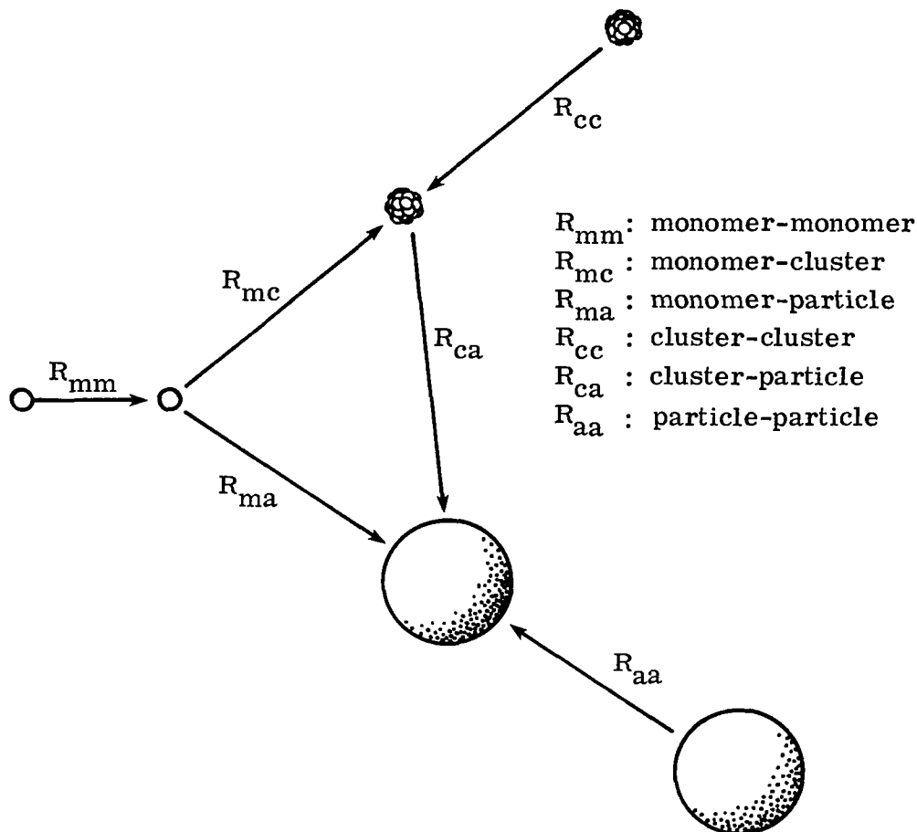
Figure 18.- Competitive processes involved in gas-to-particle conversion.
