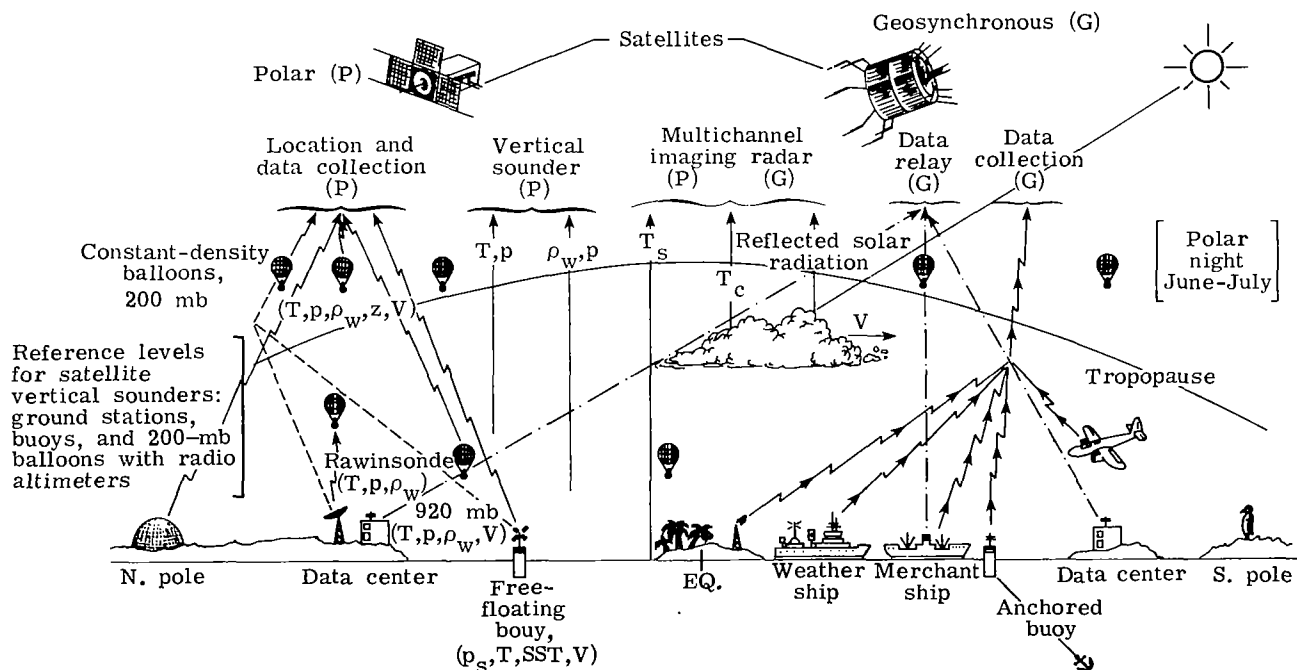
Figure C1.- Schematic of the Global Observing System. (Constant-density balloons are used only for special observations.)
