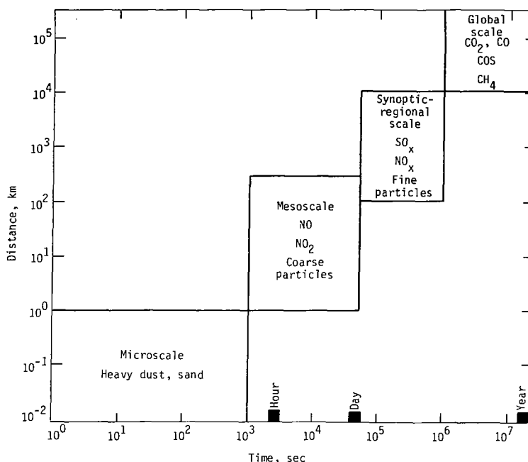
Figure 8.- Spatial and temporal scales relevant to tropospheric air pollutants.
