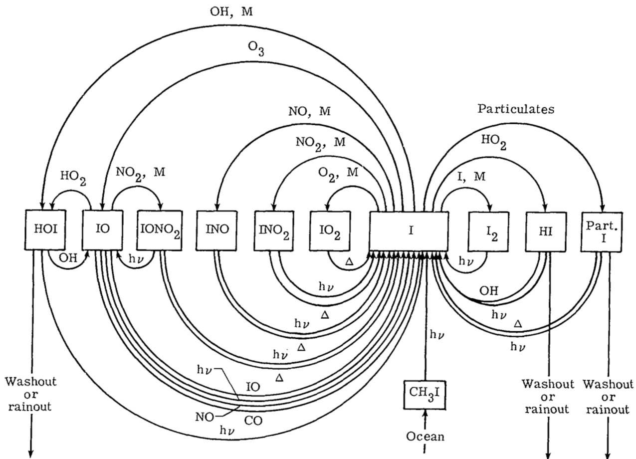
Figure 5.- A possible chemical scheme for iodine (I) in the tropospheric marine boundary layer.
