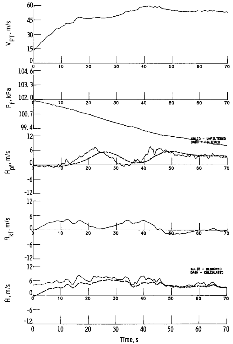
Figure 11.- Take-off; flight 2; run 1.
