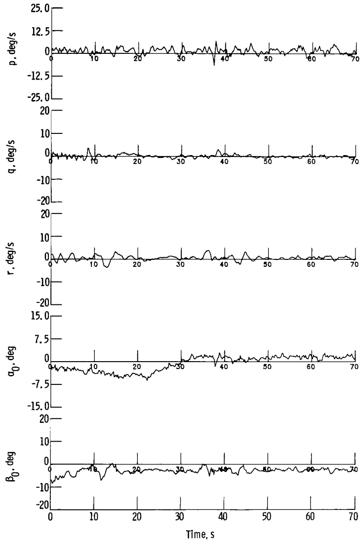
Figure 11.- Take-off; flight 2; run 1.
