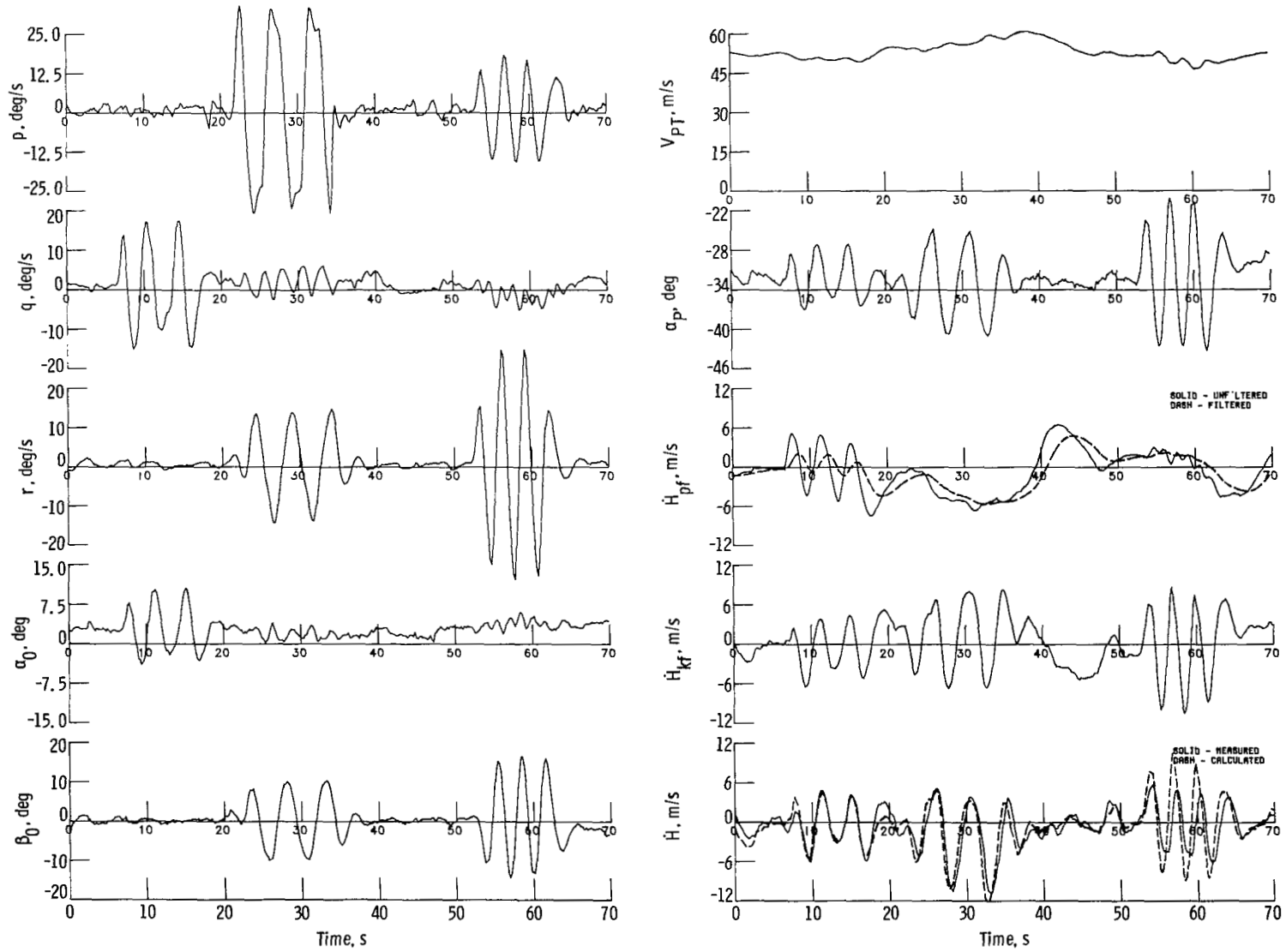
Figure 14.- Calibration maneuvers; flight 3; run 5.
