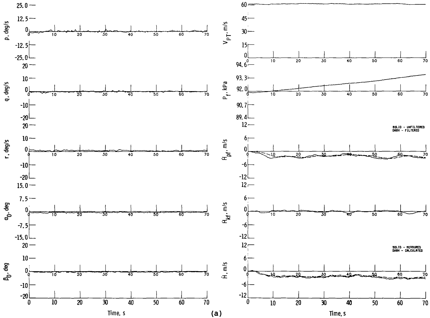
Figure 9.- Potential energy change; flight 1; run 5.
