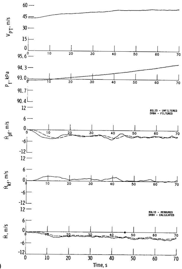
Figure 8.- Potential/kinetic energy exchange; flight 1; run 4.
