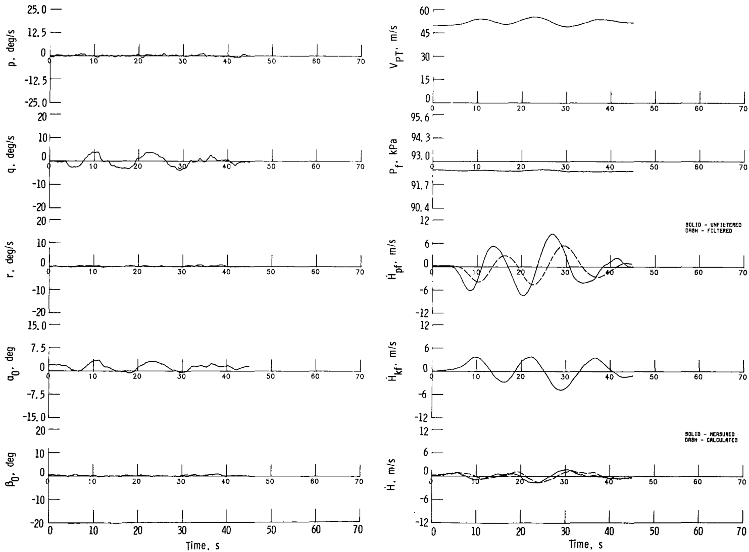
(a) Pitch maneuver.
