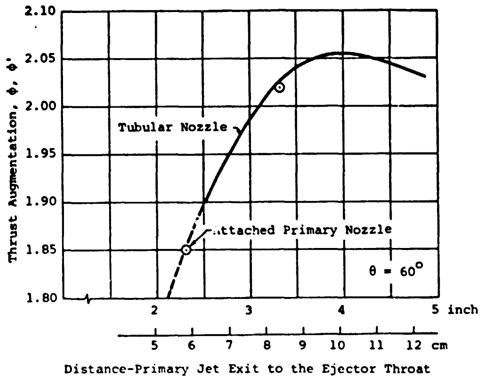
Figure 5. Influence of Primary Nozzle Location on Ejector Performance ( \theta = 60 deg.; see Figure 6 for definition of location)
