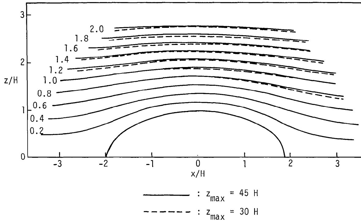
Figure 5.4 Streamline, \tilde{\psi} , patterns of flow over a semiellipse for D/H = 2.0 . (below \tilde{\psi} = 0.6 solutions coincide)
