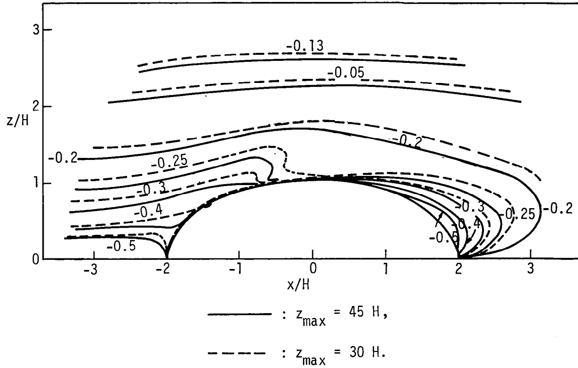
Figure 5.7 Vorticity, \tilde{\omega} , patterns for flow over a semiellipse for D/H = 2.0
