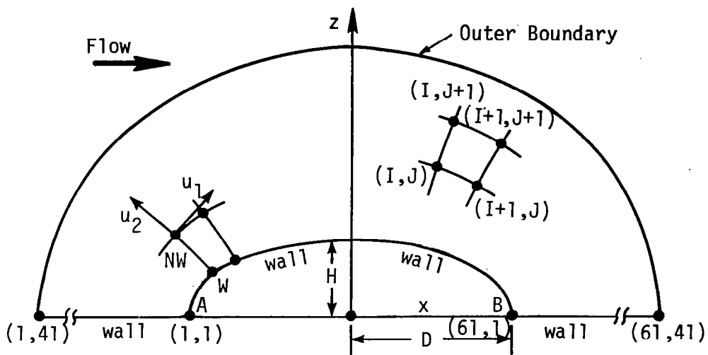
(a) Schematic diagram of the numerical coordinates used
