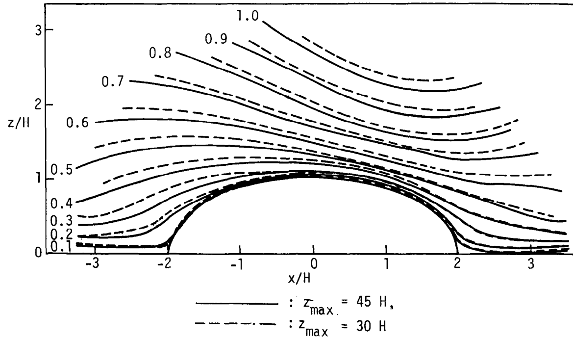
Figure 5.6 Distributions of turbulence length scale, \tilde{L} , for D/H = 2.0
