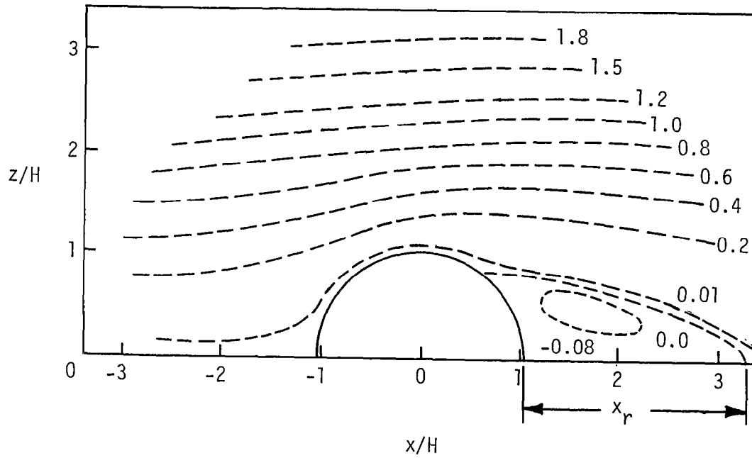
Figure 6.22 Streamline, \tilde{\psi} , patterns over a semiellipse for D/H = 1.02 , \tilde{z}_0 = 0.001 , and Re = 100
