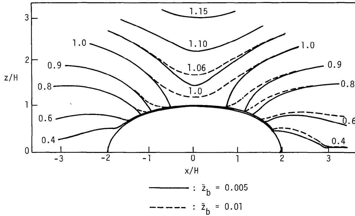
Figure 6.9 V/V_H isotachs over a semiellipse for D/H = 2.0 and \tilde{z}_0 = 0.005
