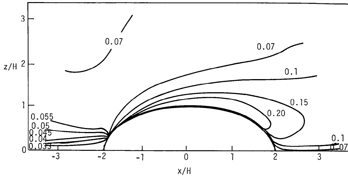
Figure 6.12 Distribution of turbulence kinetic energy, \tilde{K} , over a semi-ellipse for D/H = 2.0 , \tilde{z}_o = 0.01 , and \tilde{z}_b = 0.01
