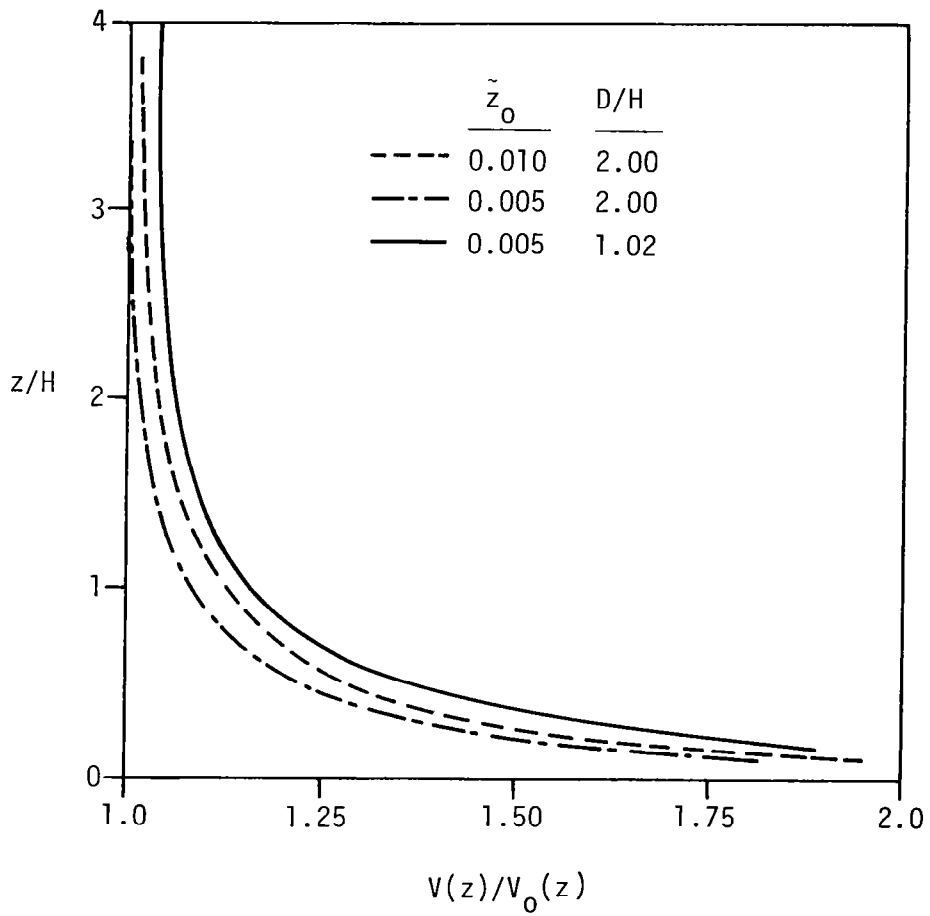
Figure 6.14 Wind speed-up ratio on top of semiellipses with different surface roughnesses and different aspect ratios
