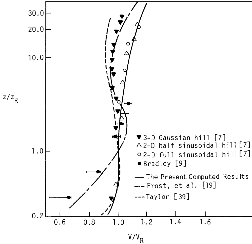
Figure 6.20 Vertical velocity profiles on the top of the respective obstacles shown in Figure 6.19
