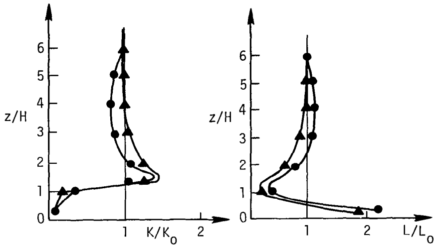
(a) Profile at 1.0 H behind a rectangular block
