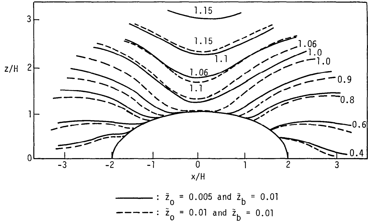
Figure 6.13 V/V_H isotachs over a semiellipse for D/H = 2.0
