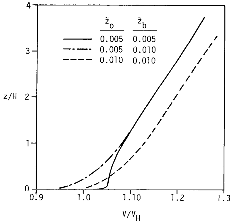
Figure 6.8 Velocity profiles on top of a semiellipse with different surface roughnesses for D/H = 2.0
