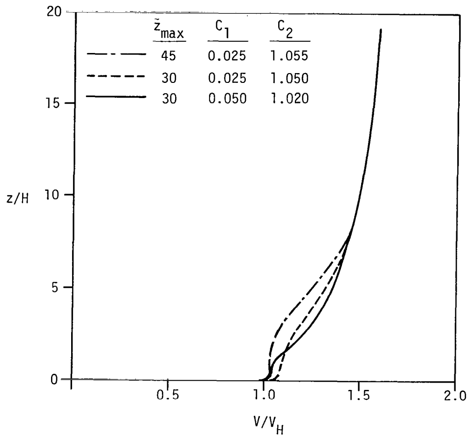
Figure 5.8 Velocity profiles on top of a semiellipse for D/H = 2.0 and \bar{z}_0 = 0.005
