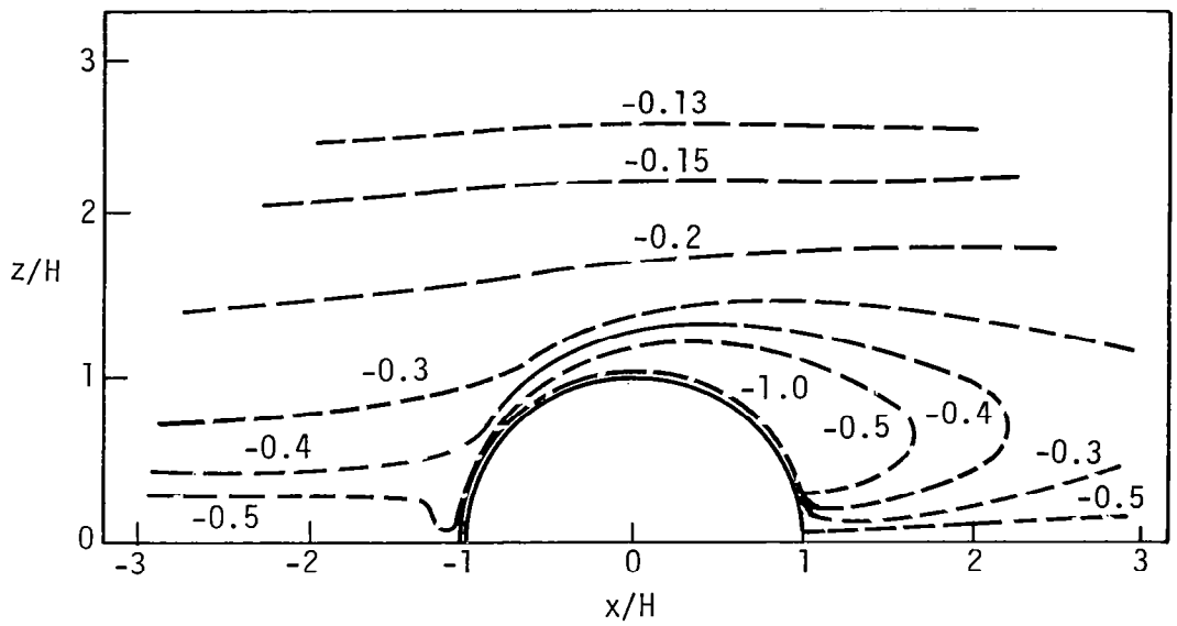
Figure 6.5 Vorticity, \tilde{\omega} , patterns over a semiellipse for D/H = 1.02 and \tilde{z}_0 = 0.005
