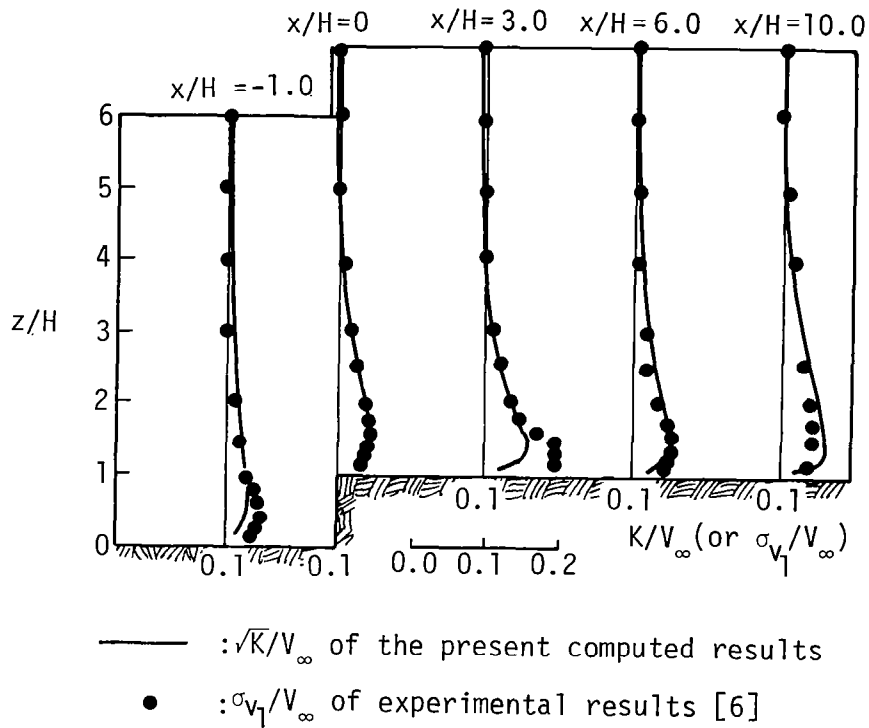
Figure 6.16 Turbulence intensity over a 90° escarpment
