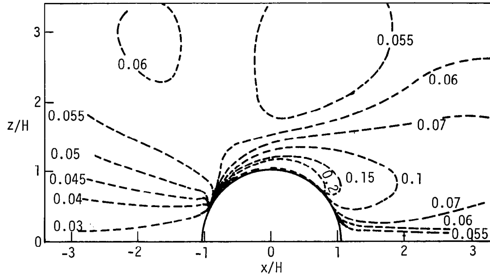
Figure 6.3 Distribution of turbulence kinetic energy, \tilde{K} , over a semiellipse for D/H = 1.02 and \tilde{z}_0 = 0.005
