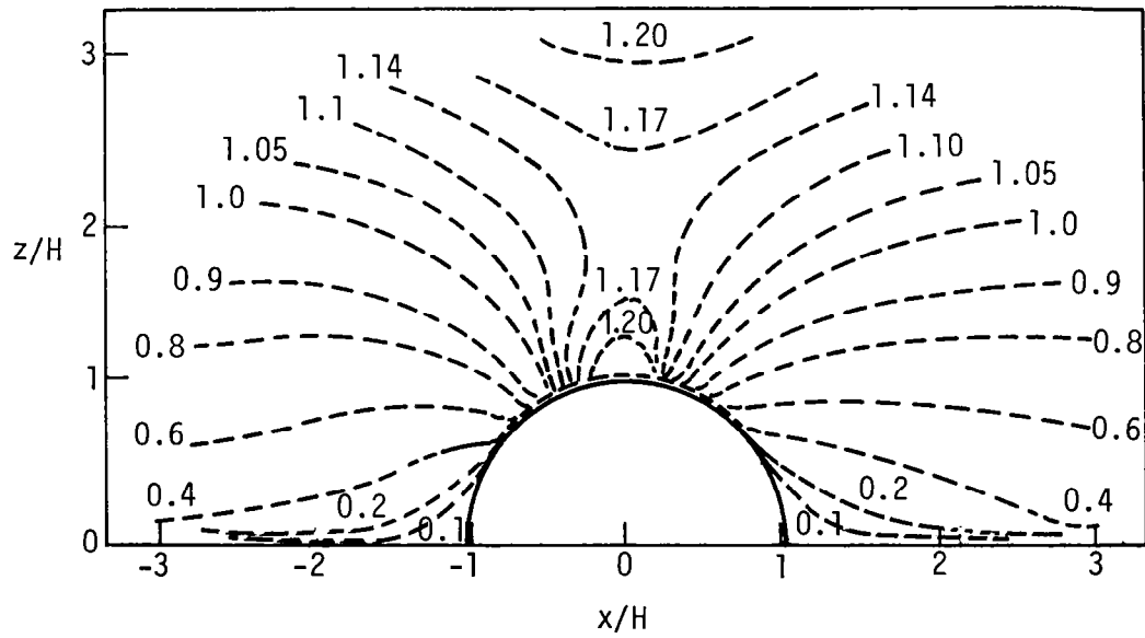
Figure 6.2 V/V_H isotachs over a semiellipse for D/H = 1.02 and \tilde{z}_0 = 0.005
