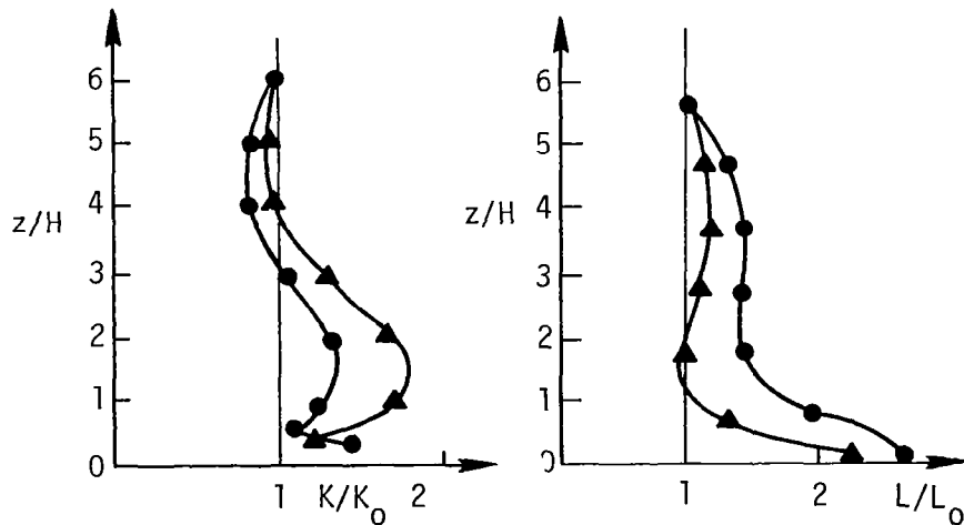
(b) Profile at 20.0 H behind a rectangular block
