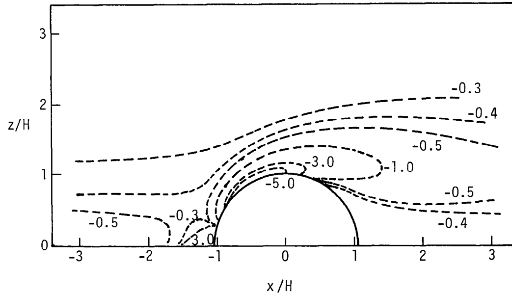
Figure 6.23 Vorticity, \tilde{\omega} , patterns over a semiellipse for D/H = 1.02 , \tilde{z}_0 = 0.001 , and Re = 100
