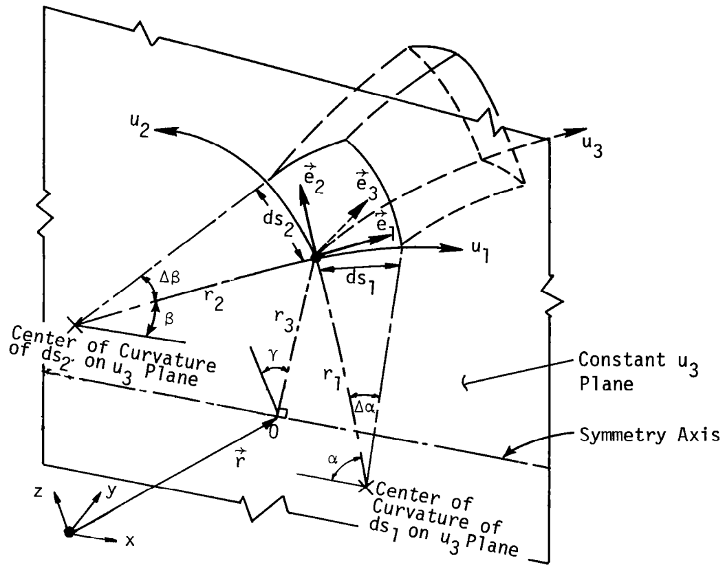
Figure 4.2 An axisymmetric coordinate system
