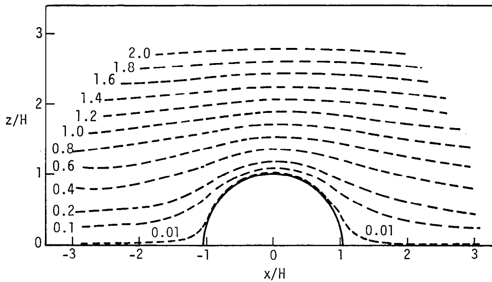
Figure 6.1 Streamline, \tilde{\psi} , patterns over a semiellipse for D/H = 1.02 and \tilde{z}_0 = 0.005
