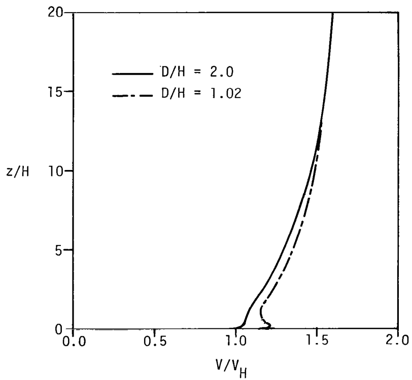
Figure 6.7 Velocity profiles on the top of semiellipses of different aspect ratios for \tilde{z}_0 = 0.005
