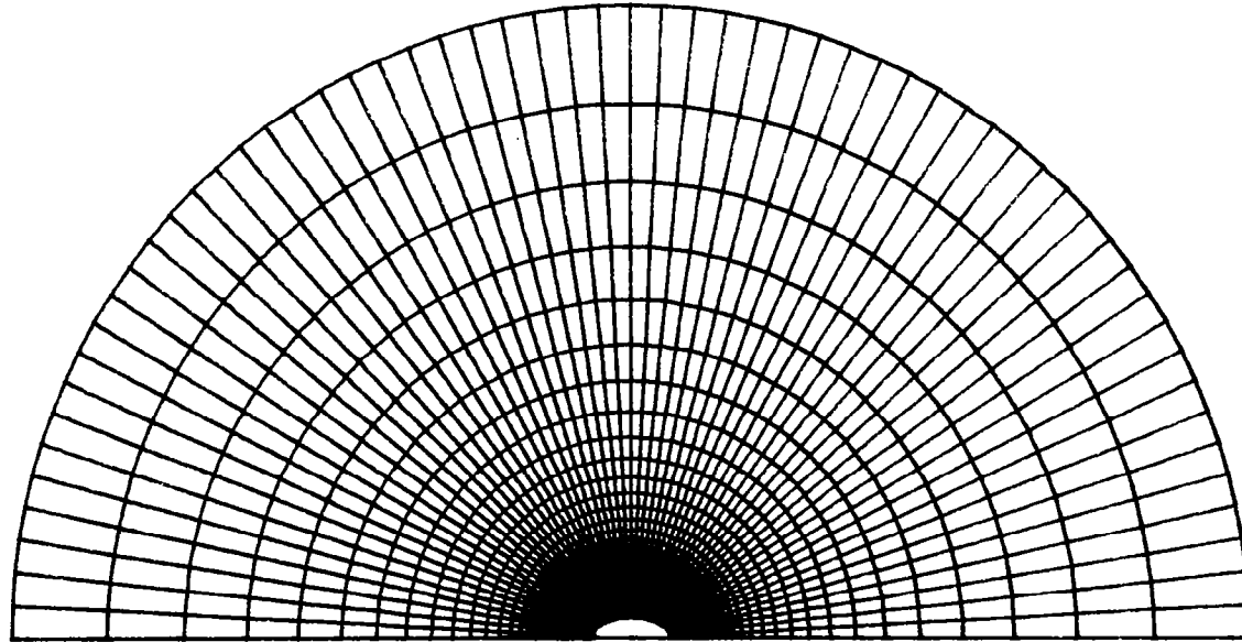
Figure 5.3 Distribution of grid sizes for D/H = 2.0 , C_1 = 0.025 , C_2 = 1.05
