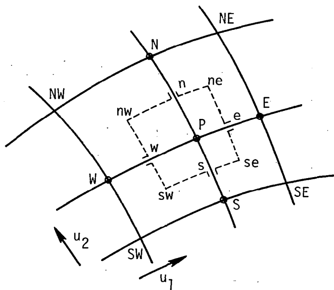
Figure 5.1 Grid arrangement with respect to the central node P
