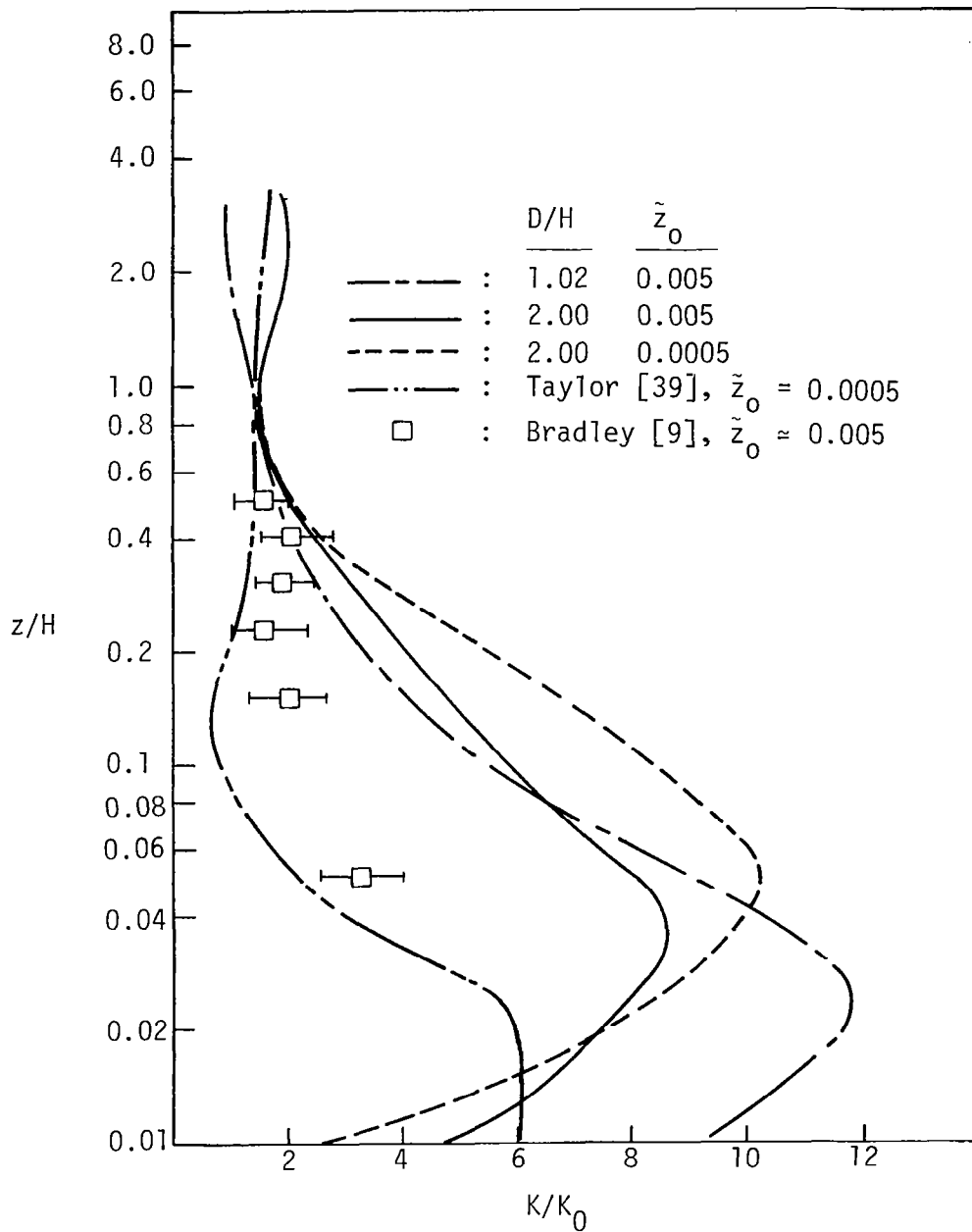
Figure 6.21 Distribution of dimensionless turbulence kinetic energy, K/K_0 , on top of semiellipses with different \tilde{z}_0 and D/H ratios
