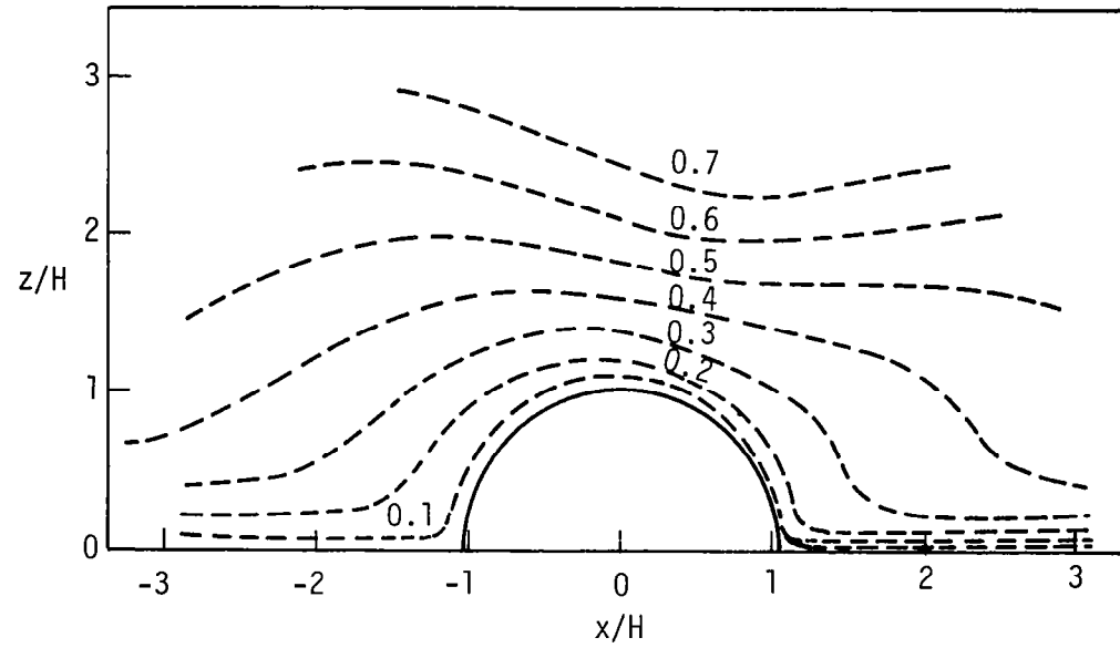
Figure 6.4 Distribution of turbulence length scale, \tilde{L} , over a semiellipse for D/H = 1.02 and \tilde{z}_0 = 0.005
