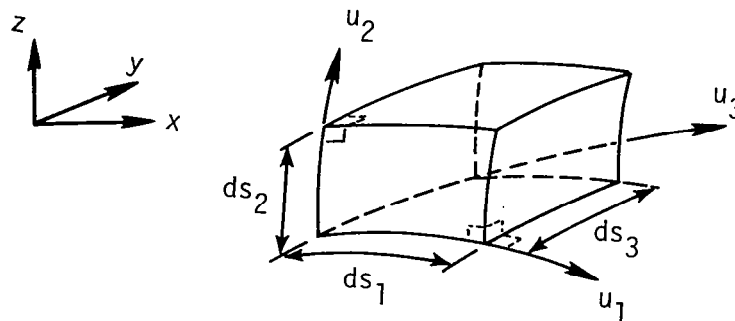
Figure 4.1 An orthogonal curvilinear coordinate system
