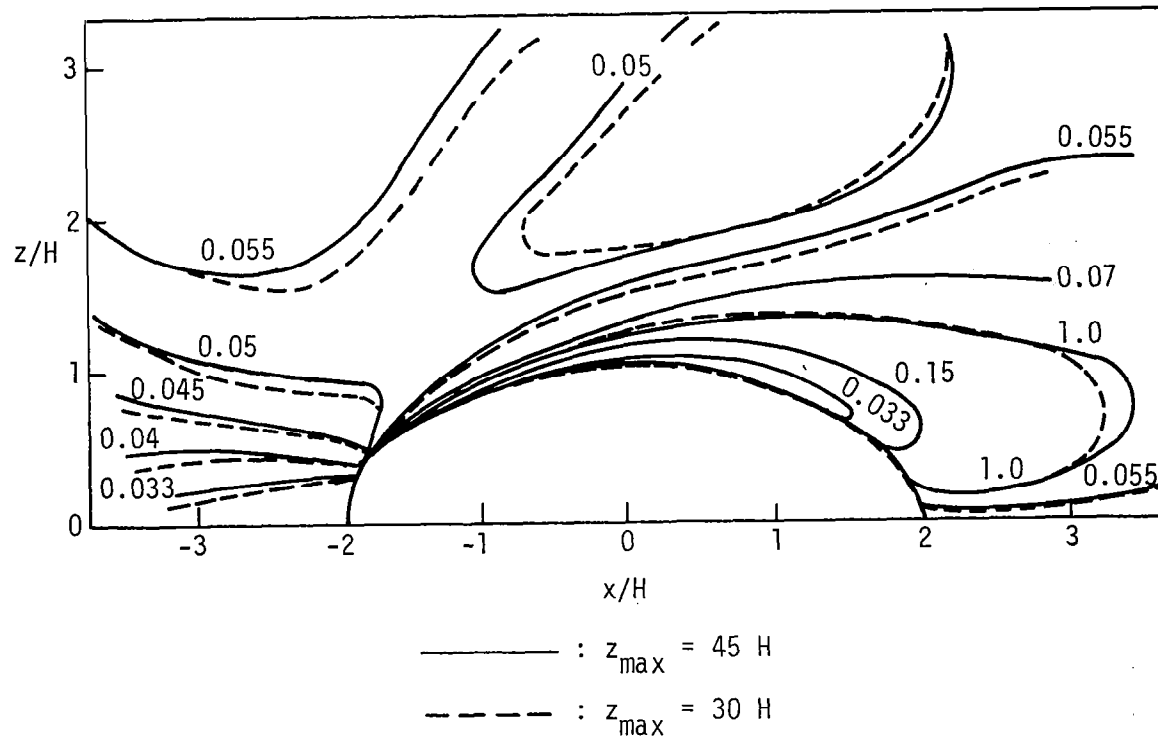
Figure 5.5 Distribution of turbulence kinetic energy, \tilde{K} , for D/H = 2.0
