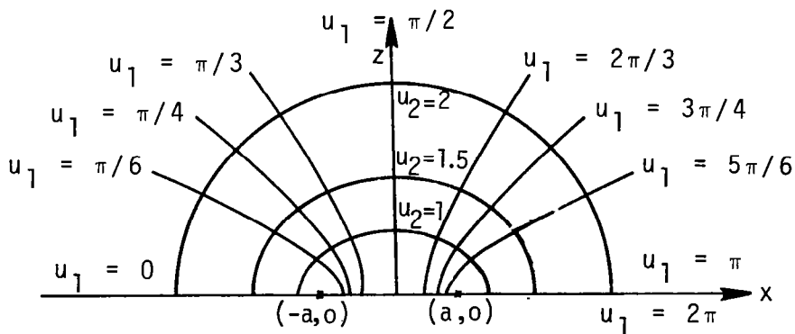
(b) Two-dimensional semielliptic coordinate system
