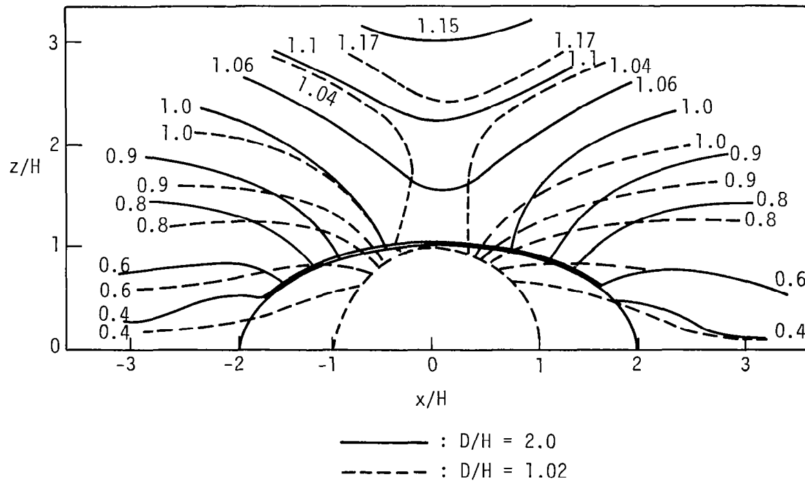
Figure 6.6 V/V_H isotachs over semiellipses for \tilde{z}_0 = 0.005
