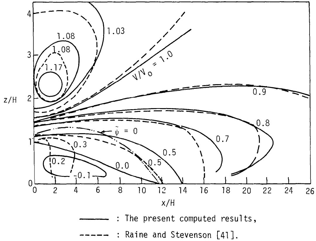
Figure 6.18 V/V_0 isotachs downstream of a solid fence, \tilde{z}_0 = 0.01
