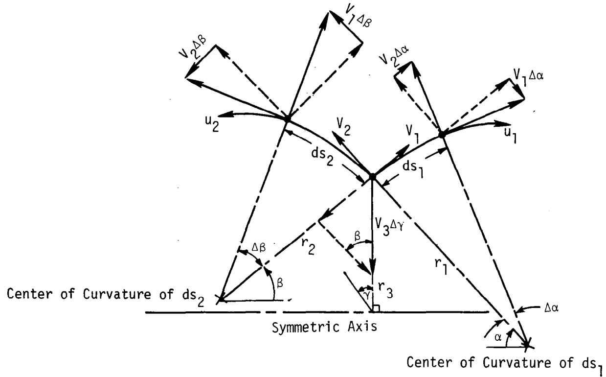
Figure 4.3 Velocity vectors of a fluid element shown in a constant u_3 plane (reference Figure 4.2).
