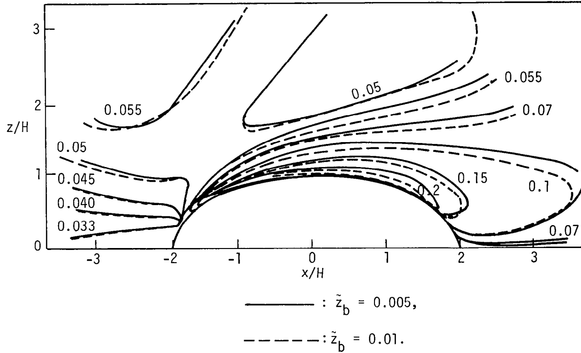
Figure 6.11 Distribution of turbulence kinetic energy, \tilde{K} , over a semi-ellipse for D/H = 2.0 and \tilde{z}_0 = 0.005
