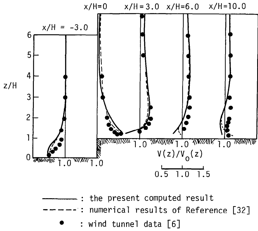
Figure 6.15 Wind speed-up ratio over a 90° escarpment
