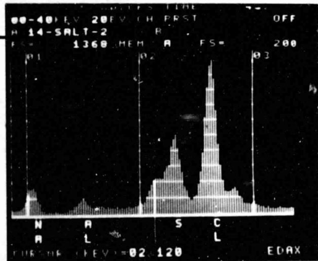
NA 2 SO 4 PARTICLES EXPOSED TO AIR AND 0.99% SO 2 AT 600 0 C. FOR 30 MINUTES.
