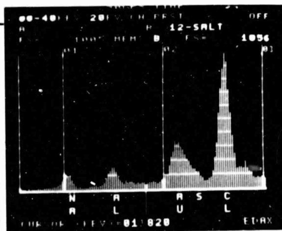
NA CL PARTICLE EXPOSED TO AIR PLUS 0.2% SO 2 AT 500 0 C. FOR TWO HOURS. FIGURE 7
