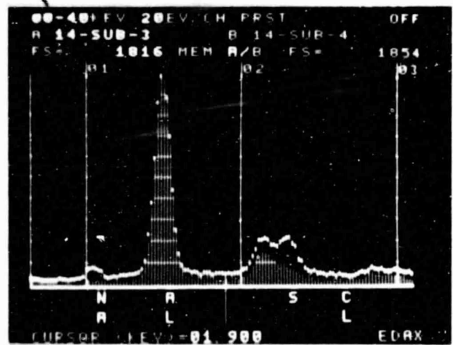
EDAX OF Al_2O_3 SUBSTRATE; SULFUR CONTENT PRESENT.
