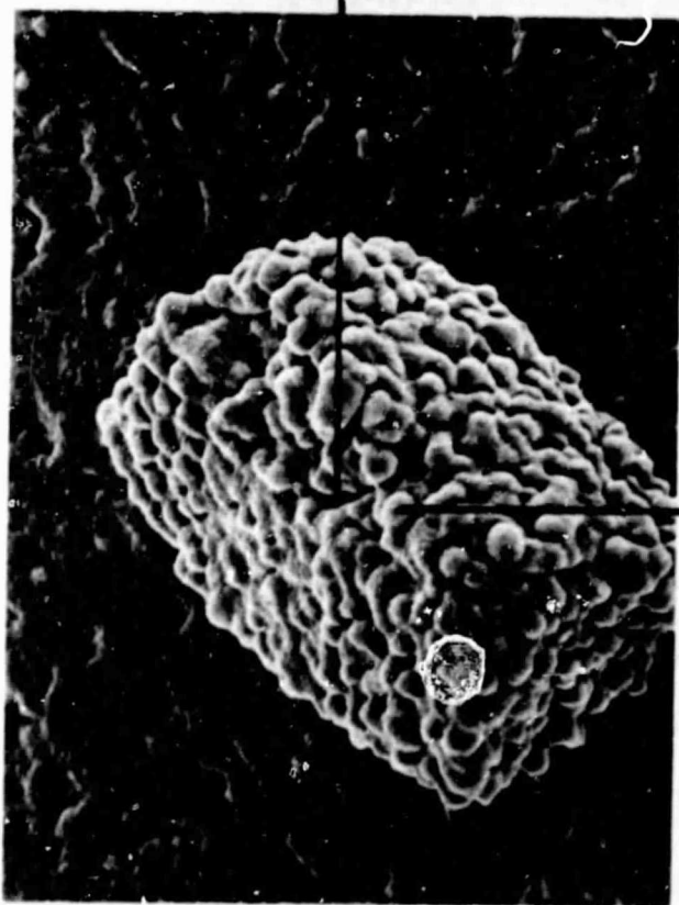
NACL PARTICLE EXPOSED TO AIR AND 0.2% SO 2 AT 600 0 C. FOR TWO HOURS. FIGURE 12
