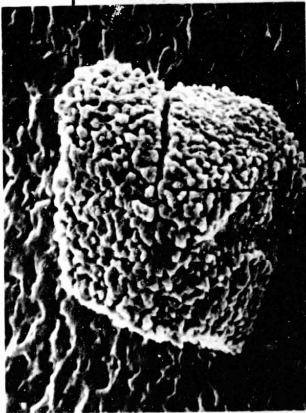
NA 2 SO 4 PARTICLES EXPOSED TO AIR AND 0.99% SO 2 AT 600 0 C. FOR 30 MINUTES.
