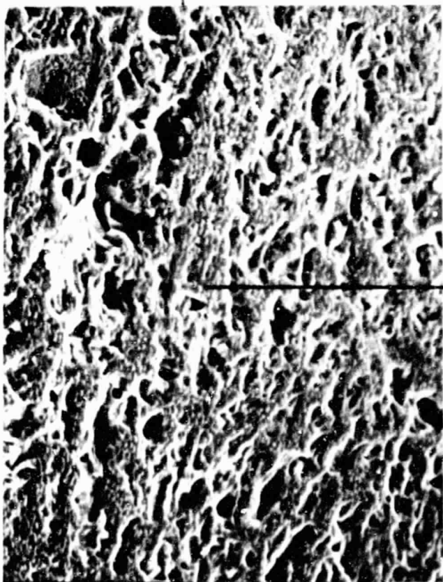
NaCl PARTICLES EXPOSED TO AIR AND 0.99% SO_2 AT 600^{\circ}C . FOR 30 MINUTES. FIGURE 18
