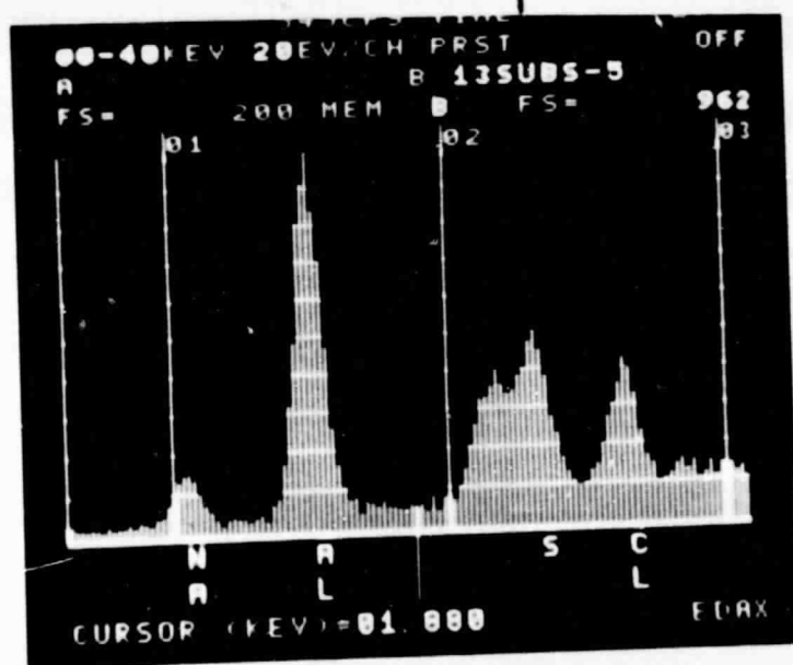
NA CL PARTICLES EXPOSED TO AIR AND 0.99% SO 2 AT 600 0 C. FOR 10 MINUTES. FIGURE 16
