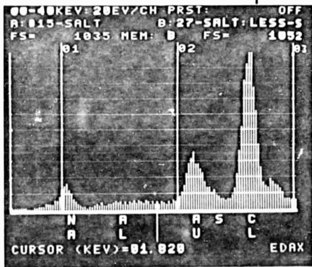
EDAX OF NA CL PARTICLE; SULFUR PRESENCE INDICATED.
