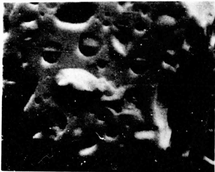
FIGURE 17 NACL PARTICLE EXPOSED TO AIR AND 0.99% SO 2 AT 600° C. FOR 10 MINUTES.
