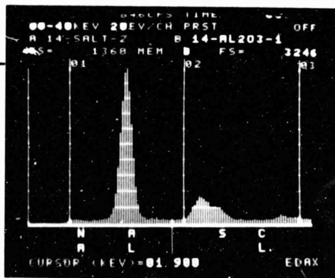
NaCl PARTICLES EXPOSED TO AIR AND 0.99% SO_2 AT 600^{\circ}C . FOR 30 MINUTES. FIGURE 18
