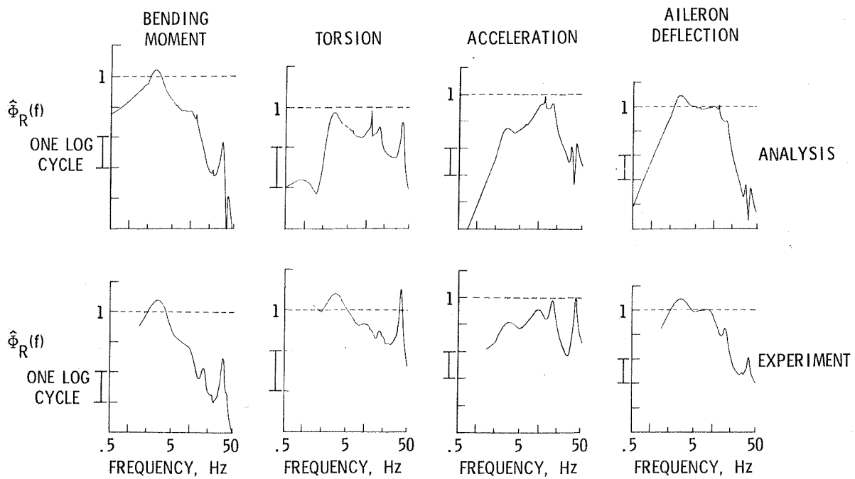
Fig. 6 Normalized power spectral density functions. System on, K_g = 1.0 , \phi = 0^0 ; 30.87 m/sec.
