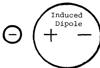
Figure 3.4 Dipole induced in spherical particle due to presence of nearby charged particle [3-9].
