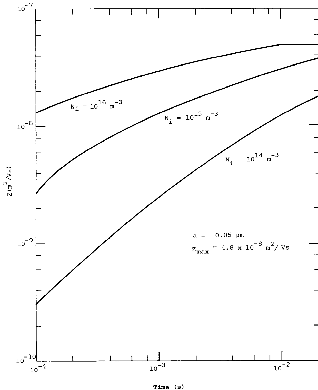
Figure 3.11 (continued).
