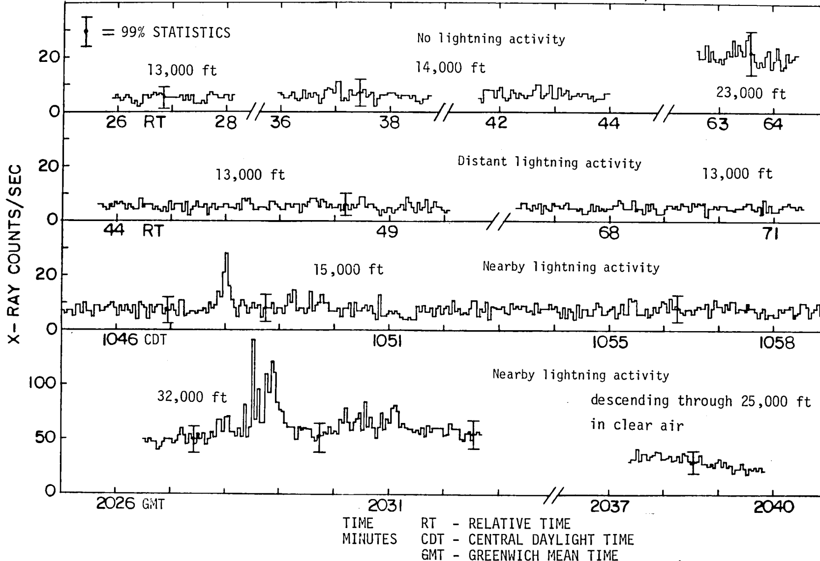
Figure 11.- X-ray activity with and without lightning.
