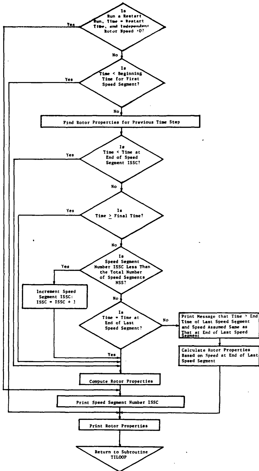
Figure 31. Flow Chart for Subroutine ROPROP.
