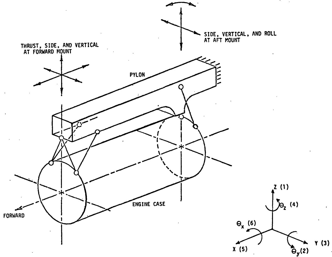
Figure 40. Typical Mounting Arrangement and Coordinate System.
