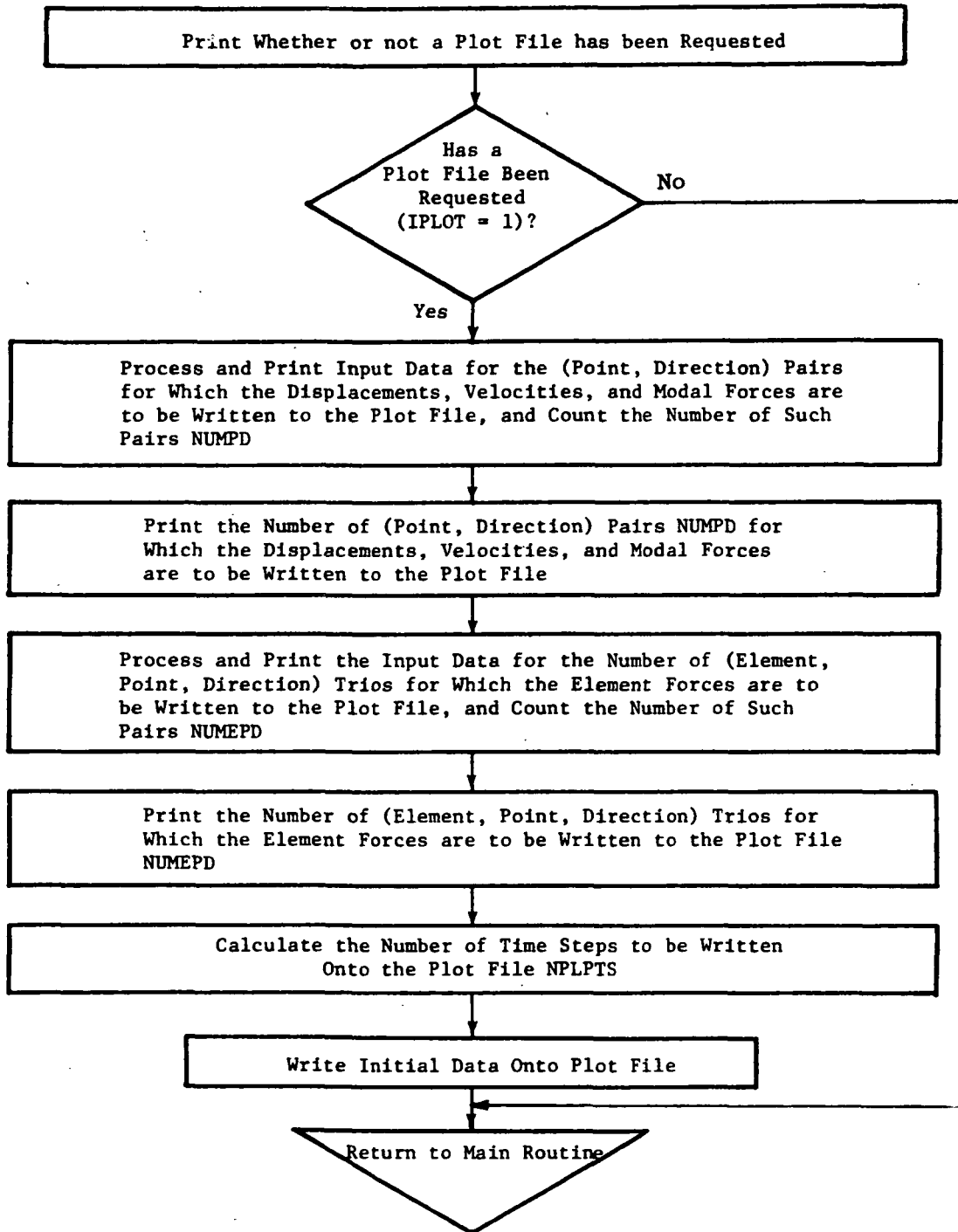
Figure 28. Flow Chart of Subroutine PLOTD.
