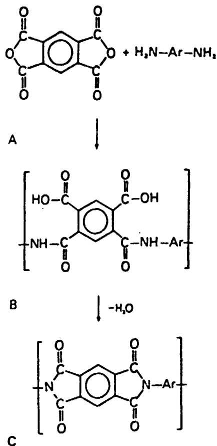
Figure 2. Polyimide synthesis.
