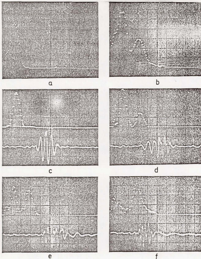
Figure 5 Integrated Spectra of a Portion of the Signal Obtained: a) Flat Plate, 2a = 0 , at x^* = 50 mm and y = 0.1 mm b) Deformed Plate, 2a = -1 , at x^* = 50 mm and y = 0.1 mm Unstable Bursts Characteristic of the Hot Wire Signals and their Instantaneous Spectra ( U_\infty = 16 m/sec): c) Flat Plate; d,e,f) Deformed Plate
