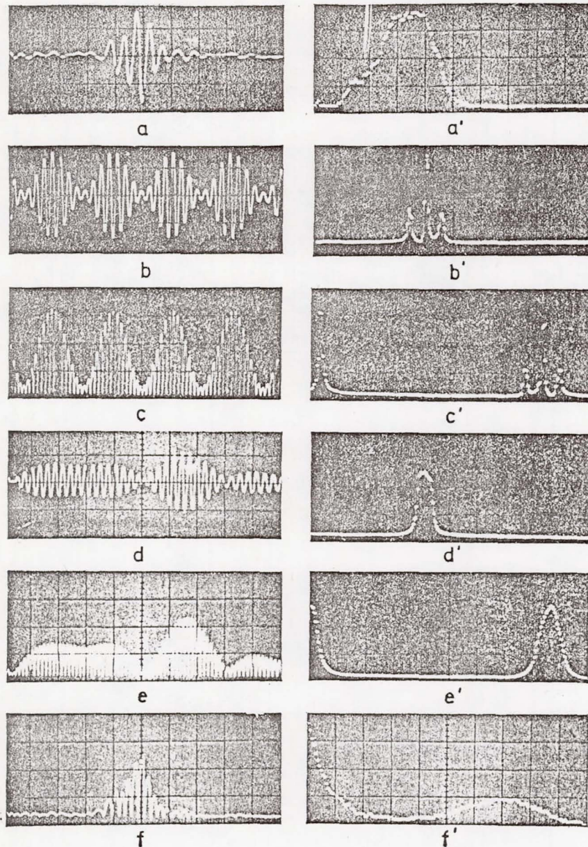
Figure 7 Amplitude Modulation by a Low Frequency Spectrum Time Scale: 8 \times 10^{-3} sec/square for Instantaneous Signals, 100 Hz/square for Spectra a) Unstable Burst on a Flat Plate for a Reynolds Number of 1110 b) Sinusoid with Amplitude Modulation c) Signal b after Full Wave Rectification d) Sinusoid Modulated by Narrow Band Noise e) Signal d after Full Wave Rectification f) Unstable Burst in a after Full Wave Rectification a',b',c',d',e', f': Spectra of Signals a,b,c,d,e,f, Respectively
