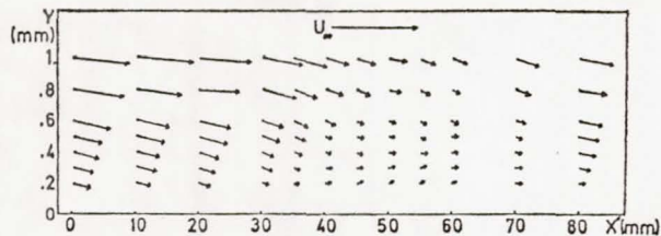
Figure 14 Representation of Velocity Vector in the Wall Deforma- tion Zone, 2a = -1 mm ( U_{\infty} = 16 m/sec)
