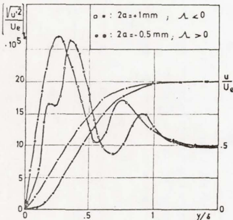
Figure 8 Energy of f_1 Instabilities vs. y/\delta and Profiles of Corresponding Average Speeds
