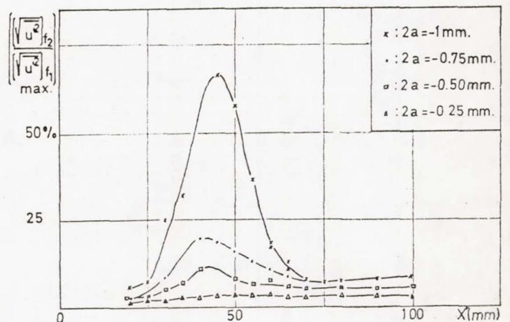
Figure 12 Harmonic Rate vs. Abscissa ( U_\infty = 16 m/sec)
