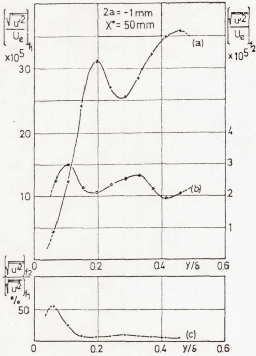
Figure 10 Ordinate Dependency of Energy of Instabilities at Frequencies f_1 (a) and f_2 (b) and of the Har- monic Rate (c) U_\infty = 16 m/sec, 2a = -1 mm, x^* = 50 mm, \delta_B = 2.27
