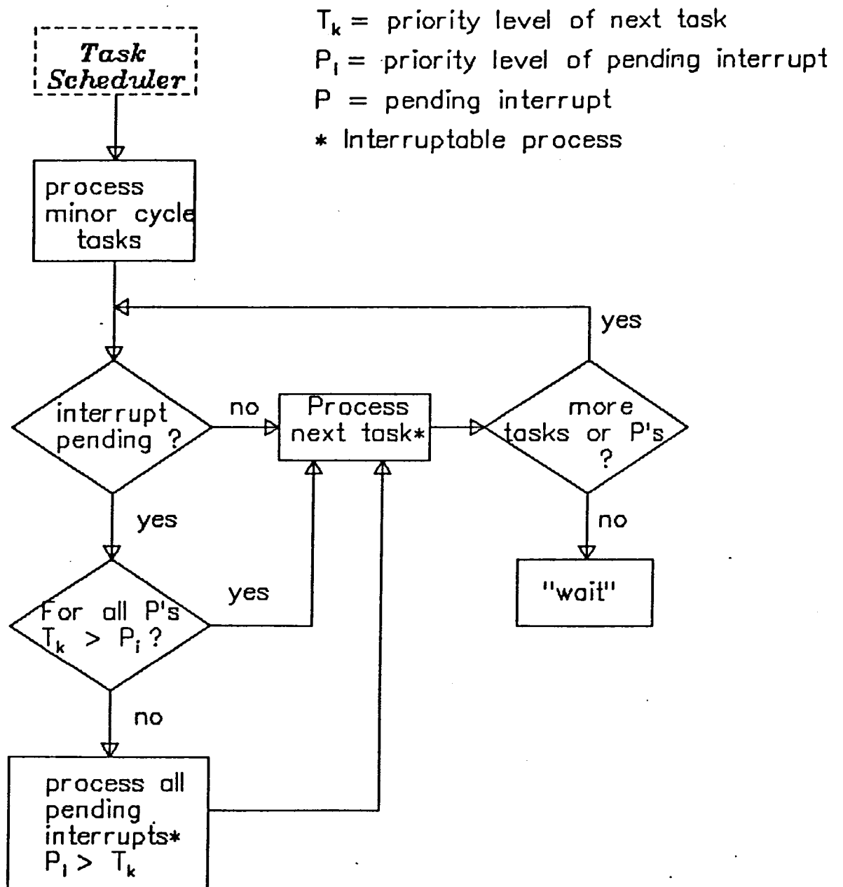
FIGURE 3 - Task Scheduler
