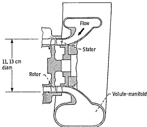
Figure 1 - Cross section of compressor-drive turbine.
