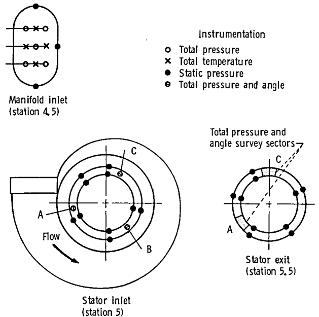
Figure 6. - Flow path measurements, viewed looking downstream.
