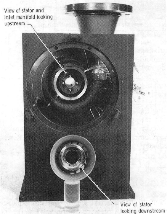
Figure 2. - Inlet-manifold and stator test hardware.
