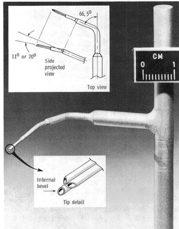
Figure 8. - Stator-exit survey probe.
