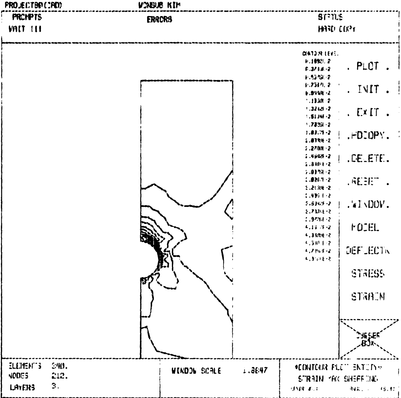
Figure I-33 Maximum Shear Strain Contour (Contact Angle 40°, Applied Load 3,000 lb.)
