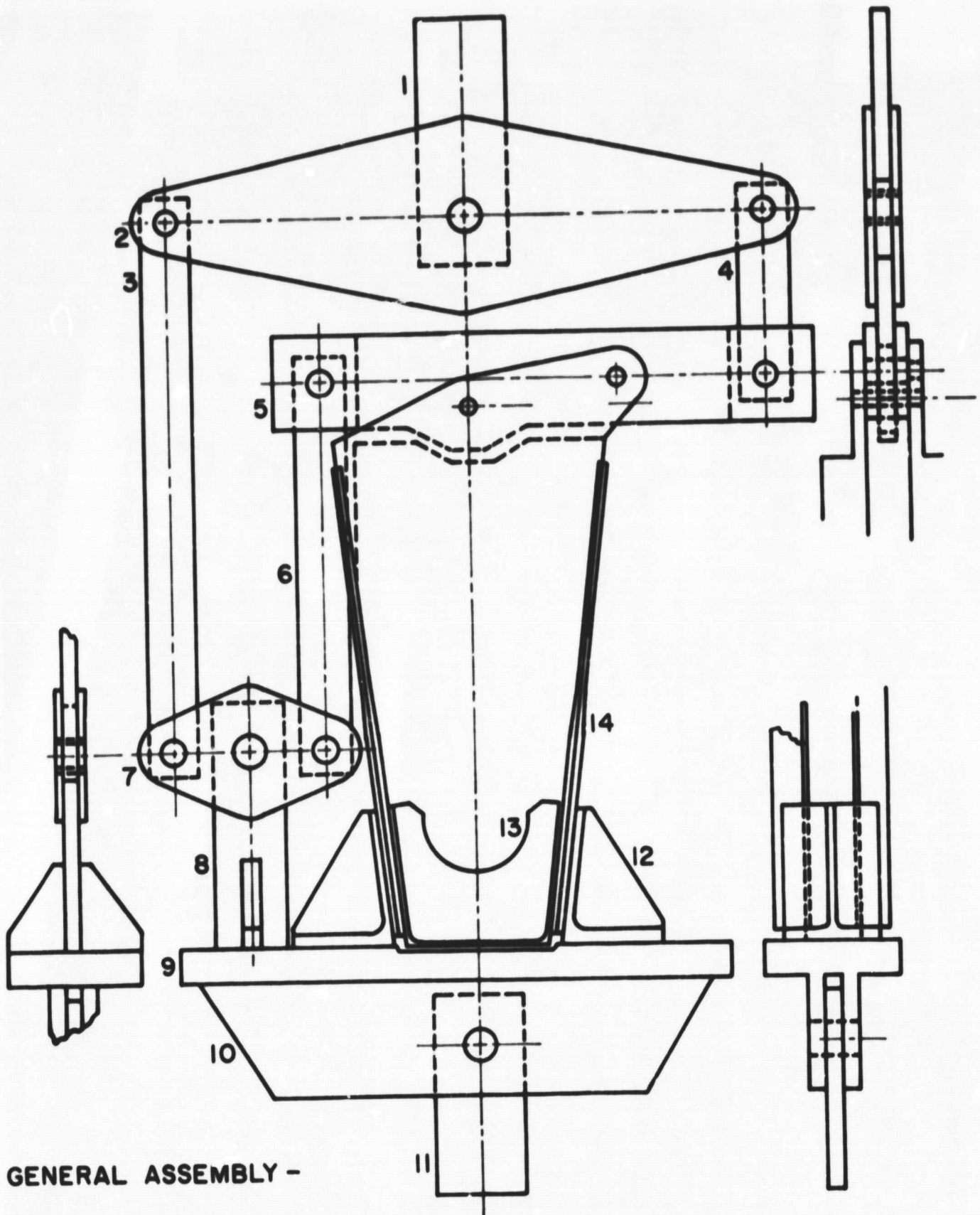
Figure I-9 Rib Test Fixture
