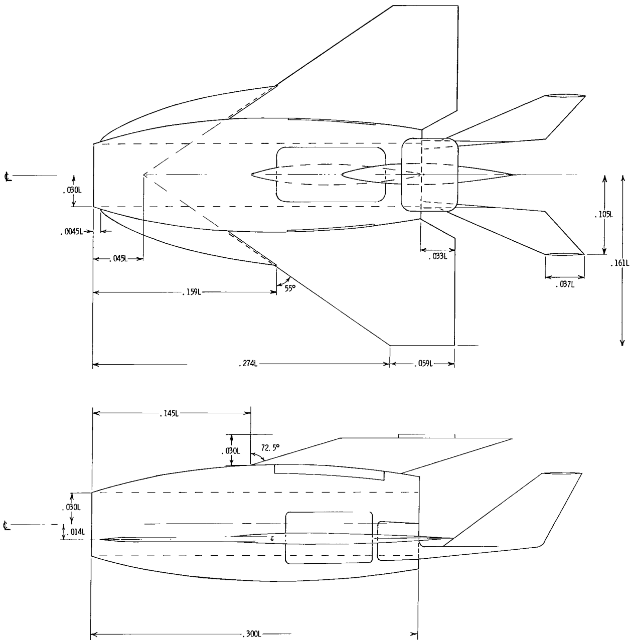
Figure 4.- Spacejet booster wind-tunnel model. L = 0.701 m.
