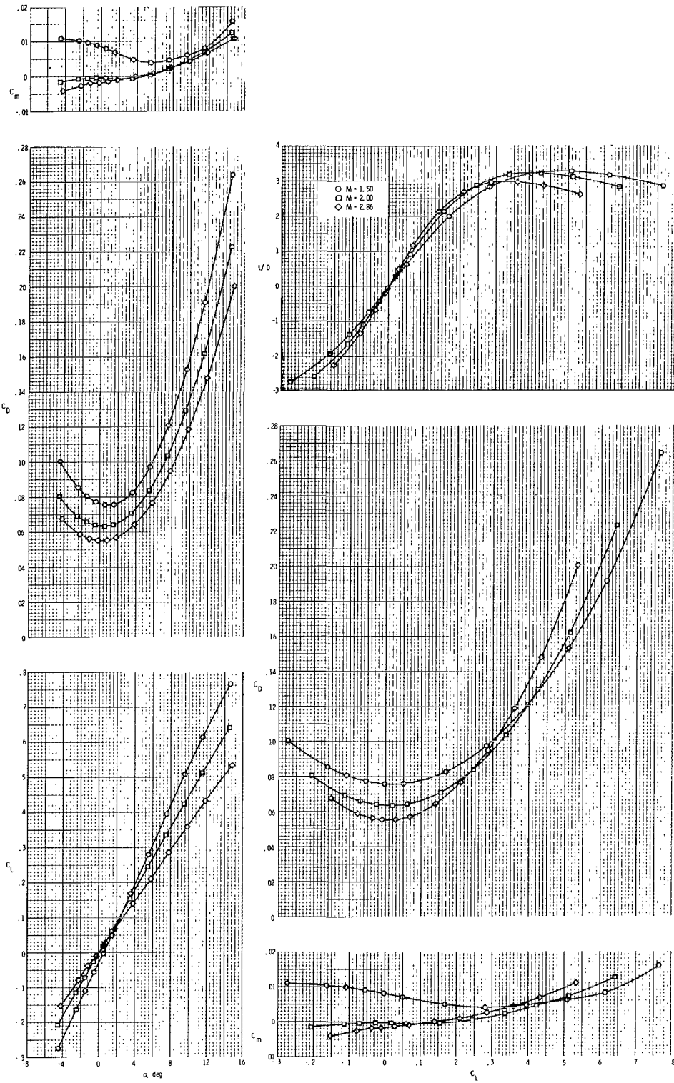
Figure 17.- Experimental aerodynamics at \beta = 3^\circ for O(B+W+S+F)LW + B(P+W+S+F)IN configuration.
