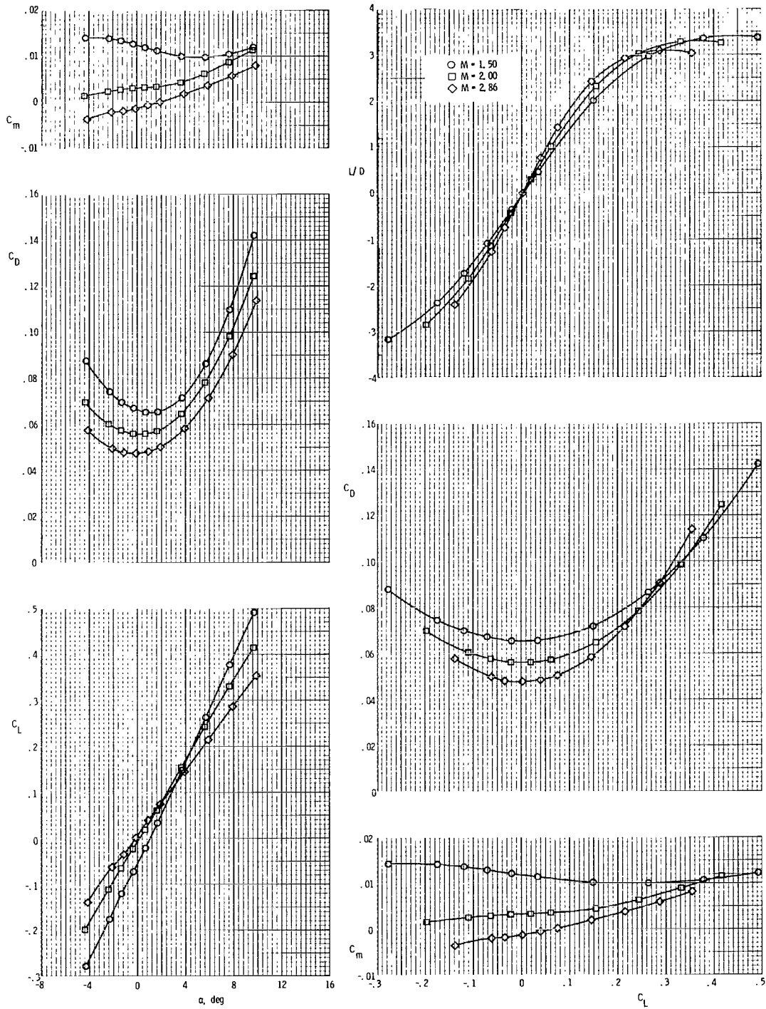
Figure 28.- Experimental aerodynamics at \beta = 0^\circ for O(B+W+S)HW + B(P+W+S)IN configuration.
