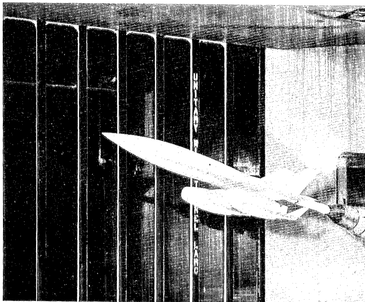
Figure 2.- Photograph of model in Langley Unitary Plan Wind Tunnel.
