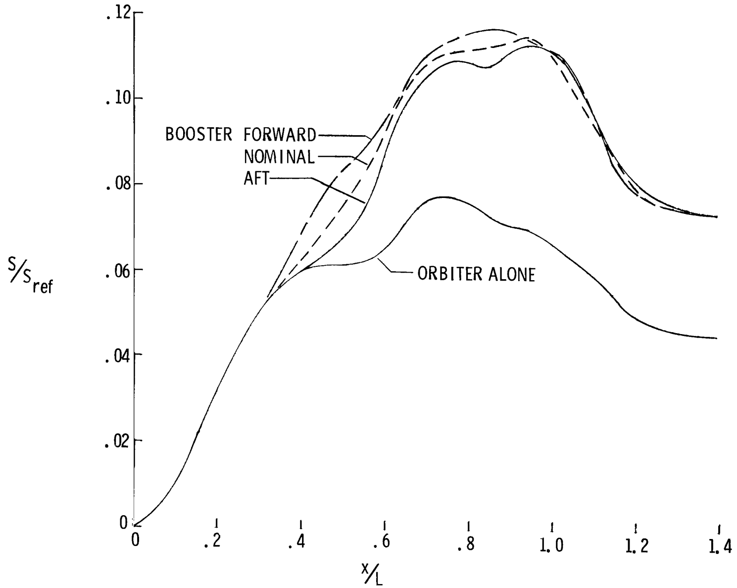
Figure 8.- Equivalent body area distribution for different inboard booster locations. M = 1.50 ; without fins.
