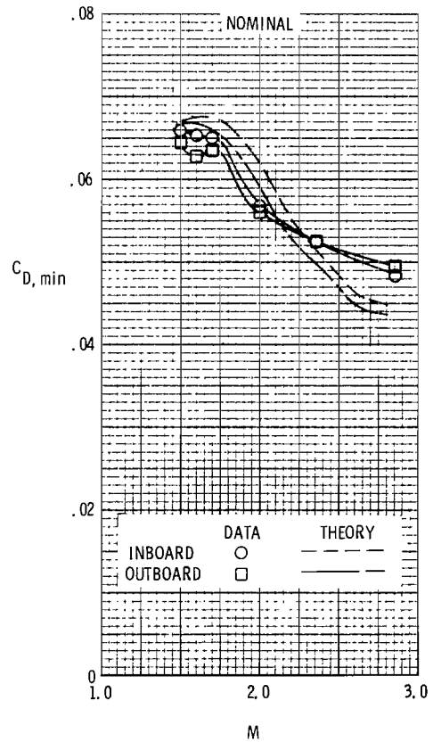
Figure 7.- Booster location effects on minimum drag.
