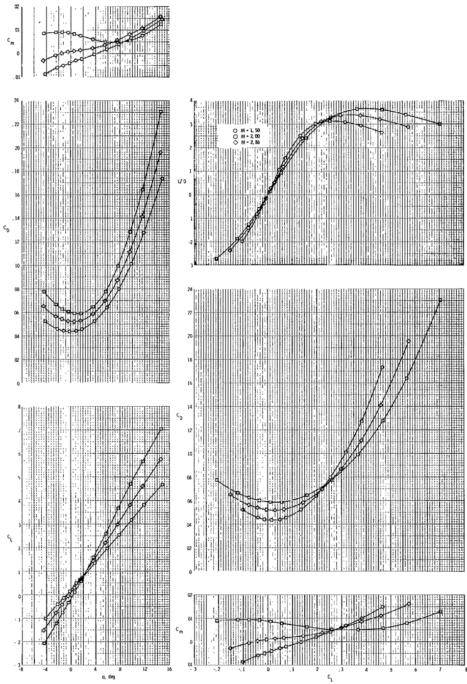
Figure 20.- Experimental aerodynamics at \beta = 0^\circ for O(B+W+S)LW + B(P)IN configuration.
