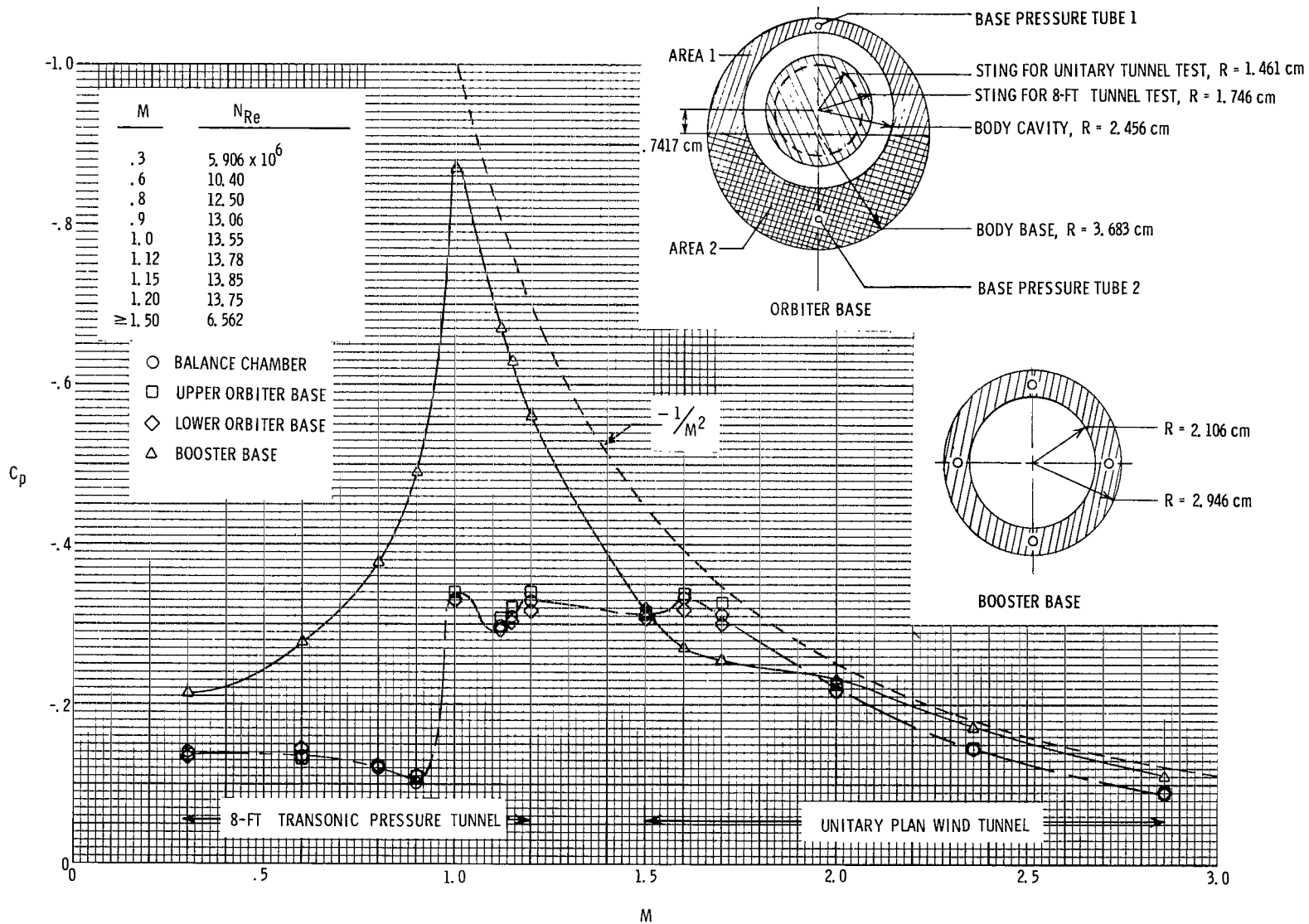
Figure 5.- Base and chamber pressure measurements. \alpha = 0^\circ .
