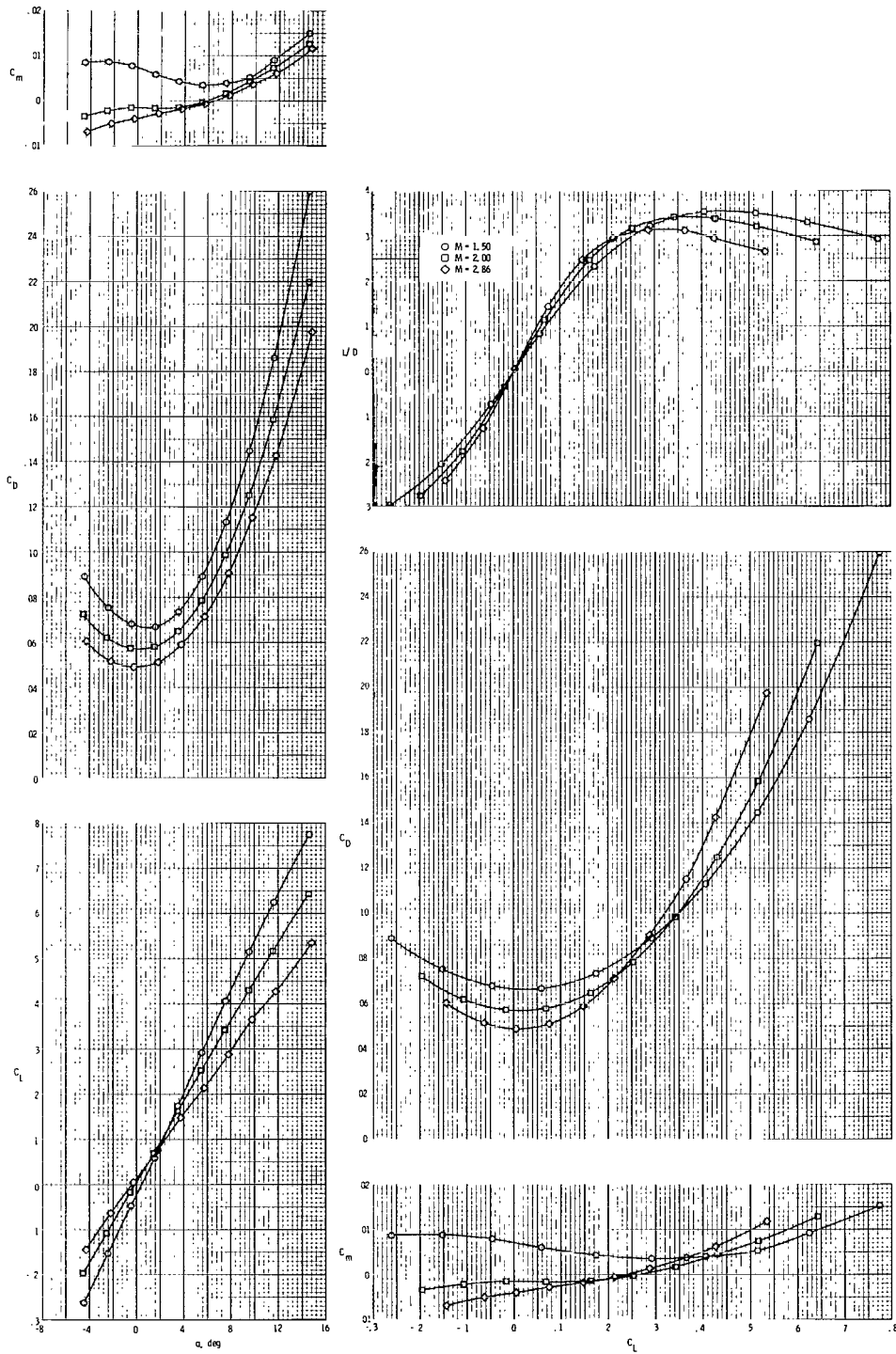
Figure 18.- Experimental aerodynamics at \beta = 0^\circ for O(B+W+S)LW + B(P+W+S)IN configuration.
