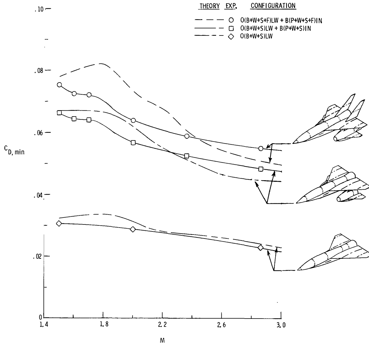
Figure 9.- Effect of configuration buildup on minimum drag.
