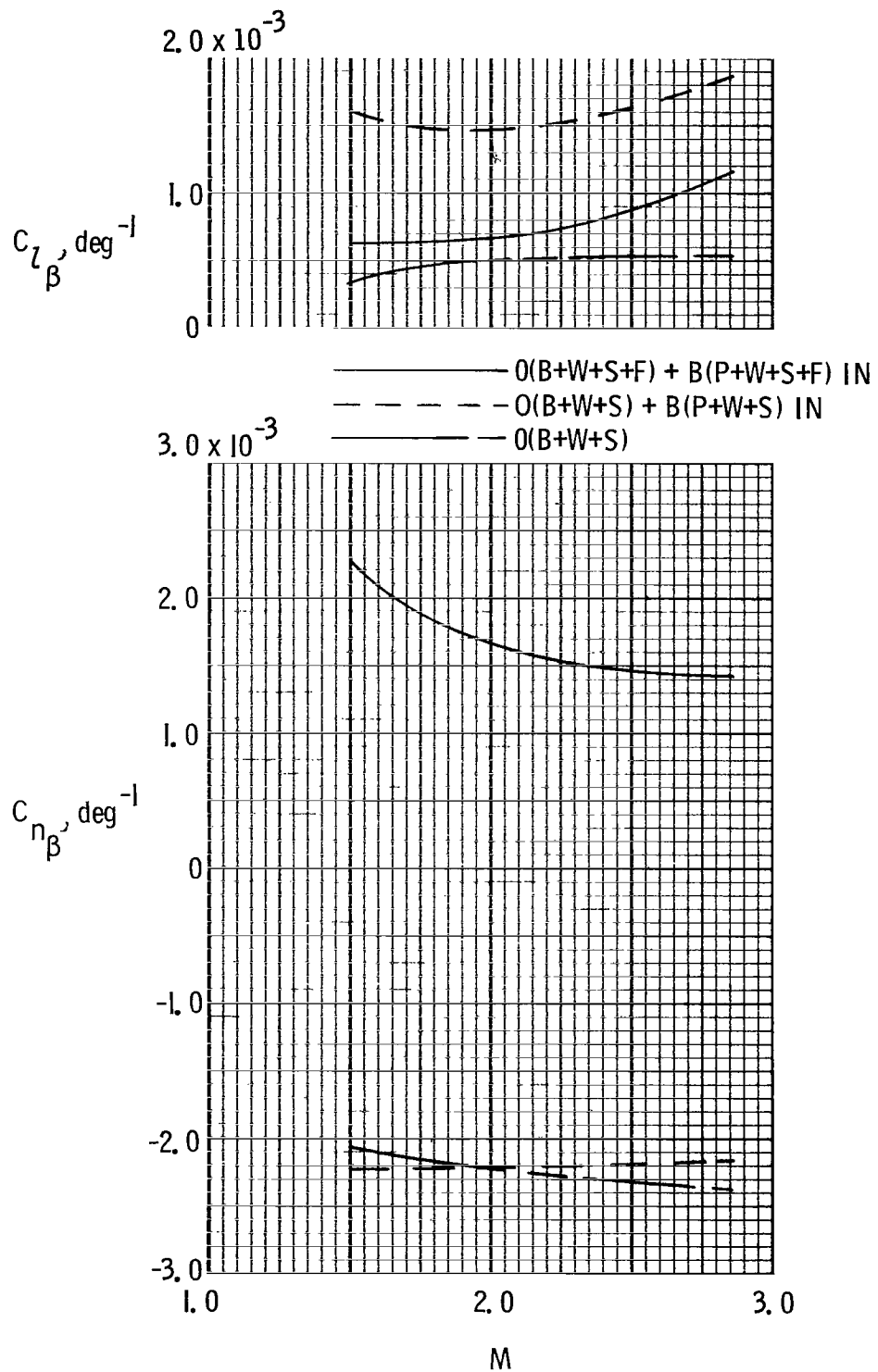
Figure 14.- Lateral-directional experimental characteristics of configuration buildup. \alpha = 0^\circ .
