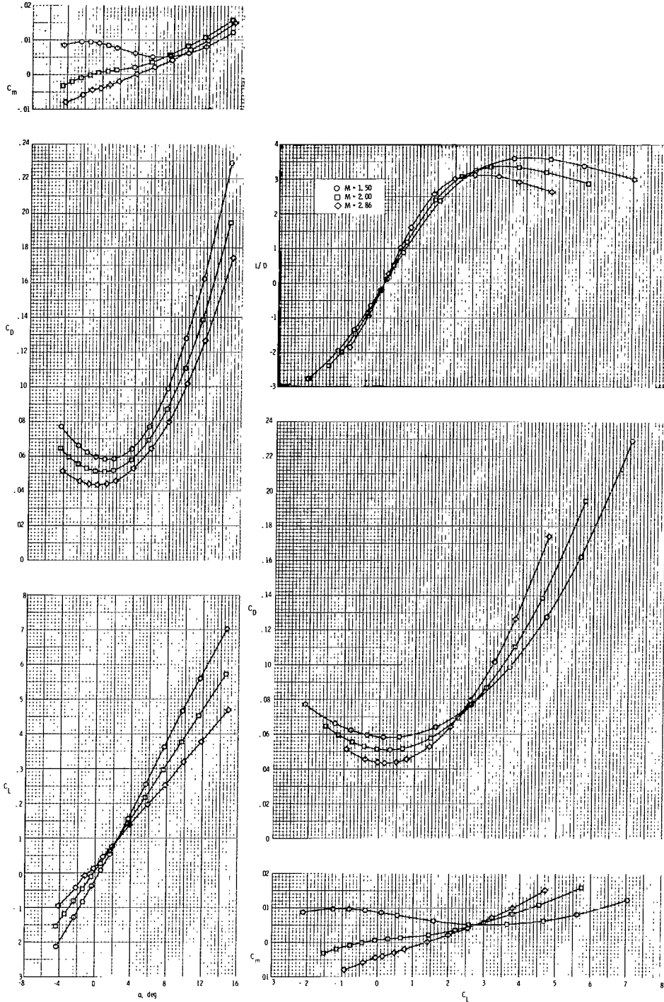
Figure 21.- Experimental aerodynamics at \beta = 3^\circ for O(B+W+S)LW + B(P)IN configuration.
