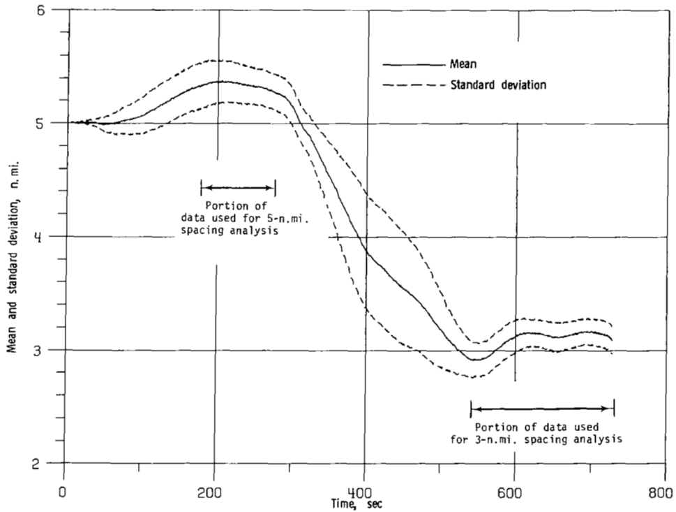
Figure 10.- Mean and standard deviation for 12.7-cm (5.0-in.) display.
