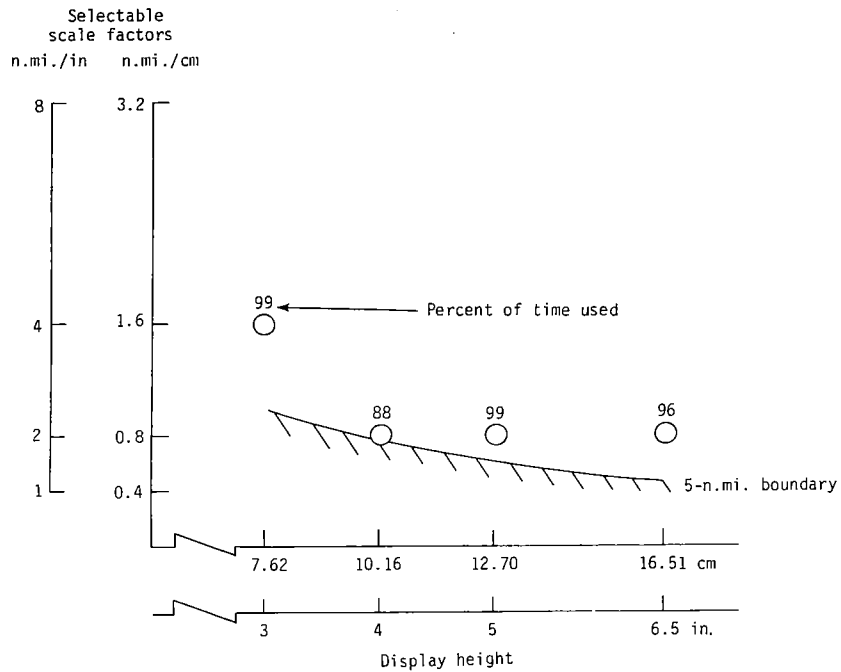
Figure 6.- Preferred map-scale factors for 5-n.mi. self-spacing task.
