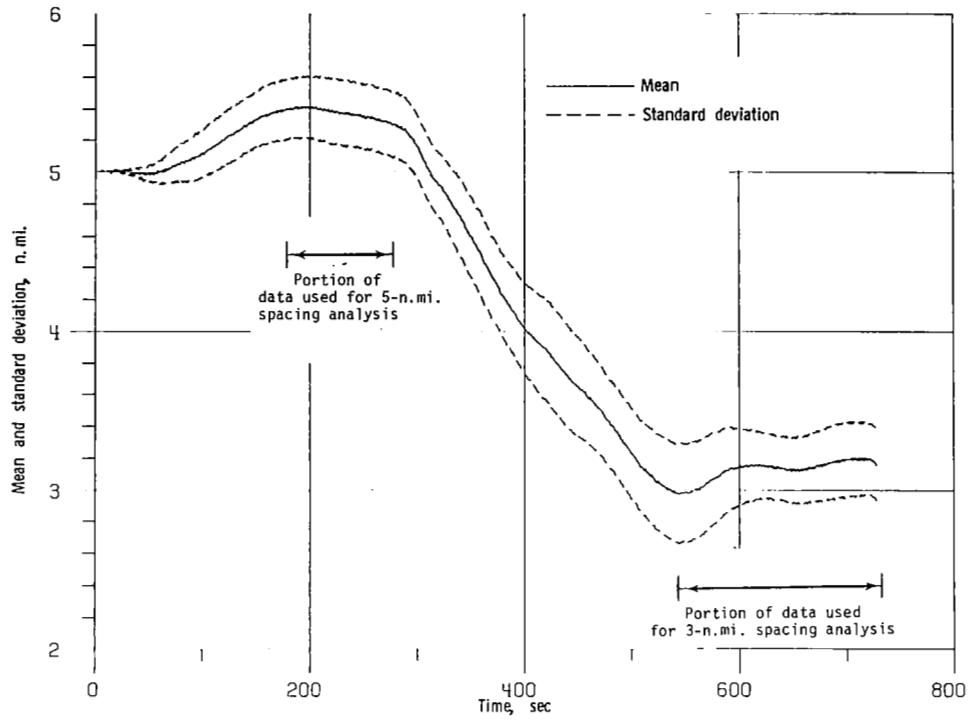
Figure 11.- Mean and standard deviation for 10.16-cm (4.0-in.) display.
