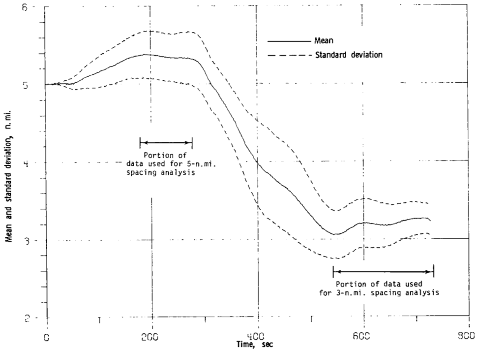
Figure 12.- Mean and standard deviation for 7.62-cm (3.0-in.) display.
