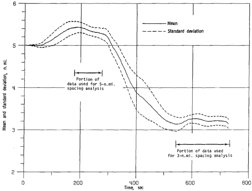
Figure 9.- Mean and standard deviation for 16.51-cm (6.5-in.) display.
