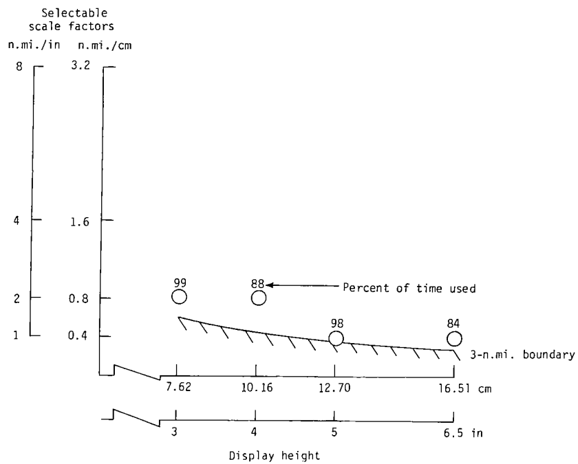
Figure 7.- Preferred map-scale factors for 3-n.mi. self-spacing task.
