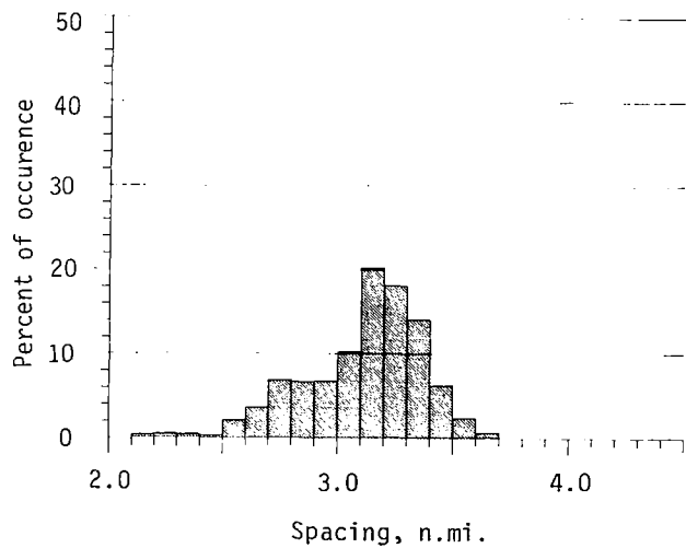
(c) 10.16-cm (4.0-in.) display height.
