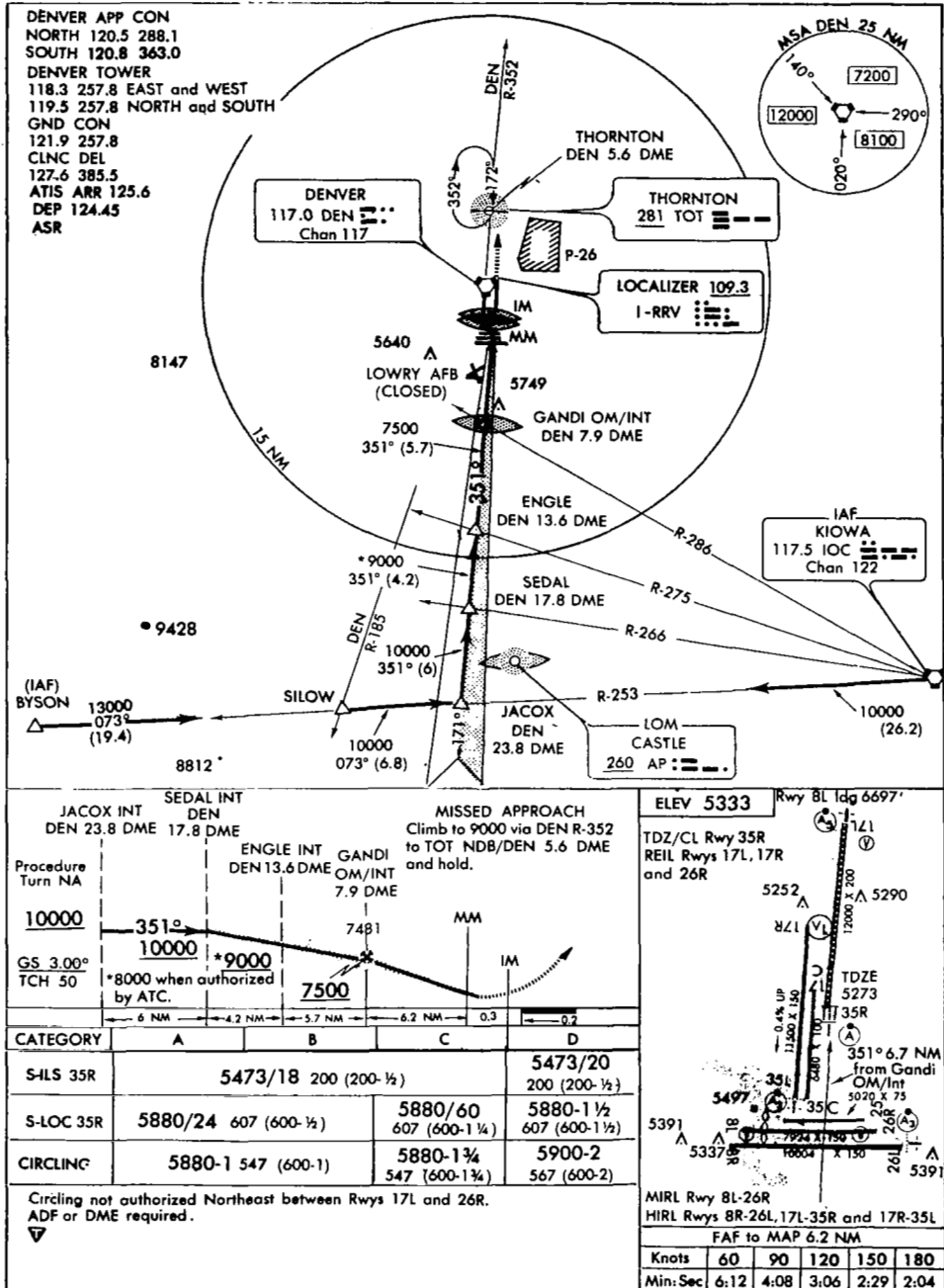
Figure 2.- Approach chart.
